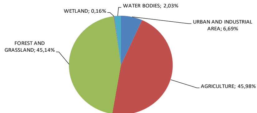
Po river basin land use
