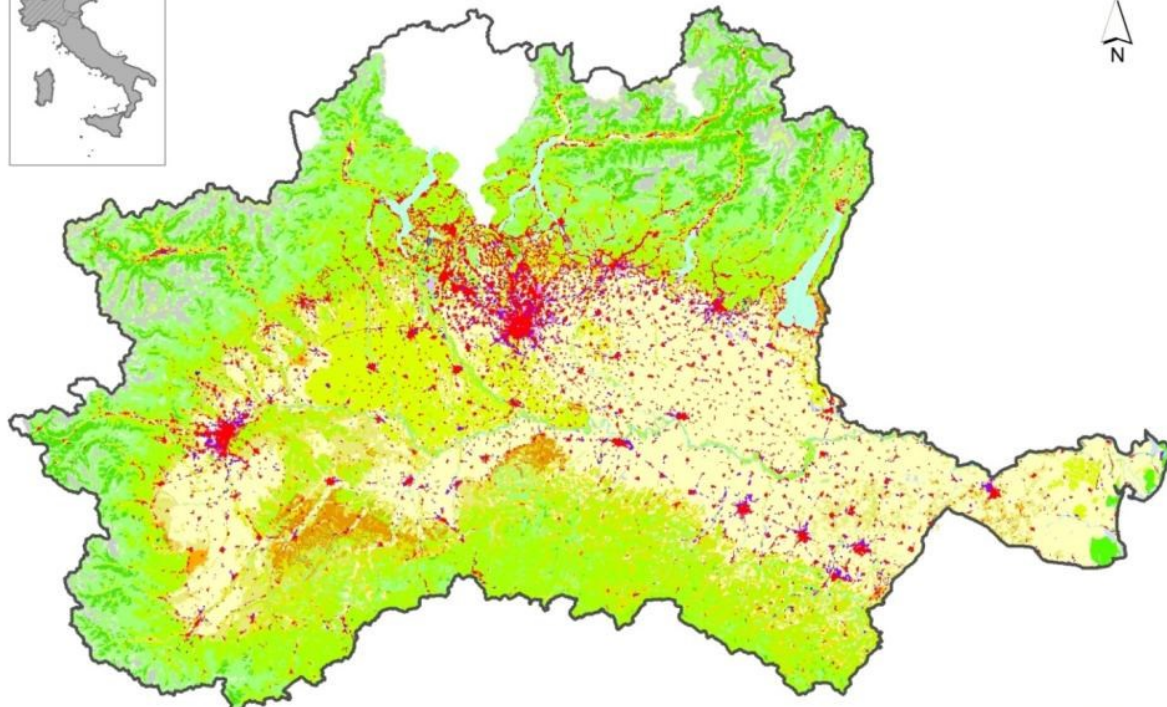
Corine land cover classes
