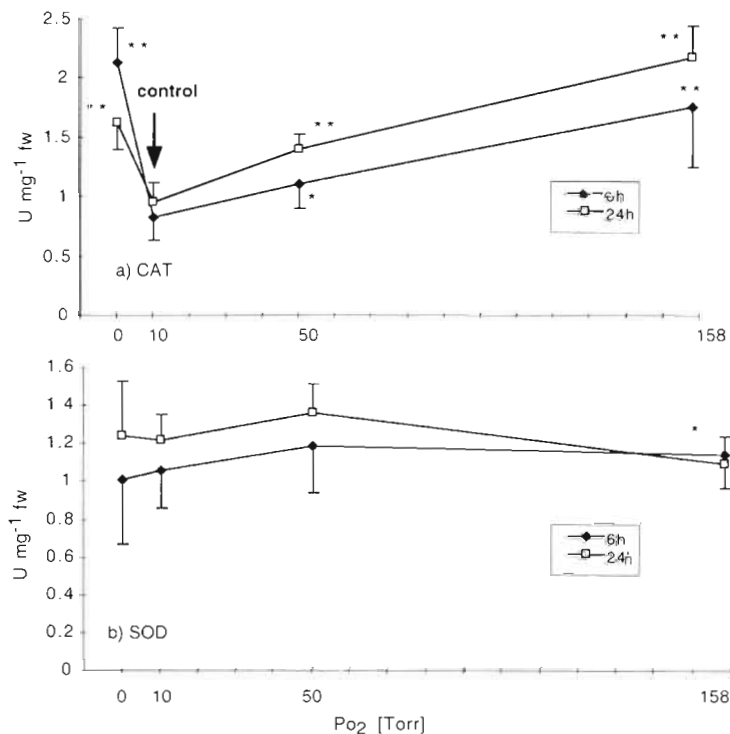
Fig. 3. Heteromastus filiformis . AOE activities in whole body extracts versus P_{O_2} . Winter worms, which had previously been acclimated to 10°C over 7 d, were incubated for 6 h and for 24 h at 15°C in a flow-through chamber without sediment. P_{O_2} was adjusted to 0, 10, 50 and 158 torr with P_{CO_2} = constant = 2.3 torr (0.03%). (a) CAT and (b) SOD after 6 h (◆) and 24 h (□) of incubation. Significant differences from control group: ** p < 0.01 , * p < 0.05 (n = 5)
