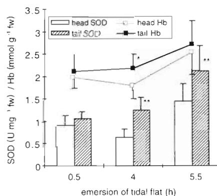
Fig. 7. Heteromastus filiformis . SOD activity (bars) and Hb content (lines) in head versus tail parts of specimens over a tidal emersion period. Both parameters were measured in whole body extracts. Data from 1995, n = 7 or 8 , each sample comprising tissues from 3 or 4 specimens. Significant differences in tail end versus head end: ** p < 0.01 , * p < 0.05
