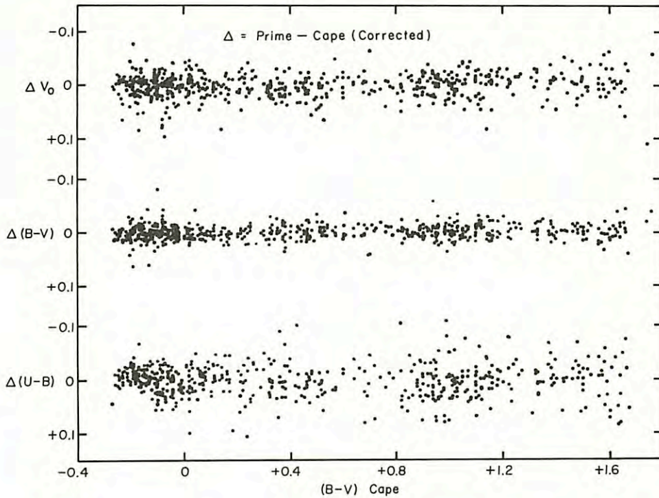
Fig. 7 The comparison of the Prime and the corrected Cape UBV photometry as a function of B-V .
