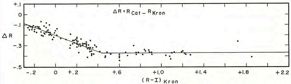
Fig. 12 The comparison of the Catalina R magnitudes with those of Kron and his collaborators.
