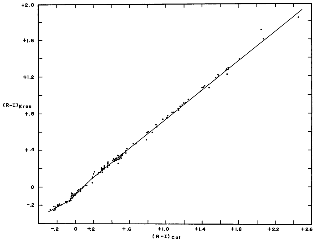
Fig. 13 The comparison of the Catalina R-I colors with those of Kron and his collaborators.
