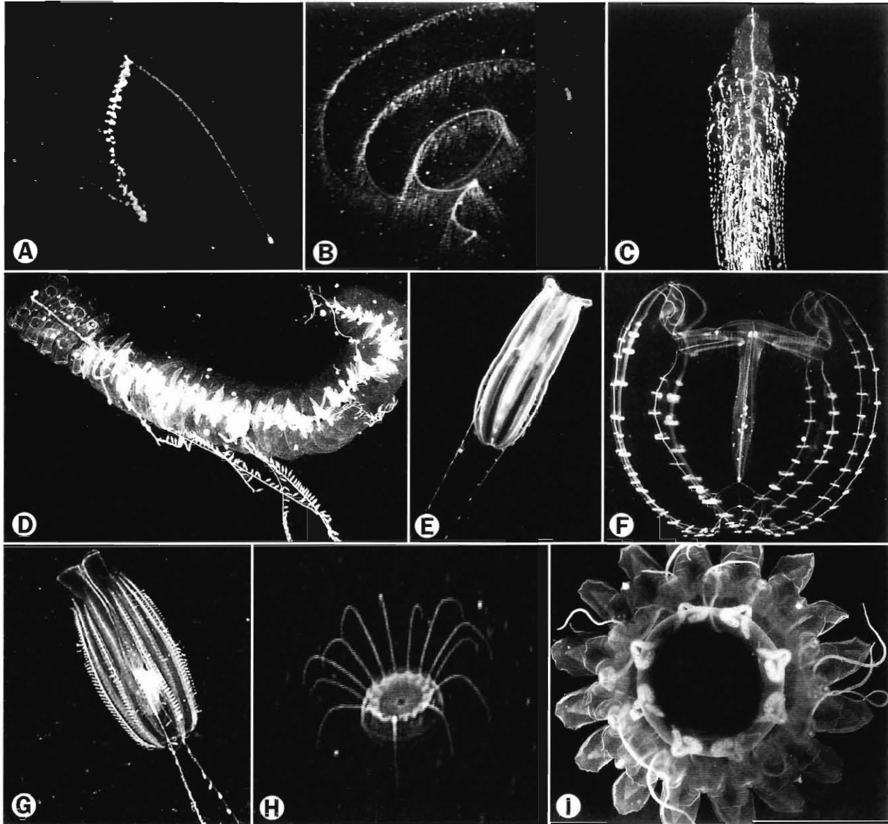
FIG. 3. — Some species of gelatinous zooplankton from the Alborán Sea. (A) Physonect sp. 2 from in situ video, nectosome about 40 cm long, total length about 5 m; (B) Physonect sp. 3 from in situ video, total length 3–4 m; (C) Forskalia sp. 1 photographed live in the ship's laboratory, total length about 30 cm; (D) Agalma clausi photographed live in the ship's laboratory, total length about 8 cm; (E) Lampea pancerina photographed live in the ship's laboratory, body height 30 mm; (F) Deiopea kaloktenota photographed live in the ship's laboratory, body height 44 mm; (G) Euplokamis stationis photographed live in the ship's laboratory, body height about 30 mm; (H) Solmissus albescens from in situ video, bell diameter about 28 mm; (I) Paraphyllina ransoni , preserved specimen, coronal diameter 12 mm.
