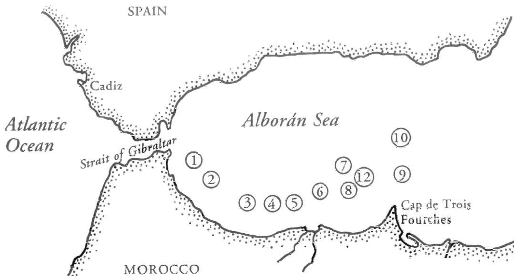
FIG. 1. — Map of the cruise stations for the RV Seward Johnson Alborán Sea cruise, 5-24 April 1991. Numbers 1-12 (there is no Station 11) correspond to the cruise station numbers of Tables 1 and 2.
