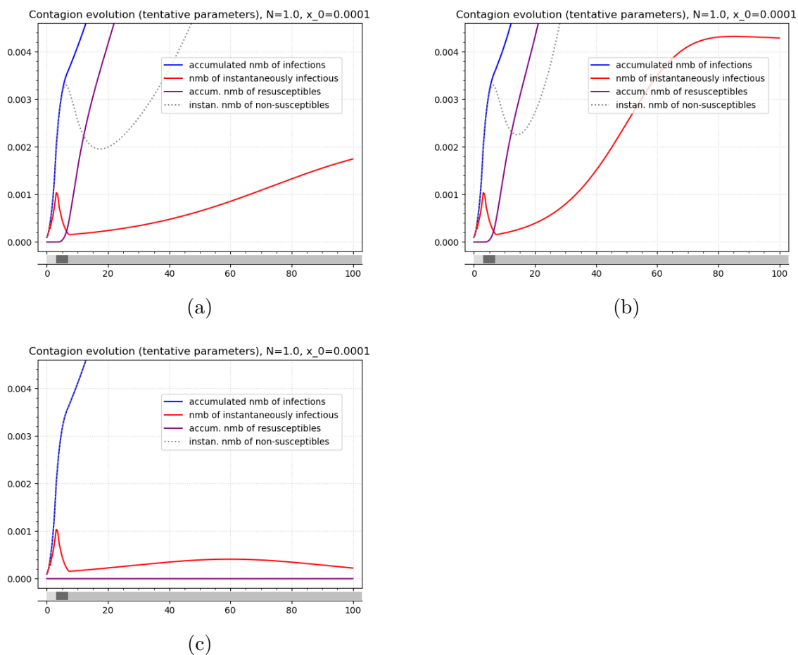
Figure 6: Proliferation evolution with renewed susceptibility possible. Abscissa: time with [0, 1] corresponding to two weeks; ordinate: share of population. The differently shaded regions at the bottom indicate phases of different d \cdot p values. It was chosen d \cdot p = 1.34 until t = 3 , then = 0.77 until t = 7 . For t \geq 7 , it was d \cdot p = 1.02 in Fig a and d \cdot p = 1.04 in Fig b. Both figures assume parameters t_c = 1.0 , t_r = 4.0 , and \alpha_r = 0.2 . For comparison, Fig c shows the otherwise equal scenario as in Fig a, but without resusceptibility (i.e. \alpha_r = 0 ). Not depicted: In Fig b, the number of instantaneously non-susceptibles converges to about 3.9% of the population as t \rightarrow 100.0 ; the number of ever infected at that time is about one fourth of the population.
