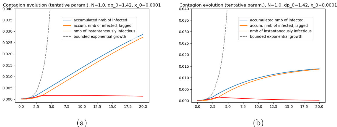
Figure 4: (a) Solution for a parameter choice such that x(t) shows a pronounced phase of nearly linear growth: it was d \cdot p = 1.42 initially, then d \cdot p = 1.02 from t = 3.0 onwards. Not depicted: Also with this parameter choice the x(t) eventually converges: the linear growth phase extends until about t = 25.0 , and finally it is x(\infty) \approx 0.04948 . (b) Solution obtained when using the same initial conditions, but switching to d \cdot p = 0.96 at t = 3.0 .
