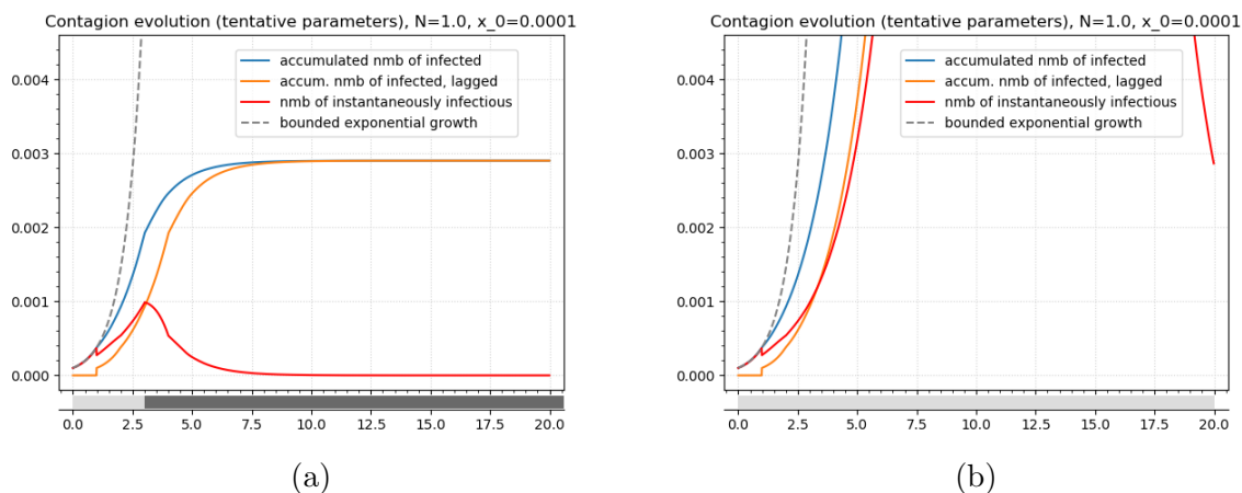
Figure 3: Tracing reported CoViD-19 infections in Germany. As in Figures 1 and 2, the ordinate values denote the share of total population. The time scale is chosen such that [0, 1] corresponds to two weeks. (a) As Fig 2, but using initial value x_0 = 0.0001 and initial d \cdot p = 1.34 . For t \geq 3 the d \cdot p is 0.65. The simulation yields x(\infty) \approx 0.00290 . (b) Shows the evolution as would occur if the parameter switch at t = 3.0 was omitted. Then x(\infty) \approx 0.44520 .
