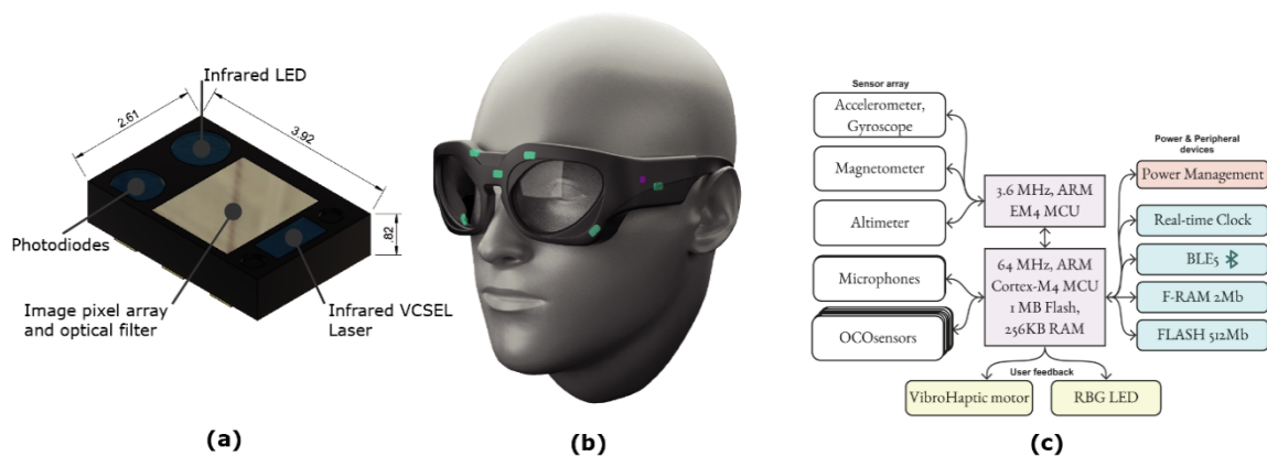
FIGURE 1. (a) shows a 3D render showing a future OCO™ sensor application specific integrated circuit (ASIC) and its dimensions and fundamental components. (b) shows a 3D-render of the OCO™ glasses on an average head model. The OCO™ sensors (green rectangles), and the IMU (purple rectangle) are highlighted on the model. (c) diagram showing the main electronics components within the OCOsense™ glasses.
