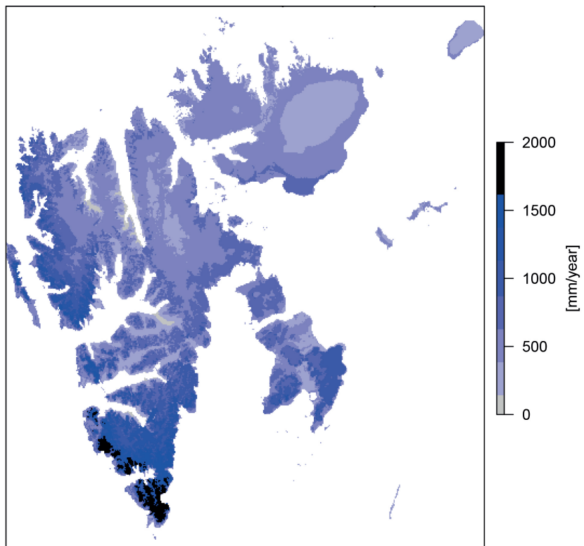
Figure 5.1.2 Annual runoff (absolute values in mm/year) averaged over 1971–2000 based on the ensemble median of eight HBV simulations driven with down-scaled Arctic CORDEX RCPs for the control period.
