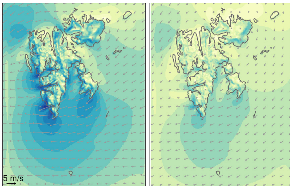
Wind speed [m/s] and direction
