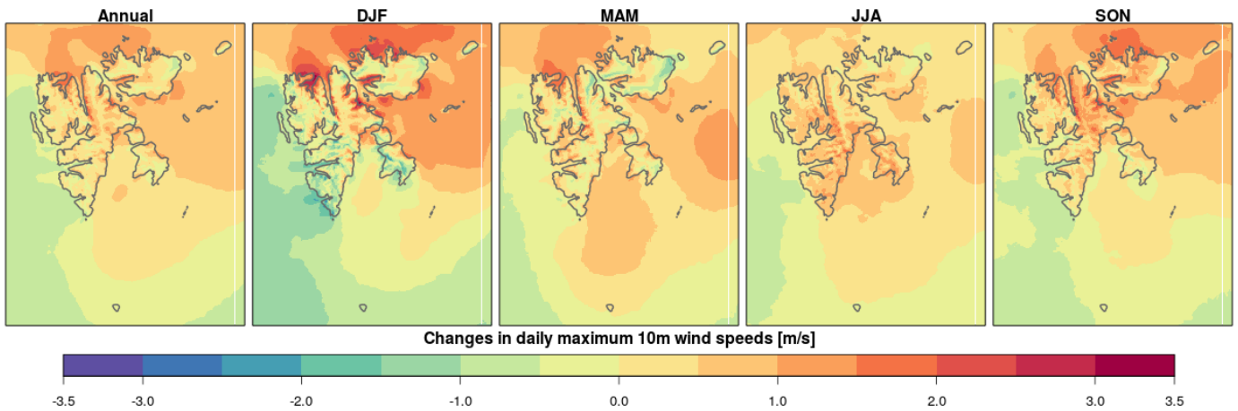
Figure 4.5.3. Annual and seasonal changes of daily maximum wind speed from 1971-2000 to 2071-2100. The estimates are based on the CCLM 2.5 km run for emission scenario RCP8.5.
