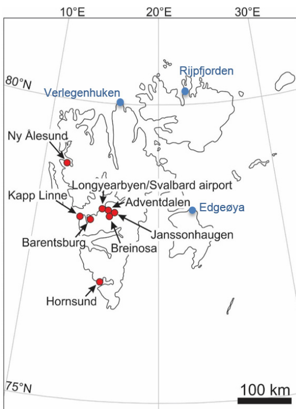
Figure 7.1.1. Location of the active permafrost observations in Svalbard (red dots, Table 7.1.1) and location of additional sites where meteorological stations exist and where permafrost modelling have been performed (blue dots). Figure from Christiansen et al., (2019a).
