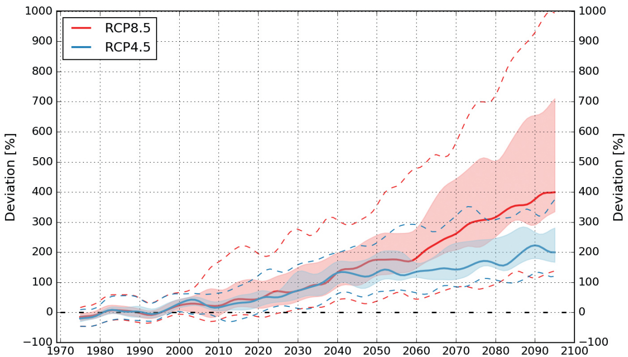
Mean annual runoff - Svalbard
