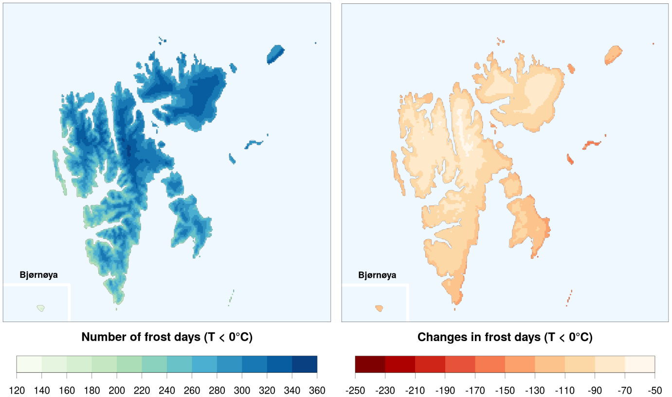
Figure 4.2.2: Average number of frost days per year in the control period 1971-2000 (left), and projected change from 1971-2000 to 2071-2100 (right) according to CCLM under the RCP8.5 emission scenario.
