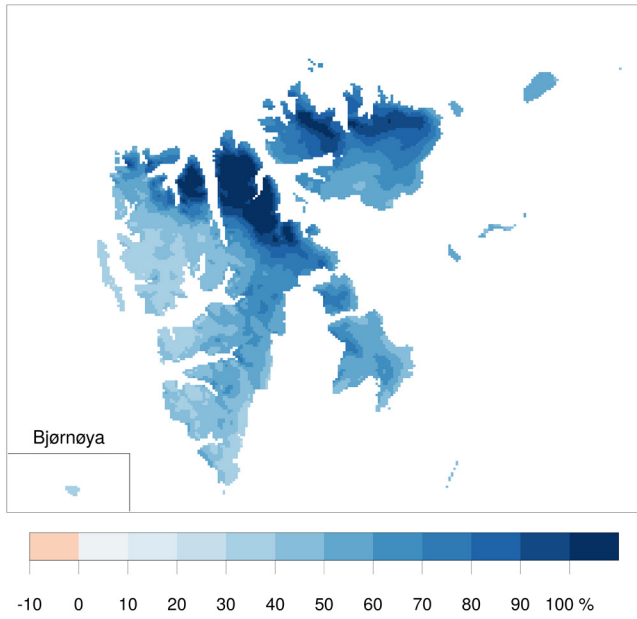
Figure 4.3.7. ‘Ensemble mean precipitation changes [%] from 1971-2000 to 2071-2100 in the Artic CORDEX simulations assuming the RCP8.5 emission scenario. The spatial resolution is improves by scaling with the signal from the CCLM simulation (cf. Chapter 3.1.4). Upper panel: Annual values. Lower panel: Summer (left) and winter (right).
