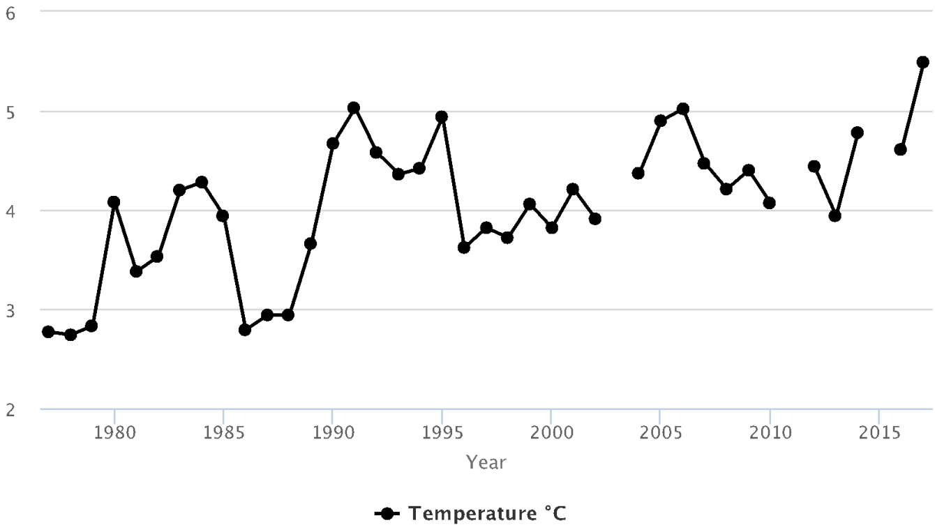
Figure 8.1.2 Sea surface temperature of Atlantic Water in the Sørkapp section in the northern Norwegian Sea (Institute of Marine Research, ICES data, www.imr.no ).
