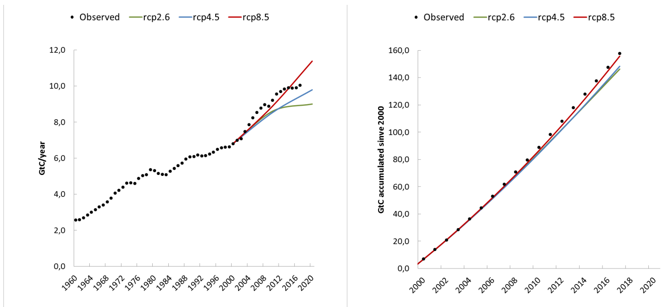
Figure 9.3.1: a) Global emissions of CO 2 (from fossil fuel and cement production ) given in billion tons of carbon per year from 1959 to 2017 (dots) and the three emission scenarios RCP2.6 (green), RCP4.5 (blue) and RCP8.5 (red) from 2000 to 2020. b) Accumulated emissions of CO 2 over the 17 years the emission scenarios have existed. Observationally based data taken from the Global Carbon Budget project (Le Quéré et al 2018).
