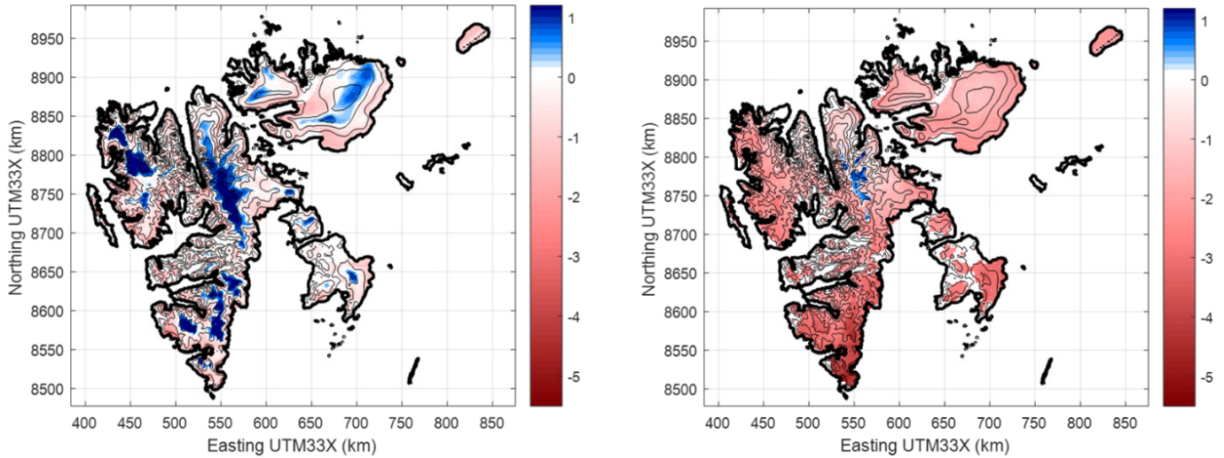
Figure 6.6.2: Mean mass balance (m w.e. yr -1 ) simulated for the time periods a) 1971-2000 and b) 2071-2100.
