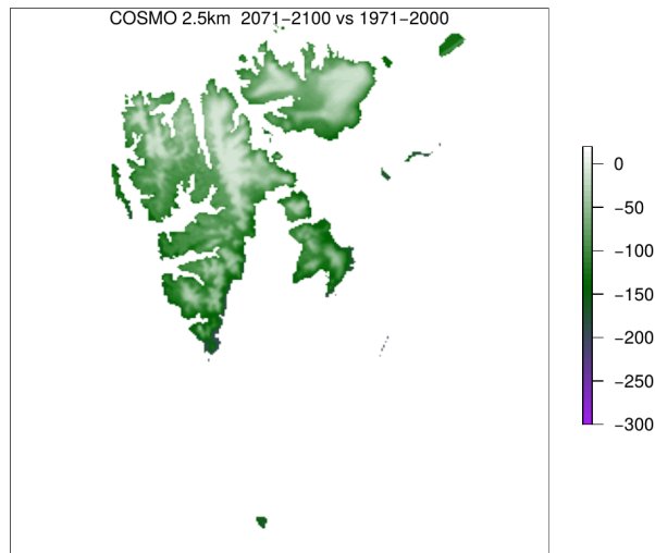
Snow days: Absolute difference
