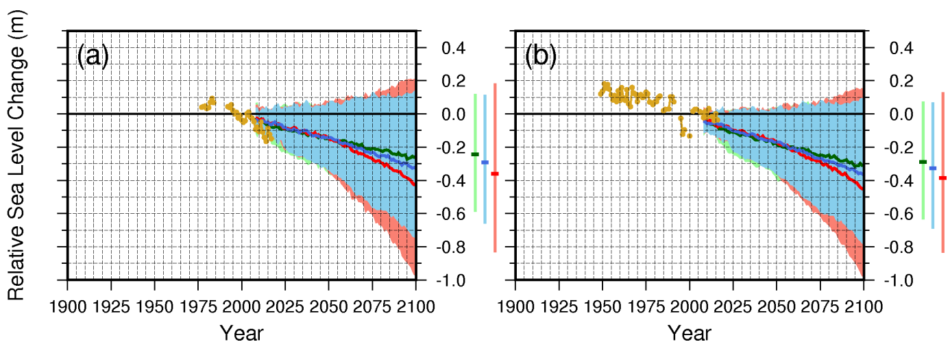
Figure 8.4.5. Relative sea-level projections for RCP2.6 (green), RCP4.5 (blue) and RCP8.5 (red) for (a) Ny-Ålesund and (b) Barentsburg. The vertical bars on the right side of the panels represent the ensemble mean and ensemble spread (5% to 95%) for RSL change for 2081–2100. Annual mean tide gauge observations are shown in yellow.
