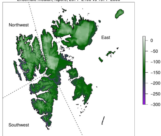
Snow days: Absolute difference
