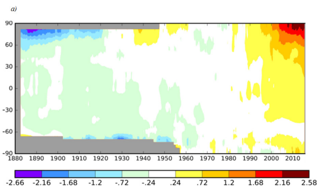
Figure 2.3.1: 5-years zonal mean temperature anomalies (°C) compared to the 1961-1990 normal (a) and temperature trends (°C) from 1950-2017 (b). Data from NASA Goddard Institute for Space Studies (NASA GISS).
