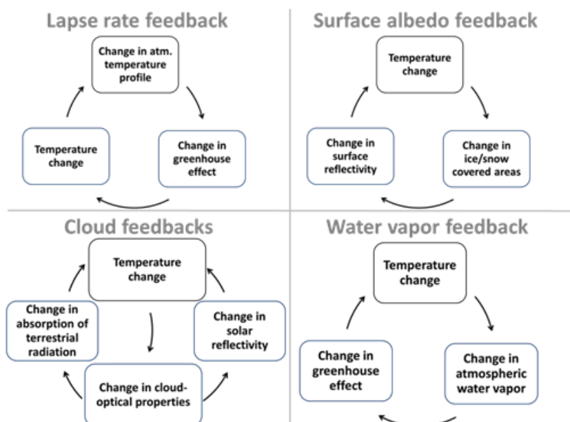
Figure 2.3.2: Four important radiative feedbacks.
