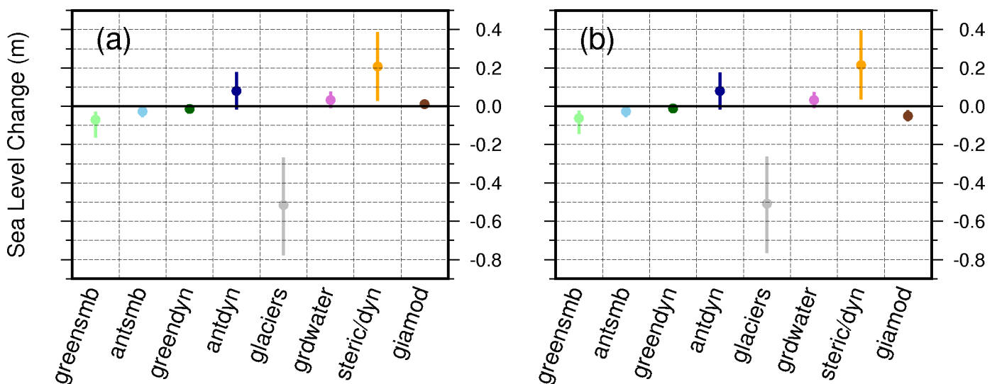
Figure 8.4.6. Contributions to projected relative sea-level change for RCP4.5 over the period 1986–2005 to 2081–2100 for (a) Ny-Alesund (b) Barentsburg. The ensemble mean and spread (5% to 95%) are shown by the circles and vertical bars, respectively.
