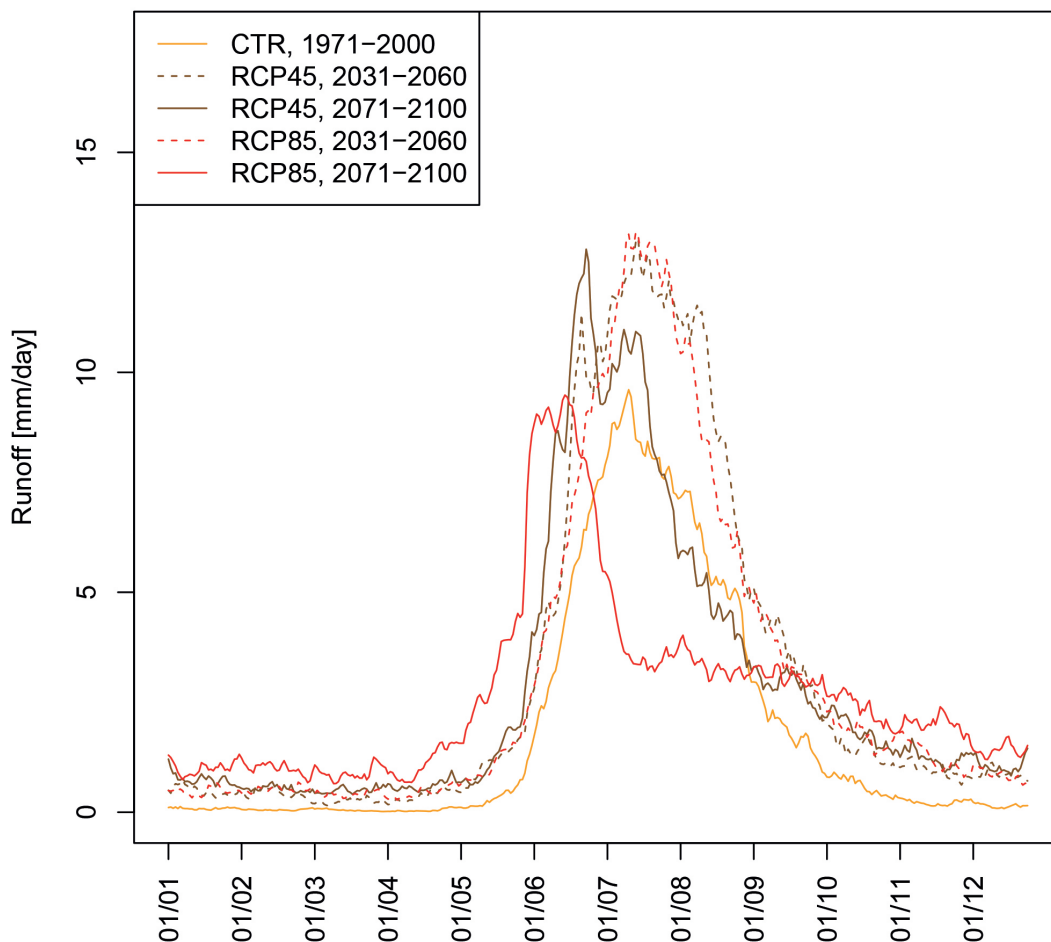
Seasonal runoff distribution, Longyearlva
