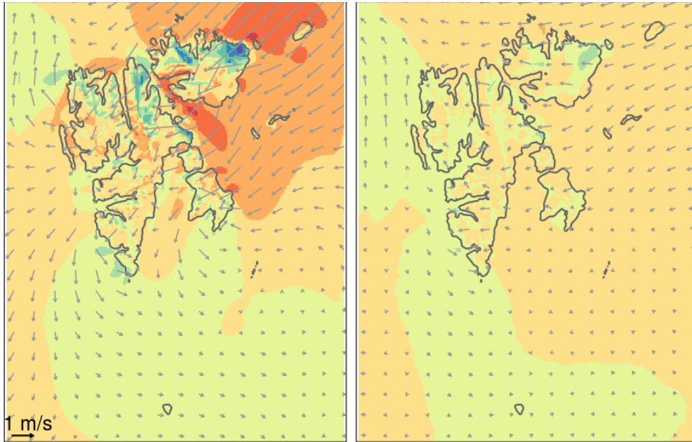
Changes in wind speed [m/s] and direction
