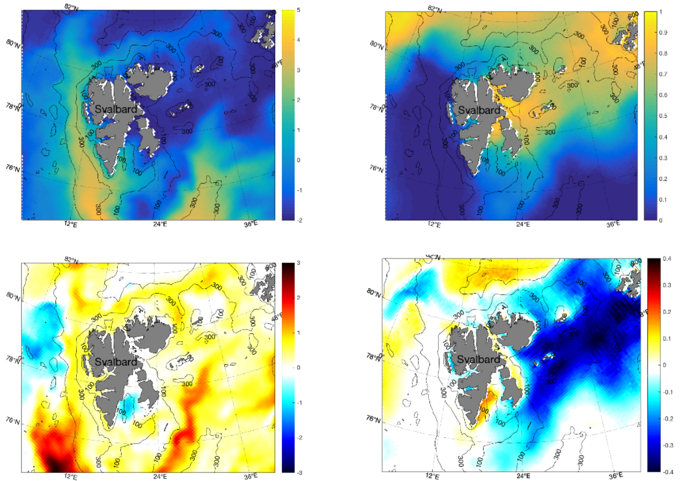
Figure 8.1.3 Simulated sea surface temperature ( ^{\circ}\text{C} , left) and sea ice concentration (fraction, right) from March in the present climate (upper) and change in the future (lower) of the RCP4.5 scenario. The present and future periods are averages from the years 2010-19 and 2060-69, respectively.
