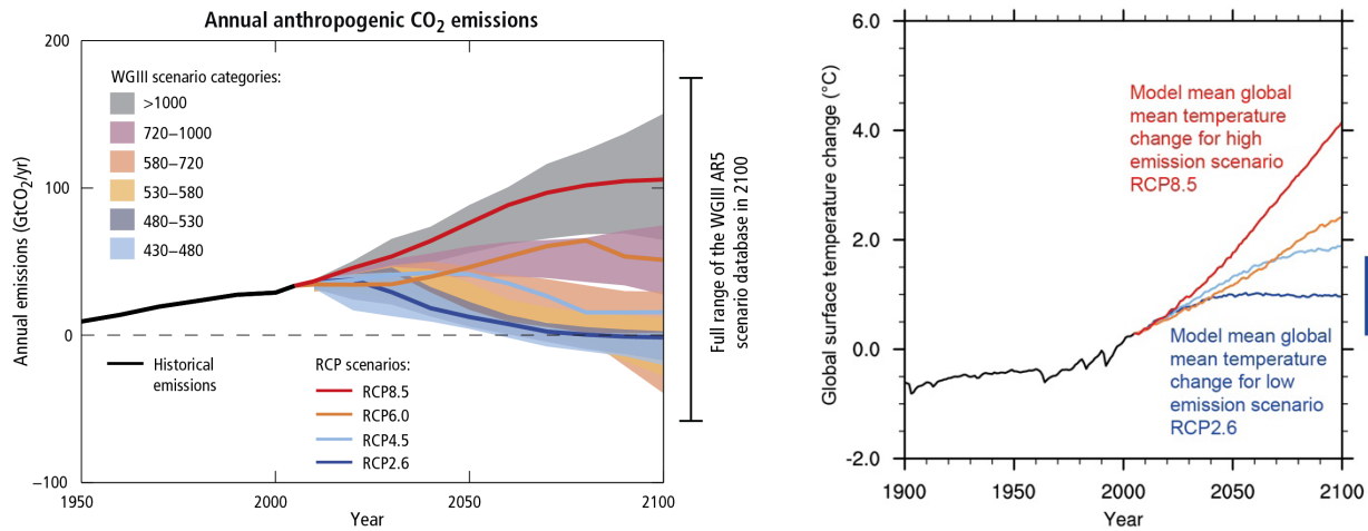
Figure 3.1.3 (left) Historical and projected annual greenhouse gas emission pathways in gigaton carbon dioxide per year from 1950 until 2100 according to four scenarios (IPCC, 2013); (right) annual global mean temperature anomalies w.r.t. the 1986-2005 global average (IPCC, 2013).
