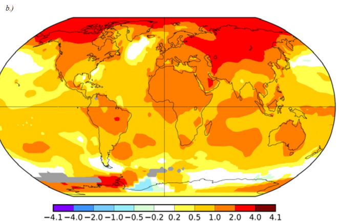
Figure 2.3.1: 5-years zonal mean temperature anomalies (°C) compared to the 1961-1990 normal (a) and temperature trends (°C) from 1950-2017 (b). Data from NASA Goddard Institute for Space Studies (NASA GISS).
