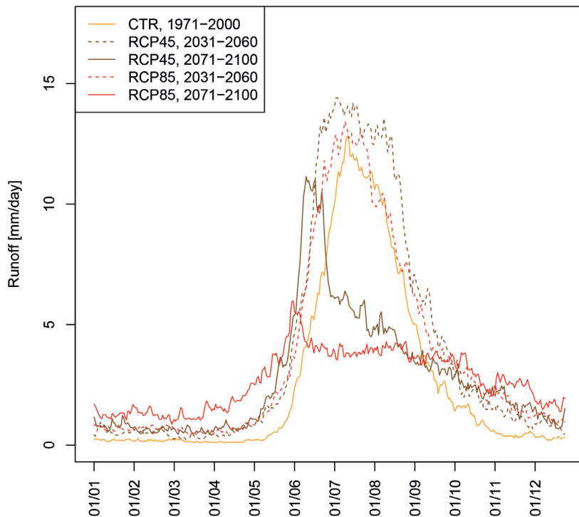
Seasonal runoff distribution, Bayelva
