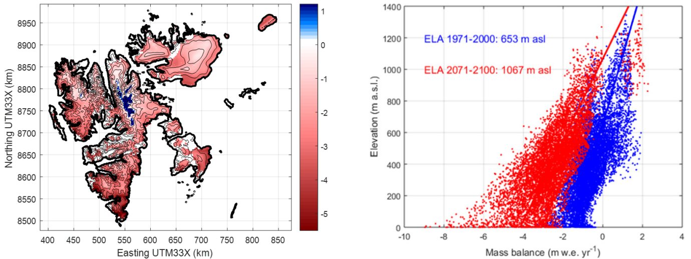
Figure 6.6.3: Change in mass balance (m w.e. yr -1 ) between the two time periods 1971-2000 and 2071-2100. a) Spatial change. b) Change as a function of elevation. ELA denotes the mean equilibrium line altitude determined from linear regression.
