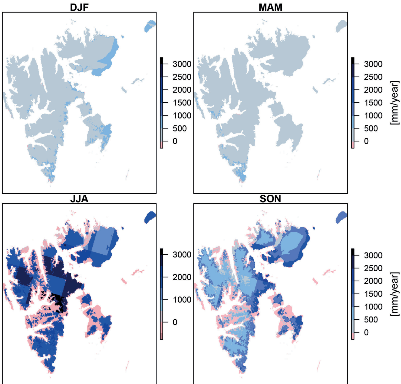
Figure 5.1.9 Projected mean seasonal runoff changes [mm] in the HBV simulations (RCP8.5) for the time period 2071–2100 compared to 1971–2000. Absolute values in mm/year. Note the different scales. The reason why large-scale squares are visible in the figure is explained in Box 5.2.
