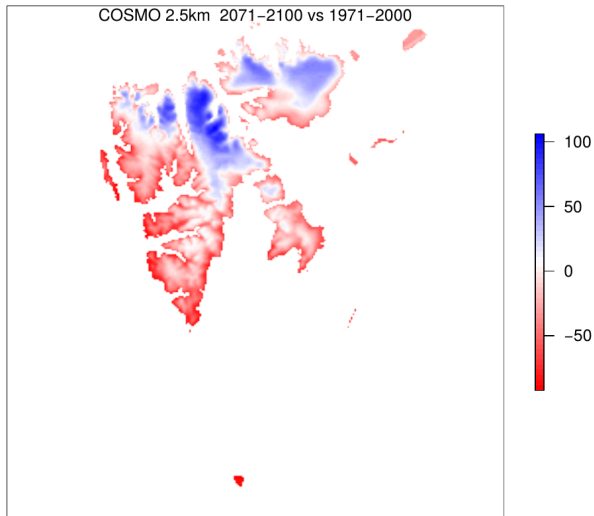
Relative difference max SWE (%)
