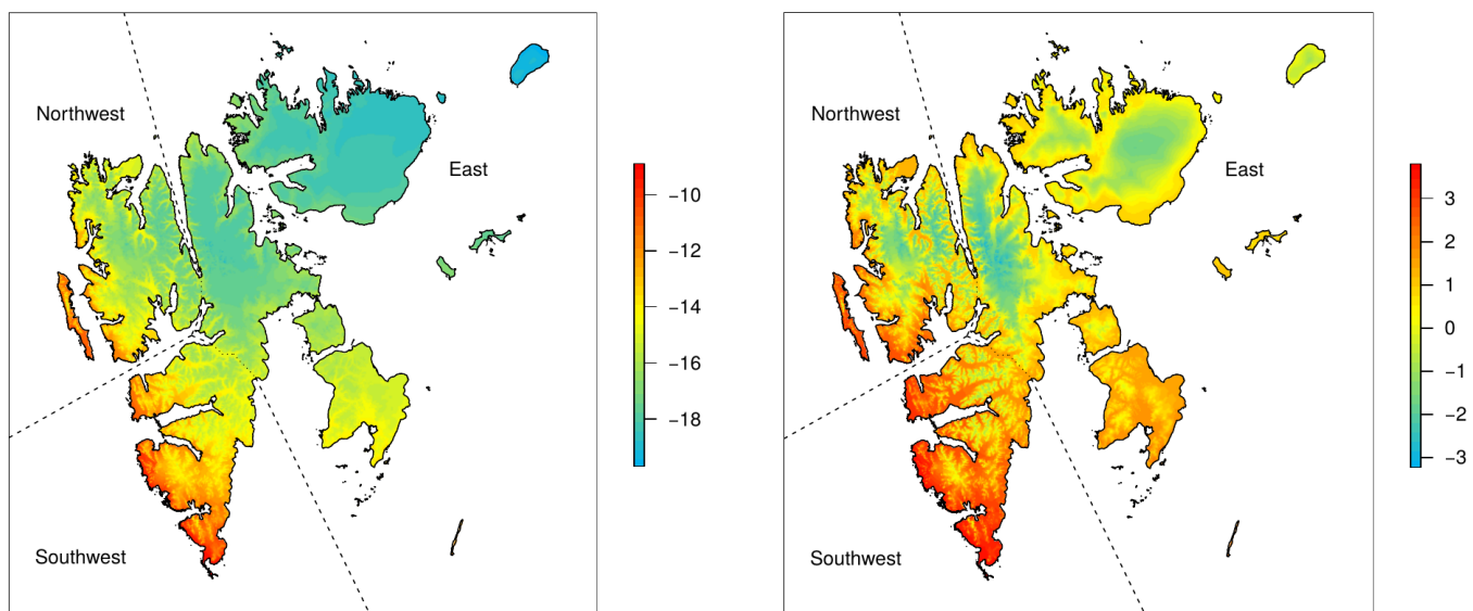
Figure 4.1.2. Winter (Dec-Jan-Feb; left) and summer (Jun-Jul-Aug; right) temperature [ ^{\circ}\text{C} ] averaged over 1971-2000 based upon the Sval-Imp dataset. Note that the colour scales are different!
