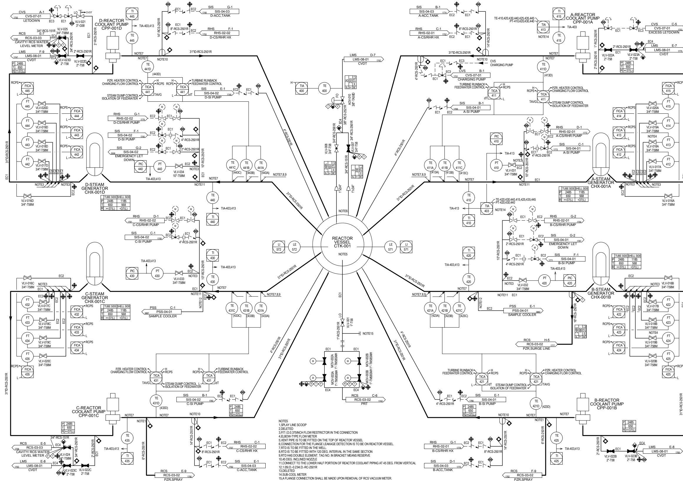
Figure 5.1-2 Reactor Coolant System Piping and Instrumentation Diagram (Sheet 1 of 3)
