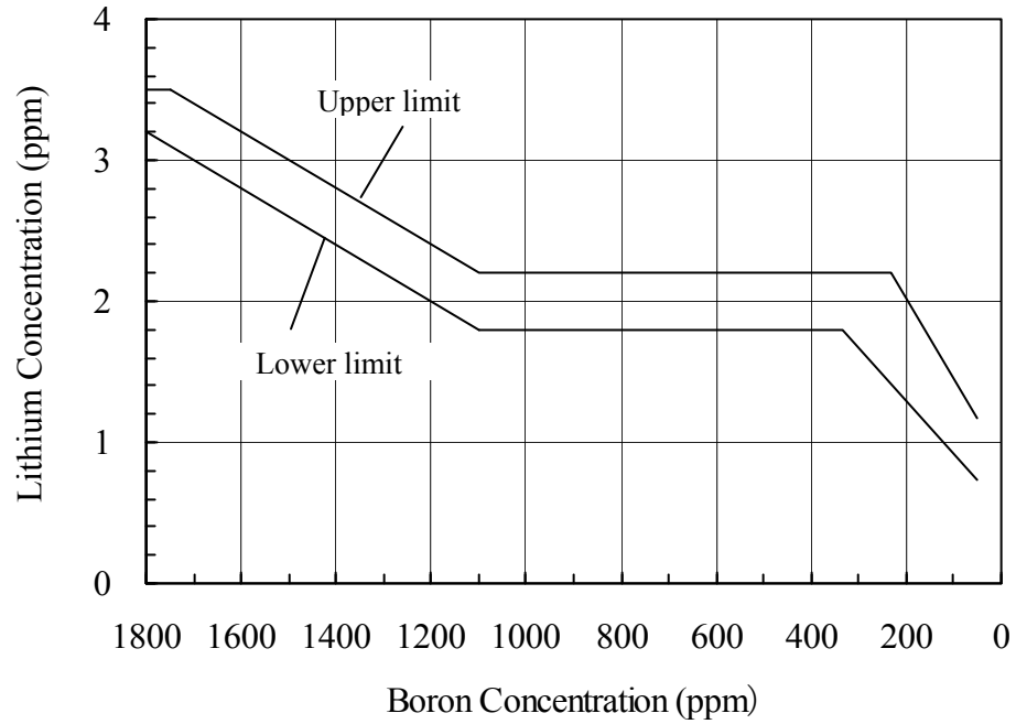
Figure-5.2.3-1 Lithium Control Band
