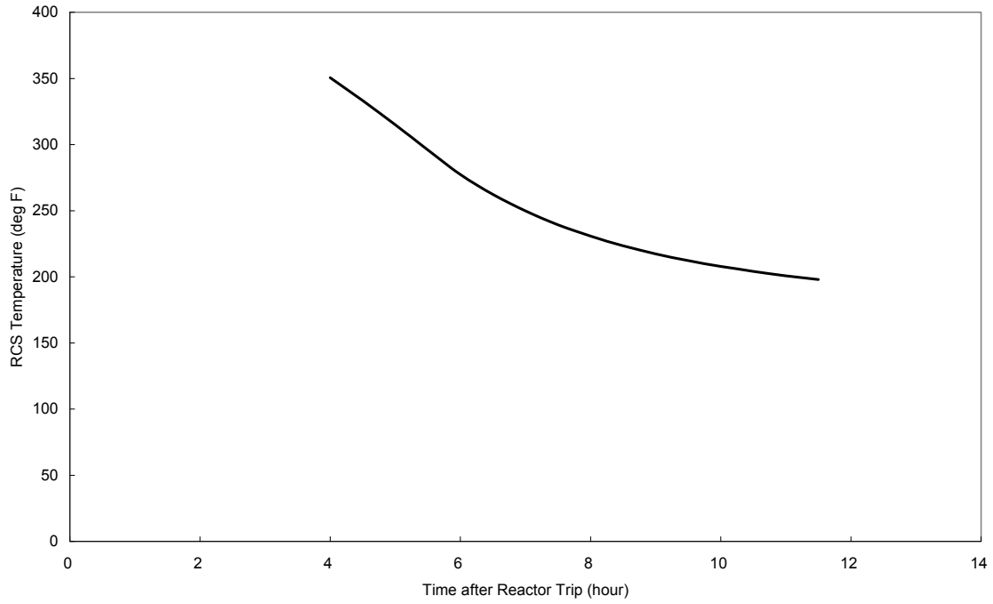
Figure 5.4.7-6 RCS Temperature Transient Curve (Safe Shutdown)
