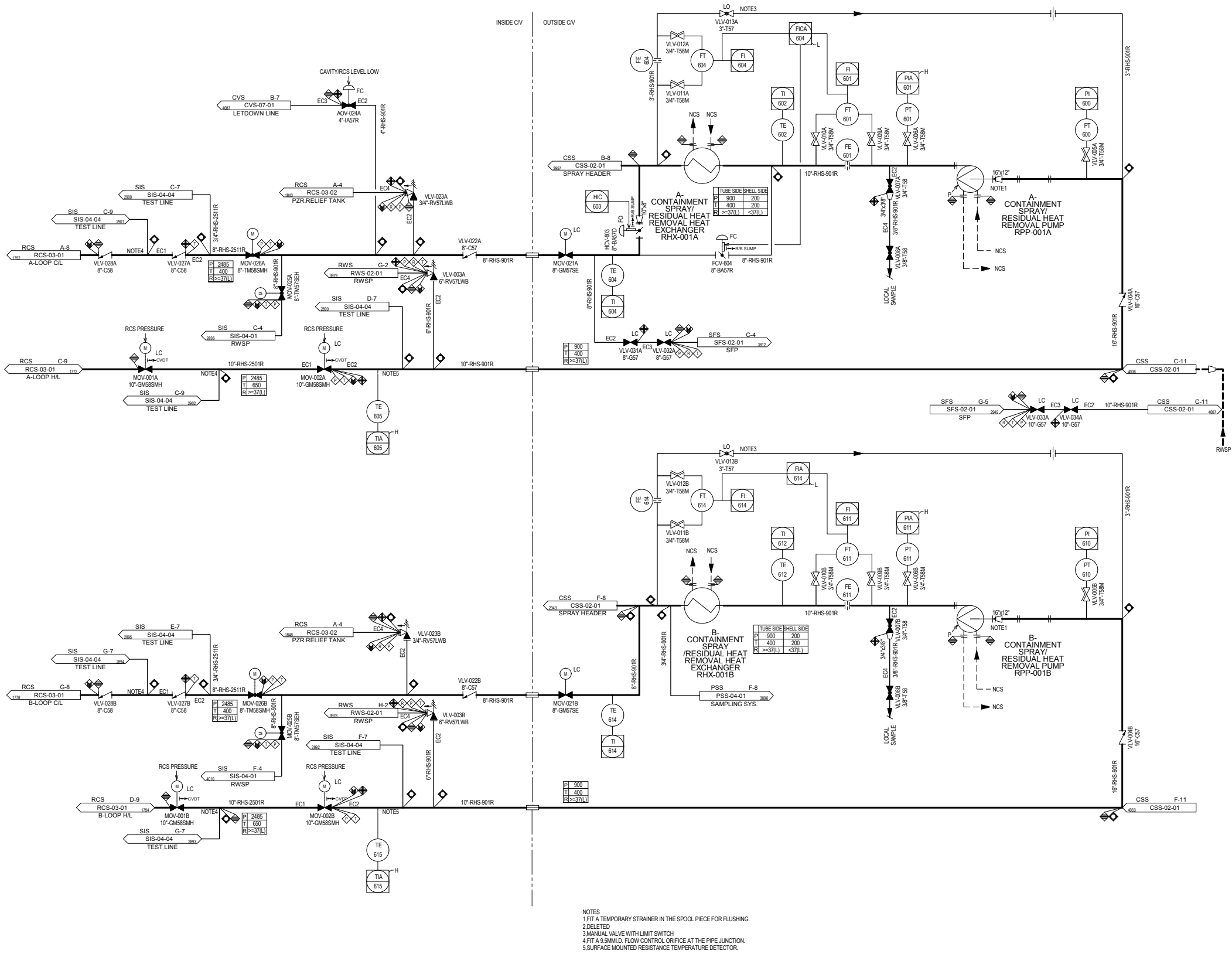
Figure 5.4.7-2 Residual Heat Removal System P&ID (Sheet 1 of 2)
