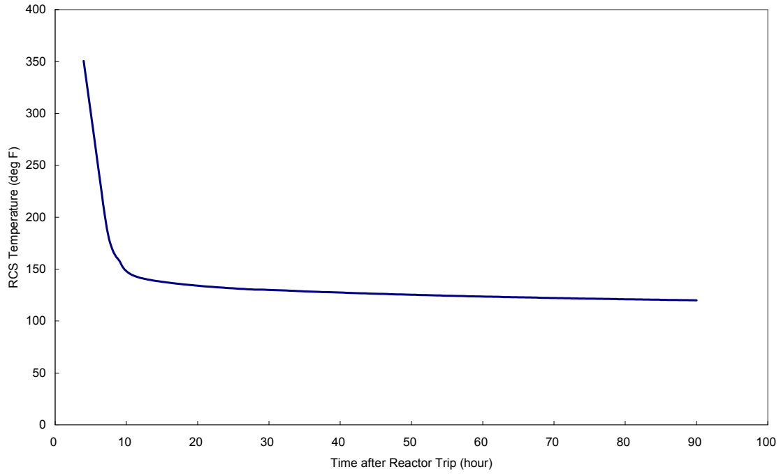
Figure 5.4.7-5 RCS Temperature Transient Curve (Normal Shutdown)
