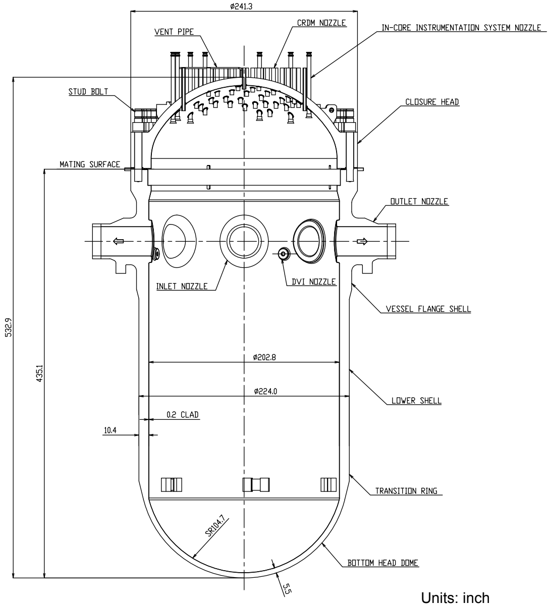
Figure 5.3-4 Reactor Vessel Side View
