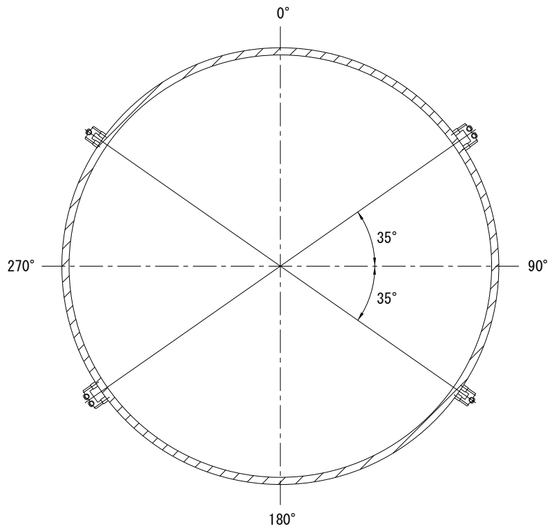
Figure 5.3-1 Orientation of Surveillance Capsules
