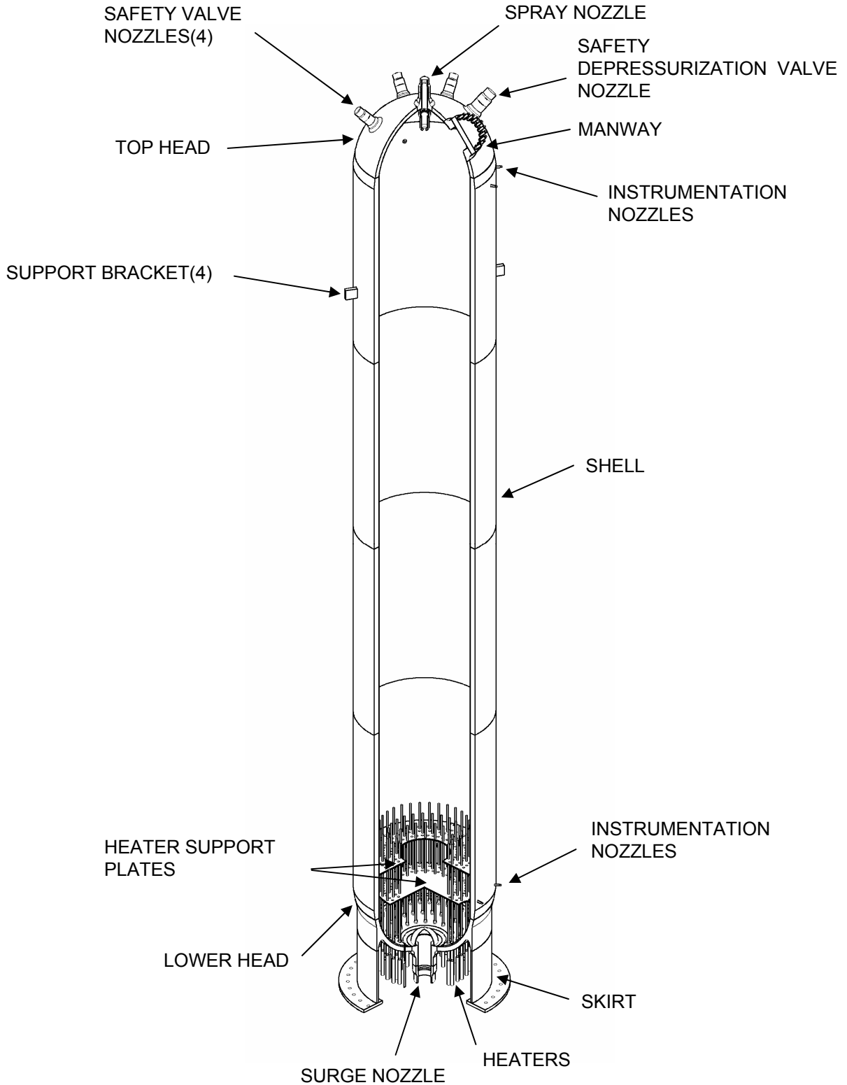
Figure 5.4.10-1 Pressurizer
