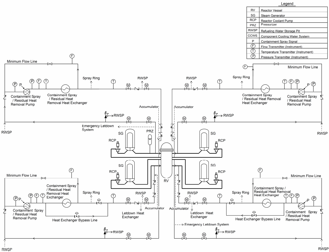
Figure 5.4.7-1 Residual Heat Removal System Flow Diagram
