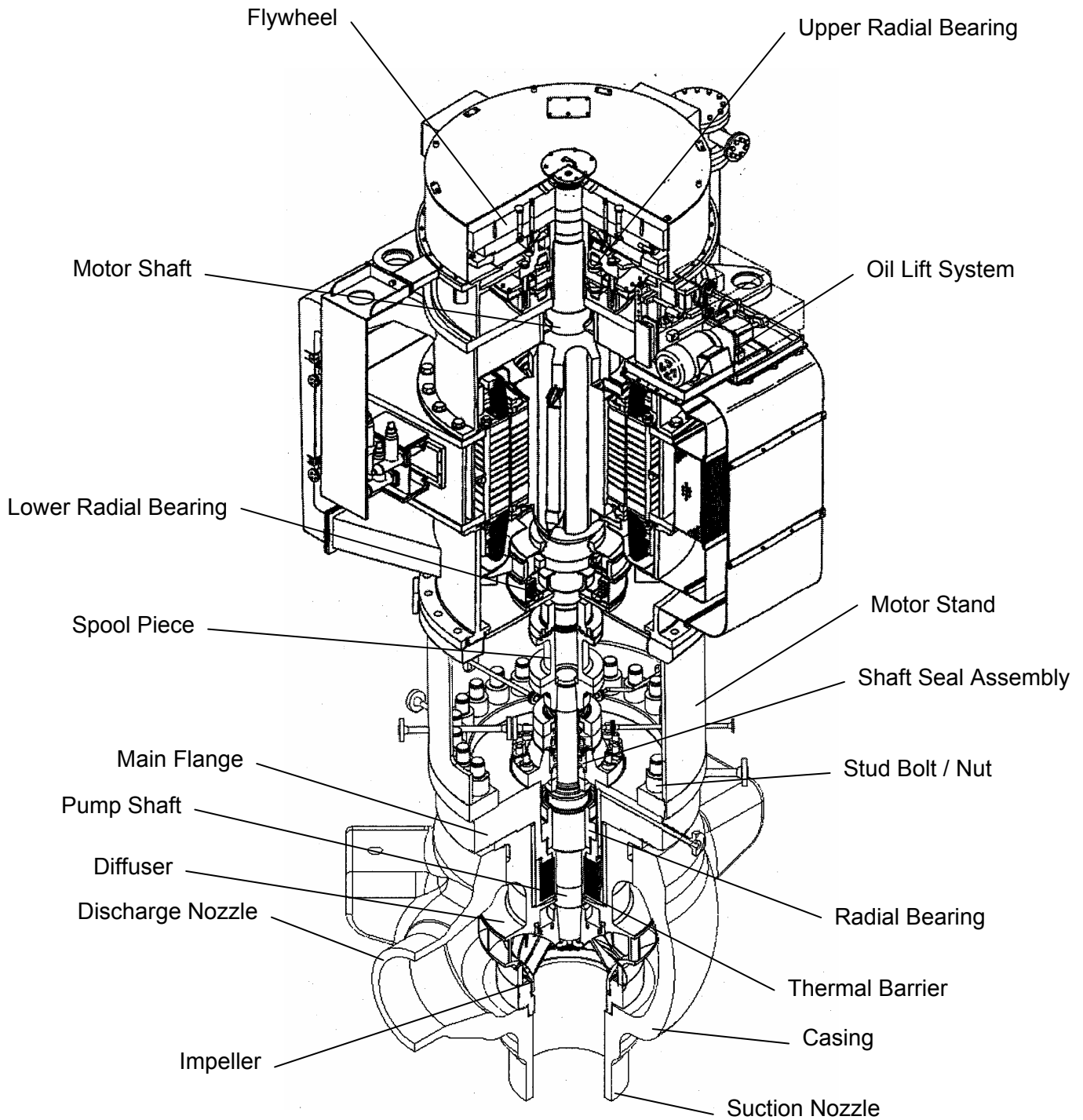
Figure 5.4.1-1 Reactor Coolant Pump
