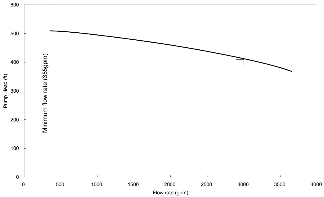
Figure 5.4.7-3 CS/RHR Pump Characteristic Curve
