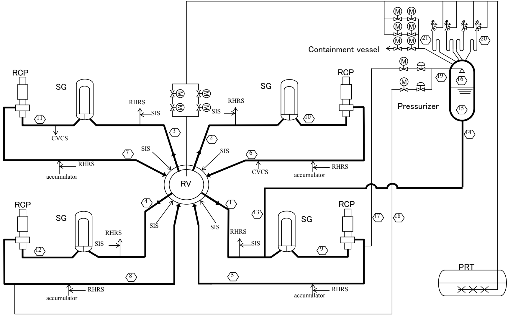
Figure 5.1-1 Reactor Coolant System Schematic Flow diagram
