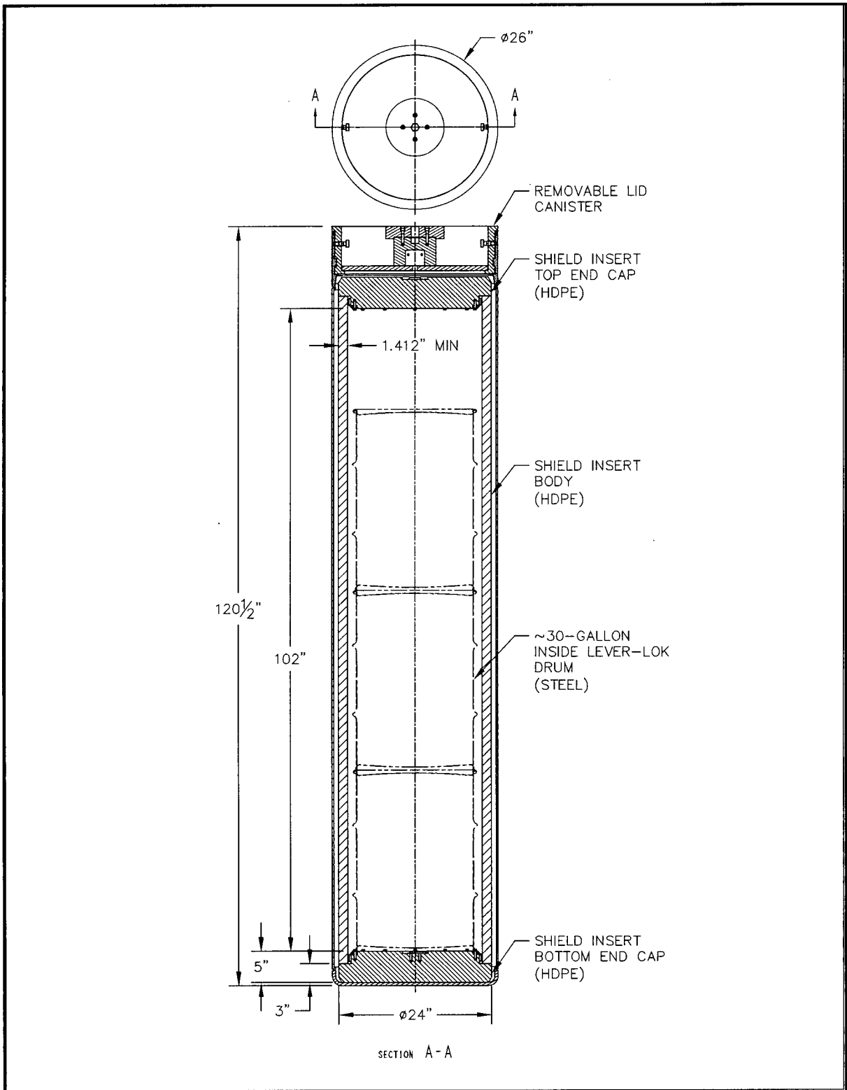
Figure 5.1-1 – Neutron Shielded Canister, NS30
