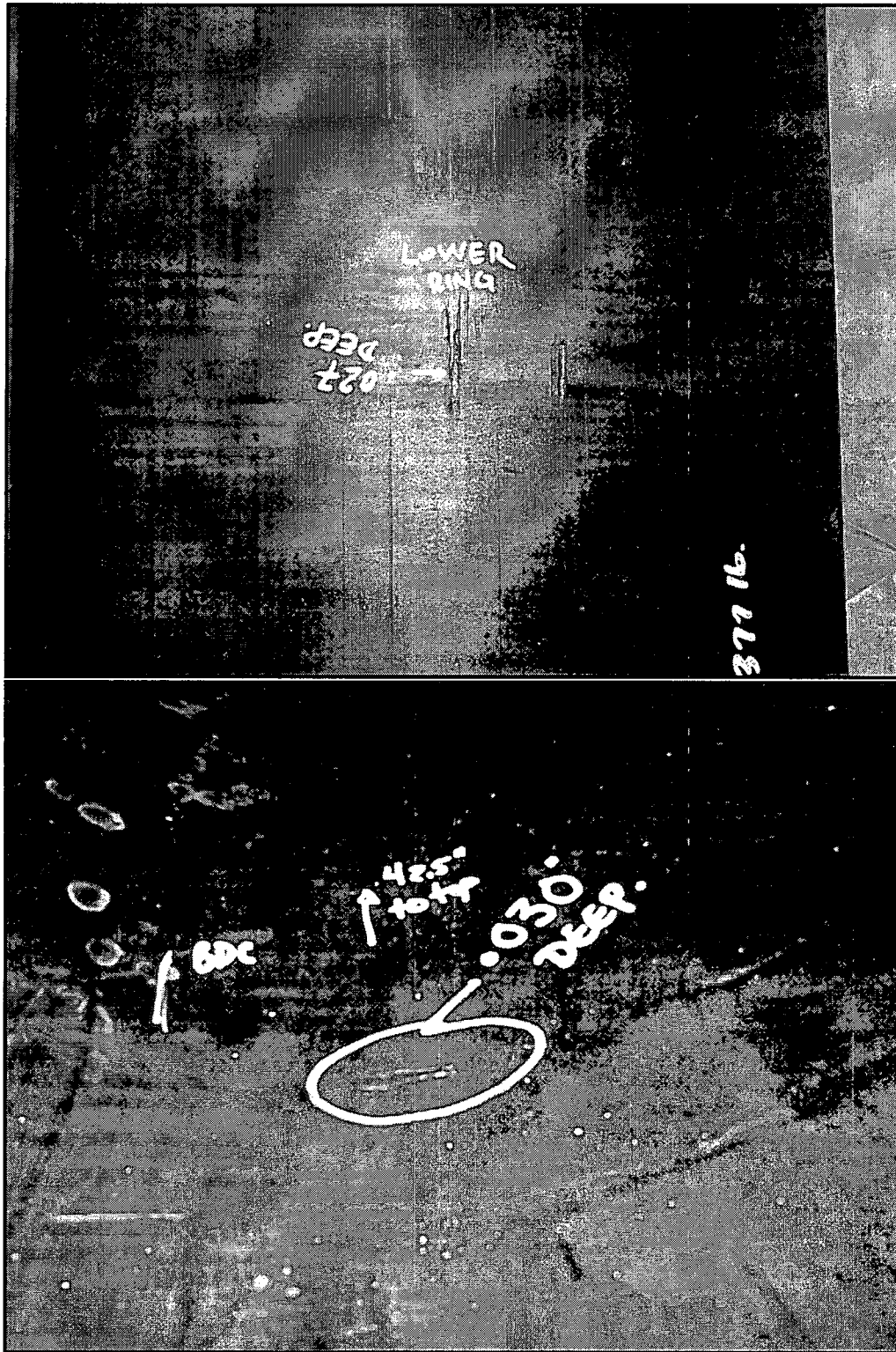
Figure 5.1-11 – Cold Drop Body Pipe Dents and Gouges
