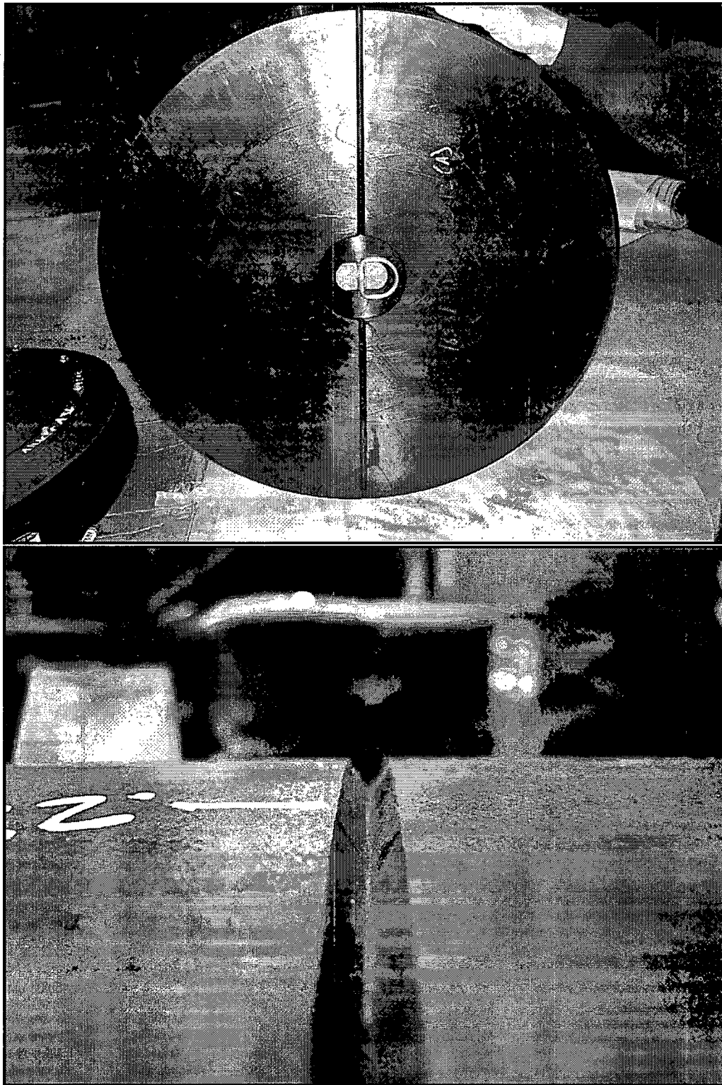
Figure 5.1-9 – Cold Drop End Cap and Body Pipe Groove V-notch Defects
