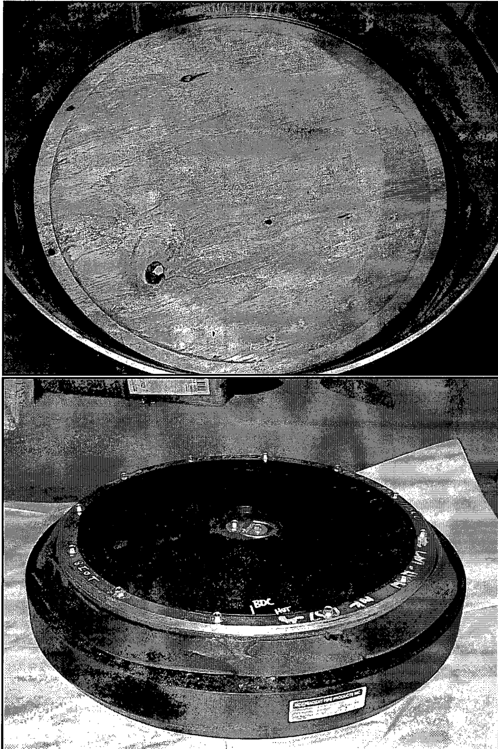
Figure 5.1-14 – Hot Drop Damage to the Spacer and End Cap Gasket
