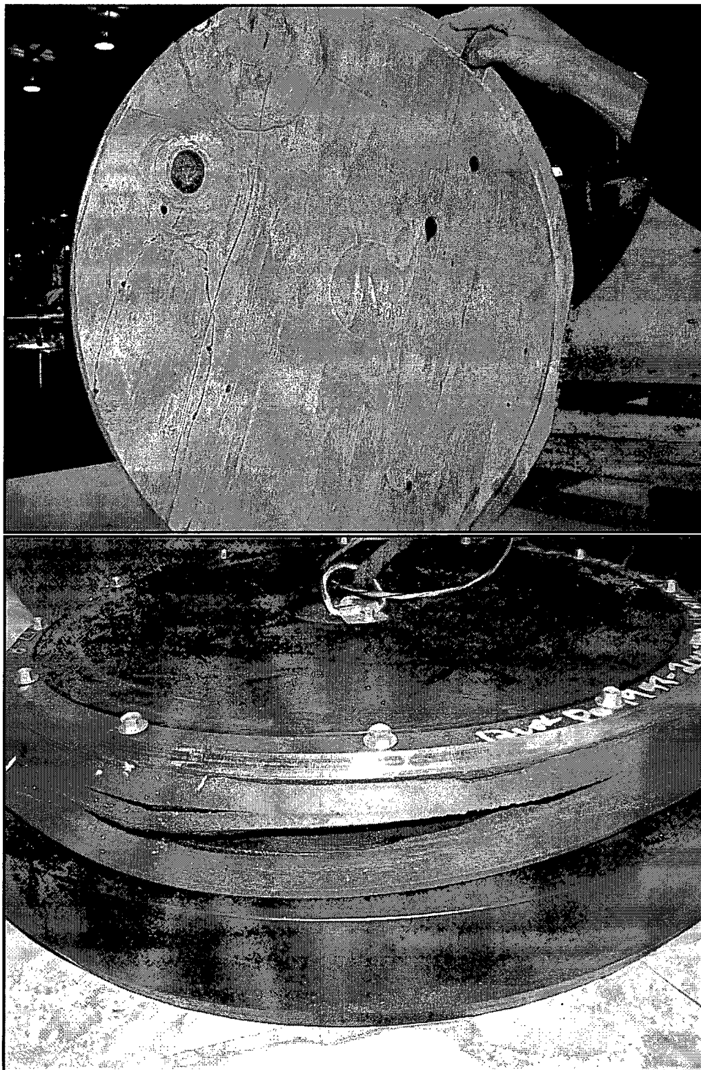
Figure 5.1-8 –Cold Drop Damage to the Spacer and End Cap Gasket
