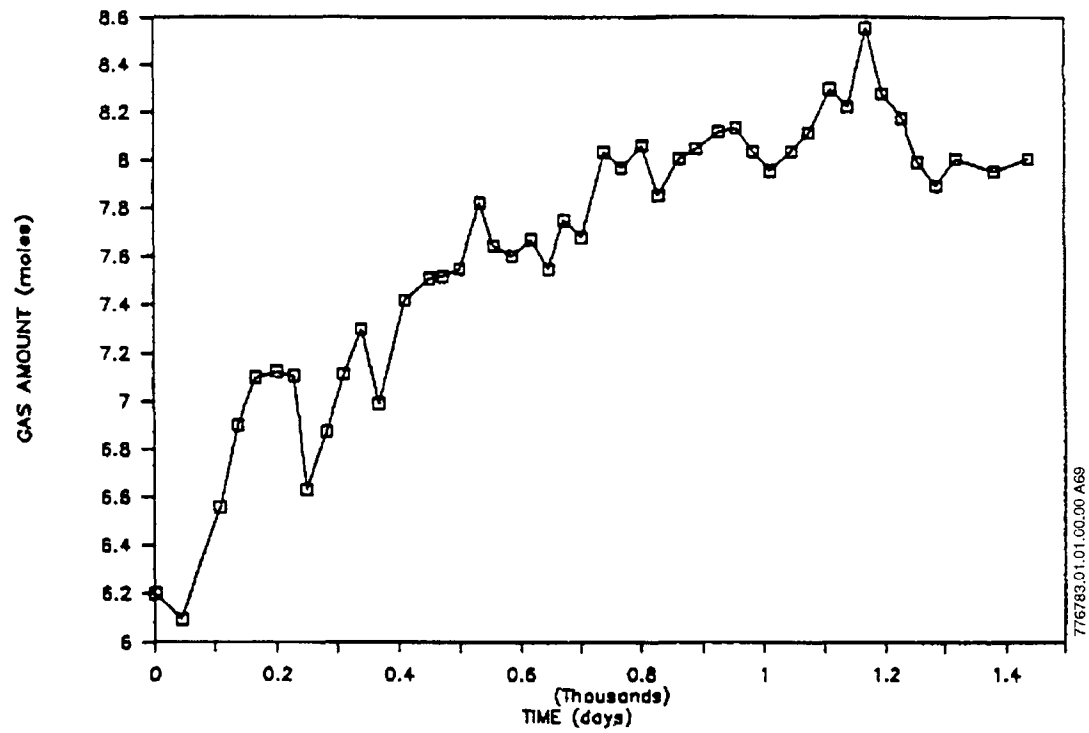
Figure 2.1-4 — Moles of Gas Present in Drum 122 vs. Time
