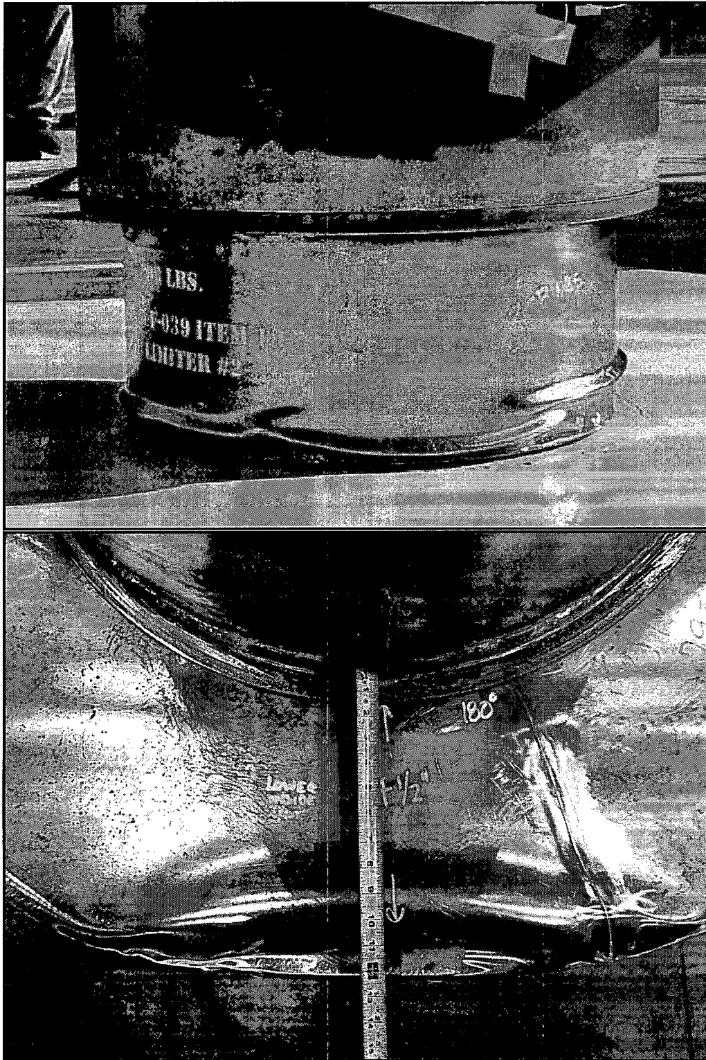
Figure 5.1-13 – Hot End and Side Drop Impact Limiter Deformation
