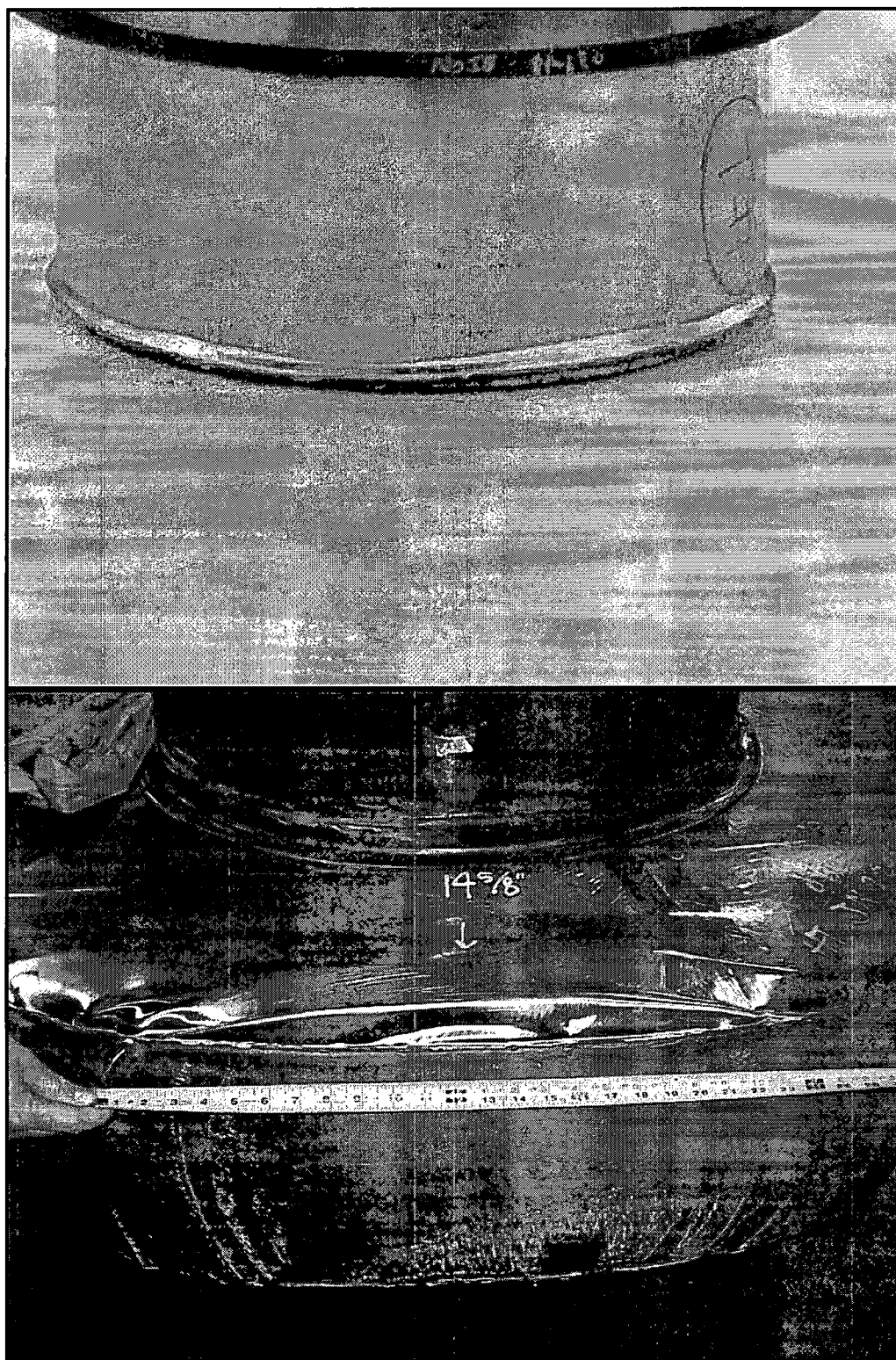
Figure 5.1-7 – Cold End and Side Drop Impact Limiter Deformation
