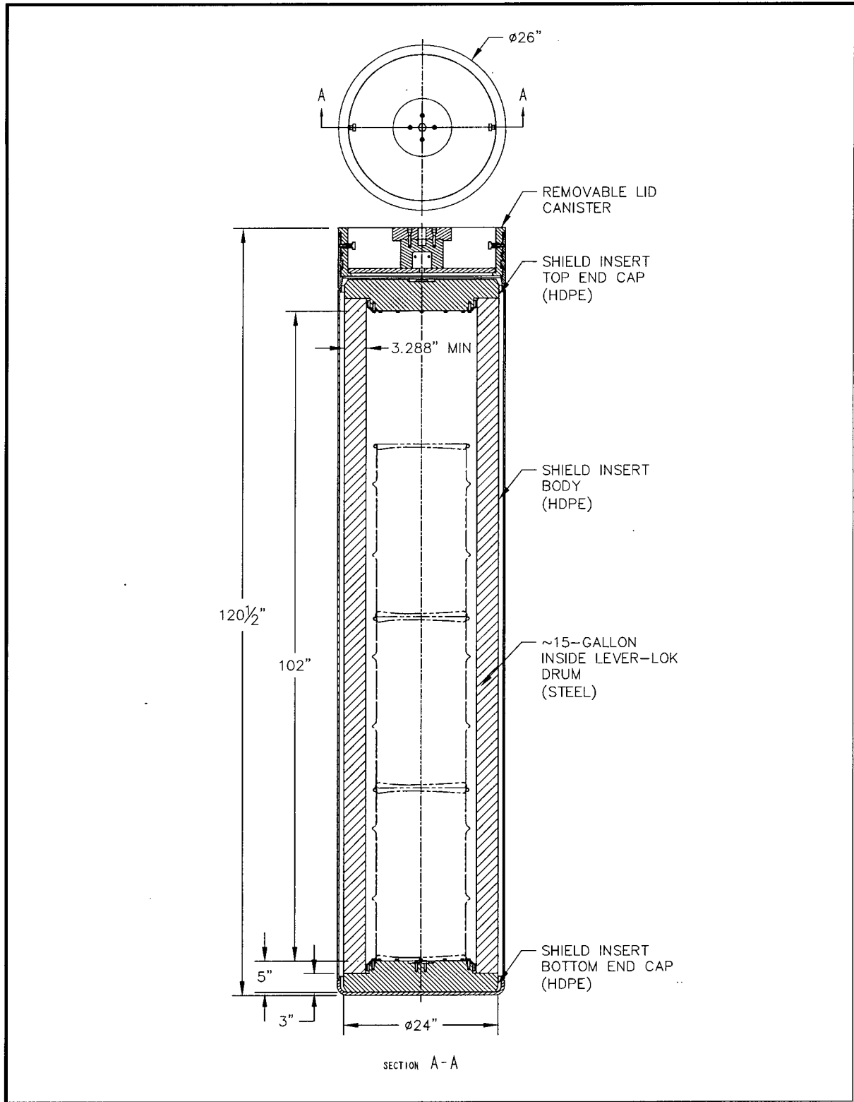
Figure 5.1-2 – Neutron Shielded Canister, NS15
