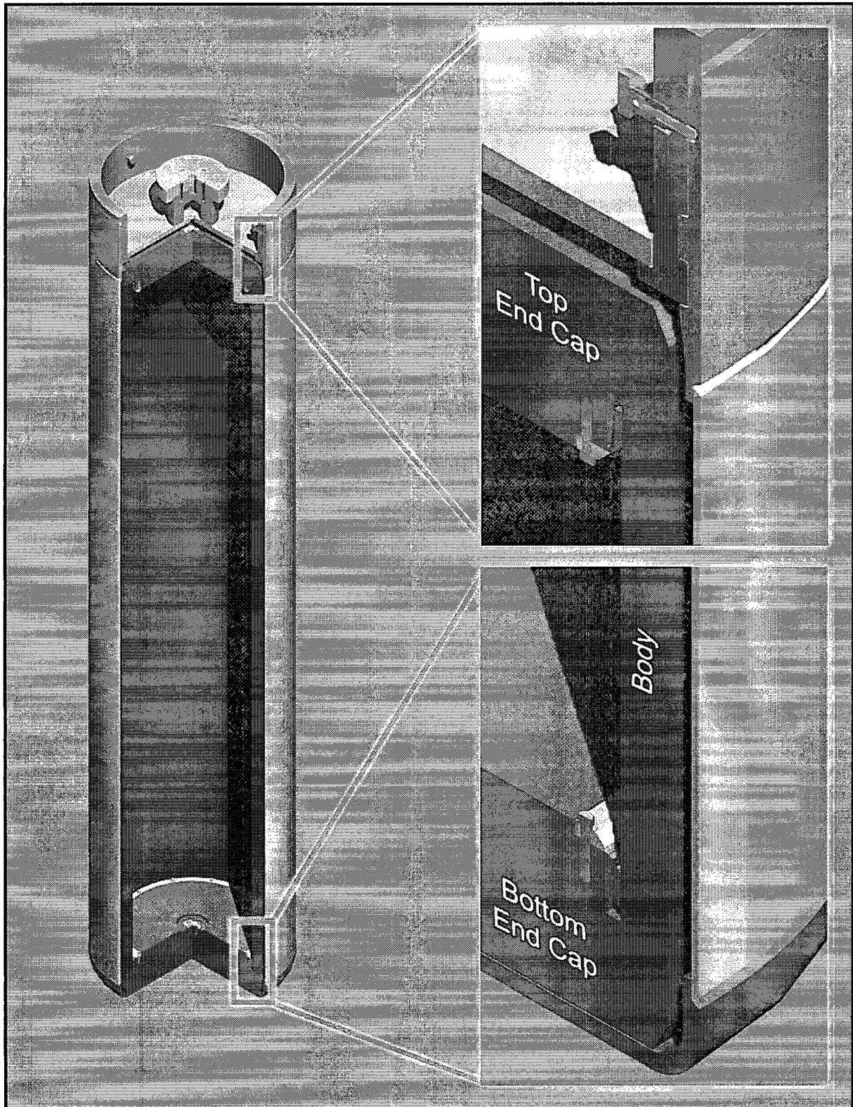
Figure 5.1-3 – NS30 Isometric
