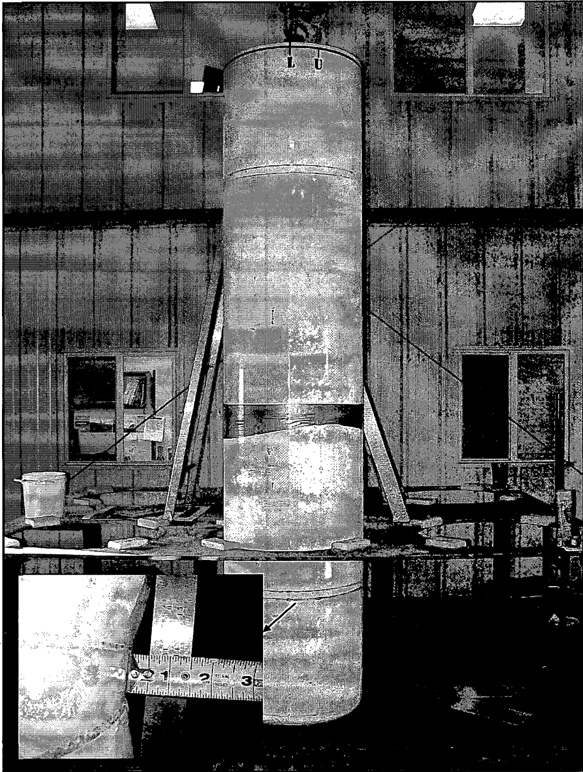
Figure 5.1-12 – Cold Drop Canister Metallic Component Deformations
