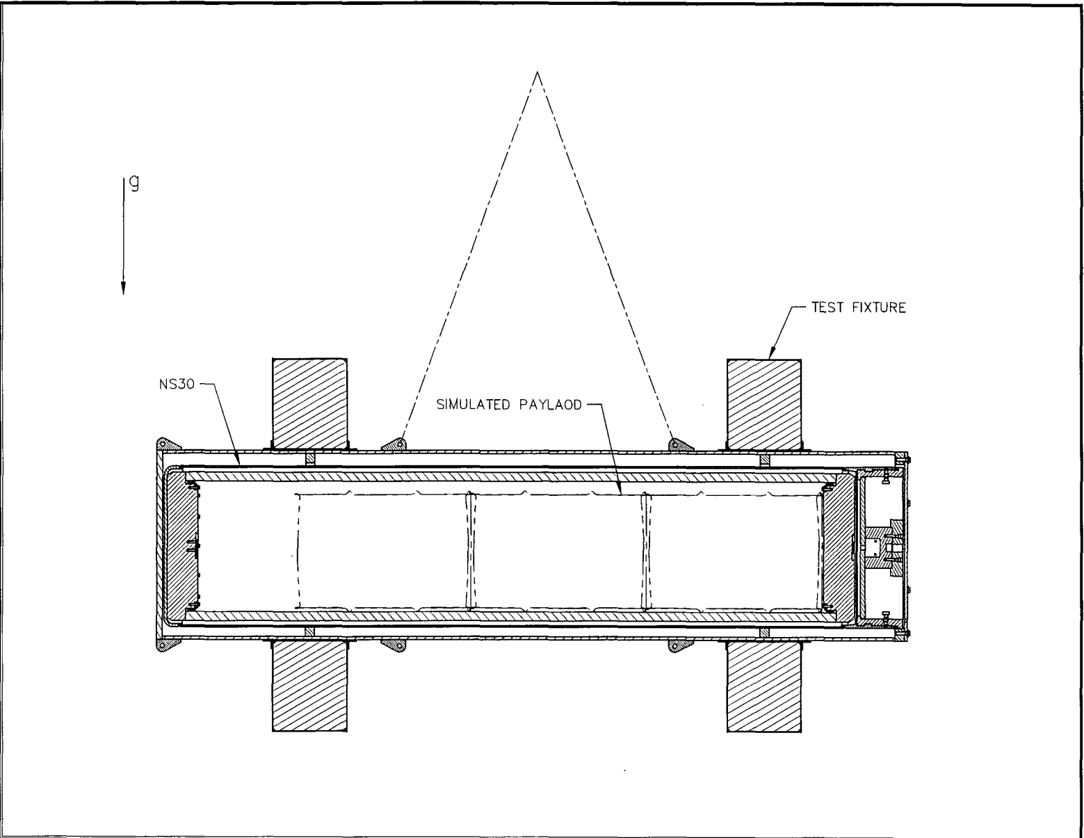
Figure 5.1-6 – Side Drop Test Configuration
