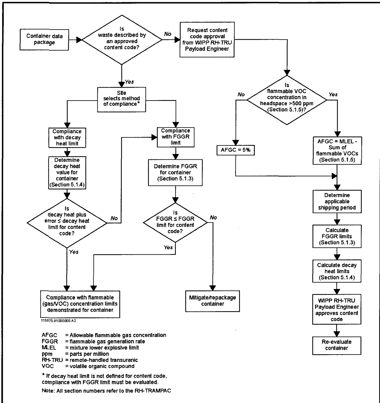
Figure 3.1-1 – Methodology for Compliance with Flammable (Gas/VOC) Concentration Limits
