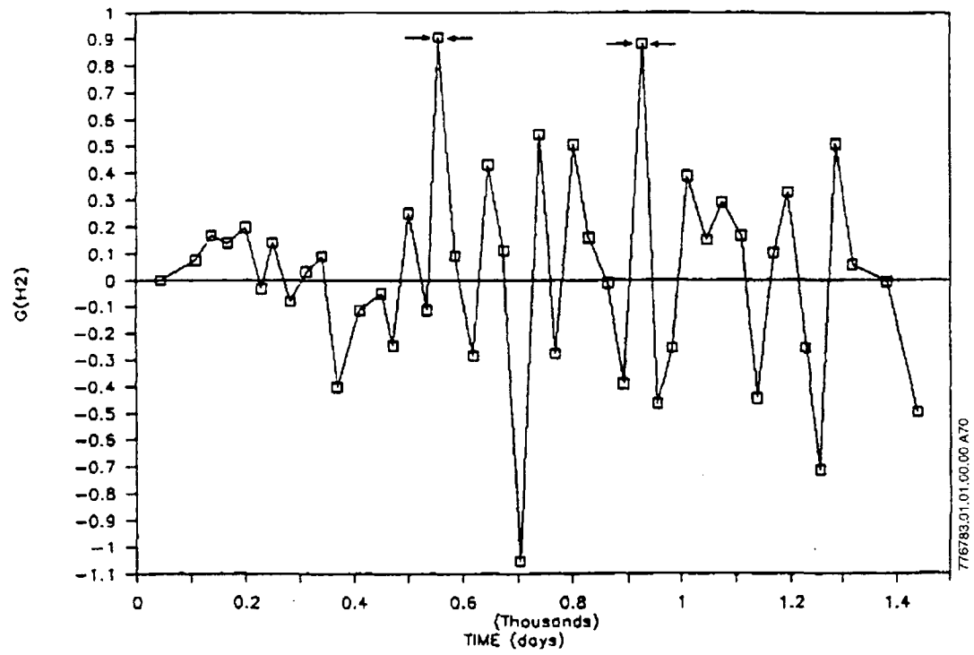
Figure 2.1-5 — G(H_2) vs. Time for Drum 122
