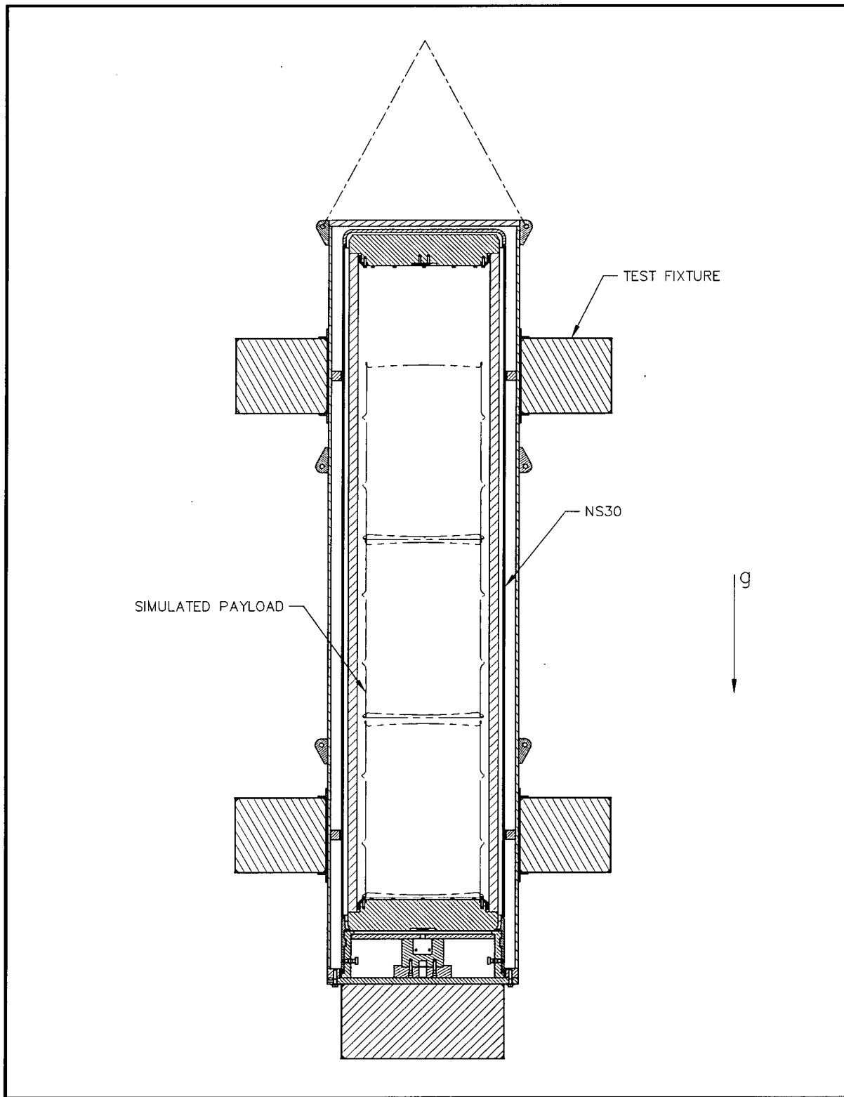
Figure 5.1-5 – End Drop Test Configuration
