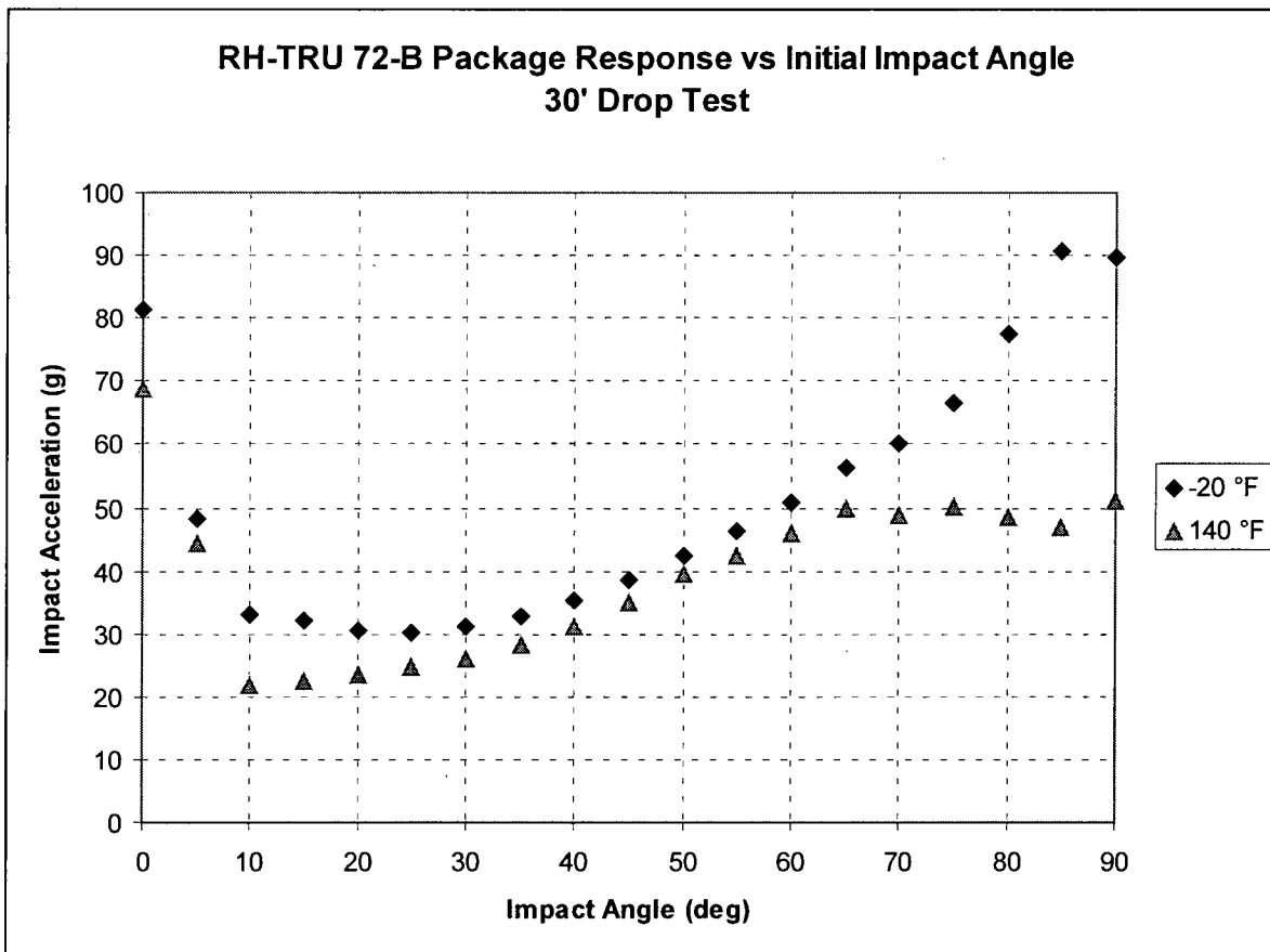
Figure 5.1-4 – RH-TRU 72-B Impact Acceleration Dependency on Impact Angle and Temperature
