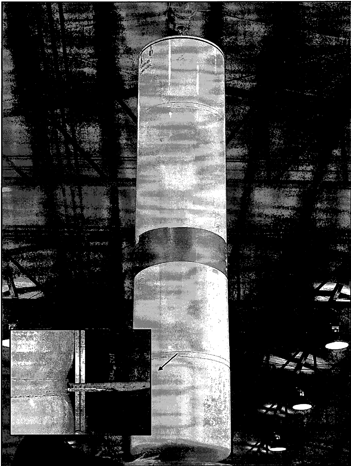
Figure 5.1-18 – Hot Drop Canister Metallic Component Deformations
