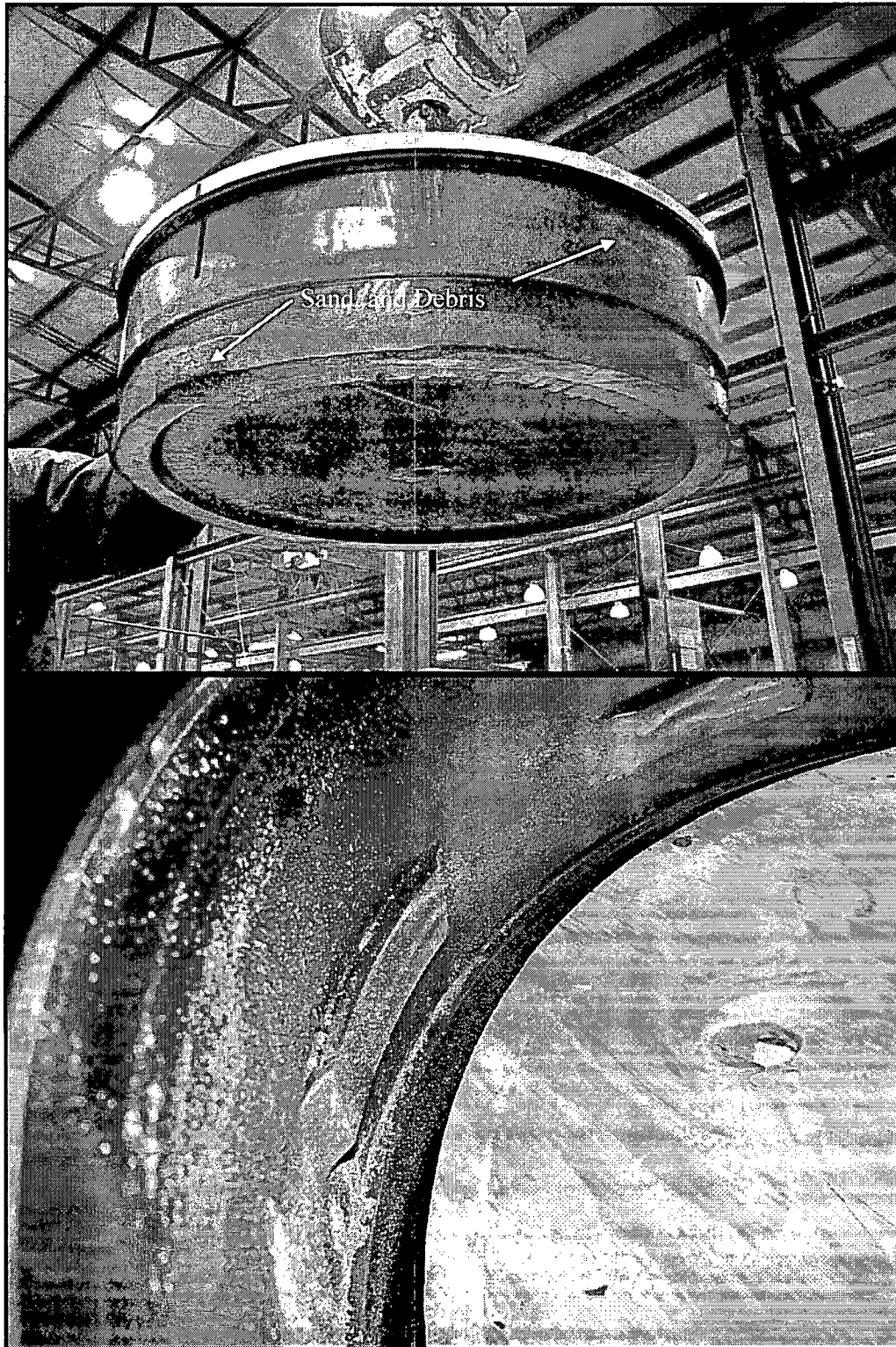
Figure 5.1-15 – Hot Drop Induced Presence of Released Fine Particulate
