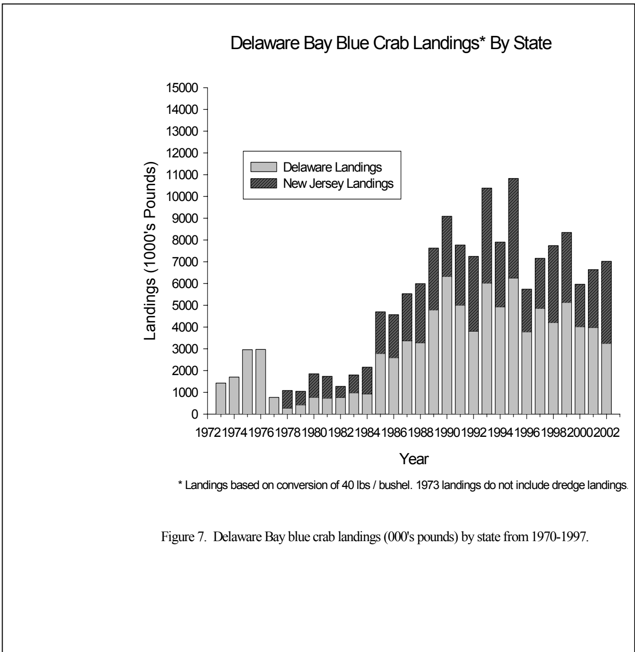
Figure 5.3-1 Delaware Bay Blue Crab Landings (1000s pounds) by State (Source: Helser, and Kahn. 2001)
