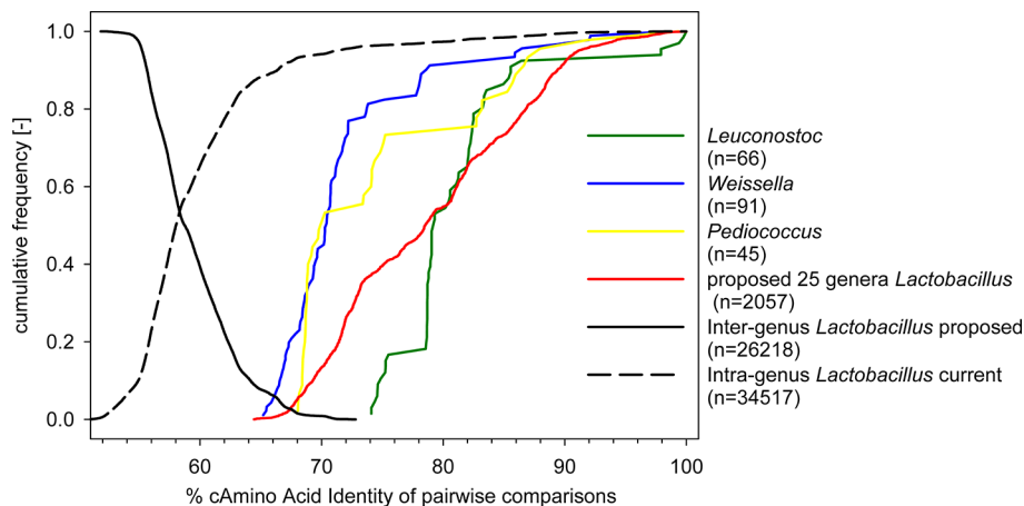
Fig. 4. Frequency distribution of pairwise cAAI in Lactobacillaceae and Leuconostocaceae . Inter-genus cAAI values are shown in descending order; Intra-genus cAAI values are shown in ascending order for the current taxonomy (dotted lines) and for the proposed taxonomy that divides the genus Lactobacillus in 25 genera (solid lines). Genera are colour coded; Lactobacillus ; Pediococcus , Leuconostoc and Weissella . The number of pairwise cAAI values that is represented by the lines is indicated in the figure legend. Owing to the low number of values, intra-genus cAAI values for Fructobacillus , Oenococcus and Convivina are not shown. The data used for the graph is provided in Table S3.
