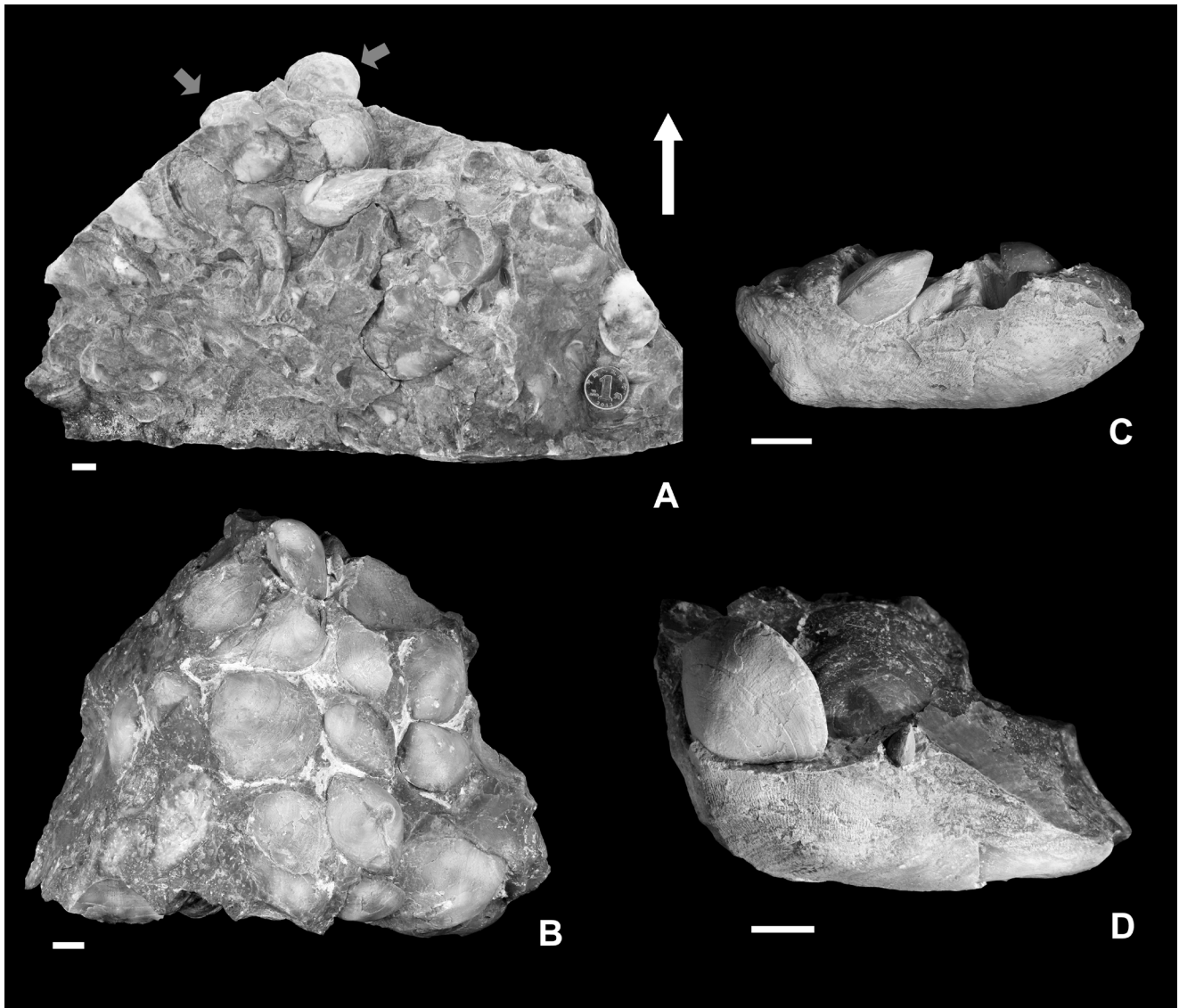
Fig. 5 - Some rock specimens from the shell bed of the Baizuo Formation. A) The lower part of ZDA. Many Striatifera striata are at the bottom and some Weiningia ziyunensis n. sp. are at the top (grey arrows). White arrow indicates vertically upward direction to bedding plane. B) The upper part of ZDA. Note the close preservation of many Weiningia ziyunensis n. sp. and the absence of other species. C, D) Original life position of Weiningia ziyunensis n. sp., showing their attachment to the dorsal valves of Striatifera striata with posterior portion downward. Scale bars represent 10 mm long.
