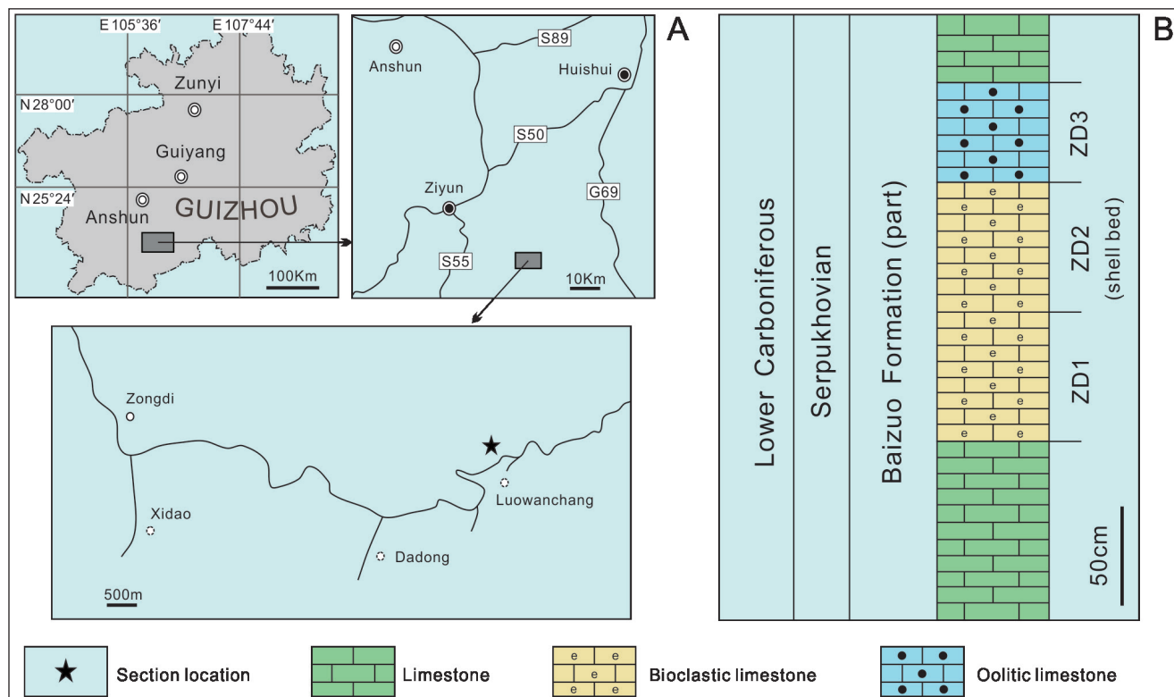
Fig. 1 - Location map (A) and lithological column (B) of the studied section near Luowanchang Village, Zongdi Town, Ziyun County, Guizhou, China.
