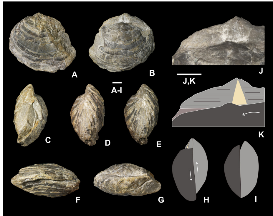
Fig. 9 - The holotype of Weiningia transversa Jin & Liao, 1974, NIGP 22450. A-G) Ventral, dorsal, lateral (C, D), oblique lateral (E), anterior and posterior views. One of the lateral slopes is broken in both valves showing the thickened posterior part of shell (C). The dorsal valve shifts anteriorly relative to the ventral one (E). H) Explanatory drawing of E showing the shifting between both valves. I) Explanatory drawing showing the original lateral view of the specimen. The dorsal and part of the ventral interareas are actually hidden between umbones. J, K) Enlargement of the ventral interarea and its explanatory drawing showing that the dorsal valve also leans to the left side, resulting in well exposure of the ventral interarea. Scale bars represent 10 mm.
