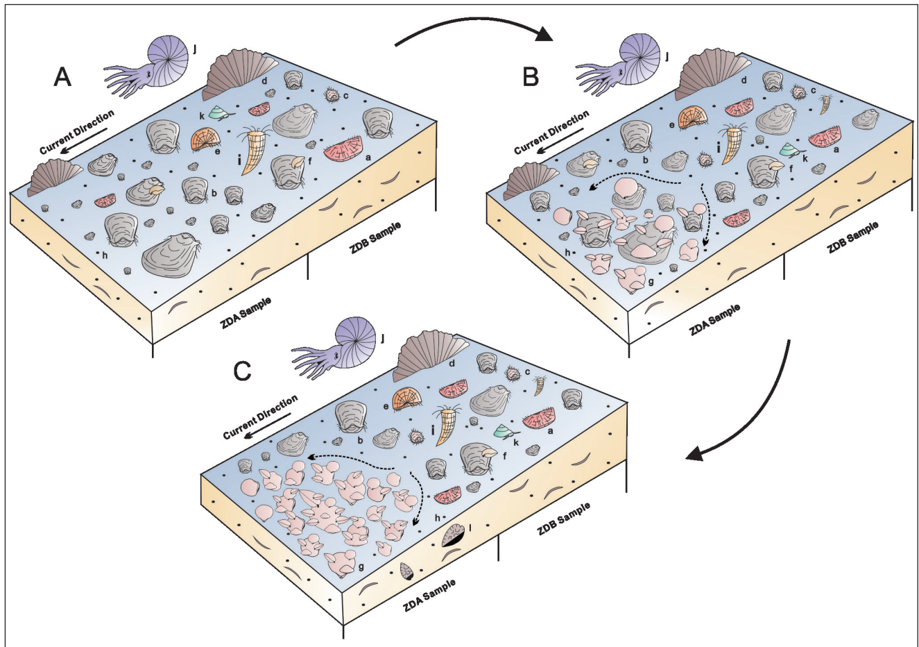
Fig. 7 - Development of the shell bed. A) Before the arrival of Weiningia ziyunensis n. sp. B) Formation of the lower part of cluster. C) Formation of the upper of cluster. Dashed lines in B, C represent spilt currents resulting from blocking by the cluster. Letter a-l represent Megachonetes , Striatifera , Echinoconchella , Gigantoproductus , Fluctuaria , Cleiothyridina , Weiningia , foraminifera, coral, ammonoid, gastropod and geopetal structure.
