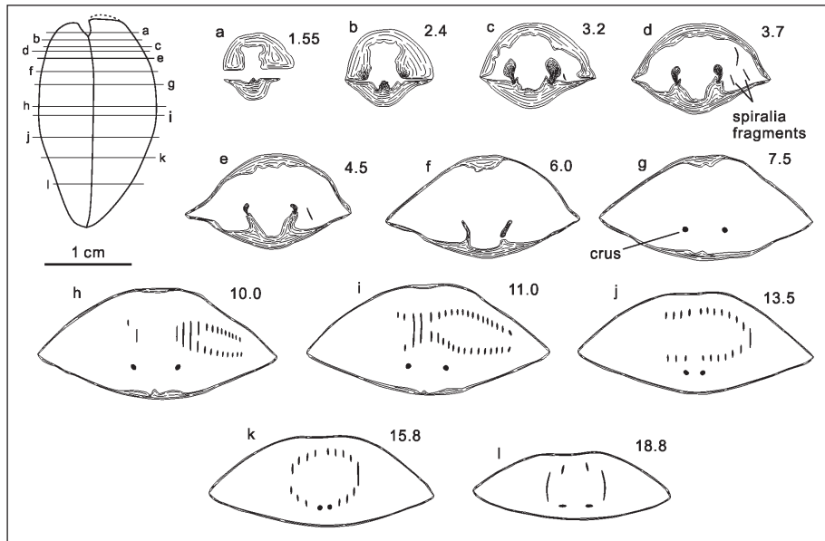
Fig 8 - Transverse serial sections of Weiningia ziyunensis n. sp., PKUM 02-0850. Distances measured in millimeters from the tip of the broken ventral beak.
