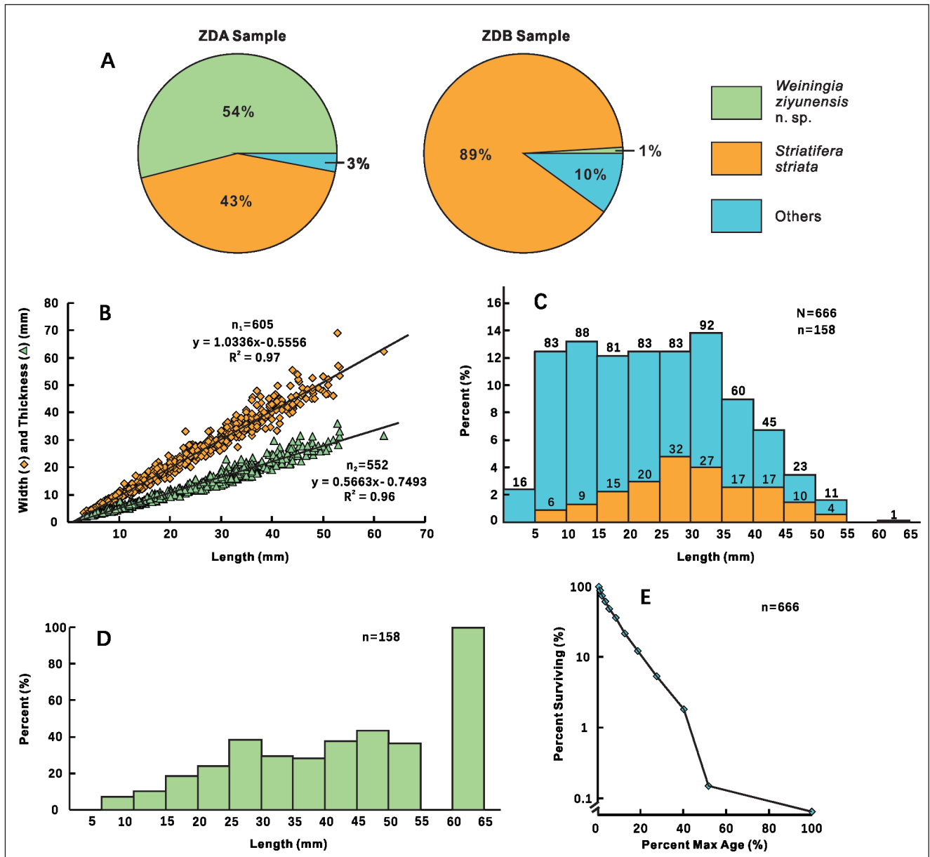
Fig. 6 - Statistical data of the shell bed. A) Composition of Weiningia ziyunensis n. sp., Striatifera striata and others species in ZDA and ZDB. B) Bivariate plots of shell width (diamond) and thickness (triangle) to length of Weiningia ziyunensis n. sp. C) Size-frequency (blue bars) and malformation (yellow bars) distribution of Weiningia ziyunensis n. sp. Numbers above the bars represent the amounts of specimens in each size class of size-frequency and malformation distribution respectively. Note that the only one specimen in the size 60-65 mm is malformed. A total of 158 malformed individuals among 666 specimens was analyzed. D) Percentages of malformed individuals among the total specimens within each size class. Note that 100% in the size 60-65 mm is attributed to the only one malformed specimen. E) Survivorship curve of Weiningia ziyunensis n. sp.
