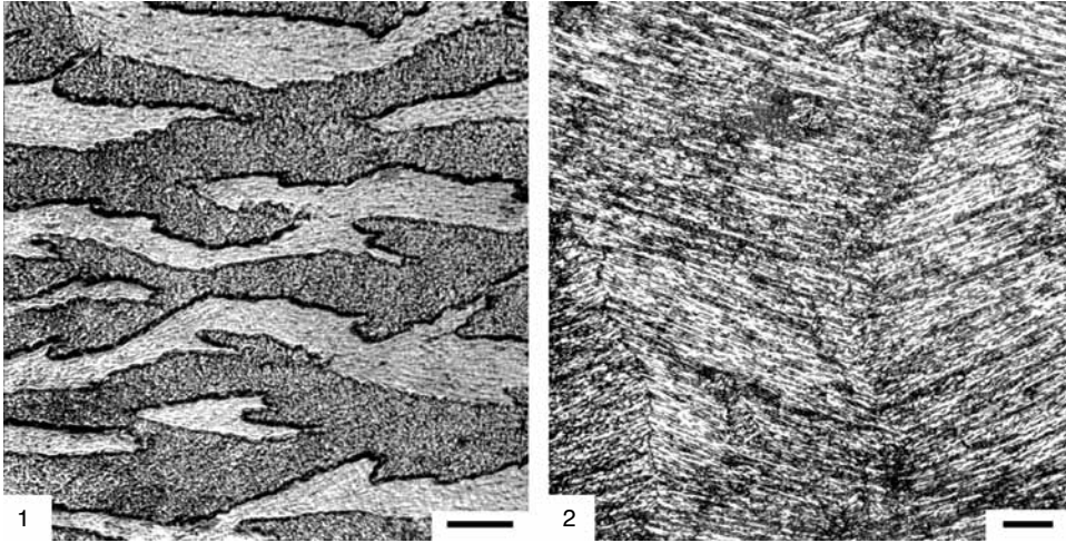
FIG. 78. Crossed foliated microstructure in Oxfordian, Upper Jurassic oxytomid Oxytoma inequivalve (J. SOWERBY, 1819, in SOWERBY & SOWERBY, 1812–1846), Bucks, England (UNC 4527), acetate peels; 1, horizontal section, with shell margin toward top; scale bar = 50 µm; 2, transverse (commarginal) section, with shell interior toward top; scale bar = 50 µm (Carter, new).
