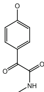
432 2-(4-methoxyphenyl)-N-methyl-2-oxoacetamide
