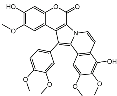
197_Lamallerin \epsilon
