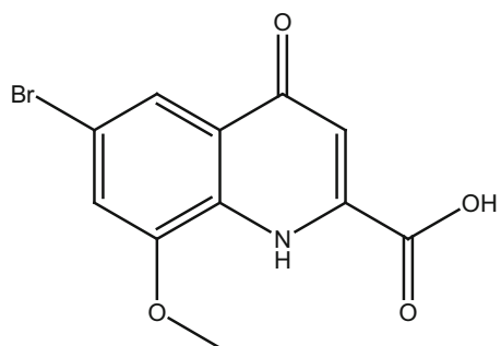
503_Caelestine C
