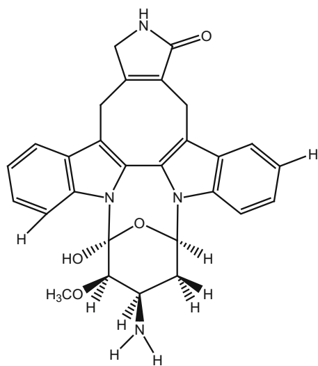
277_3'-demethoxy-3'-hydroxy-4'-N demethylestaurosporine
