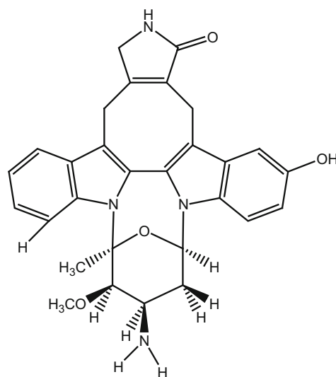
276_3-hydroxy-4'-N-demethylstaurosporine
