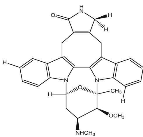
272_11-Hydroxystaurosporine
