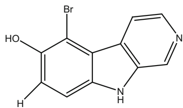
308_eudistomins D
