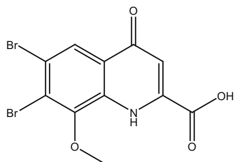
504_Caelestine D
