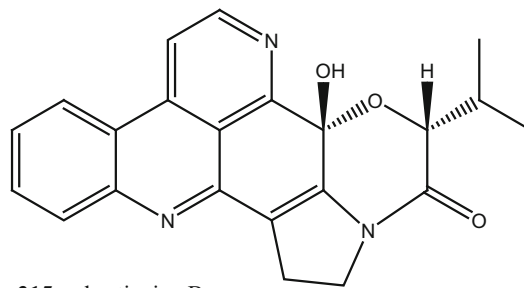
315_sebastianine B
