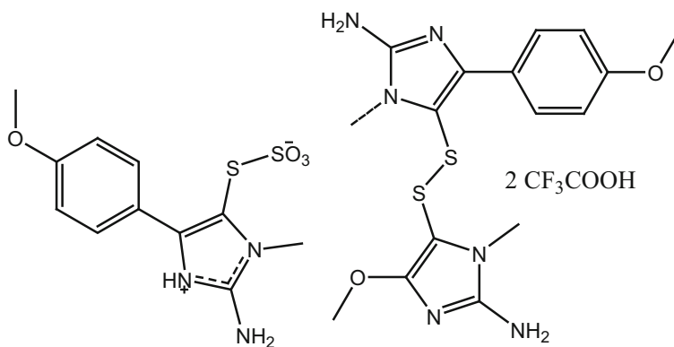
429_polycarpaurines C
