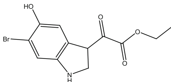
300 _ethyl 6-bromo-5-hydroxyindolyl-3-glyoxylate
