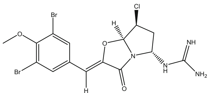
88_Synoxazolidinone C
