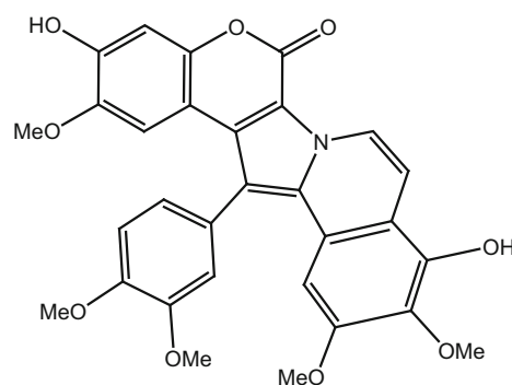
547_Lamallarin X
