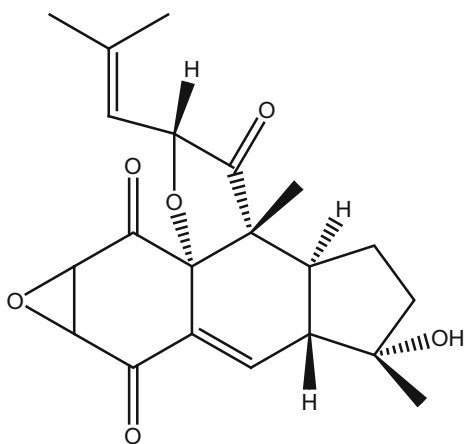
97_2,3-Epoxy-rossinone
