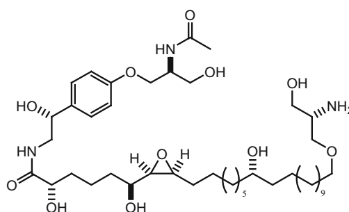
80_Shishididemniol B
