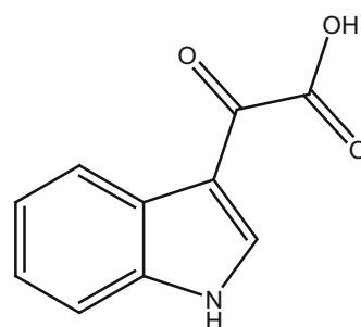
504_Caelestine D
