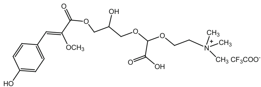
347_durabettaine A
