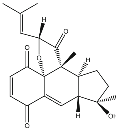
98_3-Epi-rossinone B
