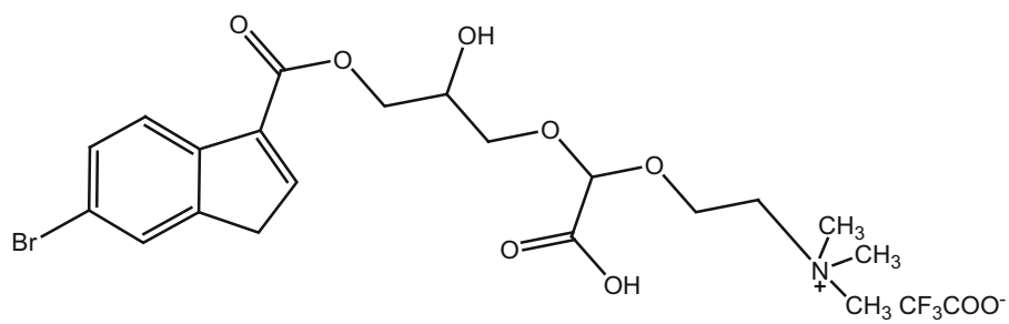
348_durabettaine B
