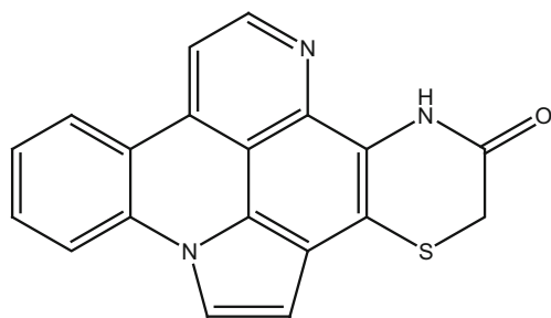
100_13-didemethylaminocycloshermilamine D
