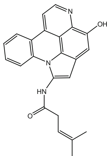
319_arnoamines D
