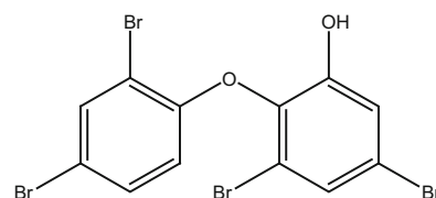
378_2-(2',4'-dibromophenoxy)-3,5-dibromophenol
