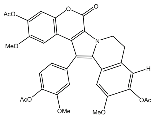
325_lamellarin-χ
