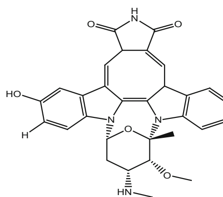
283_3-hydroxy-7-oxostaurosporine
