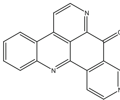
101_demethyldeoxyamphimedine
