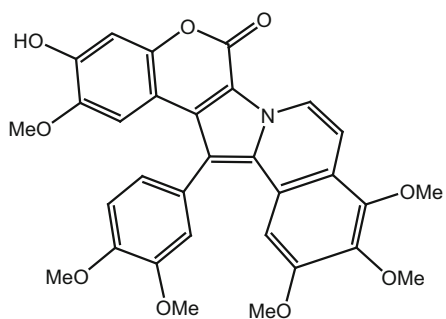
322_lamellarin-ζ
