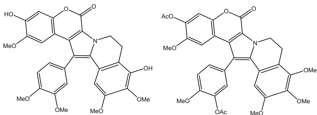
329_lamellarin-T diacetate
