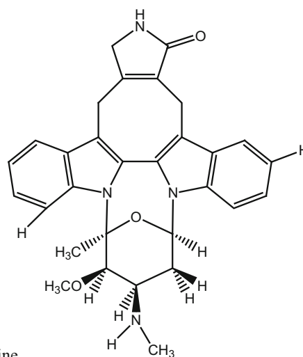
278_staurosporines
