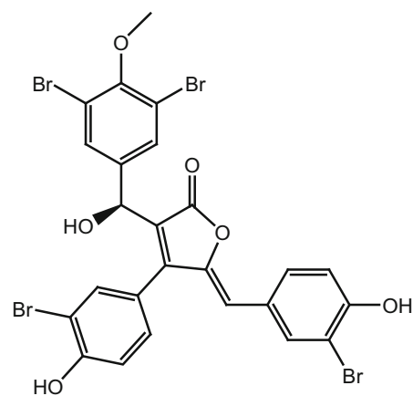
103_cadiolides_F
