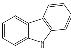
377_beta-Carboline
