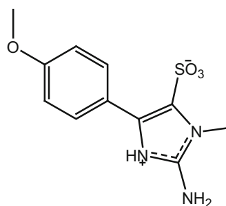
428_polycarpaurines B
