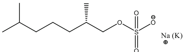
405_2,6-Dimethylheptyl sulphate
