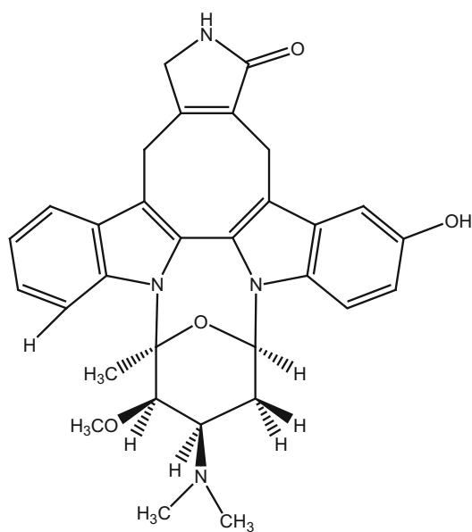
275_3-hydroxy-4'-N-methylstaurosporine
