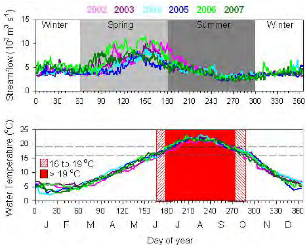
Figure 11. Seasonal and interannual variation in river flow (upper panel) and temperature (lower panel) by day of year at Bonneville Dam 2002-2007. Seasonal divisions are indicated in the upper panel, and temperature regimes in the lower panel. Data courtesy of Columbia River Data Access in Real Time (CRDART 1995).
