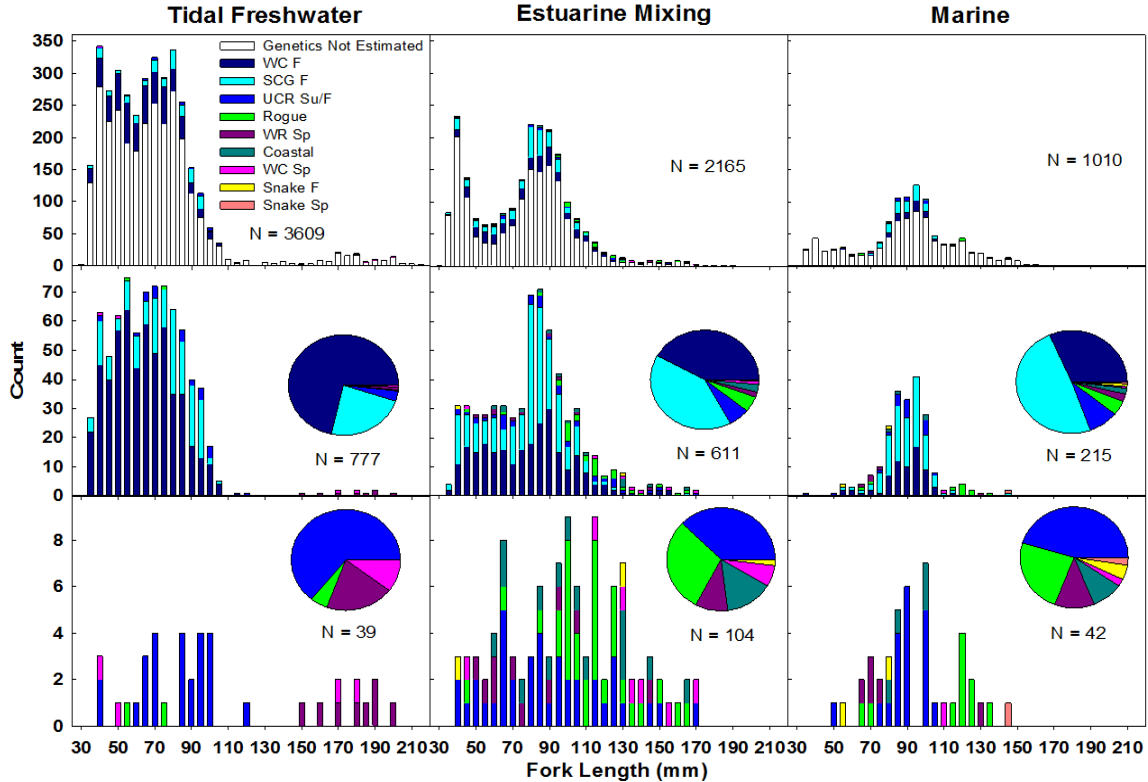
Figure 46. Genetic stock-of-origin of Chinook salmon sampled from beach seine sites at tidal freshwater, estuarine mixing and marine zones during 2002-2006. Bar graphs show length-frequency distribution; pie graphs show proportional distribution. Upper panel shows all fish sampled, including those for which no stock origin was estimated. Middle panel shows major contributors and lower panel minor contributors. Stock codes listed in Table 16.
