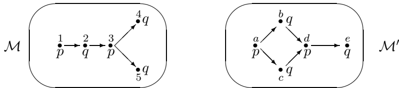
Figure 1: Bisimilar models.
