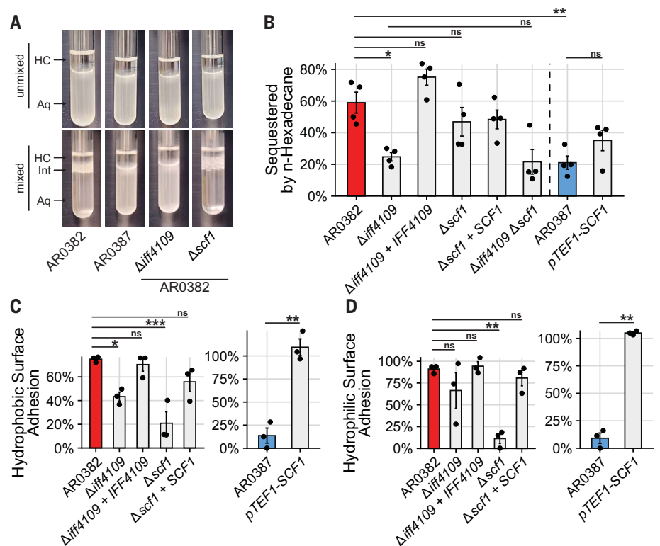
Fig. 3. Iff4109 , but not Scf1 , mediates adhesion through cell surface hydrophobicity. (A) Representative images from the microbial attachment to hydrocarbons (MATH) assay. Hydrophobic cells are sequestered from the aqueous phase (Aq) to the aqueous-hydrocarbon interface (Int) after mixing with the hydrocarbon phase (HC). (B) Proportion of cells sequestered out of the aqueous phase during the MATH assay. (C and D) Cells were allowed to attach to a hydrophobic, untreated polystyrene surface (C) or a hydrophilic, vacuum plasma-treated polystyrene surface (D) for 1 hour. The surface was then washed and the proportion of cells that remained attached after washing was measured. Statistical differences were assessed using one-way ANOVA with Tukey's post hoc test [(B), (C), and (D)] or Student's t test [(C) and (D)]; * P \leq 0.05 ; ** P \leq 0.01 ; *** P \leq 0.001 ; ns: P > 0.05 .
