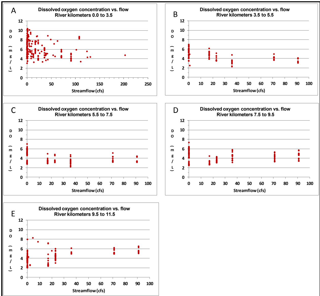
Figure 2-17. Relationship between dissolved oxygen (DO) concentrations in five zones in the Pithlachascotee River and flow measured at the Pithlachascotee River near New Port Richey gage.
