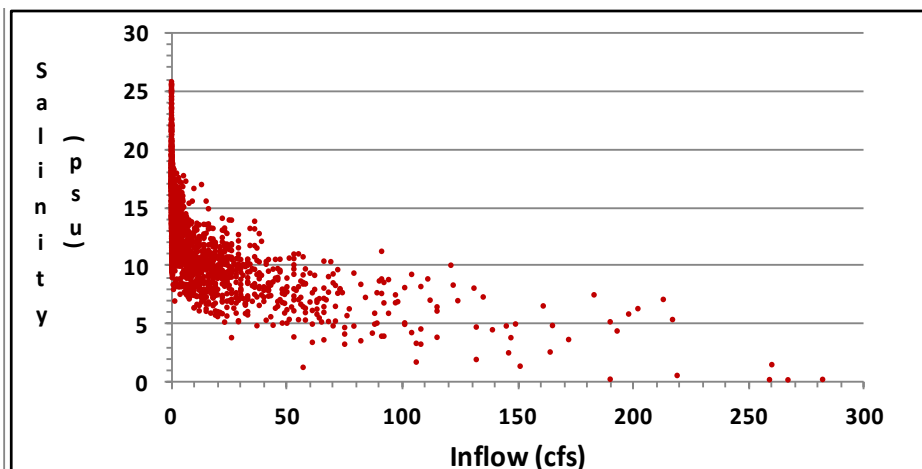
Figure 3-11. Average daily salinity at the Pithlachascotee River at Main Street gage vs. same-day flow at the Pithlachascotee River near New Port Richey gage.
