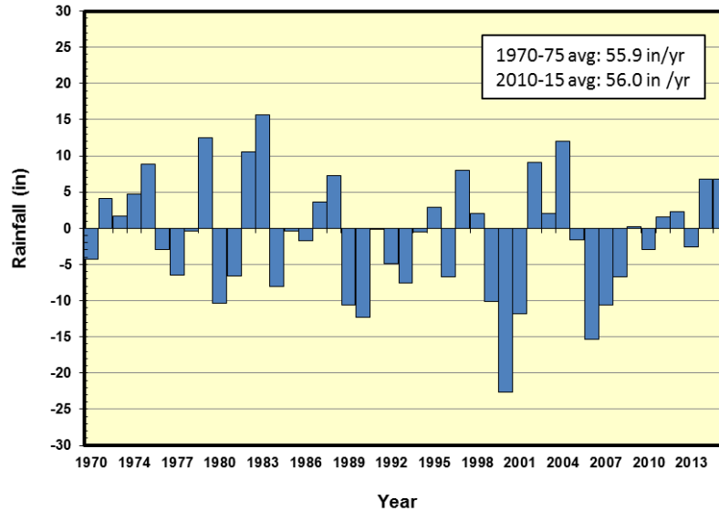
Figure 6-15. Annual rainfall departure from the long-term mean for Pasco County, Florida from 1970 through 2015. Data source: http://www.swfwmd.state.fl.us/data/wmdbweb/rainfall_data_summaries .
