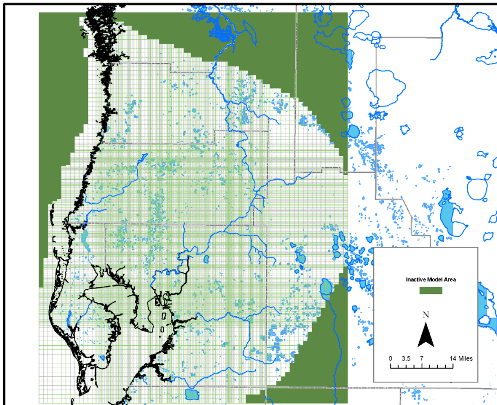
Figure 2-12. Groundwater grid used in the INTB model.
