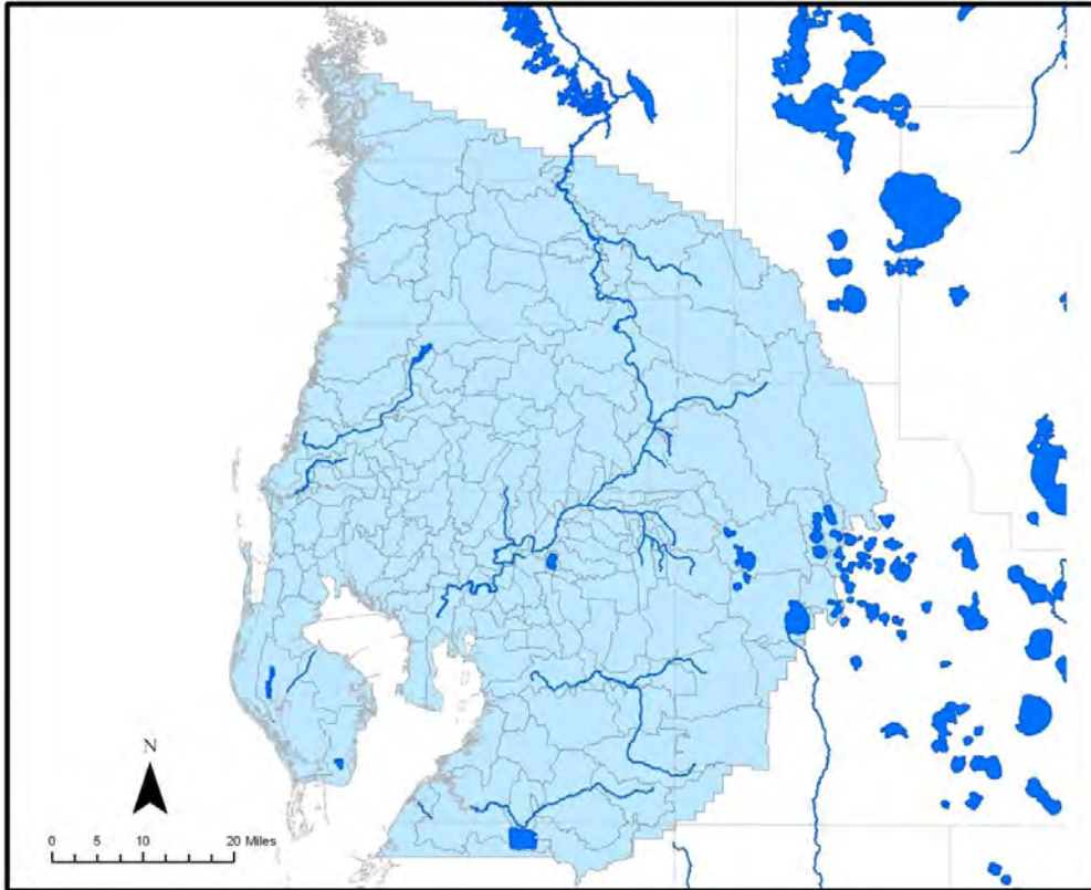
Figure 2-13. HSPF sub-basins in the INTB model.
