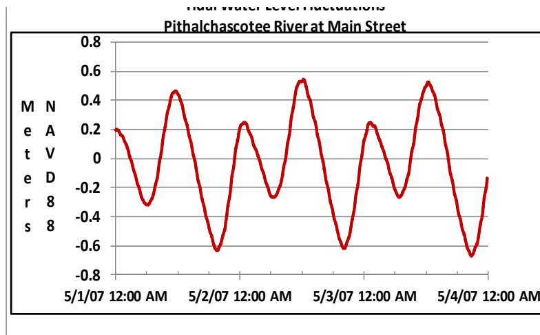
Figure 3-2. Mixed semi-diurnal tidal water level fluctuations at the Pithlachascotee River at Main Street at New Port Richey gage from May 1 through May 3, 2007.
