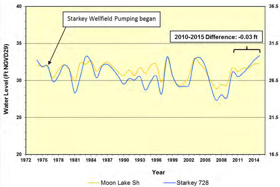
Figure 6-8. Comparison of water levels at Starkey Wellfield 728 monitor well with the Moon Lake Sh background monitor well using the hydrograph separation technique.
