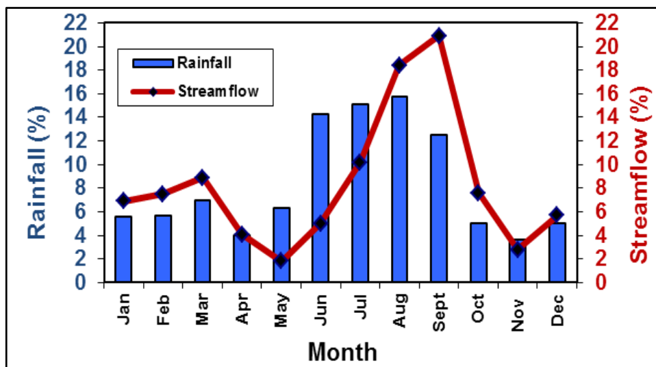
Figure 2-9. Monthly rainfall and streamflow for the Pithlachascotee River watershed. Data taken from Pasco County rainfall estimates and flows at the Pithlachascotee River near New Port Richey gage for water years 1964 through 2013.
