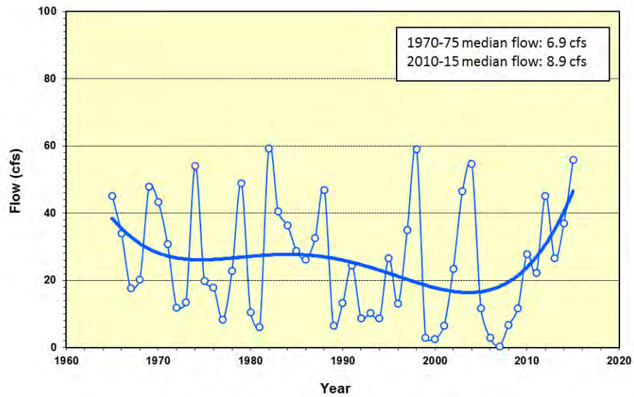
Figure 6-14. Mean annual flow of the Pithlachascotee River at the New Port Richey gage from 1964 through 2015 with a 4 th -order polynomial fit to the data.
