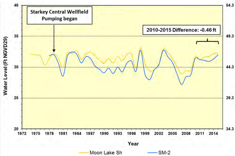
Figure 6-10. Comparison of water levels at Starkey wellfield SM-2 monitor well with the Moon Lake Sh background monitor well using the hydrograph separation technique.
