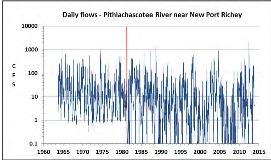
Figure 2-10. Daily streamflow at the Pithlachascotee River near New Port Richey gage for April 1, 1963 through September 30, 2013. Values less than 0.1 cfs converted to 0.1 cfs for plotting purposes. Red vertical line identifies date when the gage was moved 1.1 miles upstream.
