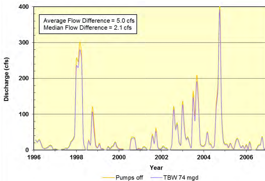
Figure 6-3. Predicted monthly streamflow impact at the Pithlachascotee River near New Port Richey gage due to Central System Facility groundwater withdrawals of 74.3 mgd and all other user’s actual withdrawals from 1996 through 2006.
