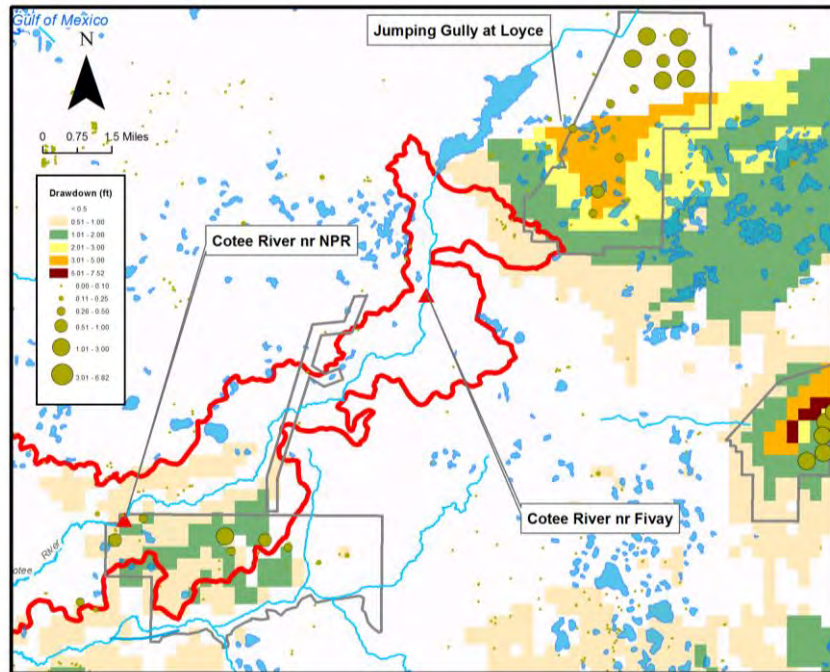
Figure 6-12. Predicted mean surficial aquifer drawdown from the INTB model based on 2014 groundwater withdrawals from the Central System Facility wellfields (74.3 mgd) and all other users pumping at their 1996-2006 quantities. Superimposed is the average magnitude of estimated and metered groundwater use from 2008-2012.
