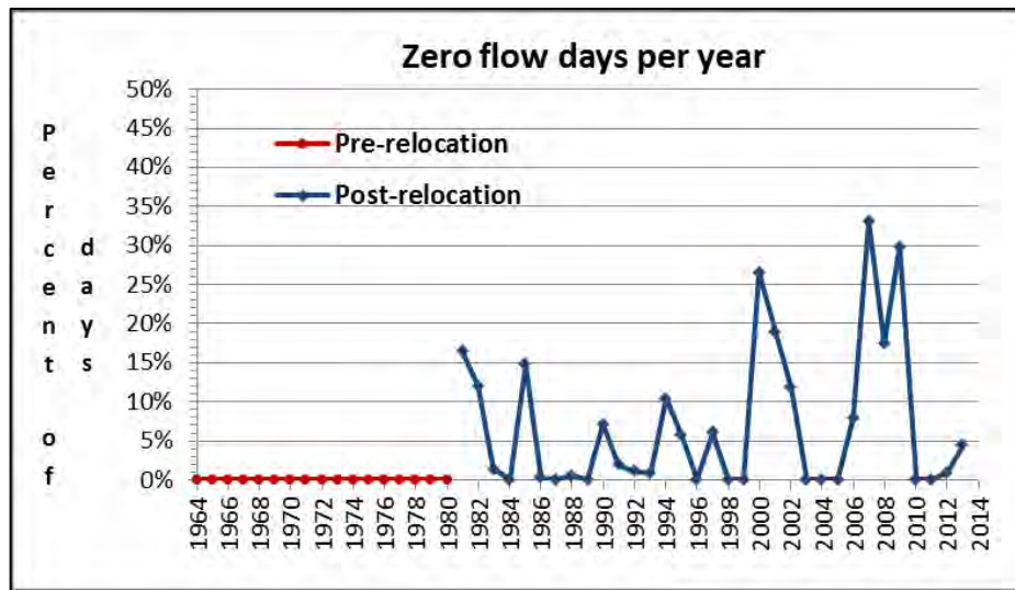
Figure 2-11. Percentage of zero flow days per year for the Pithlachascotee River near New Port Richey gage for water years 1964 through 2013. Pre-location versus post-relocation refers to periods before and after the gage was moved 1.1 miles upstream. Water year 1981 is assigned to the post-relocation period.
