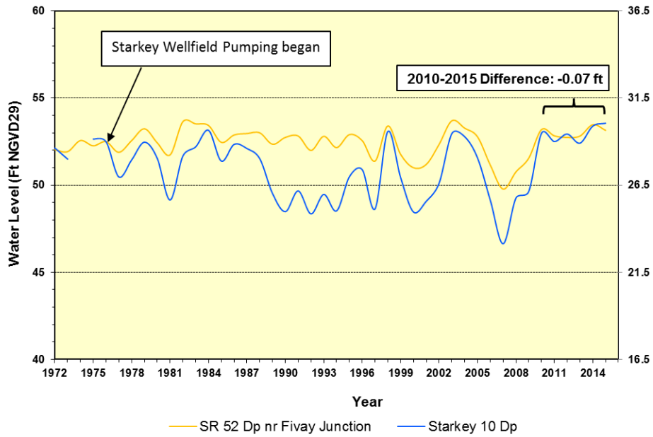
Figure 6-7. Comparison of water levels at Starkey Wellfield 10-Dp monitor well with the SR 52 Dp near Fivay Junction background monitor well using the hydrograph separation technique.
