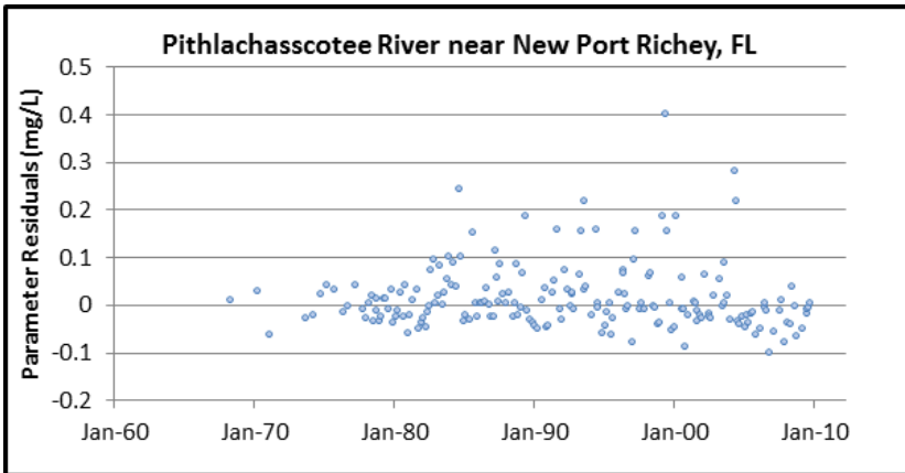
Figure 2-15. Phosphorus concentrations over time (top), phosphorus concentration vs. flow (middle), and trends in phosphorus concentration residuals over time (bottom) at the Pithlachascotee River near New Port Richey gage.
