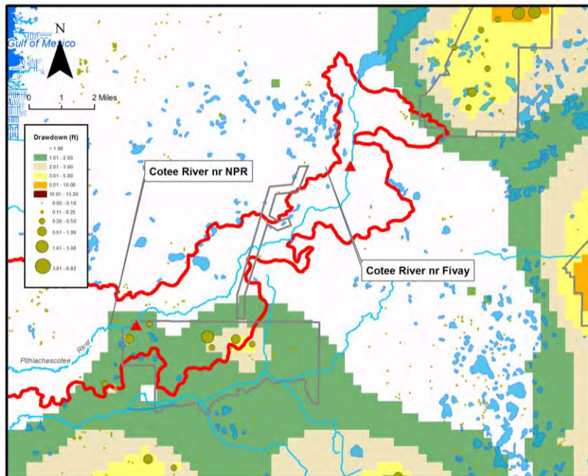
Figure 6-13. Predicted mean Upper Floridan aquifer drawdown from the INTB model based on 2014 TBW groundwater withdrawals (74 mgd) and all other users pumping at their 1996-2006 quantities. Mean estimated and metered groundwater pumping from 2008 through 2012 is also shown.
