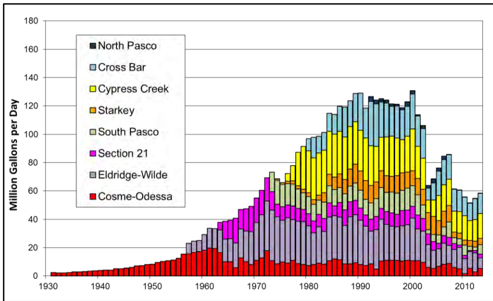
Figure 2-7. Average yearly withdrawal rates for the eight wellfields shown in Figure 2-6 for the years 1931 through 2013.
