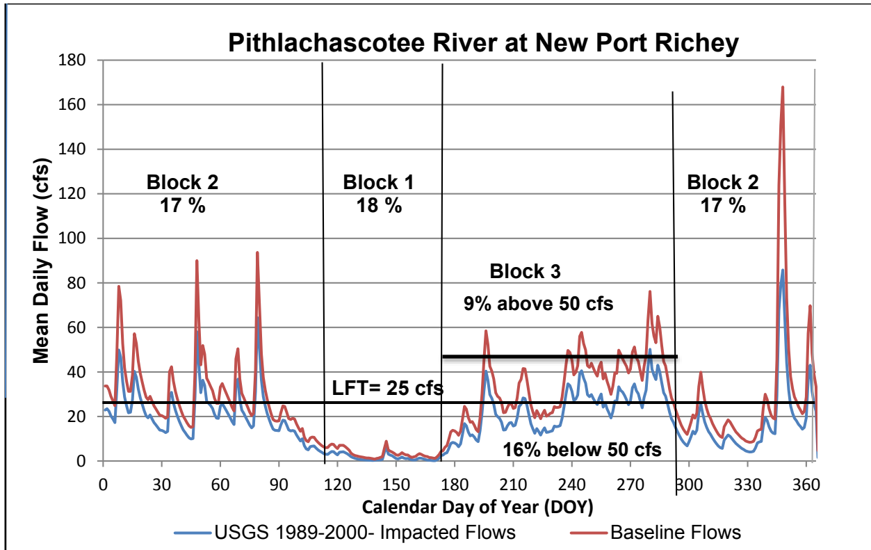
Figure 5-11. Mean annual flow prescription (USGS –impacted flows) and historical flows (baseline flows) for Pithlachascotee River near New Port Richey gage. LFT = Low Flow Threshold.
