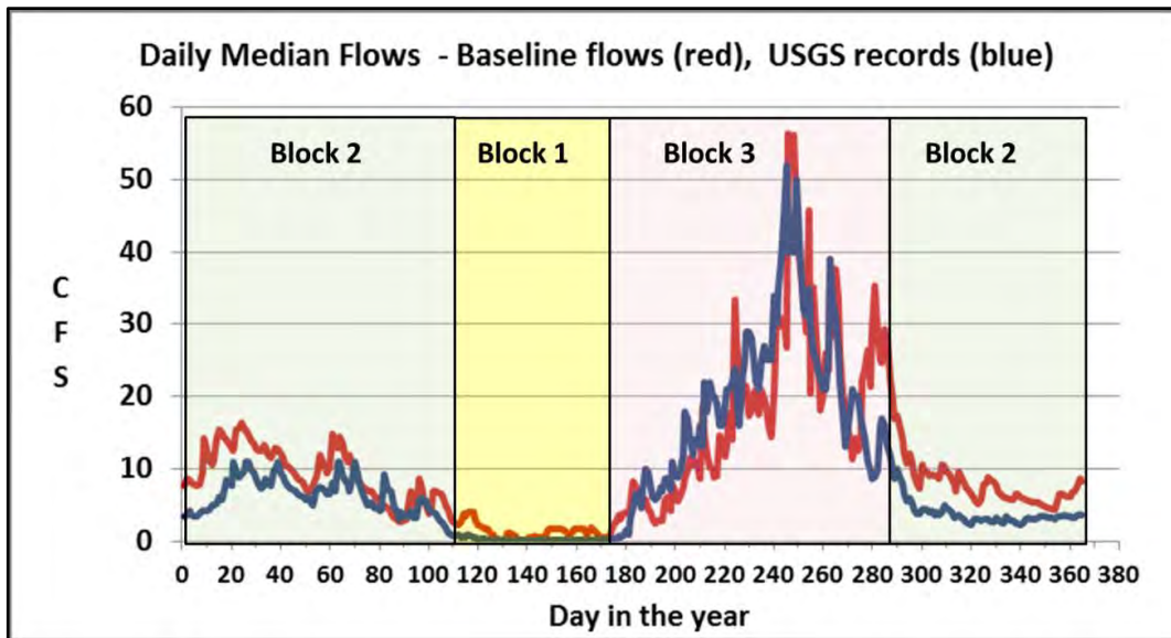
Figure 4-4. Median daily flows for each day of the calendar year for flows recorded at the Pithlachascotee River near New Port Richey gage for years 1982-2012 and baseline flows calculated at the site for the years 1990-2000. Also shown are the three seasonal blocks used for the minimum flows analyses.
