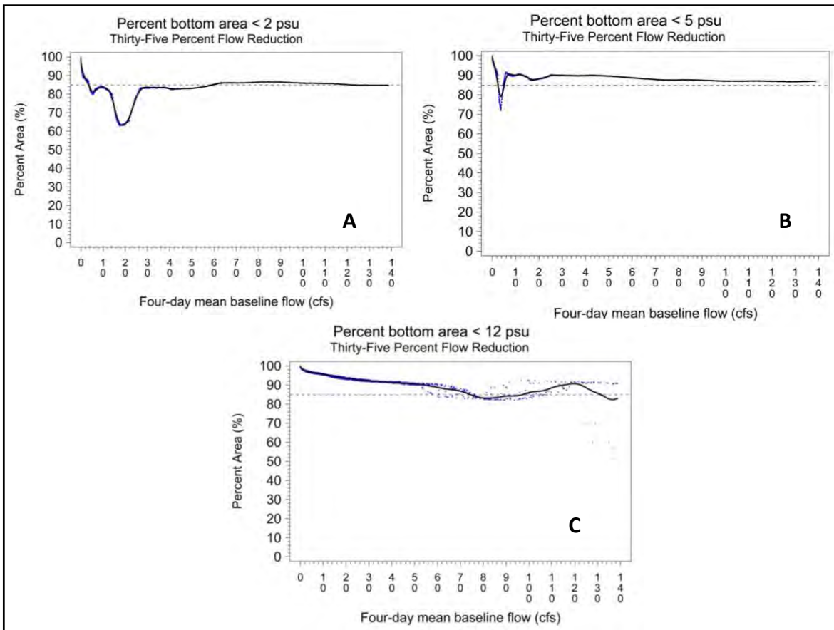
Figure 5-12. Daily values of percent of bottom area for the < 2, <5, and < 12 psu salinity zones for the thirty-five percent flow reduction scenario vs. the preceding four-day mean baseline flow.
