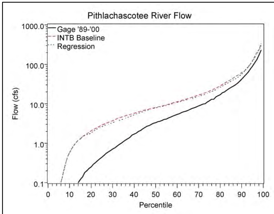
Figure 4-3. Comparison of INTB-modeled baseline (INTB Baseline) flows, baseline flows predicted by substitution into Equation 1 (Regression), and observed (Gage '89-'00) flows at the Pithlachascotee River near New Port Richey gage (reprinted from Janicki Environmental, Inc. 2011). There is little visible difference between the two estimates of baseline flows and both are greater than the observed, gaged flows, as expected.
