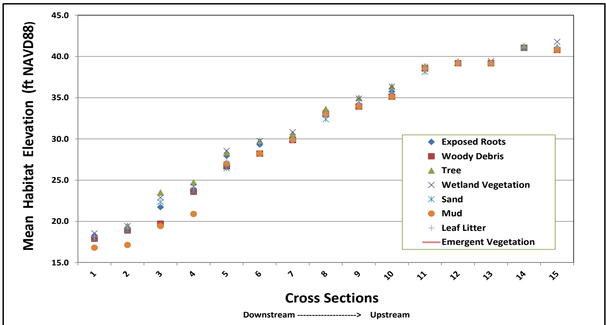
Figure 5-6. Mean elevations of instream habitats at fifteen cross-section sites on the Pithlachascotee River.
