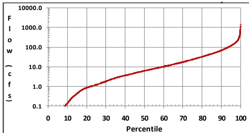
Figure 2-8. Cumulative frequency distribution curve for flows at the Pithlachascotee River near New Port Richey gage for the period of record (April 1, 1963 through September 30, 2013). Flows less than 0.1 cfs were converted to 0.1 cfs for plotting purposes.
