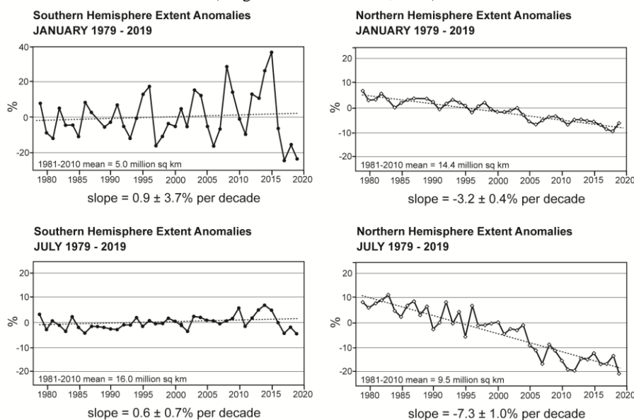
Figure 1. Trends in summer (upper left and lower right) and winter (upper right and lower left) sea-ice extent for both the Northern and Southern Hemisphere polar regions since satellite imagery became available in 1979 (Fetterer and others, 2017; source table ref.1). The slope of the trend line in each panel is shown. The Northern Hemisphere trends are statistically significant at the 0.01 level, while the Southern Hemisphere trends are not significant.
