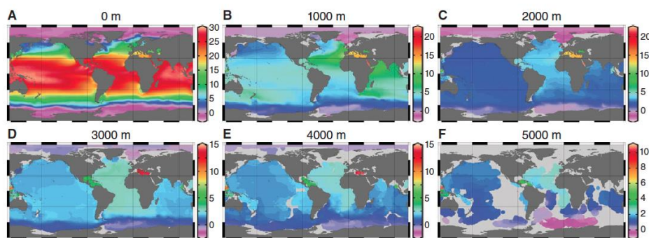
Figure 4. Global temperature (°C) distributions at (A) 0 m, (B) 1,000 m, (C) 2,000 m, (D) 3,000 m, (E) 4,000 m, and (F) 5,000 m water depths. Data from World Ocean Atlas 2009 ( http://www.nodc.noaa.gov/OC5/WOA09/pr_woa09.html ). The map was created using Ocean Data View ( http://odv.awi.de ) (Yasuhara and Danovaro, 2016).
