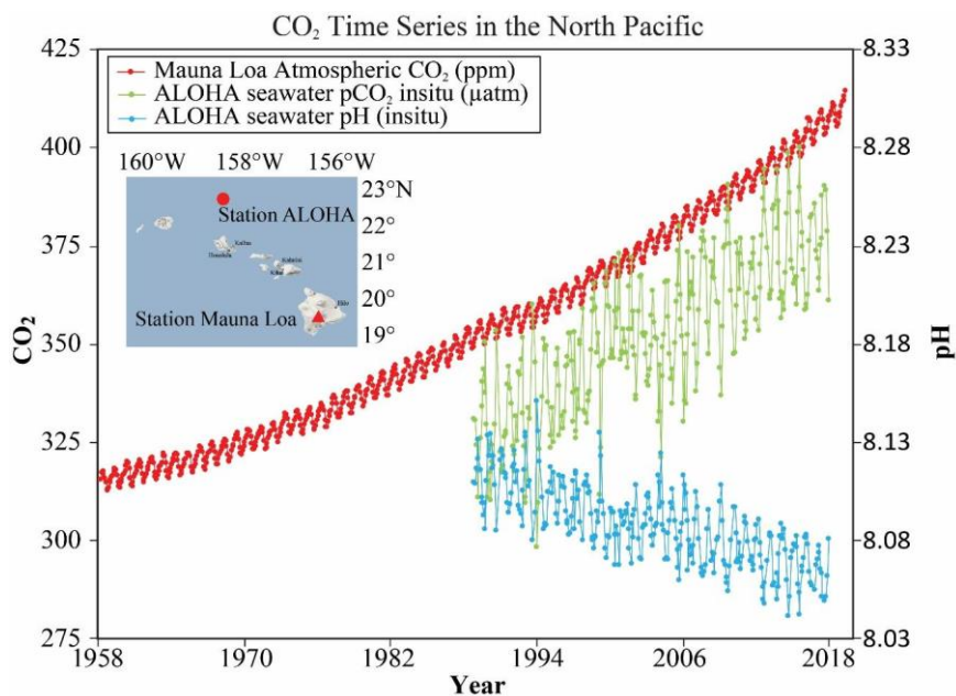
Figure 8. Trends in surface (< 50 m) ocean carbonate chemistry calculated from observations obtained at the Hawaii Ocean Time-series (HOT) Program in the North Pacific over 1988–2018. The figure shows the linked increase in atmospheric (red points) CO 2 concentrations, seawater (green points) pCO 2 concentrations and a corresponding decline in seawater pH (blue points, secondary y-axis). Ocean chemistry data were obtained from the Hawaii Ocean Time-series Data Organization and Graphical System (HOT-DOGS) (Figure source: NOAA PMEL Carbon Program).
