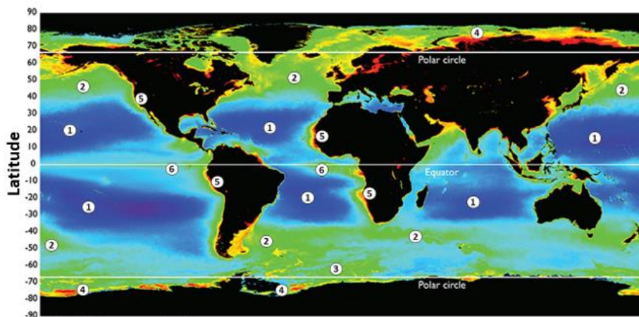
Figure 1. Mean sea surface chlorophyll- a concentration 1997 – 2010 (adapted from Sundby and others, 2016) and
