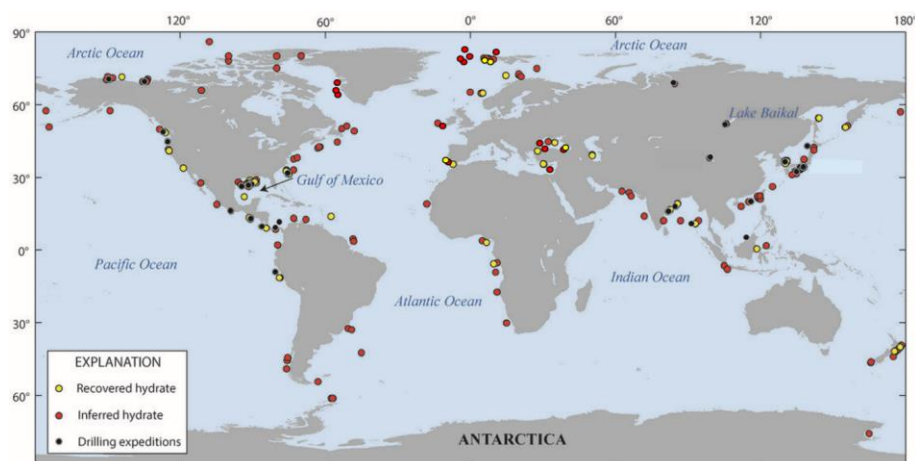
Figure 2. Map showing locations where gas hydrate has been recovered, where gas hydrate is inferred to be present on the basis of seismic data, and where gas hydrate drilling expeditions have been completed in permafrost or deep marine environments, also leading to the recovery of gas hydrate. Source: Ruppel, 2018; amended to reflect Ryu and others, 2013, and Minshull and others, 2020. 305
