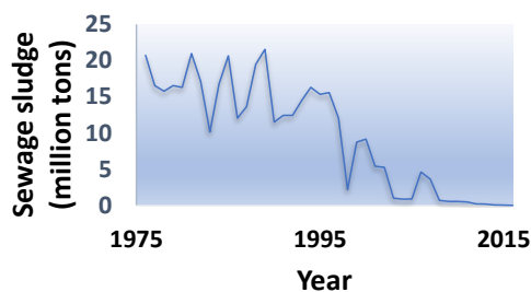
Figure 3. Amount of sewage sludge dumped (IMO, 2019).
