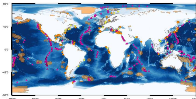
Figure 1: Active vent sites from the InterRidge Vent Database (pink triangles) (Beaulieu and Szafranski, 2020) and seep areas from the Biogeography of Deep-Water Chemosynthetic Ecosystems Database (orange circles) (ChEssBase, 2019) and more recent inventories (yellow circles) (Olu and others, 2010; Quattrini and others, 2015; Baumberger and others, 2018; Feng and others, 2018; Etiope and others, 2019; McDonald and others, 2020). Polygons are currently designed MPAs ( United Nations Environment Programme World Conservation Monitoring Centre database — UNEP-WCMC and IUCN (2019)(WDPA) ). Bathymetry from https://www.gebco.net/data_and_products/gridded_bathymetry_data/ . Map created using Q-GIS version 2.18.20 (QGIS Development Team, 2018).
