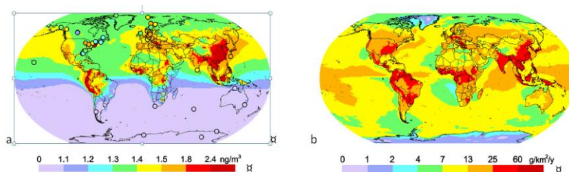
Figure 2. Global distribution of model ensemble median Hg^0 concentration in surface air (a) total (wet and dry) deposition flux (b) in 2015. Source: EMEP homepage, 3 March 2019, and UNEP (2019).
