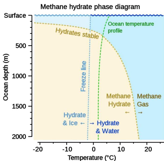
Figure 3: Methane hydrate stability diagram. (Source: https://commons.wikimedia.org/wiki/File:Undersea_methane_hydrate_phase_diagram.svg ).
