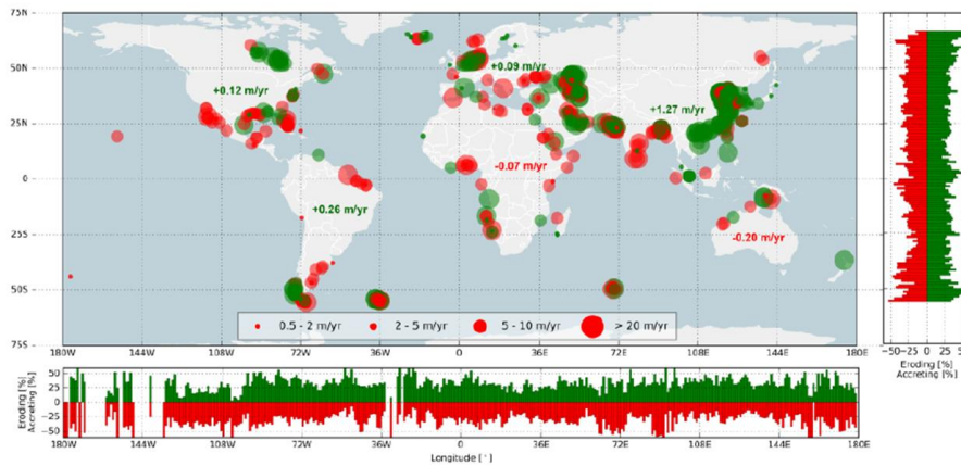
Figure 1. Global hotspots of beach erosion and accretion; the red (green) circles indicate erosion (accretion) for the four relevant shoreline dynamic classifications (see legend). The bar plots to the right and at the bottom present the relative occurrence of eroding (accreting) sandy shorelines per degree latitude and longitude, respectively. The numbers presented in the main plot represent the average change rate for all sandy shorelines per continent. Figure taken from Luijendijk and others (2018a), reprinted under the Creative Commons license ( https://creativecommons.org/licenses/by/4.0/ ).
