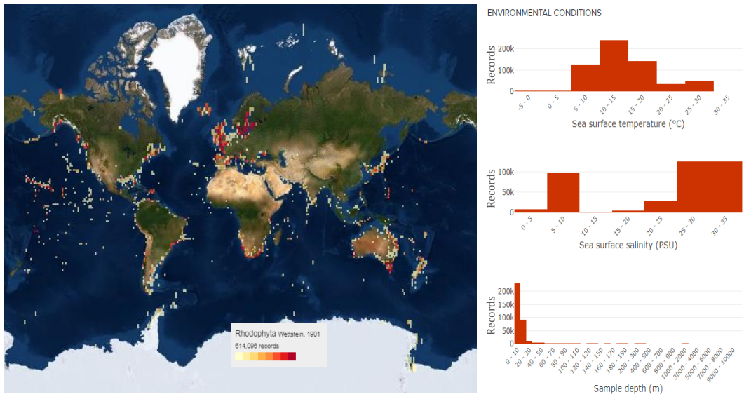
Figure 3. Distribution of red algae (Rhodophyta) and environmental conditions (temperature, sea surface salinity and depths) of occurrence around the world (OBIS 2020, https://mapper.obis.org/?taxonid=852 ).
