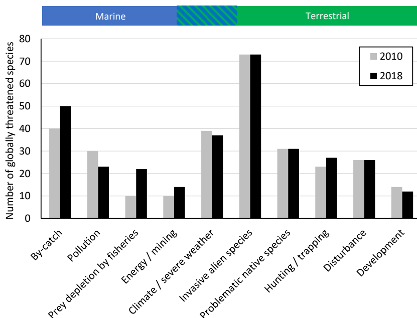
Figure 1. The number of globally threatened seabird species assessed as being affected by marine, terrestrial, and over-arching threatening processes in 2010 (Crocoll and others, 2012, grey bars) and in 2018 (Dias and others, 2019, black bars). Only processes considered in both assessments are shown.
