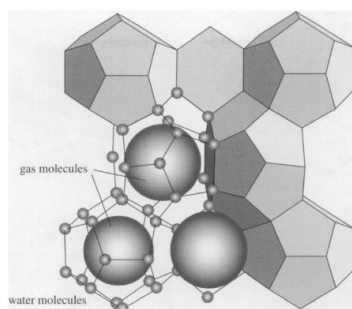
Figure 1. Typical structure of a gas hydrate with water molecules linked together to form a cage that traps gas molecules such as methane within. Source: Maslin and others, 2010.
