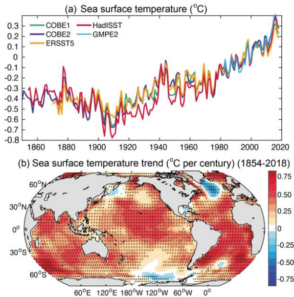
Figure 6. (a) Global average surface temperature anomalies (°C, annual mean). In situ estimates are shown from COBE1, COBE2, ERSST5, HadISST and GMPE2 (GHRSSST (Group for High Resolution Sea Surface Temperature) Multi-Product Ensemble dataset, version 2); (b). Spatial pattern of the long-term SST trend (°C per century) from 1854 to 2018 for ERSST data. All data use a common 1981–2010 baseline. Black dot signs (in b) indicate grid boxes where trends are significant (i.e., a trend of zero lies outside the 90 per cent confidence interval).
