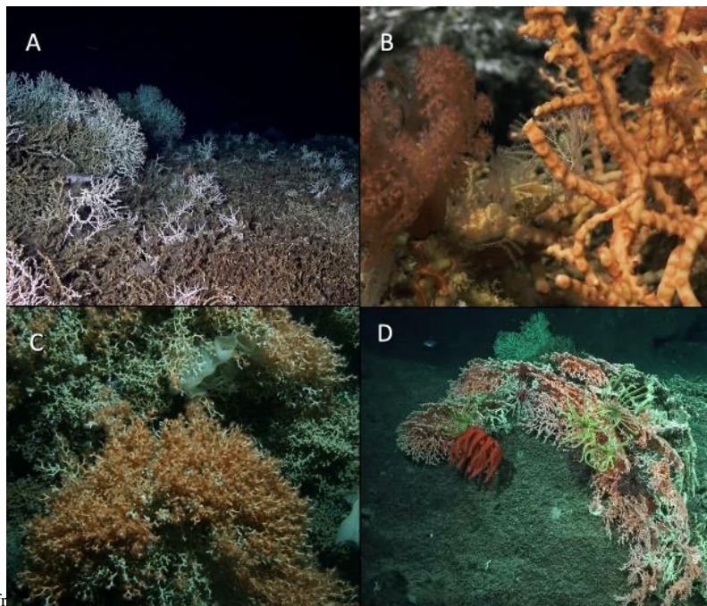
Figure 2. Common cold-water scleractinian corals. A. Lophelia pertusa and B. Madrepora oculata and a neptheid octocoral from the Atlantic coast of the United States. Images courtesy of the Deep Search program, US BOEM, USGS, NOAA, copyright WHOI. C. Solenosmilia variabilis from the Pacific off New Zealand. Image courtesy of Malcolm Clark, NIWA. D. Enallopsamia profunda on the Phoenix Islands in the Central Pacific. Image courtesy of Erik Cordes and the Schmidt Ocean Institute.
