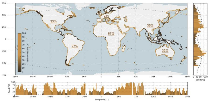
Figure 3. Global distribution of sandy shorelines; the coloured dots along the world’s shoreline represent the local percentage of sandy shorelines (yellow is sand, dark brown is non-sand). The subplot to the right presents the relative occurrence of sandy shorelines per degree latitude, where the dashed line shows the latitudinal distribution of sandy shorelines reported by Hayes (Hayes, M. O. Relationship between coastal climate and bottom sediment type on the inner continental shelf. Jour. Mar. Geol. 5, 111–132 (1967)). The lower subplot presents the relative occurrence of sandy shorelines per degree longitude. The curved, dashed grey lines in the main plot represent the boundaries of the ice-free shorelines considered in our analysis. The underlined percentages indicate the percentages of sandy shorelines averaged per continent. Map is created with Python 2.7.12
