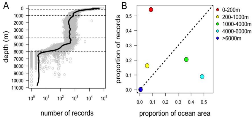
Figure 1. The depth distribution of Ocean Biodiversity Information System (OBIS) records of global marine biodiversity. (A) Number of OBIS records plotted against ocean depth (grey symbols); a loess smooth (solid line) illustrates the general trend. (B) Proportion of all OBIS records occurring in different depth zones, plotted against the proportion of the global ocean that occurs at those depths. The 1:1 line identifies those areas of the ocean with proportionately more (points above the line) or fewer (points below the line) records than expected given their area. This depiction provides a conservative view of under- and over-representation based on the volume of each habitat. Figure retrieved from Webb and others (2010).
