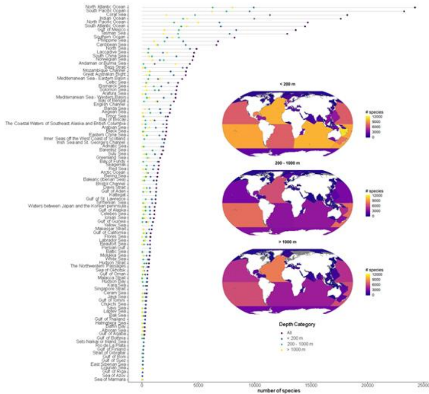
Figure 1. The total numbers of recorded marine invertebrate benthic species are represented as three depth categories (<200m, 200-1000m, >1000m). Information of sea area based on adapted from MarineRegions.org (Claus and others, -(2014); Flanders Marine Institute, -(20198), International Hydrographic Organization Sea Areas version 3 (available online at http://www.marinerregions.org/ - https://doi.org/10.14284/323 ), species occurrences (OBIS, 2019), species group information (WoRMS), and bathymetry data (EMODnet, 2016; GEBCO, 2015; Provoost and Bosch, 2018).
