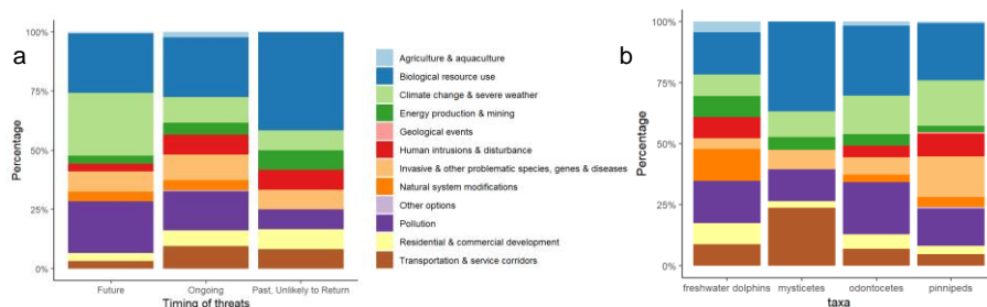
Figure 2. (a) Currently identified main conservation threats for all marine mammals categorized by the timing of their impact on those species; (b) Conservation threats for specific groups. Threat categories are IUCN Red List threats where anthropogenic noise is categorized as pollution and fisheries impacts as biological resource use (IUCN, 2019).
