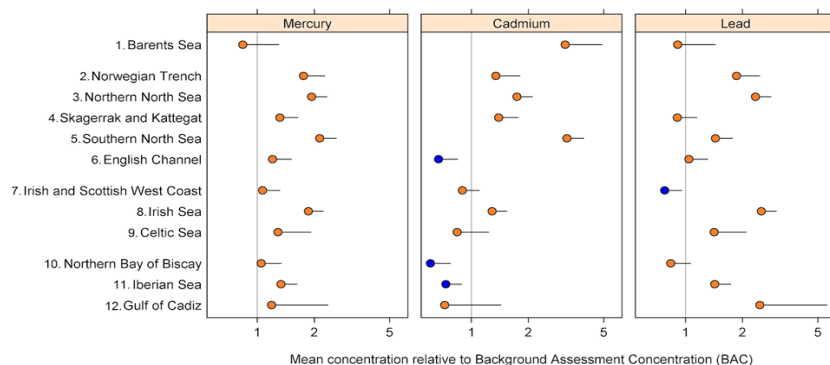
Figure 3. Mean concentrations of mercury, cadmium and lead in fish and shellfish in each assessment area relative to BAC (OSPAR, 2017b). Value of 1 means that the mean concentration equals BAC. Blue: mean concentration statistically significant below BAC and EC maximum levels for food ( p < 0.05 ); orange: mean concentration at (if confidence limit crosses 1), or above BAC, but significantly below the EC maximum levels for food. The EC maximum levels are more than five times higher than the BAC and hence not shown.
