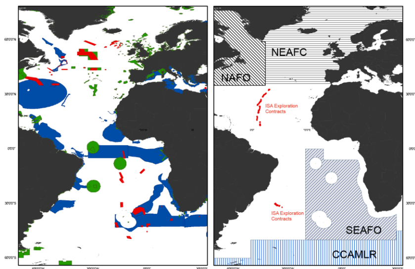
Figure 2. Left: close up for the Atlantic area. Areas identified as Ecological and Biologically Significant (EBSA) and areas with protection measures at the bottom in the Atlantic. Marine Protected Areas in both areas of national or beyond national jurisdiction and the high seas (Green) are from (UNEP-WCMC and IUCN 2019). EBSA (Blue) and areas of closures to bottom fisheries (Red). Right: boundaries of CCAMLR - Convention for the Conservation of Antarctic Marine Living Resources within the Antarctic Treaty system and Regional Fisheries Management Organizations (RFMO). NEAFC- Northeast Atlantic Fisheries Commission; NAFO – Northwest Atlantic Fisheries Organization; SEAFO – South East Atlantic Fisheries Organization. The red Polygons represent ISA exploration contracts in the Area.
