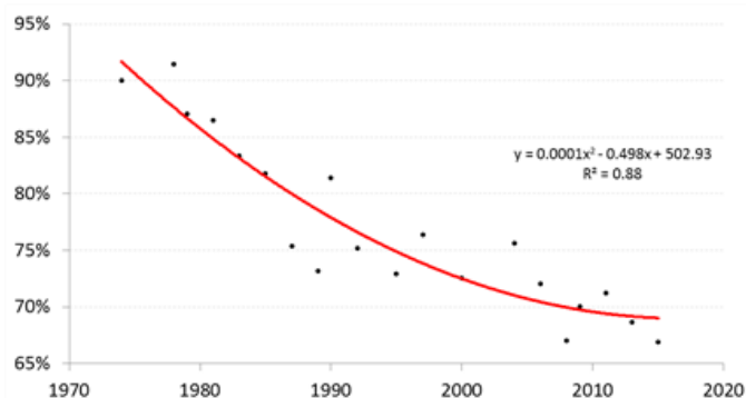
Figure 1. Proportion of fish stocks within biologically sustainable levels, SDG indicator 14.4.1. These data comprised the sum of the percentages of the world’s marine capture fisheries that were considered to be either “maximally sustainably fished” (59.6% in 2017) or “underfished” (6.2% in 2017). Note that the percentage of fisheries that were maximally sustainably fished increased from 1990 to 2017. Alternatively, if subtracted from 100% in any year, the data comprised the growing percentage of the number of fisheries that were “overfished” (FAO, 2020a, 2020b).
