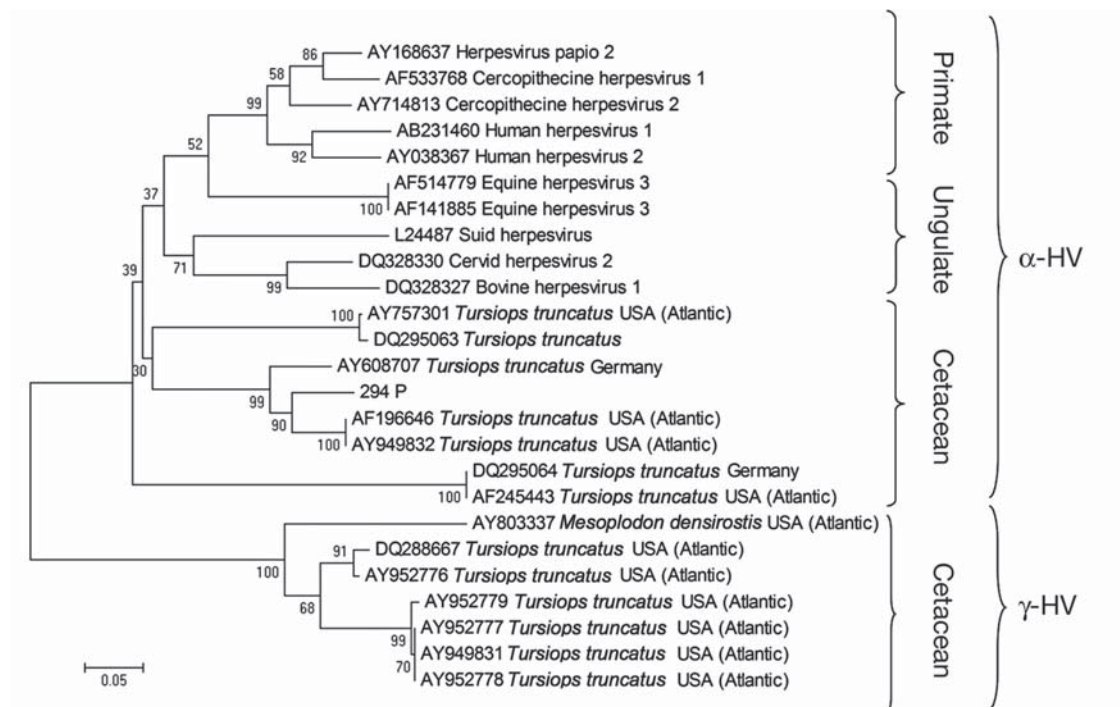
Fig. 5. Neighbor-joining phylogram of 25 selected sequences from cetacean alpha- and gammaherpesvirus (HV) and other phylogenetically related alphaherpesviruses. Either the virus name or the host species is given alongside each GenBank Accession Number. The isolate from the present study (294P, GenBank Accession Number GU066291) showed greatest homology (84.2%) with Genbank sequences AF196646 and AY949832
