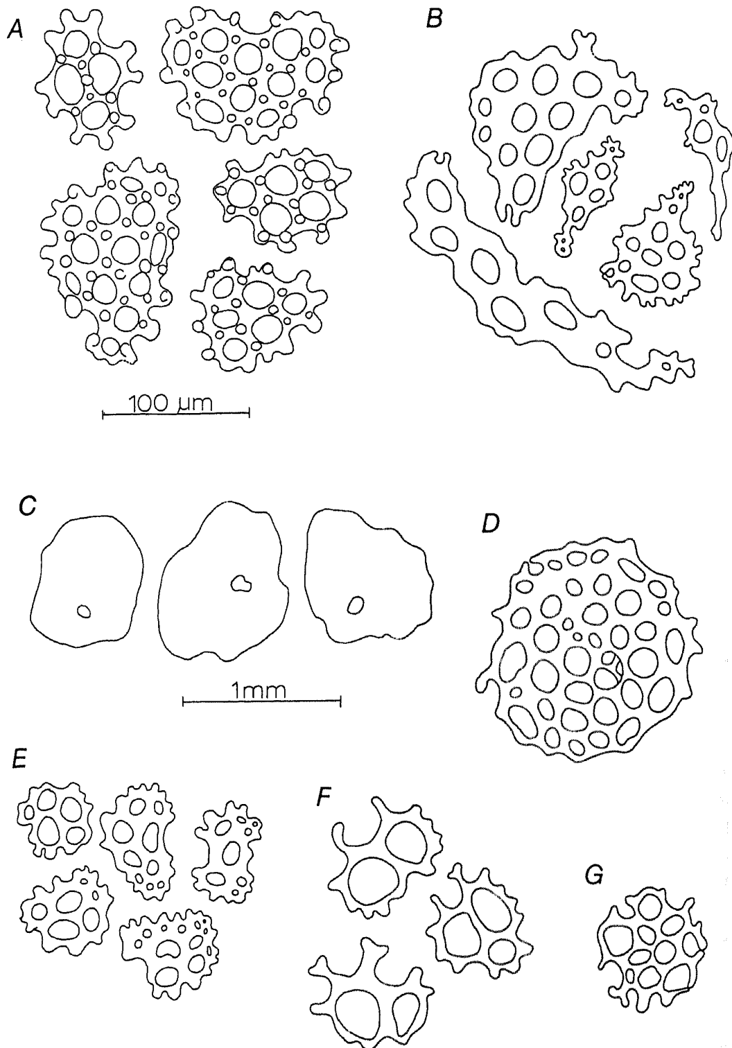
Fig. 2. Psolidium prostratum , ossicles: A, Knobbed buttons from sole; B, Perforated plates from tentacles; C, Outline drawings of dorsal plates, showing holes for passage of tube feet; D, Endplate from ventral tube foot; E, Plates from dorsal tube feet; F, Developing buttons from sole of 1.5 mm total length juvenile; G, Endplate from tube foot of 1.5 mm total length juvenile. The scale on Fig. 2A also applies to figs. 2B, D-G.
