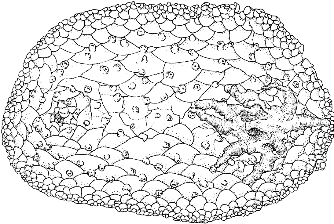
Fig. 1. Psolidium prostratum : Holotype, dorsal aspect. Drawing by C. G. Messing.
