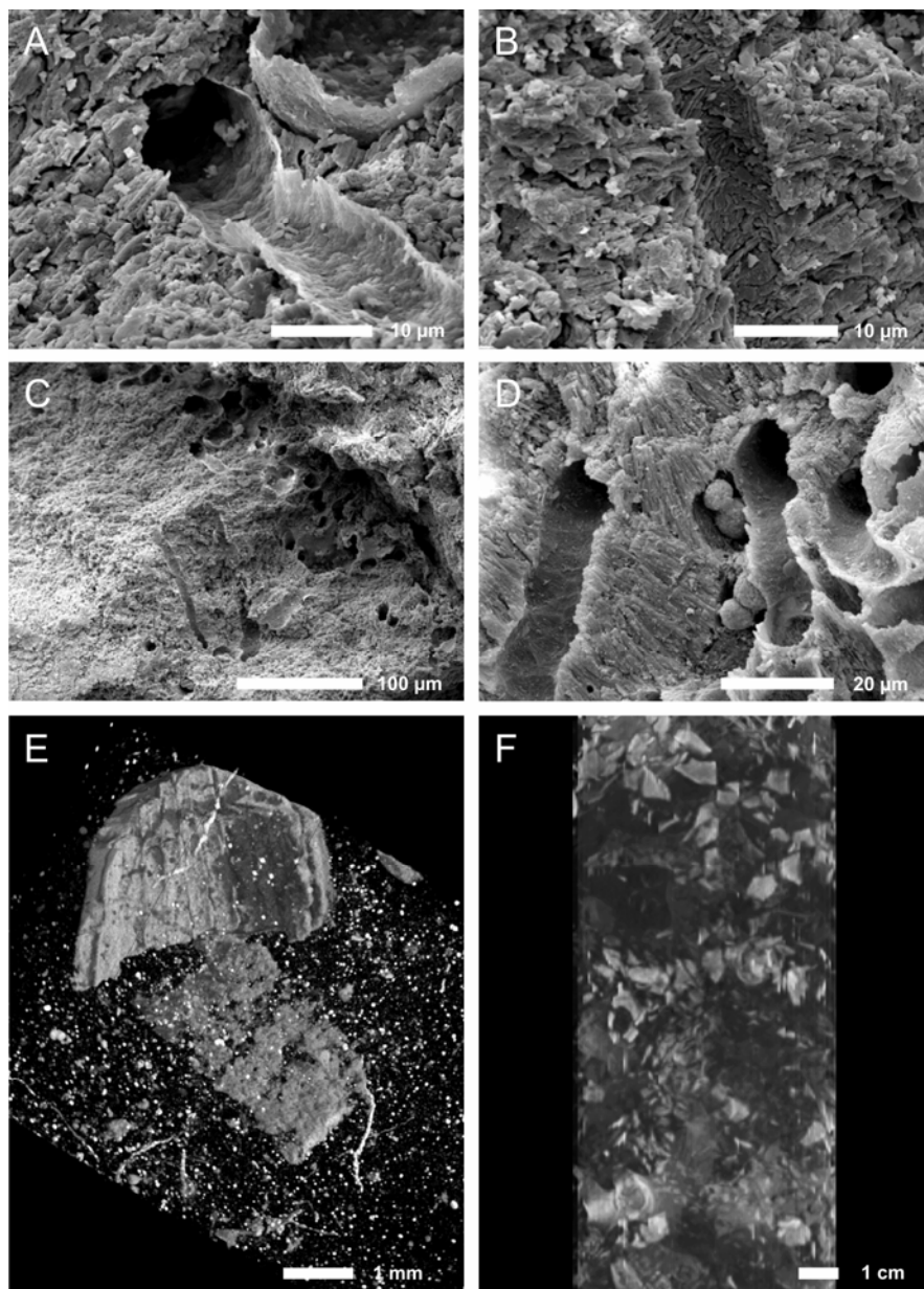
Fig. 3.12 A-D SEM pictures (Léonide 2006) presenting different traces of bioerosion on the coral fragments. Tunnels of 5 to 10 μm are Orthogonum lineare (Glaub 1994) (A-B) and round chambers are Saccomorpha clava (Radtke 1991) (C-D). E μCT scan showing dissolution of coral fragment. F medical CT scan showing fragmentation of coral fragments.
