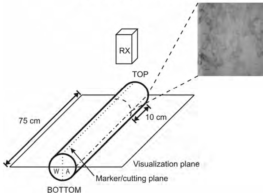
Fig. 6.4 Method of two-dimensional X-ray analyses for unopened cores containing coral fragments as used with SCOPIX (DGO, University Bordeaux I).
