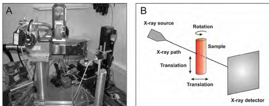
Fig. 3.2 A Picture of the set-up of the micro-CT scanner installed at the UGCT (Masschaele et al. subm.). B Schematic illustration of the set-up of a micro-CT scanner (modified after Cnudde 2006).
