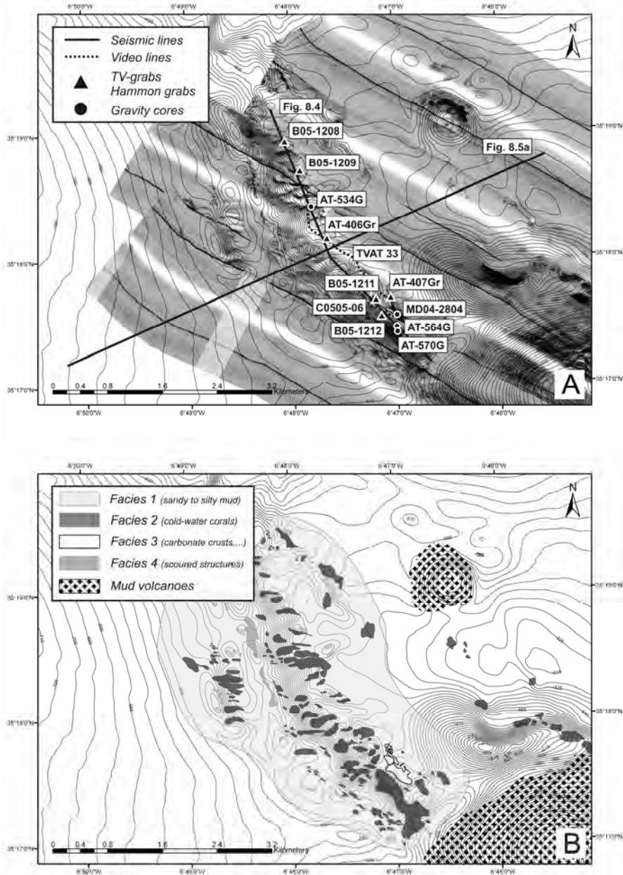
Fig. 8.3 A Bathymetry (contour spacing is 5 m), sidescan sonar imagery and location of the seismic profiles, core material and video lines in the Pen Duick Mound Province. B Interpretation of sidescan sonar imagery (MAKAT 66-68), representing the four described facies.
