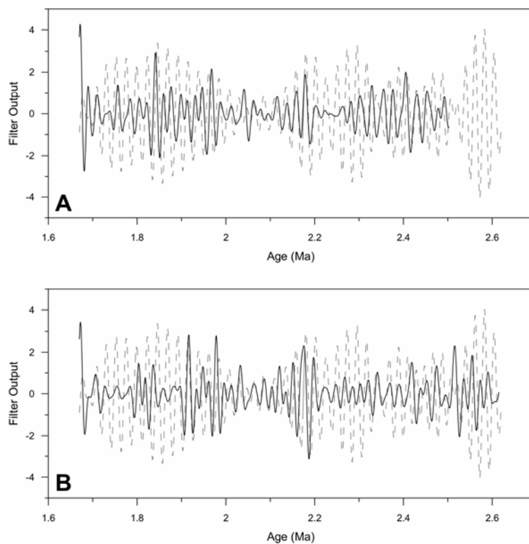
Fig. 5.11 Gaussian filter centred at 0.05 ka (20 ka period) with a 0.02 ka band-pass applied to the susceptibility record (solid black line) compared with the orbital solution for obliquity and precession from Berger and Loutre (dashed grey line) (1991) for Holes U1317B ( A ) and U1317E ( B ).
