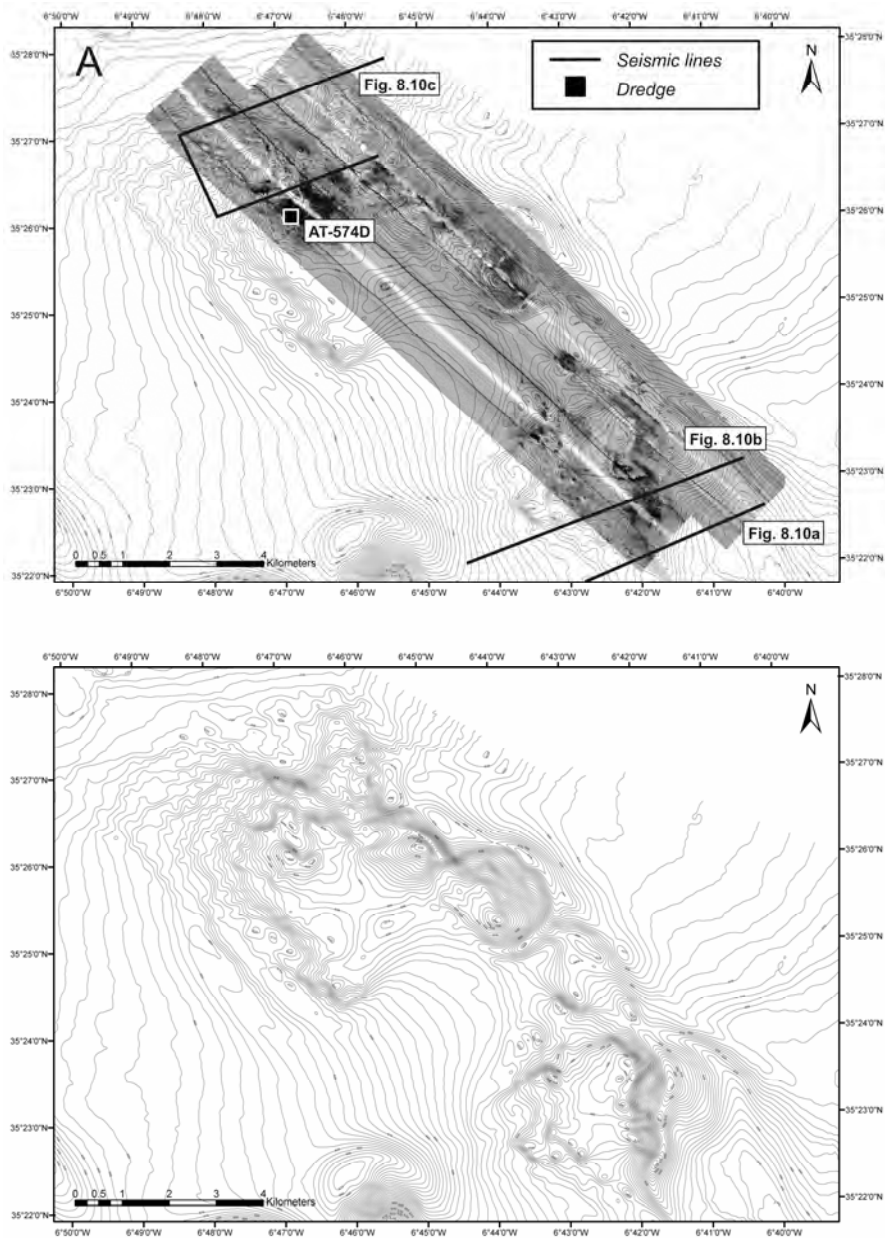
Fig. 8.9 A Bathymetry (contour spacing is 5 m), sidescan sonar imagery and location of the seismic profiles and core material in the Vernadsky Mound Province. B Interpretation of sidescan sonar imagery (MAKAT 107-108), representing four distinctive facies.
