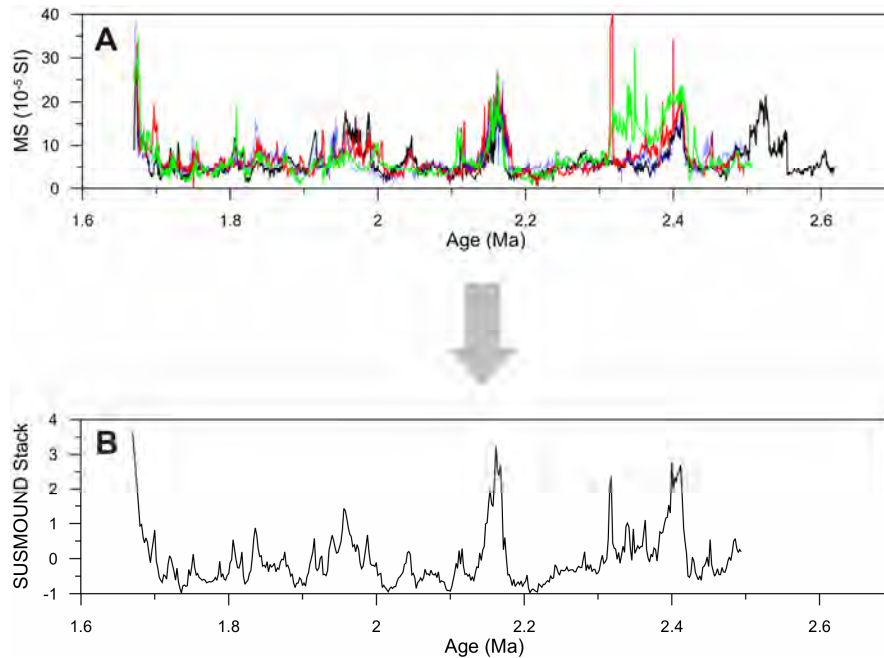
Fig. 5.13 A Magnetic susceptibility records for Holes U1317A (green line), U1317B (blue line), U1317C (red line), and U1317E (black line) placed on an age model defined by tuning the susceptibility records with the standard benthic \delta\text{O}^{18} TARGET curve (Shackleton et al. 1990, 1995a, b). B SUSMOUND stack determined as an arithmetic mean of the individual normalized (subtraction of core mean and division by standard deviation), interpolated ( \delta t = 2 ka) susceptibility records from Holes U1317A, U1317B, U1317C, and U1317E.
