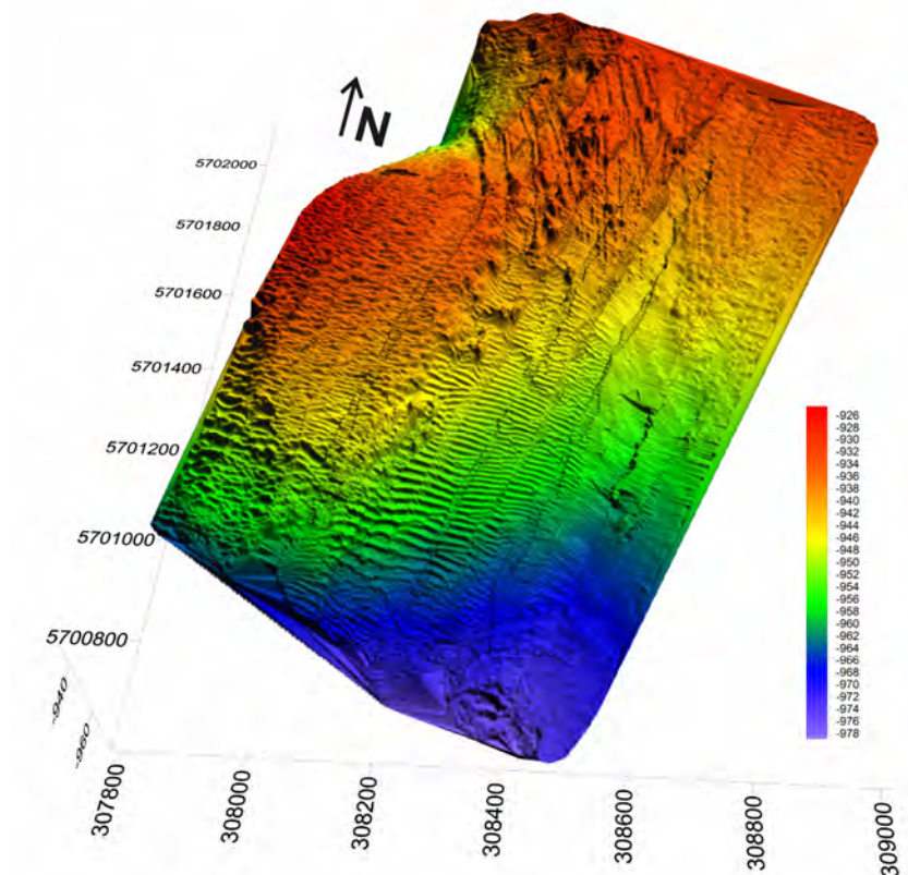
Fig. 7.5 Three-dimensional view of the micro-bathymetric grid over the Moira Mounds east of Thérèse Mound and the surrounding sedimentary environment.
