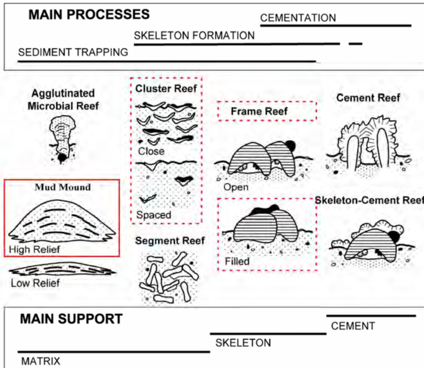
Fig. 3.19 Outline of "organic reef" and "carbonate mud mound" classification, showing main processes and structural support (after Riding 2002). Red boxes suggest appropriate names for Challenger Mound.
