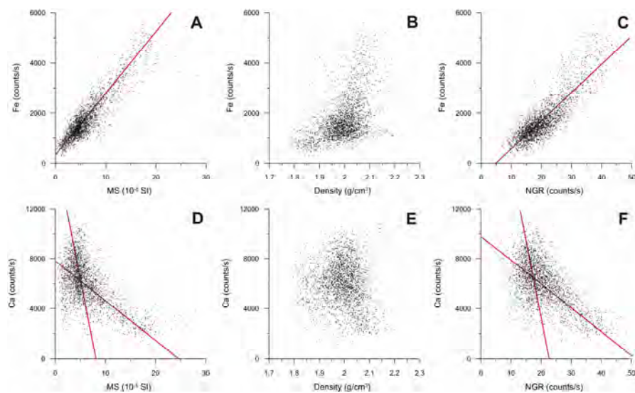
Fig. 4.9 A Fe intensities (counts/s) in function of magnetic susceptibility ( 10^{-5} SI units). B Fe intensities (counts/s) in function of GRA density ( g/cm^3 ). C Fe intensities (counts/s) in function of NGR (counts/s). D Ca intensities (counts/s) in function of magnetic susceptibility ( 10^{-5} SI units). E Ca intensities (counts/s) in function of GRA density ( g/cm^3 ). F Ca intensities (counts/s) in function of NGR (counts/s). Red lines represent trend lines but have no statistical relevance.
