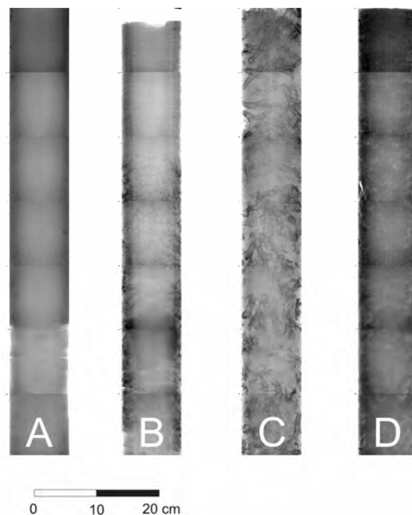
Fig. 6.7 Four different "radiofacies", based on the coral content (X-ray imagery); darker values represent denser material: (A) facies with no corals but only sediment, (B) a combined facies consisting of small coral and bioclastic fragments (debris) embedded in a matrix of silty sediments, (C) facies with large coral chunks filled up by sediments (sediment filled coral framework), (D) facies with altered and dissolved coral fragments.
