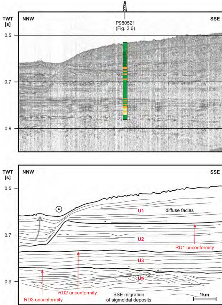
Fig. 2.17 High-resolution NNW-SSE seismic profile P010520, illustrating the upslope sediments off Challenger Mound (modified after Van Rooij et al. 2004). The different described units and unconformities are annotated. The location of the described seismic profile is noted on Fig. 2.16. The drill location is visualized.
