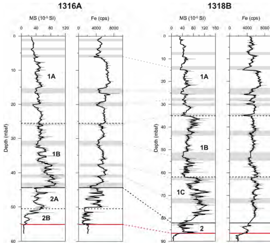
Fig. 4.14 Correlation between Hole U1316A and U1318B based on magnetic susceptibility (SI units) and Fe intensities (counts/s). Grey lines represent raw values. Black lines represent smoothed records (7-points running mean). Grey boxes correspond with specific minima and maxima. Red horizontal line corresponds with the mound base. Black horizontal lines and numbers represent correlating lithological units as described by the Exp. 307 Scientists (2006c, 2006e) and summarized in Sect. 3.5.2.
