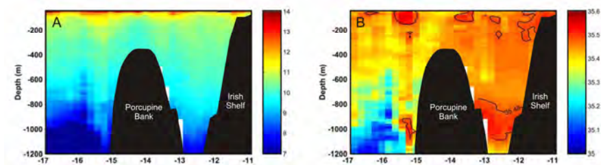
Fig. 2.10 Transect of temperature ( A ) and salinity ( B ) across the Porcupine Seabight and Porcupine Bank at 51.5°N in June 2002, taken from Mohn et al. (2002) and White et al. (1998, 2007). A colourscale for all plots is shown on the right. The salinity 35.48 contour on Fig. 2.10B is shown for clarity.
