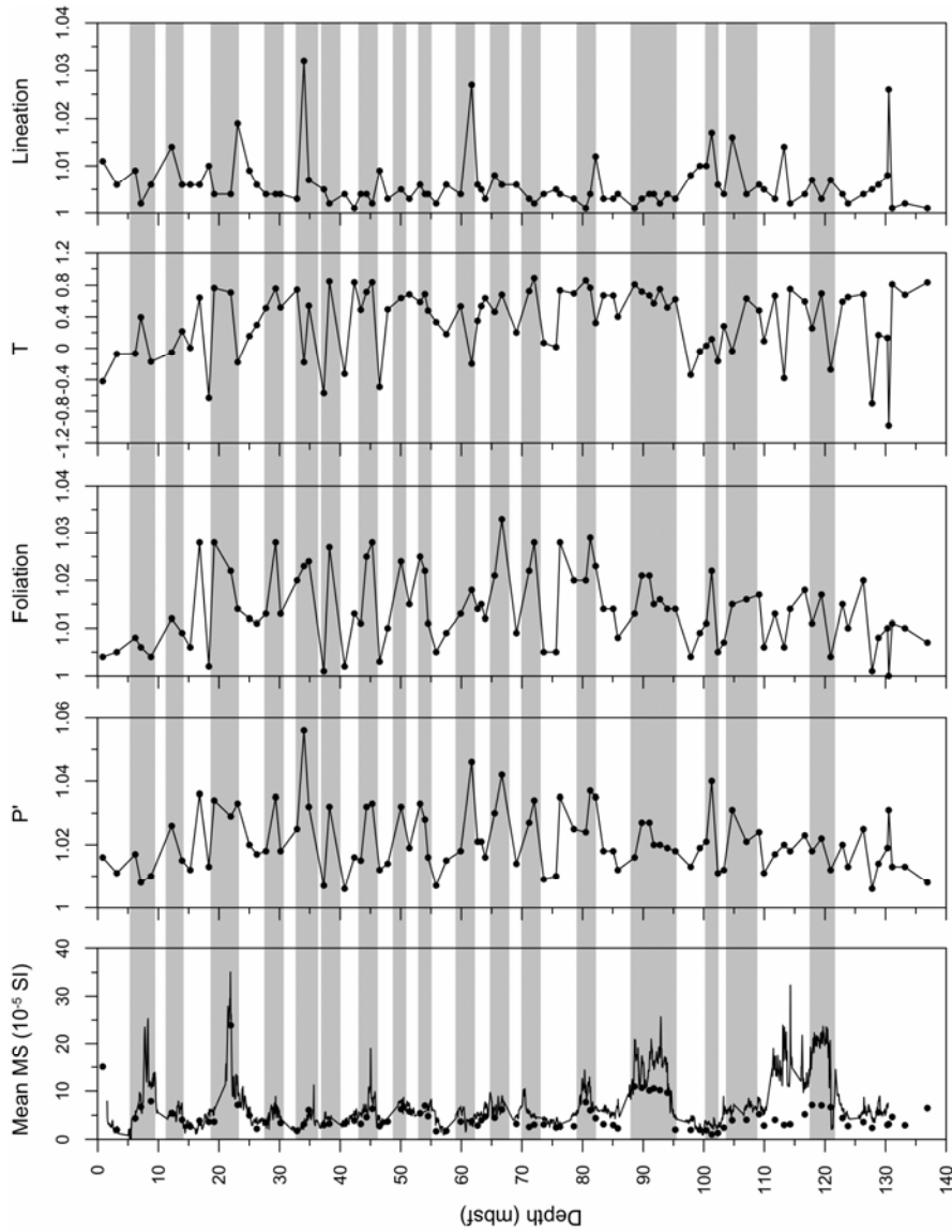
Fig. 5.9 The degree of anisotropy P' , shape parameters T , L (lineation) and F (foliation) and mean susceptibility in function of depth (mbsf). Grey boxes represent correlations between the different parameters (peaks in degree of anisotropy can be correlated with peaks in the magnetic susceptibility).
