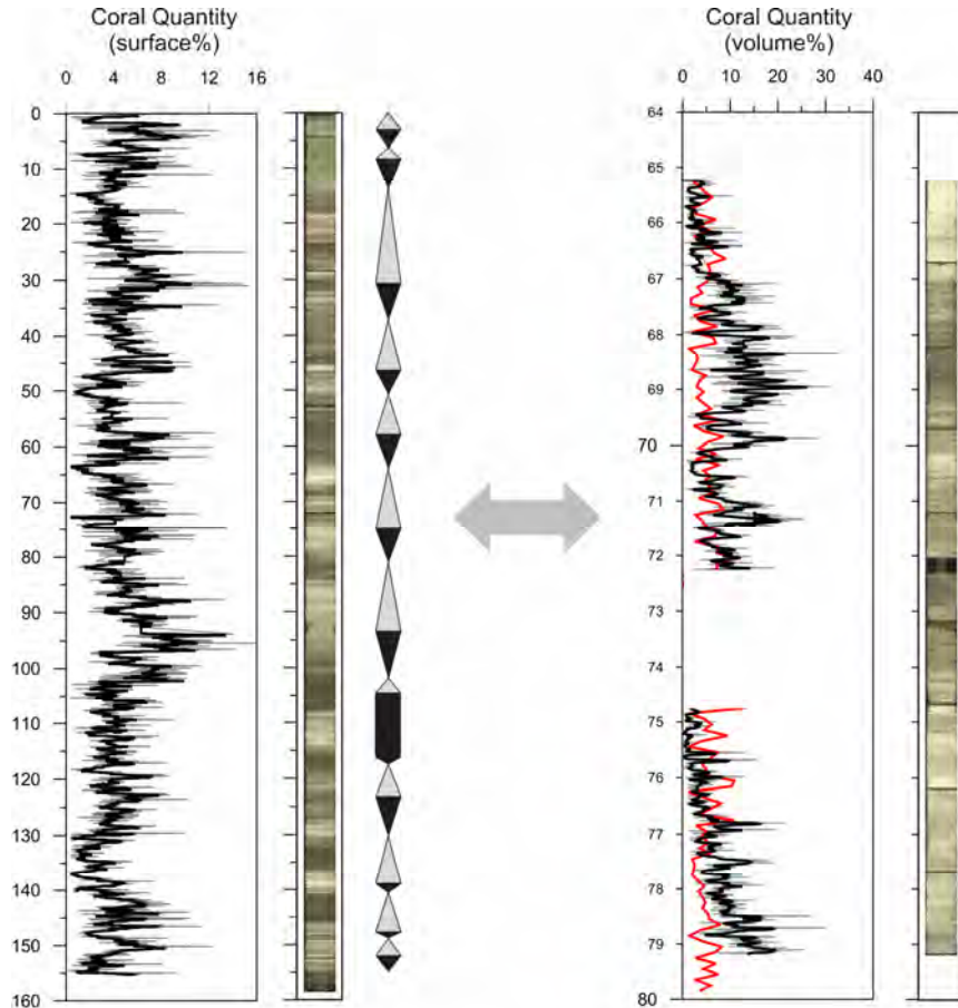
Fig. 3.9 Left panel: Surface percentage of coral determined on two-dimensional surface pictures of split core sections and image stack in function of depth (mbsf) for Hole U1317E. Grey line represents raw records. Black line represents smoothed record (7-points running mean). Right panel: Volume percentage of coral determined on medical CT scans from whole-round Sections 307-1317E-8H-2 to 6, 307-1317E-9H-2 to 4 and corresponding image stack in function of depth (mbsf). Grey line represents raw record. Black line represent smoothed record. Red line represents corresponding surface percentages.
