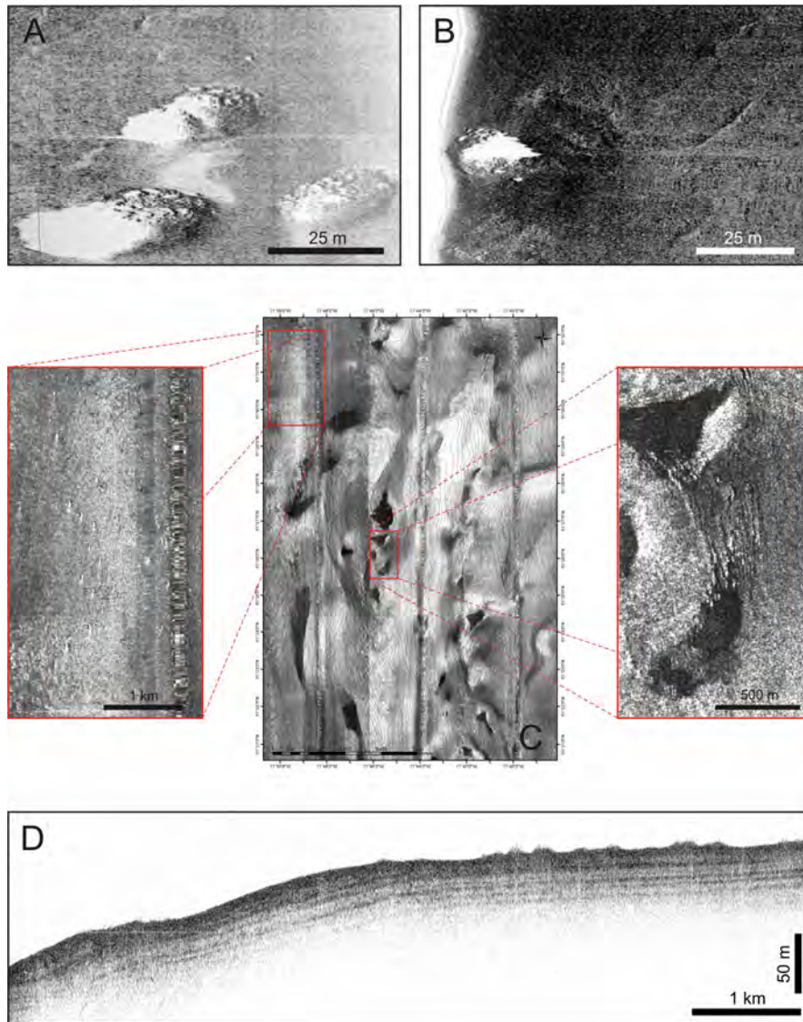
Fig. 7.3 A-B Moira Mounds visualized on 100/410 kHz GeoAcoustic sidescan sonar imagery, collected during the RRS Discovery 248 cruise (Bett et al. 2001; Kozachenko 2005; Wheeler et al. 2005b). C TOBI sidescan sonar imagery of the Belgica Mound Province (de Haas et al. 2002; Huvenne et al. 2005). Insets display the small Moira Mounds on the TOBI sidescan sonar imagery. D Detail of 3.5 kHz echosounder profile showing small positive features on the seabed, interpreted as the Moira Mounds.
