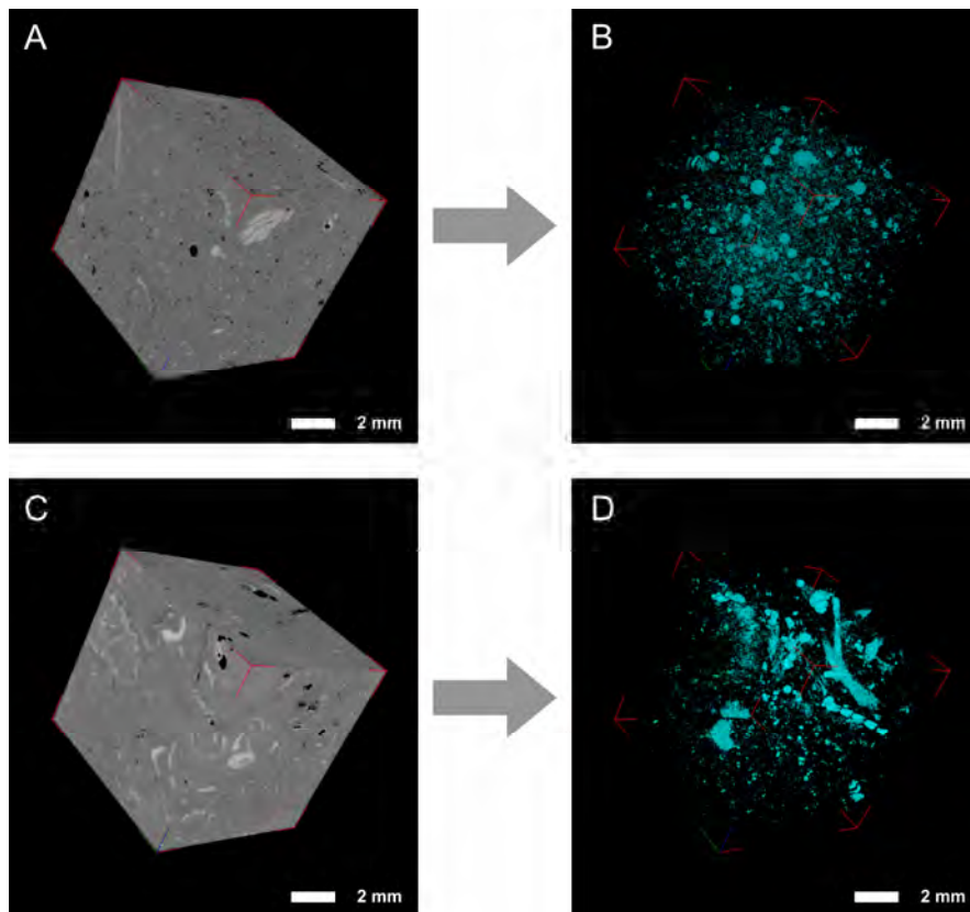
Fig. 3.15 Micro-CT scans representing bioclasts, matrix and porosities (left panels) and porosities (right panels). A-B Sample from Section 307-1317A-2H-3 representing intergranular and intragranular porosity. C-D Sample from Section 307-1317A-6H-3 visualizing intergranular and intragranular porosity.
