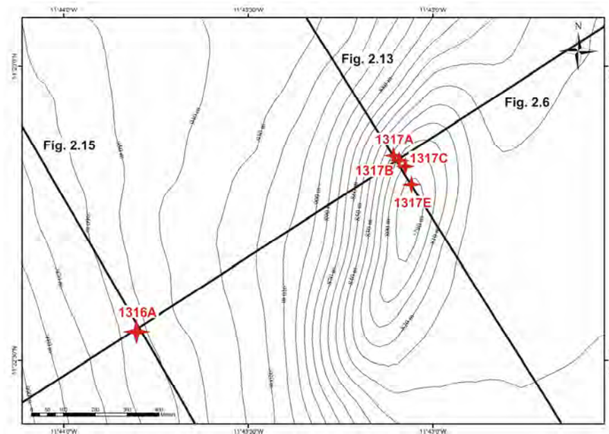
Fig. 2.12 Bathymetric map of Challenger Mound showing the location of the IODP Holes (on-mound Site U1317 and off-mound Site U1316) (red stars) and the seismic lines visualized on Figs 2.6, 2.13 and 2.15. Contour interval set at 10 m. Map is based on AWI bathymetry (Beyer et al. 2003).
