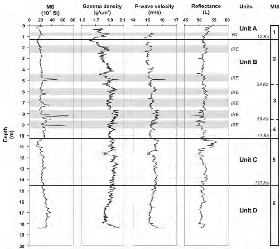
Fig. 6.6 Interpretation of core MD01-2452 based on magnetic susceptibility ( 10^{-5} SI), gamma density ( \text{g}/\text{cm}^3 ), P-wave velocity (m/s) and reflectance ( L^* ). Grey boxes correspond with IRE. A tentative correlation with Marine Isotopic Stages (MIS) according to Martinson et al. (1987) is proposed.
