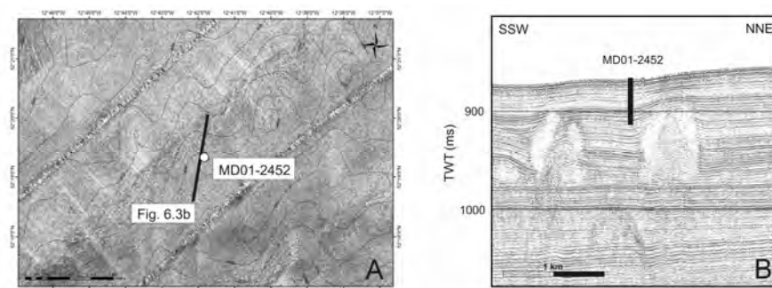
Fig. 6.3 Localization of core MD01-2452 (Magellan Mound Province). A TOBI sidescan sonar imagery of sediments above buried Magellan Mounds (de Haas et al. 2002) and GSI multibeam bathymetry. Contour interval is set at 10 m. B SSW-NNE orientated RCMG sparker profile through core site.
