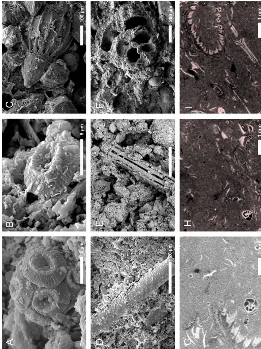
Fig. 3.7 SEM pictures (Léonide 2006) (A-F) and \mu CT scans (G-I) from bioclasts in the mound sediments: (A-B) coccoliths (C) radiolarian (D) sponge spiculae (E) echinoid spine (F) foraminifera (G-H-I) foraminifera, bivalve and echinoderm fragments in micritic matrix.
