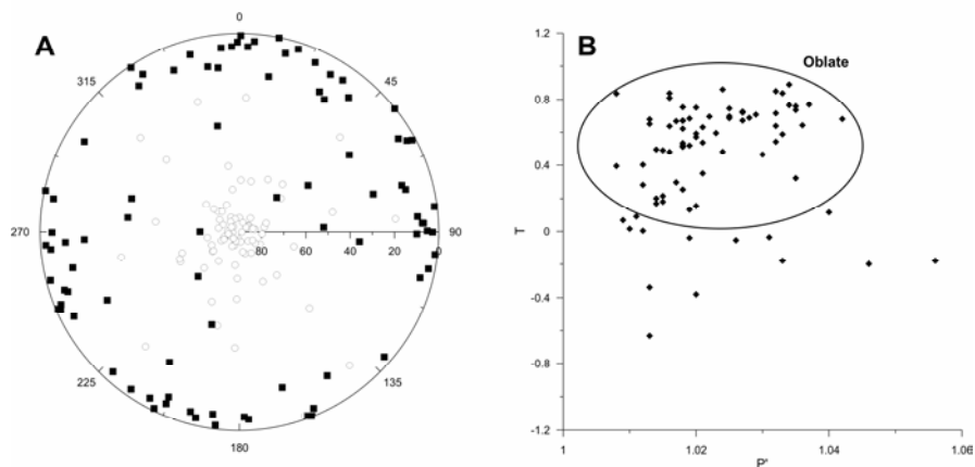
Fig. 5.8 A Stereographic projection of the K_1 (maximum) (black squares) and K_3 (minimum) (white circles) axes of the anisotropy of magnetic susceptibility (AMS). B Shape parameter T versus the corrected degree of anisotropy P' .
