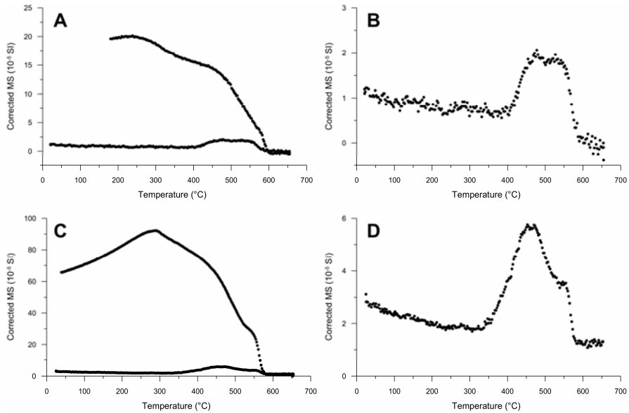
Fig. 5.7 Heating and cooling curves (magnetic susceptibility ( 10^{-5} SI units) in function of temperature ( ^{\circ}\text{C} )) for samples at Section 307-1317A-2H-3 at 9.98 mbsf (A) and Section 307-1317A-3H-3 at 19.84 mbsf (C). Heating curves for samples at Section 307-1317A-2H-3 at 9.98 mbsf (B) and Section 307-1317A-3H-3 at 19.48 mbsf (D).
