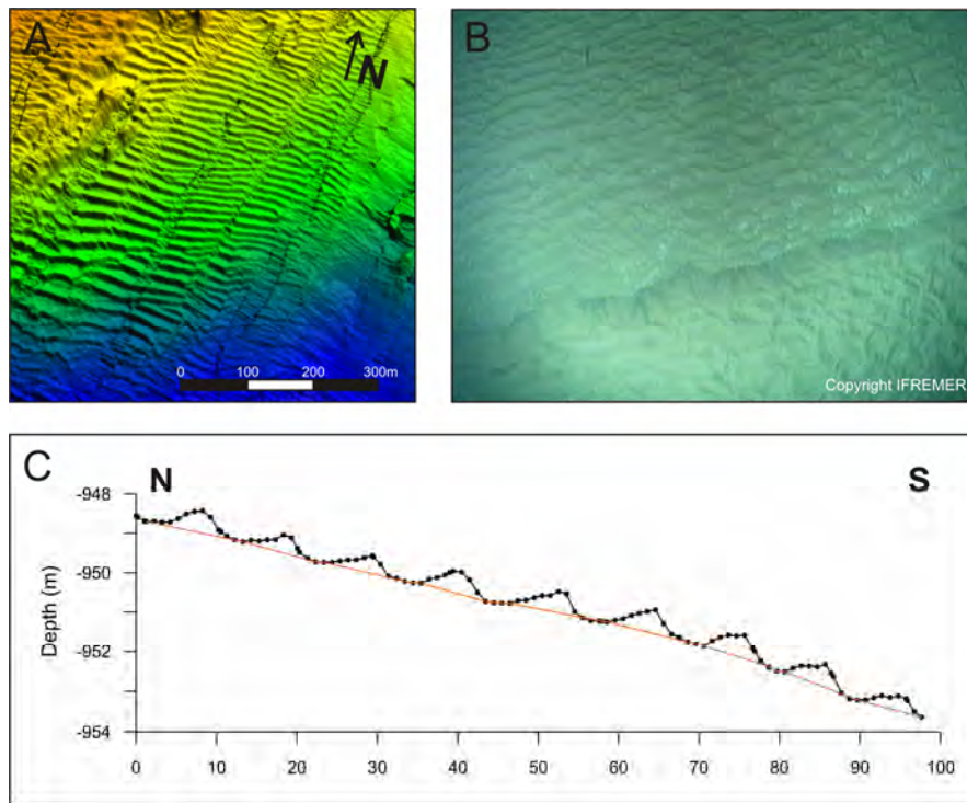
Fig. 7.7 A Zoom in on zone 1 of the micro-bathymetric grid visualizing the regular E-W directed sandwaves. B ROV video imagery showing the sandwave-pattern with superimposed ripples. Note the changing ripple patterns, probably resulting from local variations in bottom current speed and direction. C N-S profile through the sandwaves (for location see Fig. 7.6).
