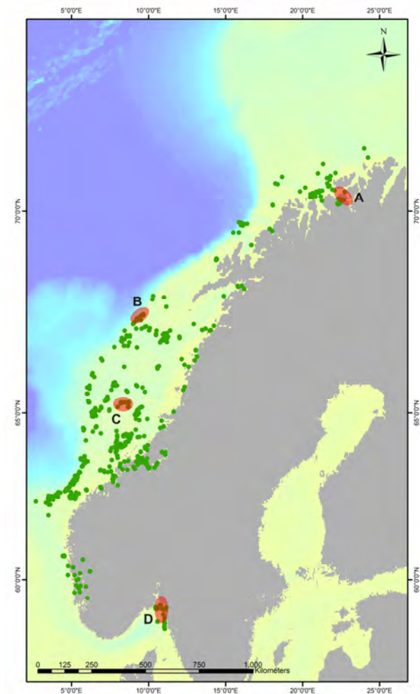
Fig. 1.2 Location of the most important cold-water coral reef frameworks (red ellipses) and distribution of the cold-water coral species Lophelia pertusa (green dots) ( http://www.searchnbn.net/hosted/ospar/ospar.html ; Wisshak et al. 2006) along the Norwegian margins plotted on GEBCO bathymetry. (A) Stjernesund Reef, (B) Røst Reef (C) Sula Reef Complex and, (D) eastern Skagerrak Reefs.
