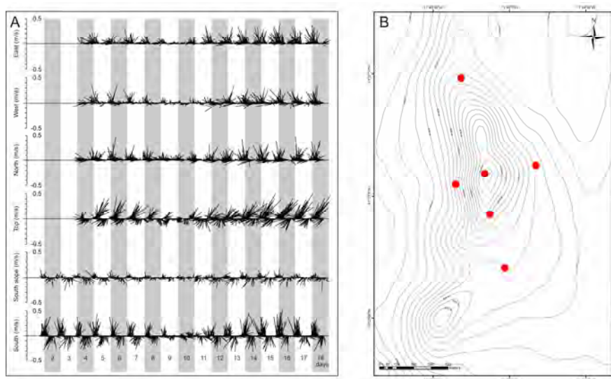
Fig. 2.11 A Current vectors, calculated from current meter measurements on the top and the flanks of Galway Mound, plotted against time (modified after Dorschel et al. subm.). The numbers are days in June 2003 starting with 08.06.2003. B Position of the current meters deployed on the top and the flanks of Galway Mound (Dorschel et al. subm.).
