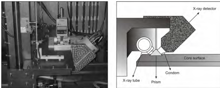
Fig. 4.2 Picture and schematic illustration of the measurement chamber of the XRF core scanner of the Geosciences Department of Bremen University. The X-ray tube and the detector are orientated so that the incident beam and the detector make an angle of 45^\circ with the surface of the sample. Schematic illustration is modified after Röhl and Abrams (2000).
