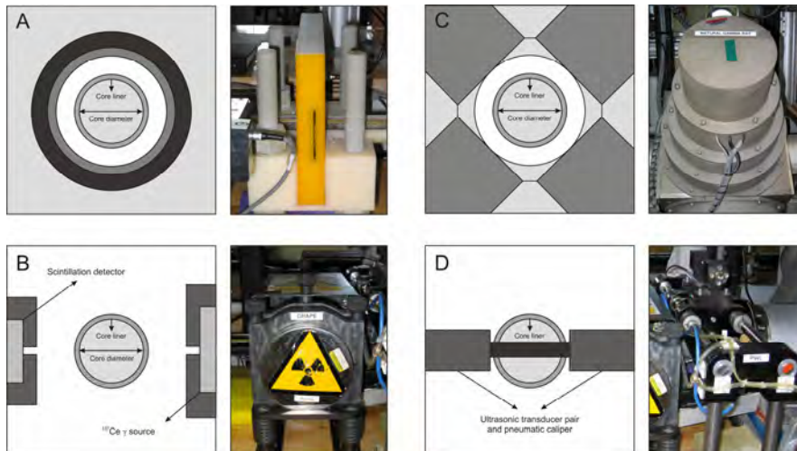
Fig. 4.1 A Schematic illustration and picture of the measurement geometry of the Bartington Model MS-2 meter integrated in the multi-sensor track (MST) for whole-core logging of the magnetic susceptibility. B Schematic illustration and picture of the measurement geometry for whole-core logging of the gamma-ray attenuation (GRA) density. C Schematic illustration and picture of the measurement geometry for whole-core logging of the natural gamma radiation (NGR). D Schematic illustration and picture of the measurement geometry for whole-core logging of the P-wave velocity (PWL). Schematic illustrations are modified after Blum 1997.
