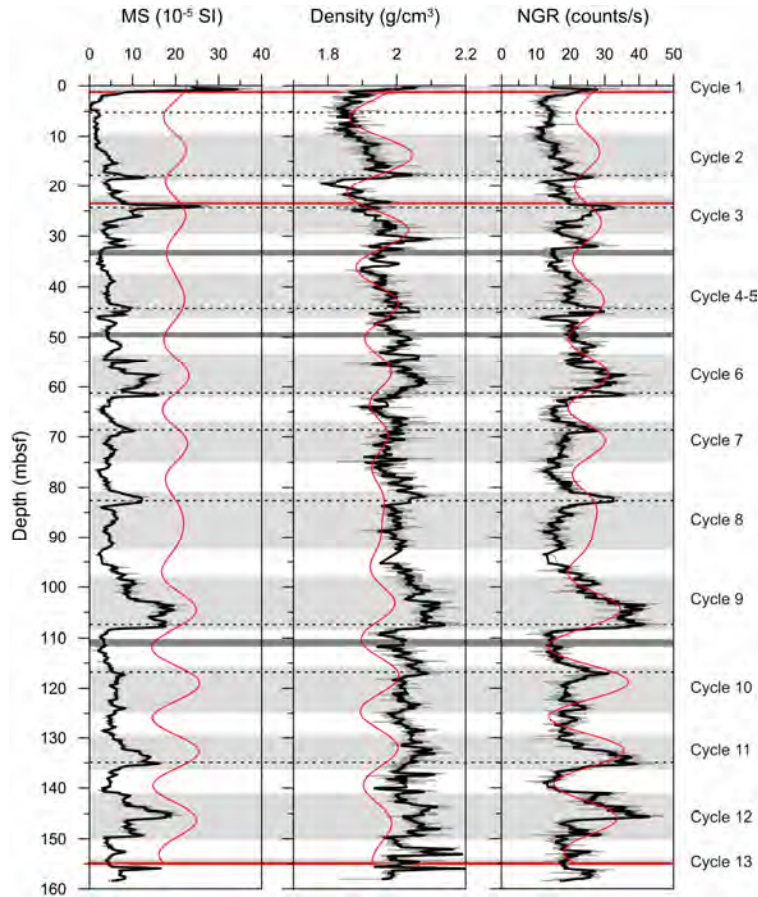
Fig. 4.6 Geophysical properties (magnetic susceptibility (SI units), density ( \text{g/cm}^3 ), and NGR (counts/s)) in function of depth (mbsf) for Hole U1317E. Grey lines represent raw values. Black lines represent smoothed records (7-points running mean). Red lines represent filtered records (Gaussian filtering centred at a frequency of 0.07 \pm 0.015 ). Grey boxes correspond with interpreted cycles. Dark grey boxes correspond with semi-lithified horizons. Red horizontal lines correspond with interpreted hiatus and the mound base. Black horizontal dashed lines represent correlating tiepoints.
