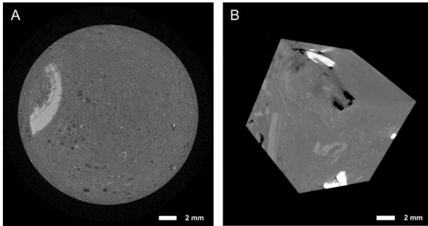
Fig. 3.13 Illustration of beam hardening at the outer margins of the \mu CT scans (A) and star effects due to the presence of dense materials like cold-water coral fragments (B) or small dense grains (A).
