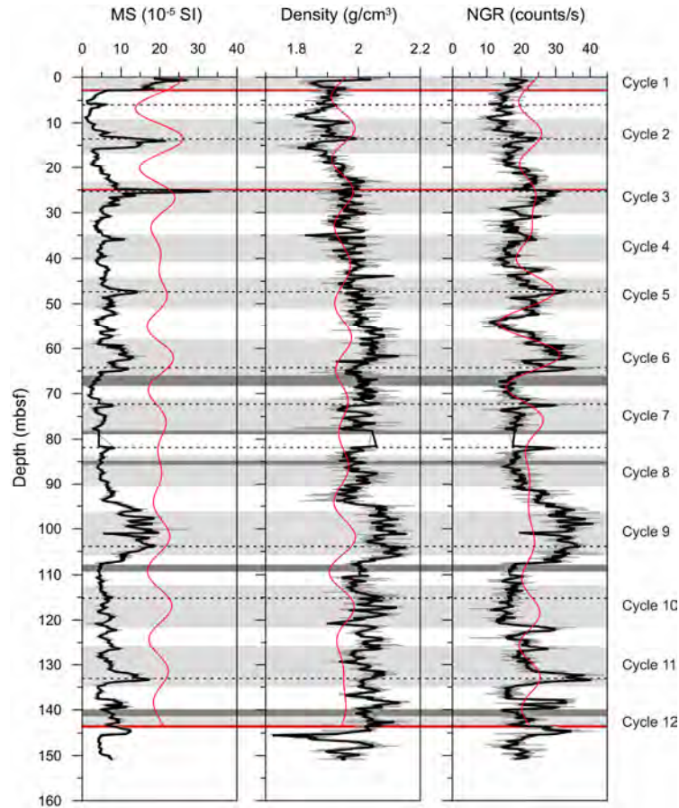
Fig. 4.4 Geophysical properties (magnetic susceptibility (SI units), density ( \text{g}/\text{cm}^3 ), and NGR (counts/s)) in function of depth (mbsf) for Hole U1317B. Grey lines represent raw values. Black lines represent smoothed records (7-points running mean). Red lines represent filtered records (Gaussian filtering centred at a frequency of 0.07 \pm 0.015 ). Grey boxes correspond with interpreted cycles. Dark grey boxes correspond with semi-lithified horizons. Red horizontal lines correspond with interpreted hiatus and the mound base. Black horizontal dashed lines represent correlating tiepoints.
