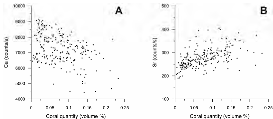
Fig. 4.8 A Ca intensities (counts/s) in function of coral quantity (volume%). B Sr intensities (counts/s) in function of coral quantity (volume%).
