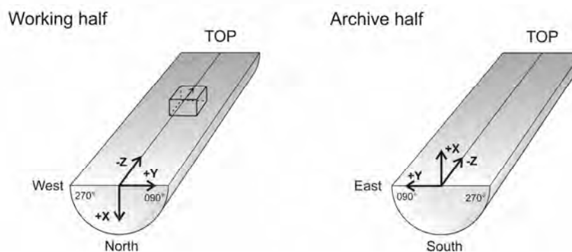
Fig. 5.2 IODP core orientation convention: +X = vertical upward from the split surface of archive halves, +Y = left split surface when looking upcore, and +Z = downcore.
