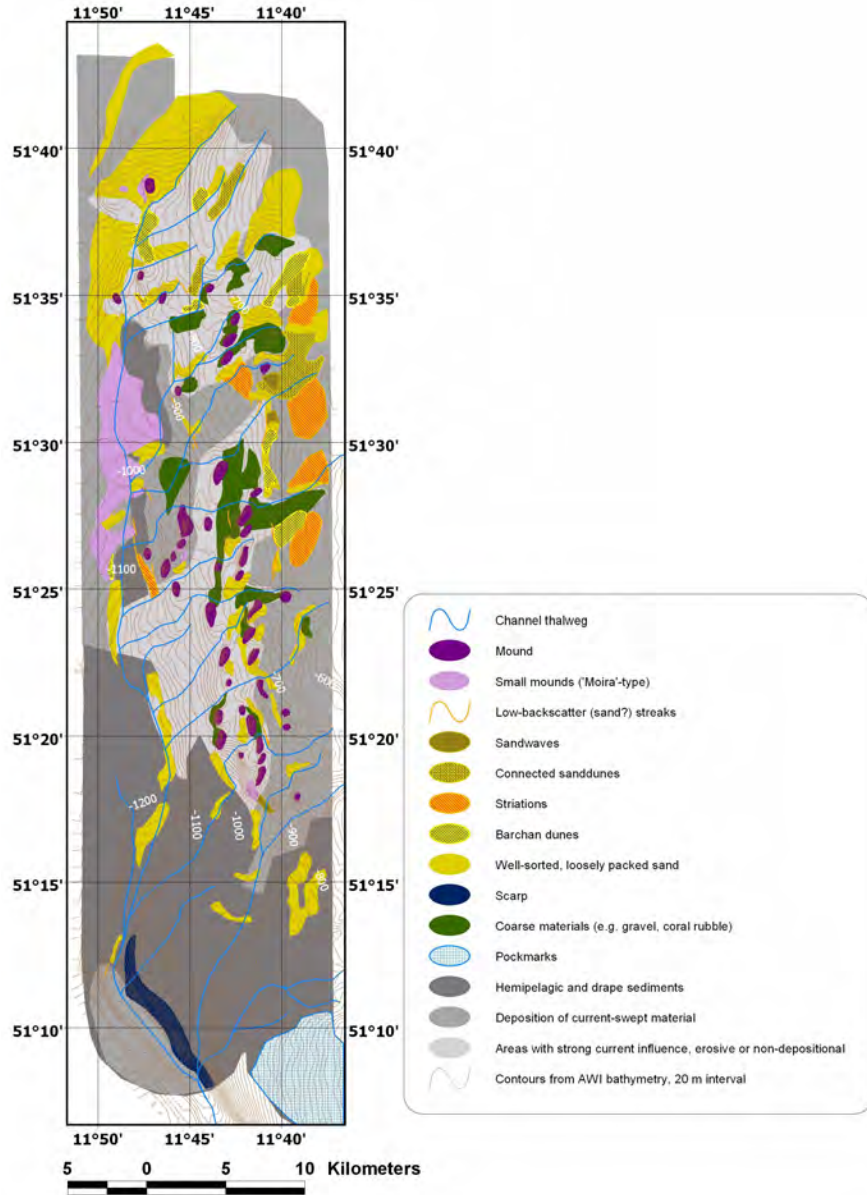
Fig. 2.9 Interpretation of the TOBI sidescan sonar mosaic in the Belgica Mound Province after Huvenne et al. 2005. AWI bathymetry is plotted on the sidescan sonar records (Beyer et al. 2003).
