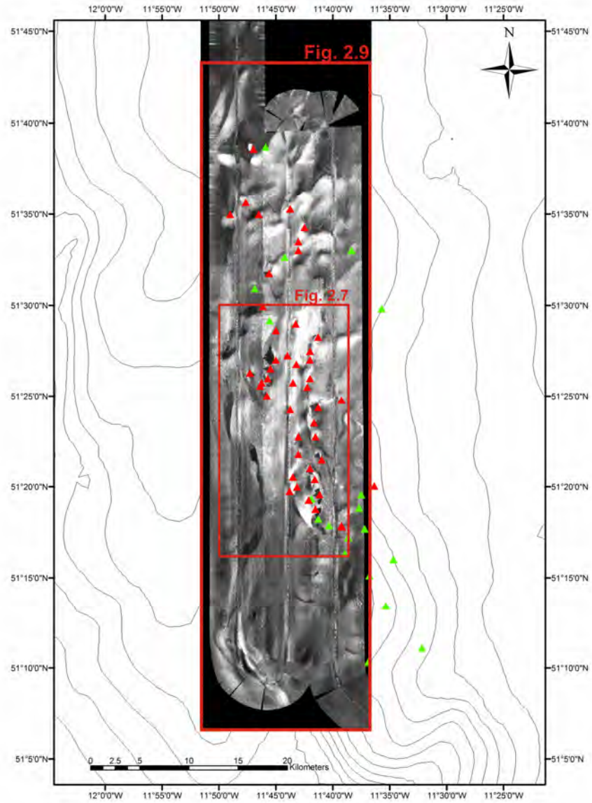
Fig. 2.8 TOBI (Towed Ocean Bottom Instrument) sidescan sonar mosaic (de Haas et al. 2002; Huvenne et al. 2005) of the Belgica Mound Province with annotation of surface mounds (red triangles) and buried mounds (green triangles).
