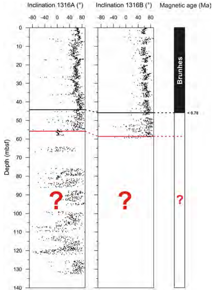
Fig. 5.15 Inclination records at peak fields of 15 mT and interpreted magnetostratigraphic framework in Holes U1316A and U1316B. Black horizontal line represents the interpreted Brunhes Chron. Red horizontal line represents the mound base. Below this base magnetostratigraphic interpretation became impossible (no stable magnetization; Fig 5.14D).
