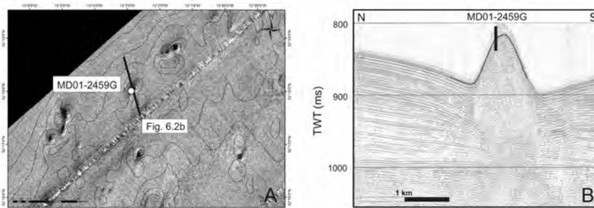
Fig. 6.2 Localization of core MD01-2459G (Magellan Mound Province). A TOBI sidescan sonar imagery of Mound Perseverance and his surroundings (de Haas et al. 2002) and GSI multibeam bathymetry. Contour interval is set at 10 m. B NNW-SSE orientated RCMG sparker profile with localization of core site.
