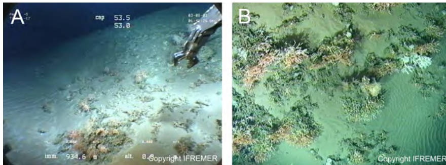
Fig. 7.4 ROV imagery visualizing the Moira Mounds. A Slope of one of the Moira Mounds with patches of live coral framework (mainly the species Madrepora oculata ) and dead coral fragments on the flank. B Rippled sand patches in between coral thickets on the flanks of a Moira Mound.
