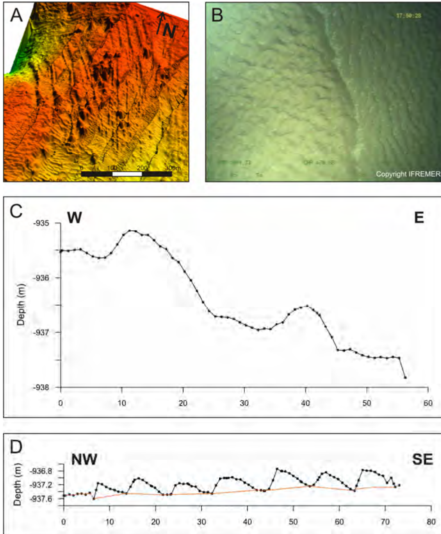
Fig. 7.9 A Zoom in on zone 3 of the micro-bathymetric grid visualizing the furrows and ridges. B ROV video imagery showing the sandwaves with superimposed ripple pattern. C W-E profile through the furrows (for location see Fig. 7.6). D NW-SE profile through the sandwaves within the furrows (for location see Fig. 7.6).
