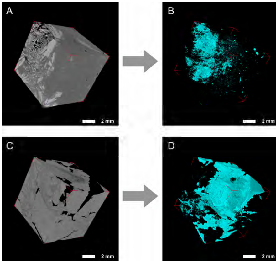
Fig. 3.16 Micro-CT scans representing bioclasts, matrix and porosities (left panels) and porosities (right panels). A-B Sample from Section 307-1317A-8H-3 showing moldic porosity around cold-water coral fragment. C-D Sample from Section 307-1317A-14H-3 visualizing secondary porosity.
