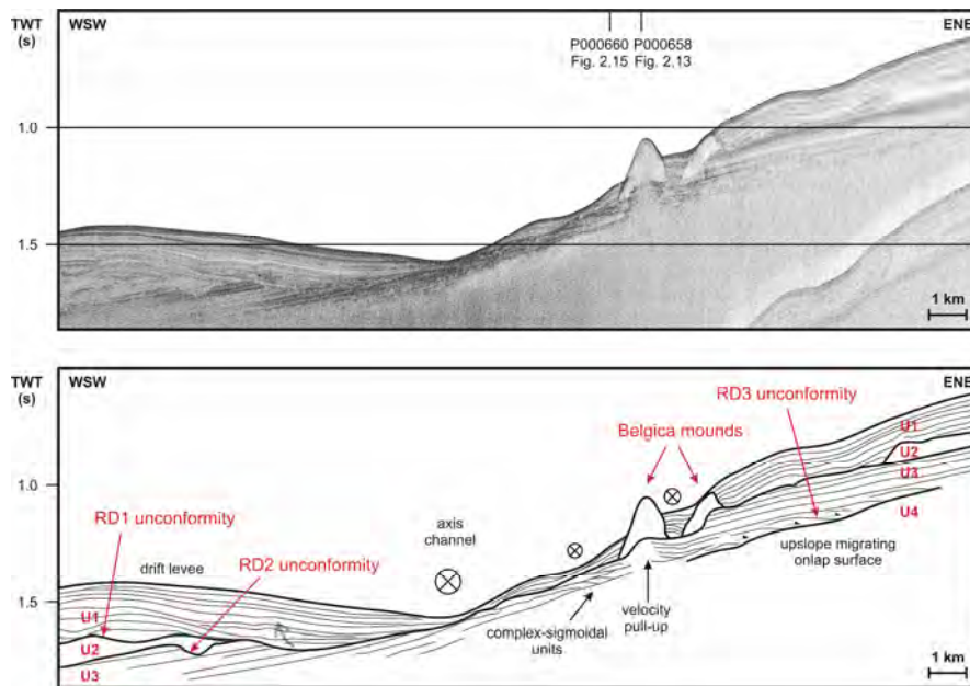
Fig. 2.6 High-resolution WSW-ENE seismic profile P980521, illustrating the general seismostratigraphic setting of the Belgica Mound Province (modified after Van Rooij 2004; Van Rooij et al. 2007a, 2007b). The different described units and unconformities are annotated. The location of the described seismic profile is noted on Figs. 2.1b, 2.12 and 2.16.
