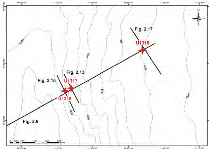
Fig. 2.16 Bathymetric map showing the location of the IODP Holes (on-mound Site U1317 and off-mound Sites U1316 and U1318) (red stars) and the seismic lines visualized on Figs. 2.6, 2.13, 2.15 and 2.17. Contour interval set at 100 m. Map is based on GEBCO bathymetry.
