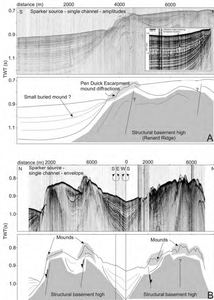
Fig. 8.5 A Sparker seismic profile perpendicular to the PDE, showing the mound diffractions on the escarpment, the structural basement high (location: see Fig. 8.3). The inset represents some small buried mounds occurring in the sediments at the foot of the escarpment. B Set of Sparker seismic profiles over Renard Ridge (location: see Fig. 8.7). The structural basement, two faults and mound structures can be recognized on the profiles.
