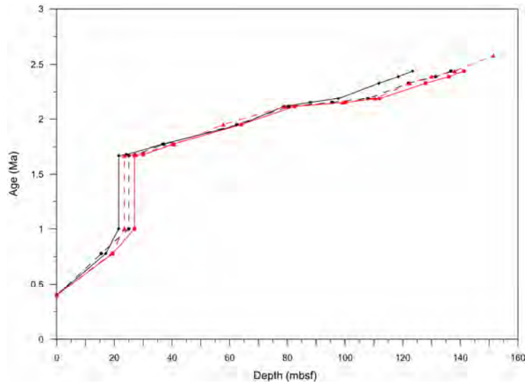
Fig. 5.5 Visualization of the sedimentation rates (age (Ma) in function of depth (mbsf)) of Holes U1317A (black line with diamonds), U1317B (black dashed line with circles), U1317C red line with squares), and U1317E (red dashed line with triangles).
