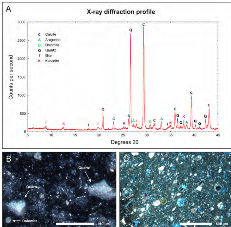
Fig. 3.8 A XRD profile from matrix sediments (Exp. 307 Scientists 2006d). B Smearslide from matrix with dominantly coccoliths and clay-sized grains and minor amounts of quartz and dolomite. C Thin section from mud matrix with forams and silt-sized quartz grains.
