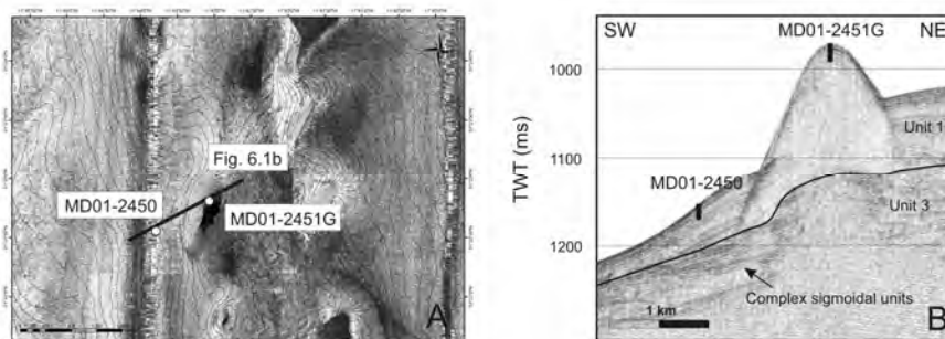
Fig. 6.1 Localization of cores MD01-2450 and MD01-2451G (Belgica Mound Province). A TOBI sidescan sonar imagery of Challenger Mound and his surroundings (de Haas et al., 2002) and detailed multibeam bathymetry (Beyer et al. 2003). Contour interval is set at 10 m. B SW-NE orientated RCMG sparker profile with localization of core sites MD01-2451G and MD01-2450 and seismic-stratigraphic features, as defined by Van Rooij et al. (2003).
