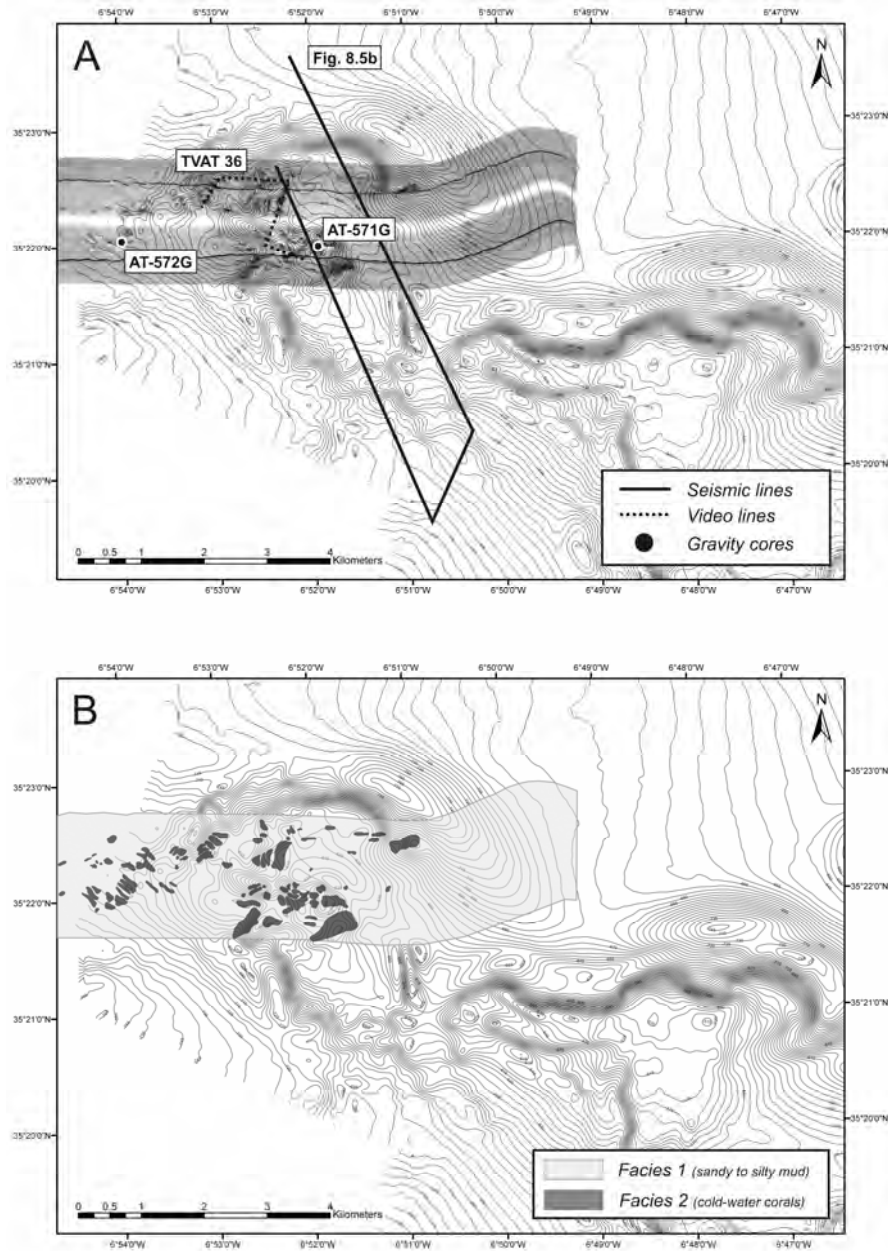
Fig. 8.7 A Bathymetry (contour spacing is 5 m), sidescan sonar imagery and location of the seismic profiles, core material and video line in the Renard Mound Province. B Interpretation of sidescan sonar imagery (MAKAT 75), representing two distinctive facies.
