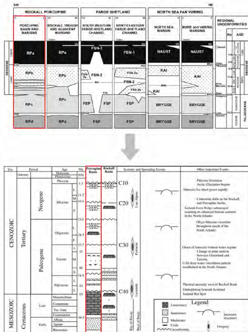
Fig. 2.3 Late Cenozoic tectonostratigraphic evolution of Porcupine Basin, and the NE Atlantic margin. Upper panel: Stratigraphic nomenclature (megasequences and key major and minor unconformities) for the Upper Palaeogene-Neogene strata on the NW European Atlantic margin as defined by the STRATAGEM project (after Stoker et al. 2005). Lower panel: Detailed tectonostratigraphic setting of the Late Mesozoic and Cenozoic of the Porcupine and Rockall region after Shannon 2007 (modified from McDonnell and Shannon 2001).
