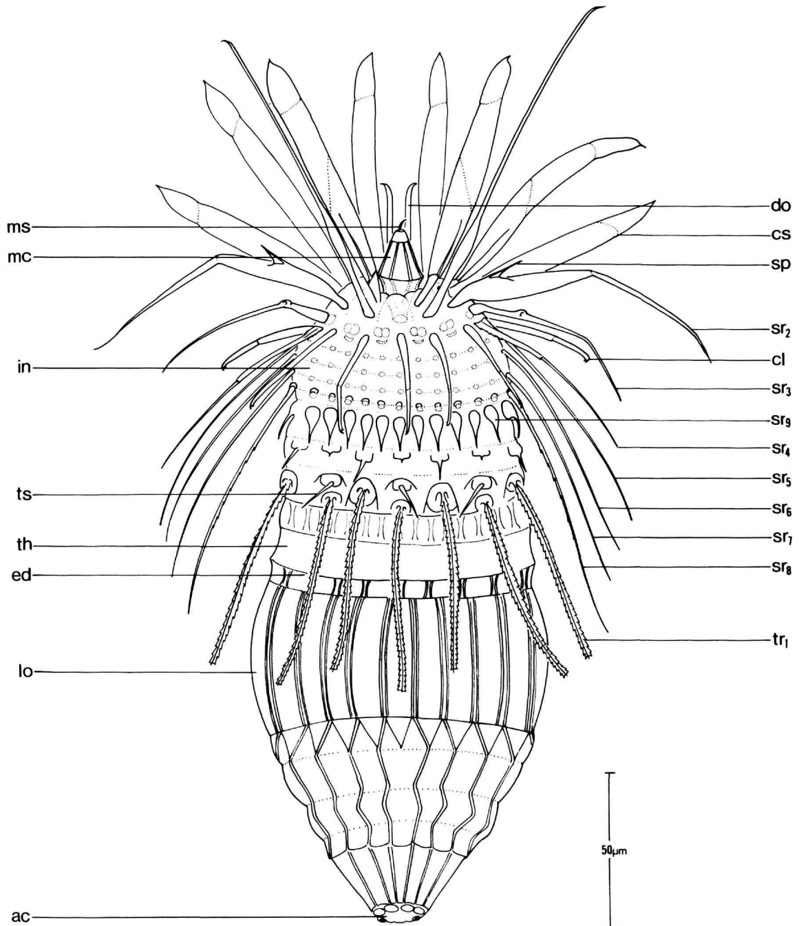
FIGURE 84.— Rugiloricus ornatus , new species, holotypic female, dorsal view (scale in μm).
