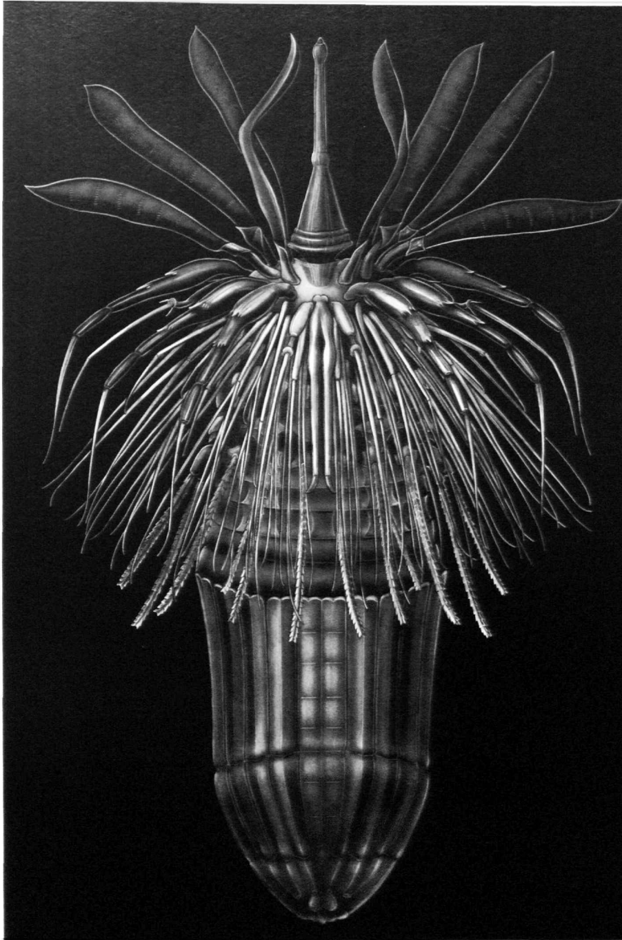
FIGURE 38.— Pliciloricus gracilis , new species, holotypic male(?), ventral view (see Figure 37 for scale).
