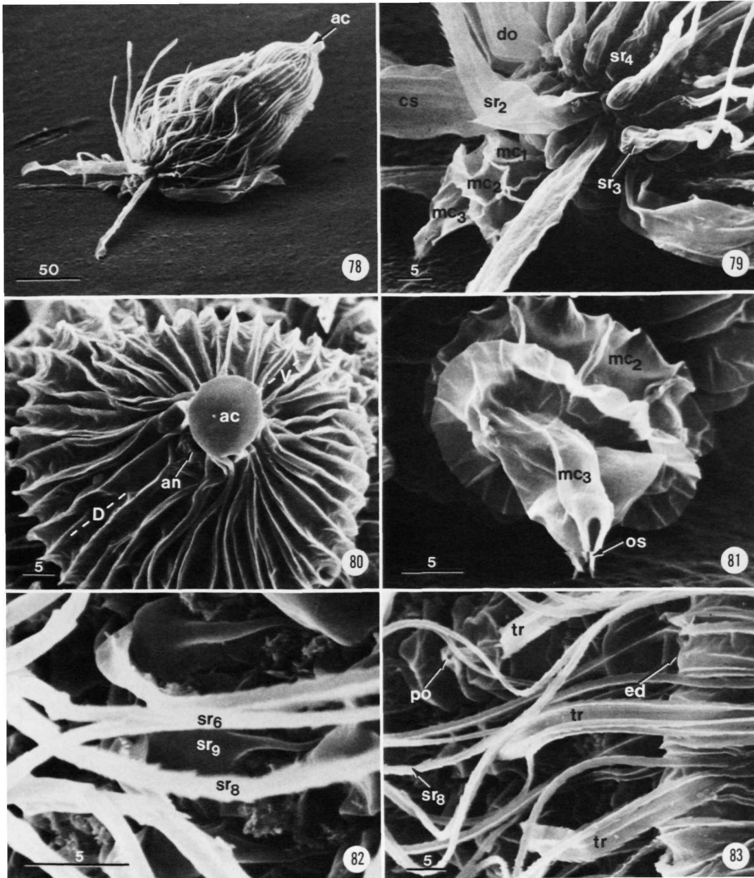
FIGURES 78–83.— Rugiloricus cauliculus , new species, paratypic adult male(?): 78, lateral view; 79, mouth cone and first few scald rows; 80, anal cone, dorsal anus, and lorica, posterior view; 81, mouth cone with oral styles, polar view; 82, last row of spinoscalids; 83, single trichoscalids with the trichoscalid plate and pore. (SEM micrographs, scales in μm.)
