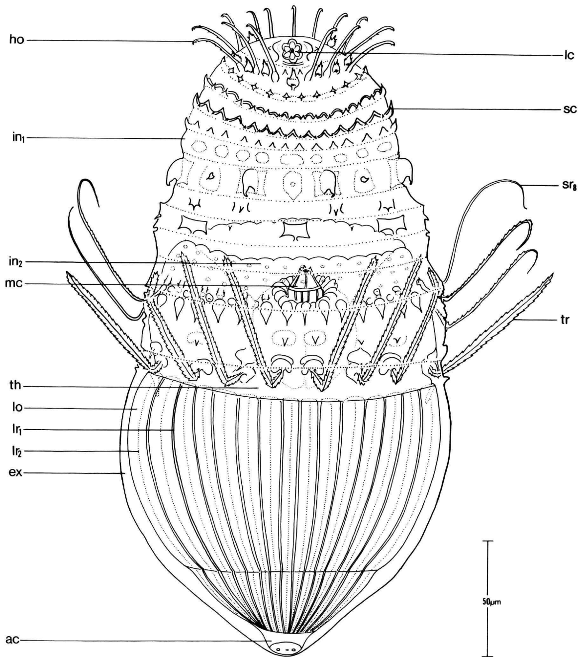
FIGURE 77.— Rugiloricus cauliculus , new species, allotypic adult male(?) in larval (postlarval?) exuvium, ventral view (scale in \mu\text{m} ).
