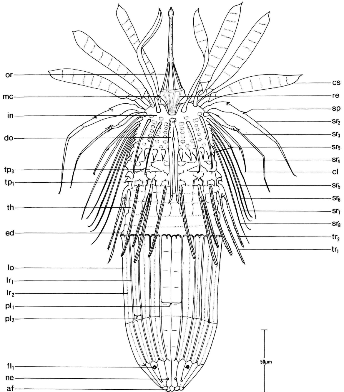
FIGURE 37.— Plicitoricus gracilis , new species, holotypic male(?), ventral view (scales in μm).
