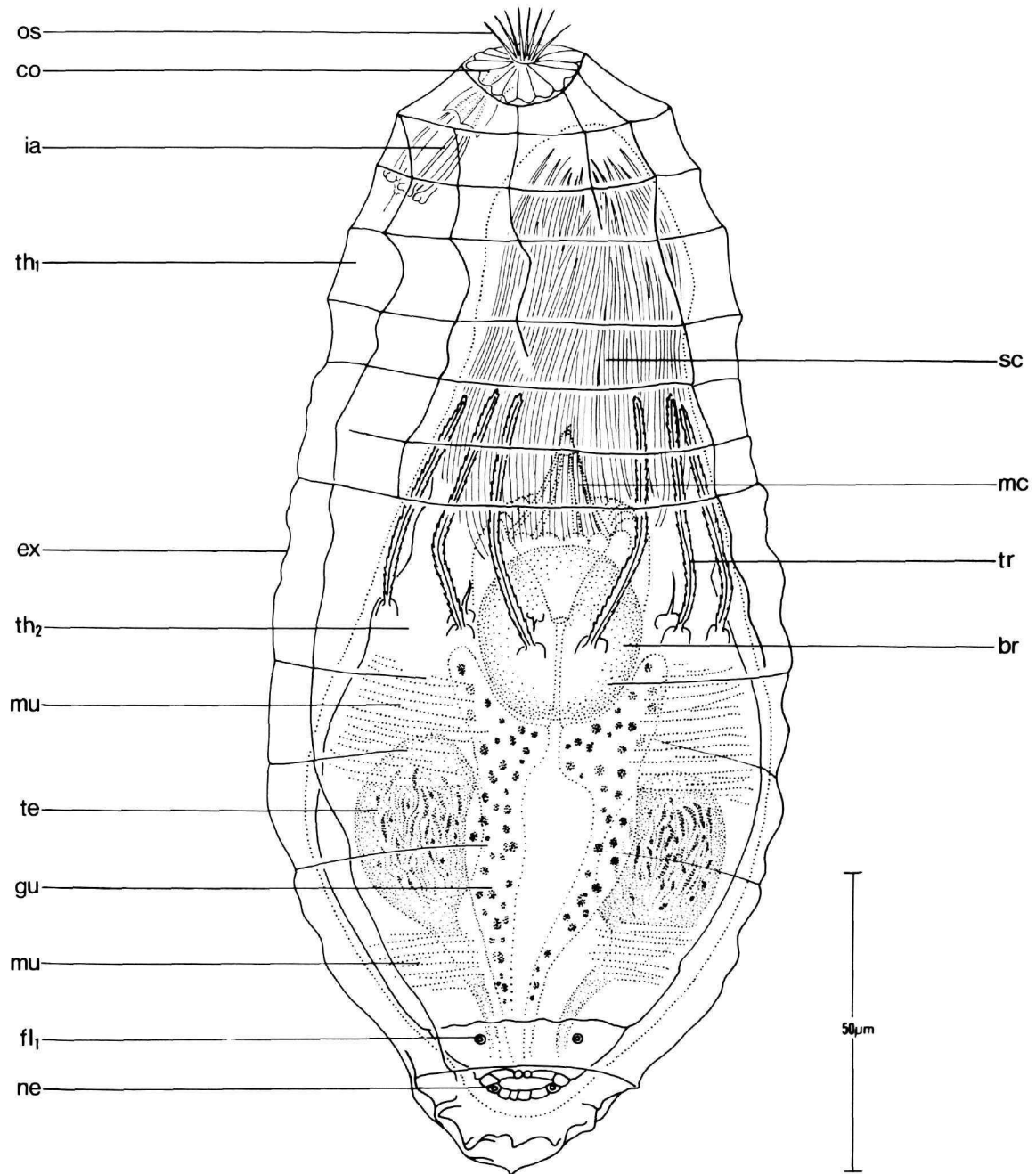
FIGURE 86.— Rugiloricus ornatus , new species, paratypic adult male in larval (postlarva?) exuvium, ventral view (scale in \mu\text{m} ).
