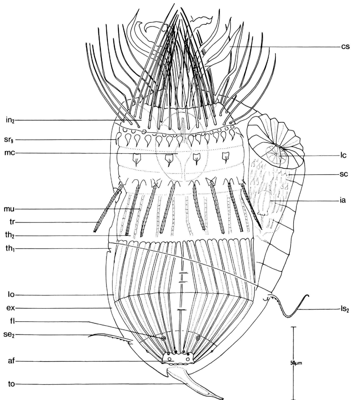
FIGURE 56.— Rugiloricus carolinensis , new species, holotypic adult female(?) in larval exuvium, lateral view of larval exuvium, ventral view of adult (scale in \mu\text{m} ).
