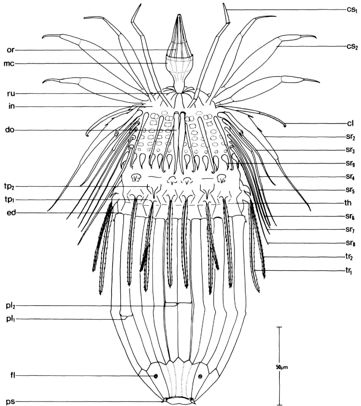
FIGURE 48.— Pliciloricus profundus , new species, holotypic male, ventral view (scale in \mu\text{m} ).
