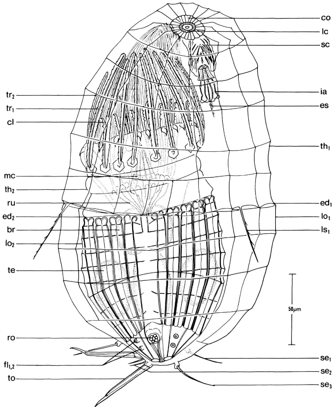
FIGURE 3.— Pliciloricus enigmaticus , new species, paratypic larva molting into an adult male, larval-exuvium in lateral view, adult in ventral view (scale in \mu\text{m} ).
