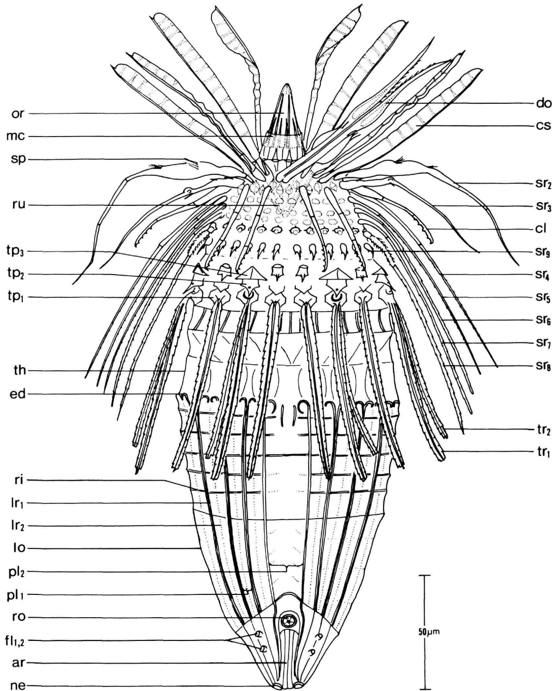
FIGURE 1.— Pliciloricus enigmaticus , new species, holotypic female, ventral view (scale in μm).
