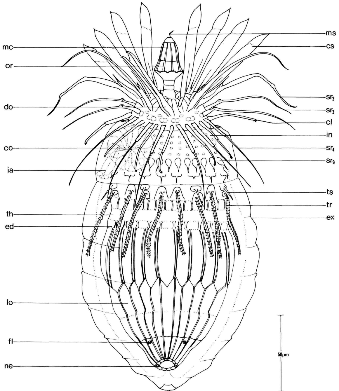
FIGURE 85.— Rugiloricus ornatus , new species, allotype, adult male in larval exuvium, ventral view (scale in μm).
