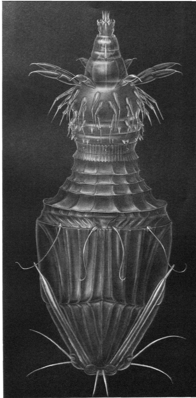
FIGURE 40.— Pliciloricus gracilis , new species, paratype larva, ventral view (see Figure 39 for scale).
