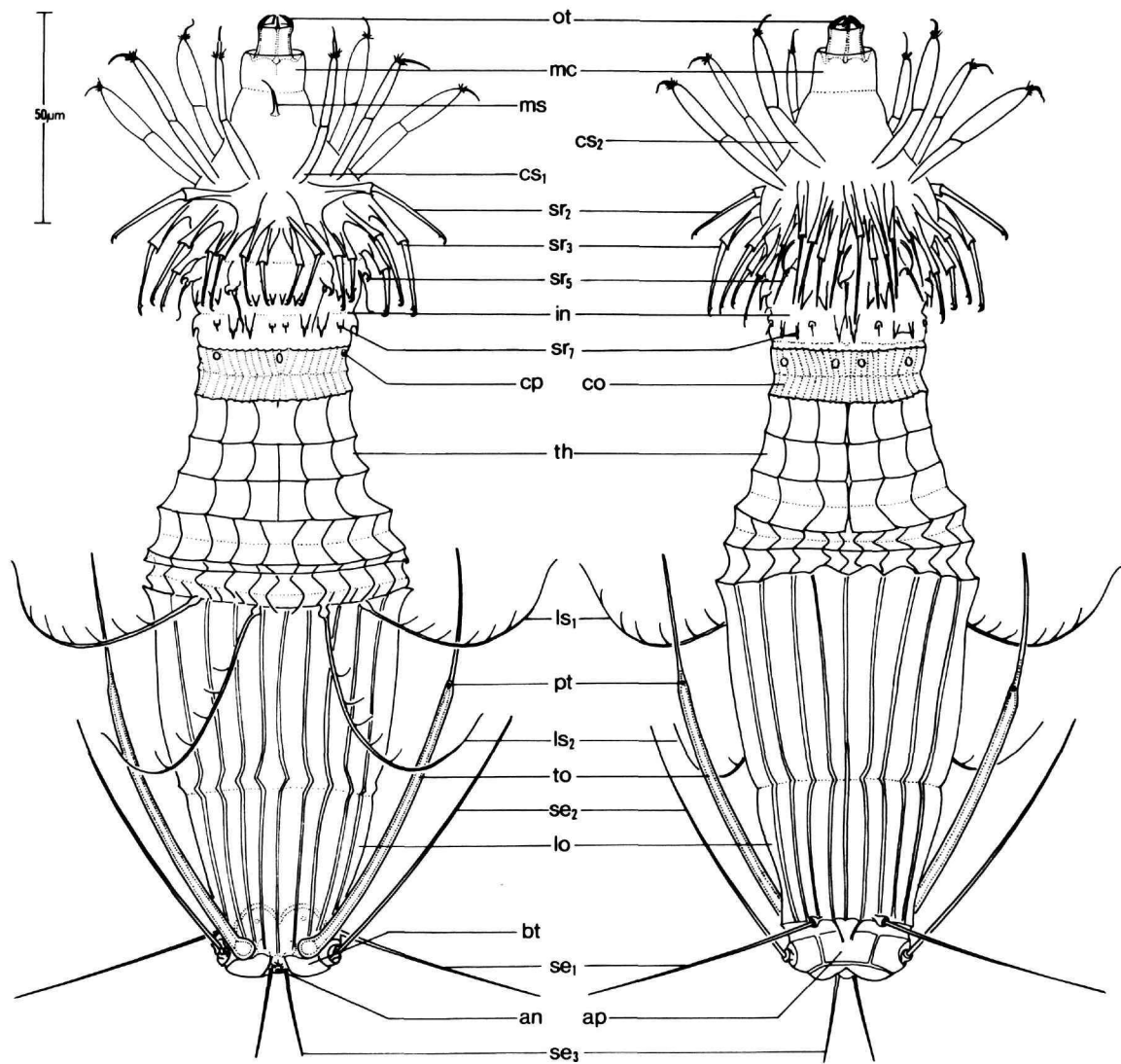
FIGURE 49.— Pliciloricus profundus , new species, paratype larva: left , ventral view; right , dorsal view (scale in \mu\text{m} ).
