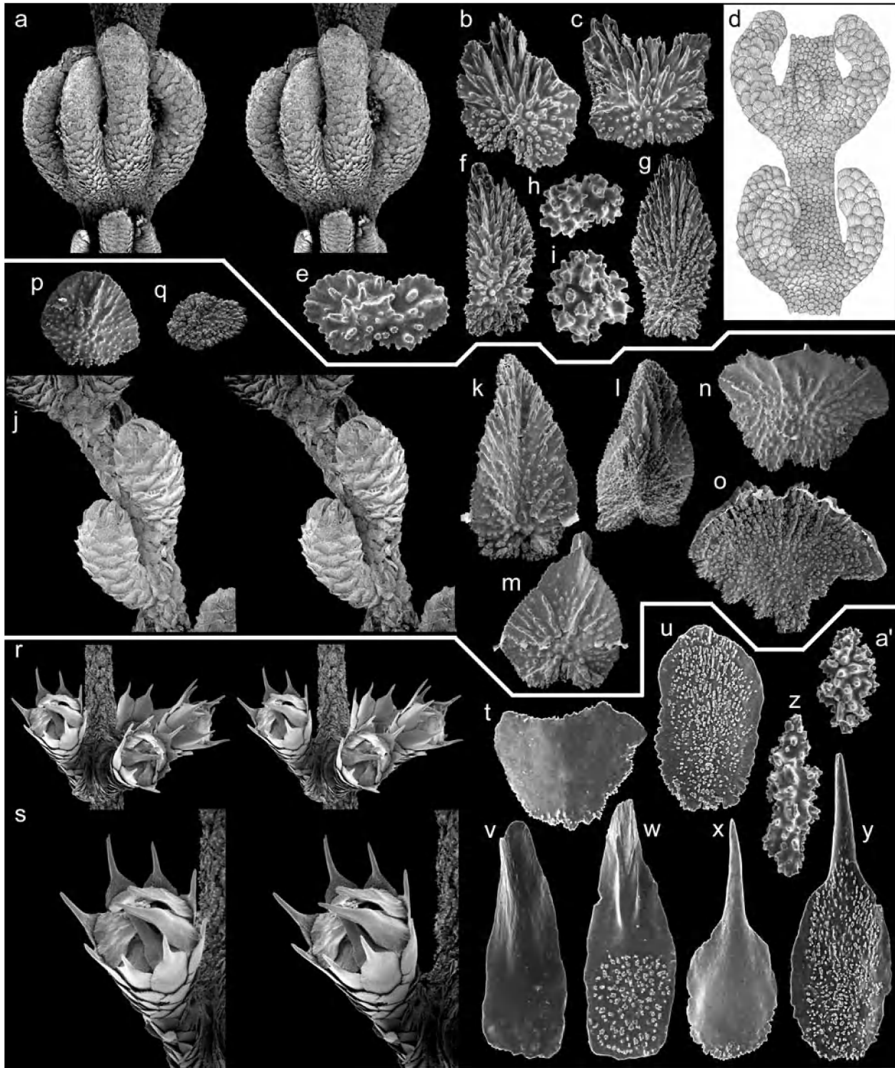
FIGURE 10. Pyrogorgia lempos (a–i, holotype, Eltanin -740, USNM 58392): (a.) stereo view of a whorl of polyps, \times 13 ; (b–c.) outer surface of body wall scales, \times 90 ; (d.) drawing of two whorls and branch, \times 10 ; (e.) outer surface of coenenchymal scale, \times 180 ; (f.) outer and (g.) inner surfaces of opercular scales, \times 90 ; (h–i.) inner coenenchymal tuberculate sclerites, \times 180 . Amphilaphis regularis (j–q, syntype, BM 1889.5.27.60): (j.) stereo view of several calyces, \times 20 ; (k.) outer and (l.) inner surfaces of opercular scales, \times 90 ; (m.) outer surface of marginal scale, \times 90 ; (n.) outer and (o.) inner surfaces of body wall scales, \times 90 ; (p.) outer and (q.) inner surfaces of coenenchymal scales, \times 90 . Miostenella articulata (r–s, Siedlecki -601-29, USNM 84344; t–a', holotype, Eltanin -1536, USNM 79959): (r.) stereo view of a whorl of calyces, \times 18 ; (s.) stereo opercular view of a calyx, \times 36 ; (t.) outer and (u.) inner surfaces of body wall scales, \times 85 ; (v.) outer and (w.) inner surfaces of opercular scales, \times 120 ; (x.) outer and (y.) inner surfaces of marginal scales, \times 73 ; (z–a'.) outer surface of coarsely granular coenenchymal sclerites, \times 85 .
