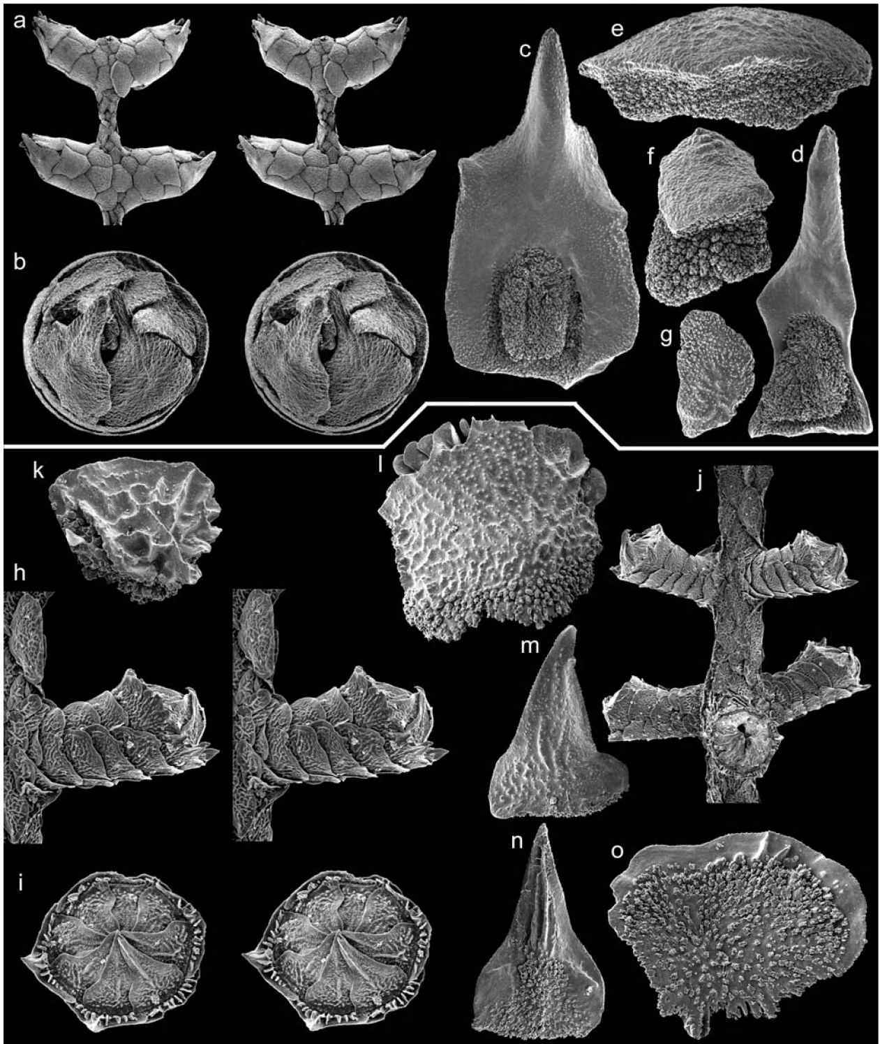
FIGURE 17. Microprimnoa diabathra (a–g, paratype, MUSORSTOM 5-306, USNM 79977): (a.) stereo view of two pairs of calyces, \times 10 ; (b.) stereo opercular view, \times 35 ; (c–d.) inner surface of opercular scales showing discrete patch of tubercles, \times 70 ; (e–f.) lateral view of two thick body wall sclerites, \times 70 ; (g.) outer surface of a coenenchymal scale, \times 70 . Pterostenella plumatilis (h–o, Albatross-5414, USNM 76964): (h.) stereo lateral view of a calyx, \times 52 ; (i.) stereo view of operculum and marginals of a calyx, \times 60 ; (j.) two whorls of calyces, \times 25 ; (k.) outer surface of a coenenchymal scale, \times 190 ; (l.) outer view of a marginal scale, \times 130 ; (m.) outer and (n.) inner surface of opercular scales, \times 130 ; (o.) inner surface of a body wall scale, \times 165 .
