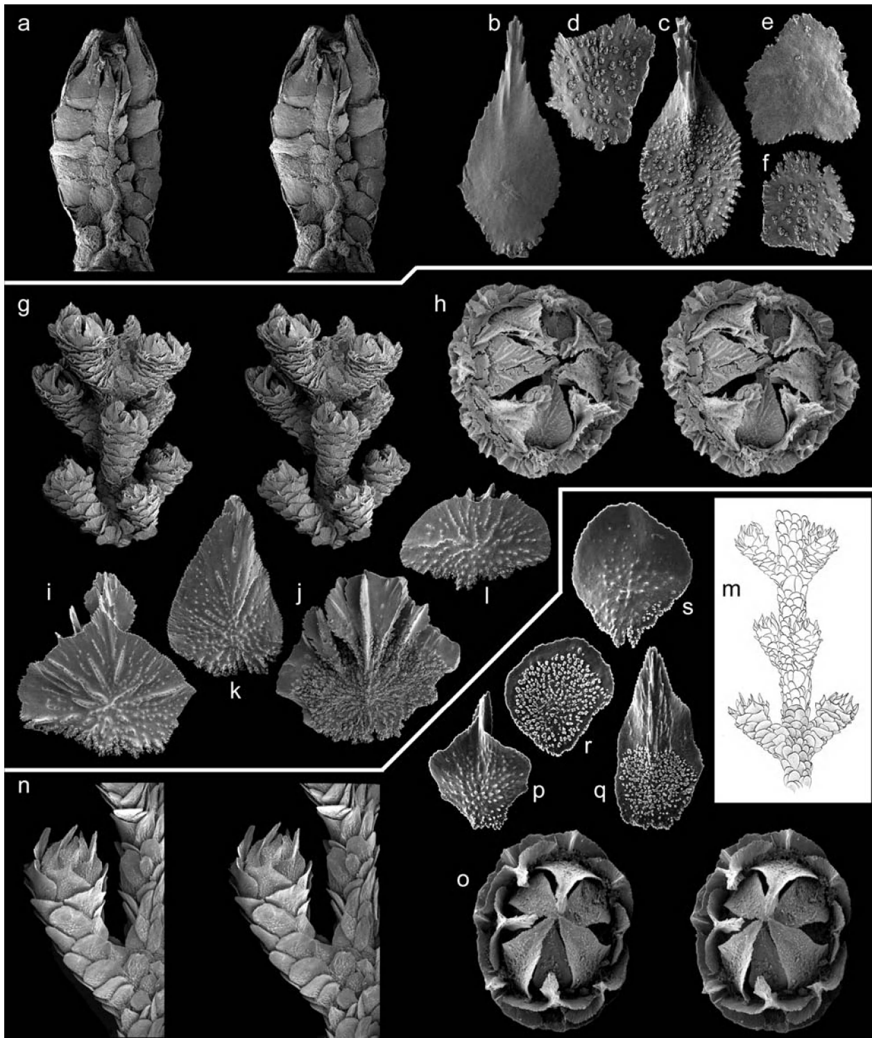
FIGURE 6. Arntzia gracilis (a–f, Islas Orcadas -109, USNM 78666): (a.) stereo view of adaxial side of a calyx, \times 33 ; (b.) outer and (c.) inner surfaces of opercular scales, \times 90 ; (d–f.) outer and inner surfaces of body wall scales, \times 90 . Thouarella ( T. ) antarctica (g–l, Hero 715-873, USNM 97966): (g.) stereo view of clustered calyces, \times 9 ; (h.) stereo opercular view showing eight opercular and eight marginal scales, \times 29 ; (i.) outer and (j.) inner surfaces of marginal scales showing ornate ridging on inner surface, \times 53 ; (k.) outer surface of an opercular scale, \times 53 ; (l.) outer surface of a body wall scale, \times 53 . Thouarella ( Euthouarella ) hilgendorfi (m, Challenger -192, BM 89.5.27.40; n–s, Siboga -251): (m.) partially stippled drawing of a branch fragment, \times 13 ; (n.) stereo lateral view of a calyx, \times 33 ; (o.) stereo opercular view, \times 44 ; (p.) outer surface of a marginal scale, \times 80 ; (q.) inner surface of an opercular scale, \times 120 ; (r.) inner and (s.) outer surfaces of body wall scales, \times 120 .
