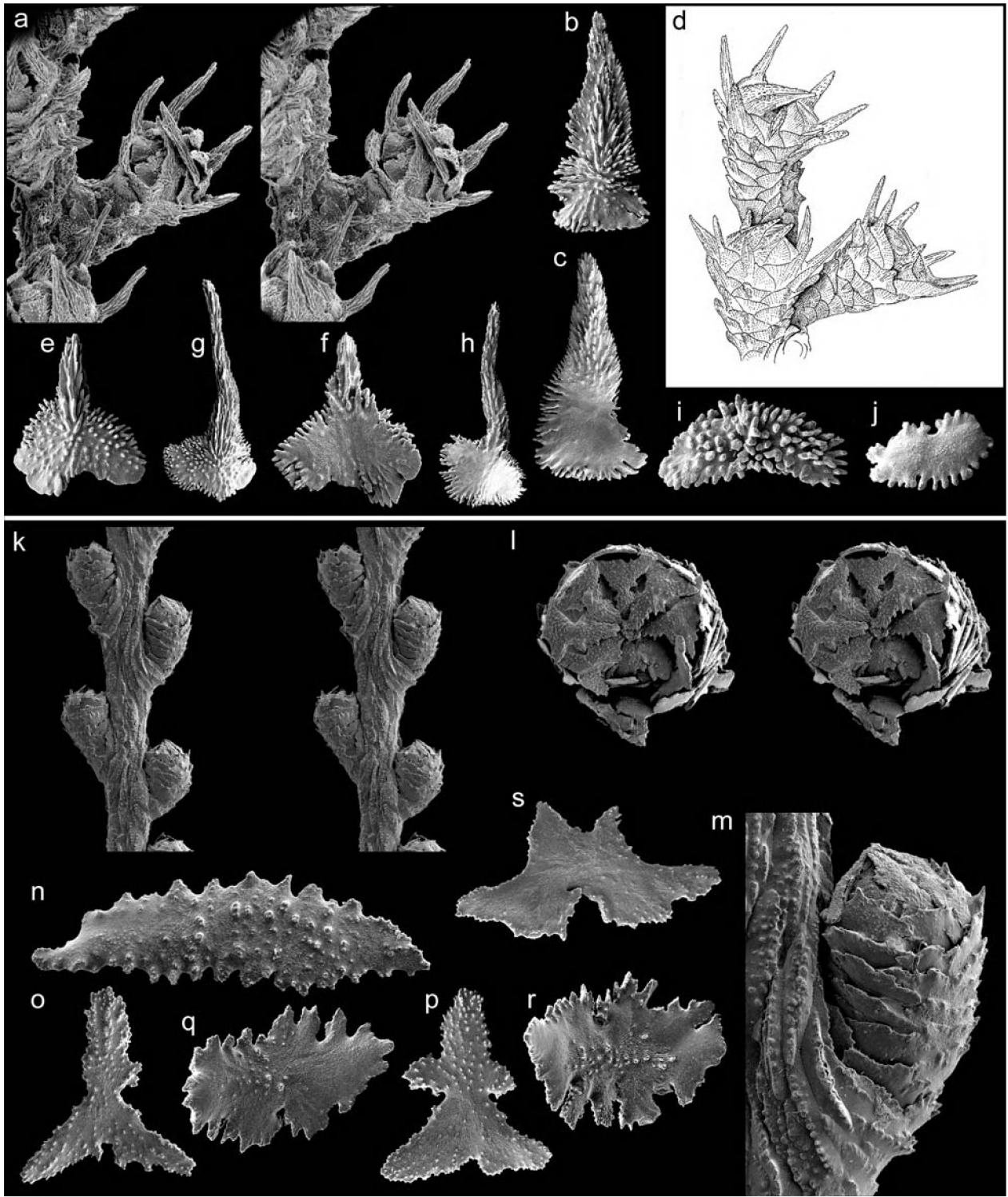
FIGURE 11. Acanthoprinnia goesi (a–c, e–j, Gerda -633, USNM 52973; d, Gerda -242, USNM 52968): (a.) stereo view of apical end of a calyx, \times 34 ; (b.) outer and (c.) inner surfaces of opercular scales, \times 85 ; (d.) drawing of three calyces, \times 28 ; (e.) outer and (f.) inner surfaces of body wall scales, \times 85 ; (g.) outer and (h.) inner surfaces of marginal scales, \times 55 ; (i.) outer (j.) and inner surfaces of coenenchymal scales, \times 125 . Plumarella penna (k–s, Darwin Harbor, USNM 1107503): (k.) stereo view of alternating calyces, \times 37 ; (l.) stereo opercular view, \times 120 ; (m.) lateral view of calyx, \times 150 ; (n.) outer surface of a coenenchymal scale, \times 325 ; (o–p.) outer surface of opercular scales, \times 350 ; (q–r.) inner surface of body wall scales, \times 235 ; (s.) outer surface of a marginal scale, \times 325 .
