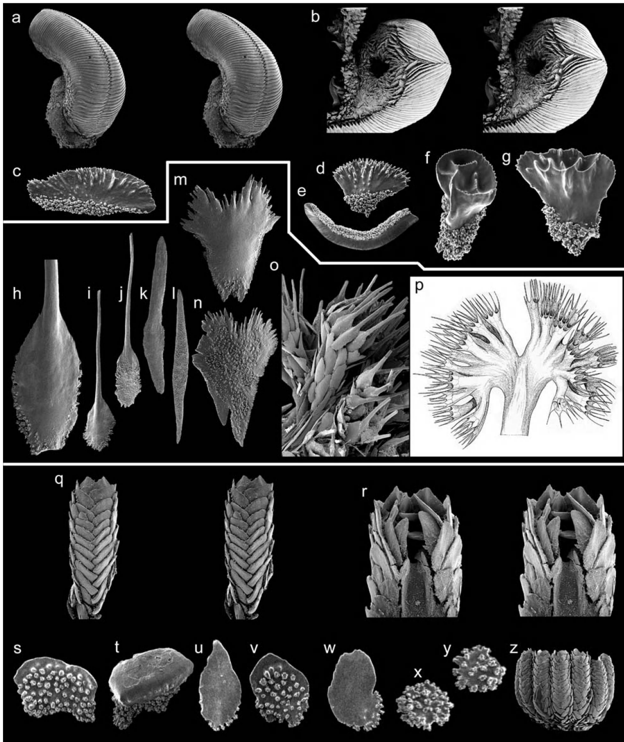
FIGURE 4. Armadilloorgia cyathella (a, Eltanin -1536, USNM 79591; b–g, holotype, USNM 58166): (a.) stereo pair of abaxial side of a calyx, \times 7.5 ; (b.) stereo view of oral region of a calyx, \times 15 ; (c–d.) circummoral (adaxial) sclerites, \times 20 , \times 40 , respectively; (e.) an abaxial sclerite, \times 14 ; (f–g.) coenenchymal sclerites, \times 105 . Ainigmaptilon edisto (h–o, Islas Orchadas -123, USNM 77140; p, holotype, USNM 49580): (h.) base of an opercular scale, \times 77 ; (i.) outer and (j.) inner surfaces of opercular scales, \times 30 ; (k.) outer and (l.) inner surfaces of coenenchymal scales, \times 40 ; (m.) outer and (n.) inner surfaces of body wall scales; (o.) a cluster of calyces, \times 1.7 ; (p.) drawing of a polyp leaf (from Bayer, 1950), \times 7.5 . Primnoella australasiae (q–z, syntype, BM 1983.3.2.13): (q.) abaxial side of a calyx, \times 37 ; (r.) adaxial side of a calyx showing bare strip, \times 71 ; (s.) inner and (t.) outer surfaces of body wall scales, \times 95 ; (u.) circummoral scale, \times 95 ; (v.) inner and (w.) outer surface of outer coenenchymal sclerites, \times 95 ; (x–y.) inner coenenchymal spheroids on canal walls, \times 125 ; (z.) whorl of calyces, \times 13 .
