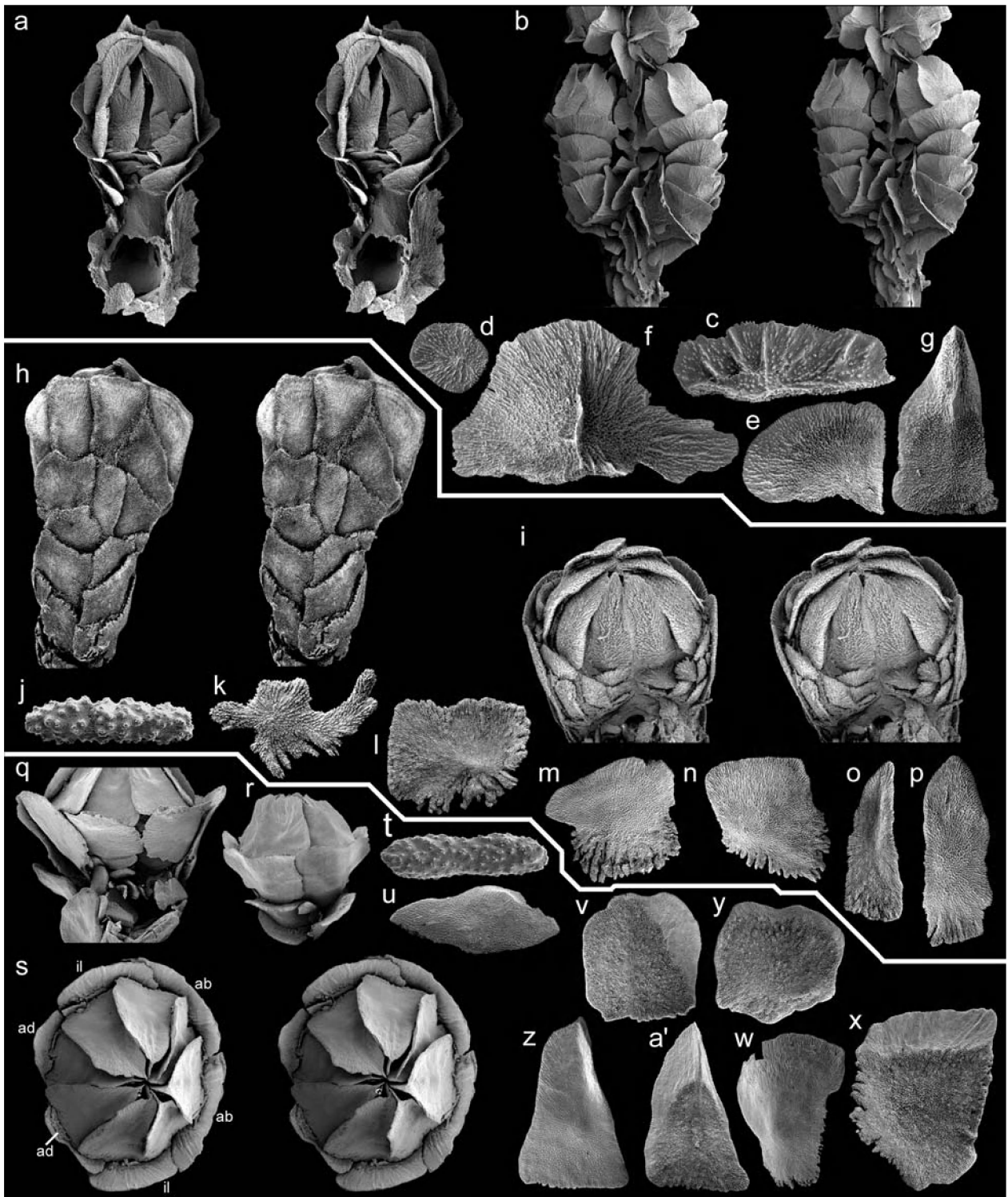
FIGURE 13. Paranarella watlingi (a–g, holotype, RB05-03, USNM 1096721): (a.) stereo view of adaxial side of a calyx, \times 21 ; (b.) stereo view of two calyces, \times 11 ; (c.) ridged coenenchymal scale, \times 62 ; (d.) outer surface of an adaxial body wall scale, \times 30 ; (e.) inner surface of an abaxial body wall scale, \times 30 ; (f.) outer surface of a basal scale, \times 30 ; (g.) inner surface of an opercular scale, \times 30 . Primnoa resedaeformis (h–i, Albatross-2068 , USNM 16946; j–p, Albatross-2527 , USNM 12262): (h.) stereo view of abaxial side of a calyx, \times 11 ; (i.) stereo opercular view of adaxial side of a calyx, \times 17 ; (j.) a tentacular rod, \times 165 ; (k.) outer surface of a coenenchymal scale, \times 28 ; (l.) outer surface of a basal scale, \times 14 ; (m.) outer surface of a marginal scale, \times 14 ; (n.) outer surface of an abaxial body wall scale, \times 14 ; (o.) inner and (p.) outer surfaces of opercular scales, \times 17 . Australogorgia aldersladei (q–a', holotype, NTM CO 13054): (q.) adaxial side of a calyx, \times 9 ; (r.) abaxial side of a calyx, \times 7 ; (s.) stereo view of operculum (marginal scales labeled: ab, abaxial; il, inner lateral; ad, adaxial), \times 11 ; (t.) tentacular rod, \times 135 ; (u.) outer surface of a coenenchymal scale, \times 15 ; (v.) adaxial, (w.) abaxial, and (x.) inner lateral marginal scales, \times 15 , \times 12 , \times 15 , respectively; (y.) abaxial body wall scale, \times 15 ; (z.) outer and (a'.) inner surfaces of opercular scales, \times 15 .
