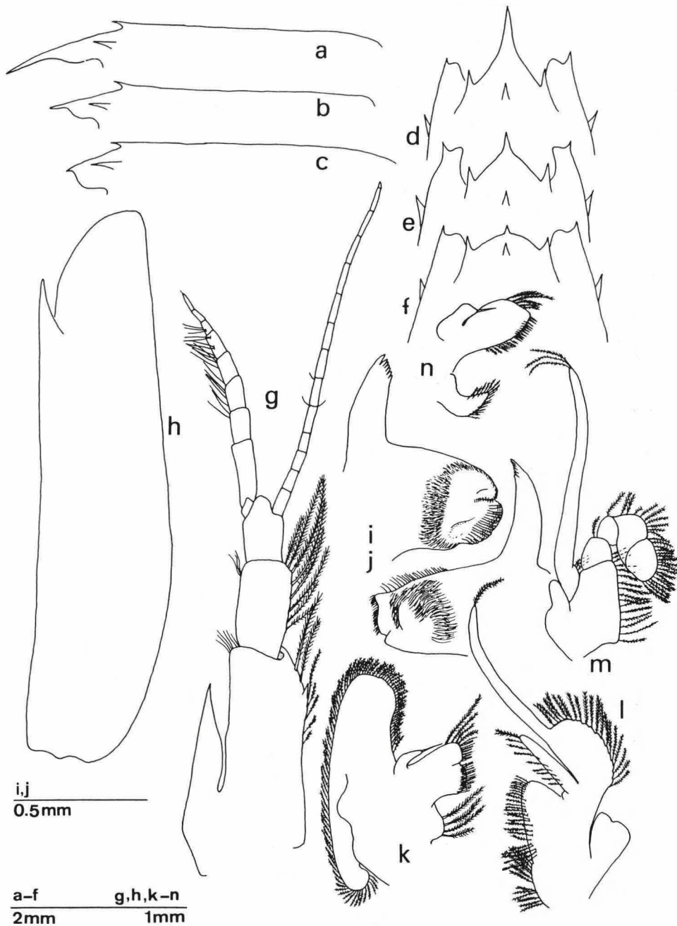
Fig. 41. Hippolyte sapphica d'Udekem d'Acoz forma B, NW Greece, Agia Triada [St. E8] (RMNH), mature females. a-c, rostrum and dorsal part of carapace; d-f, anterior part of carapace of the same specimens; g, left antennula; h, left scaphocerite; i, right Md; j, left Md; k, right Mxp2; l, left Mxp1; m, right Mx2; n, right Mx1.
