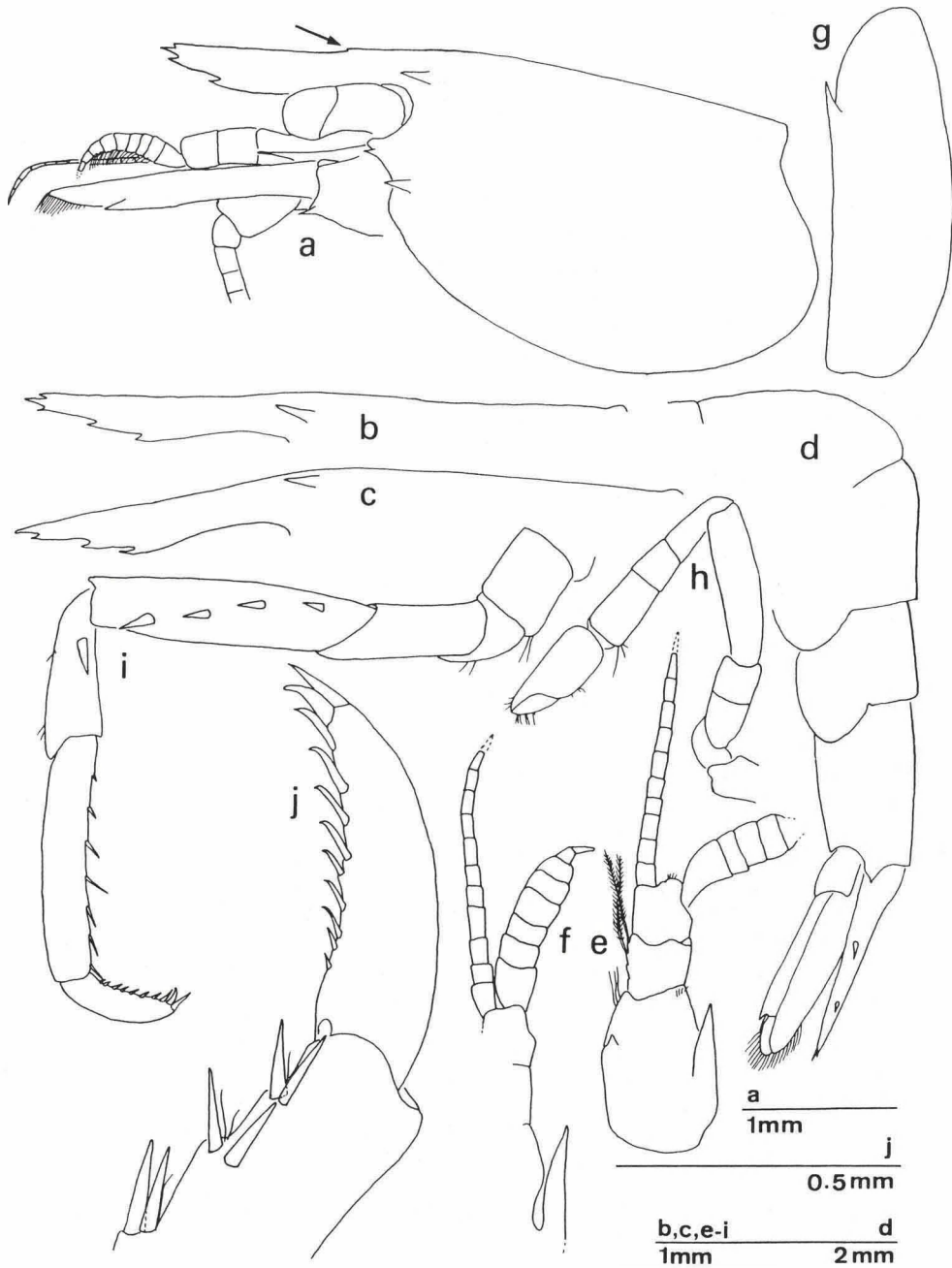
Fig. 16. Hippolyte lagarderei d'Udekem d'Acoz, Morocco, Témara; a-i, paratypes (a-d, f, h-i: females; e, g: males) (IRScNB, I G. 27 945); j, female holotype (MNHN, Na 12 127). a, cephalothorax [in some specimens the dorsal proximal tooth is larger]; b-c, rostra and dorsal part of carapace; d, posterior part of pleon; e-f, right antennula, g, left scaphocerite, h, left P2, i, left P3; dactylus of left P3.
