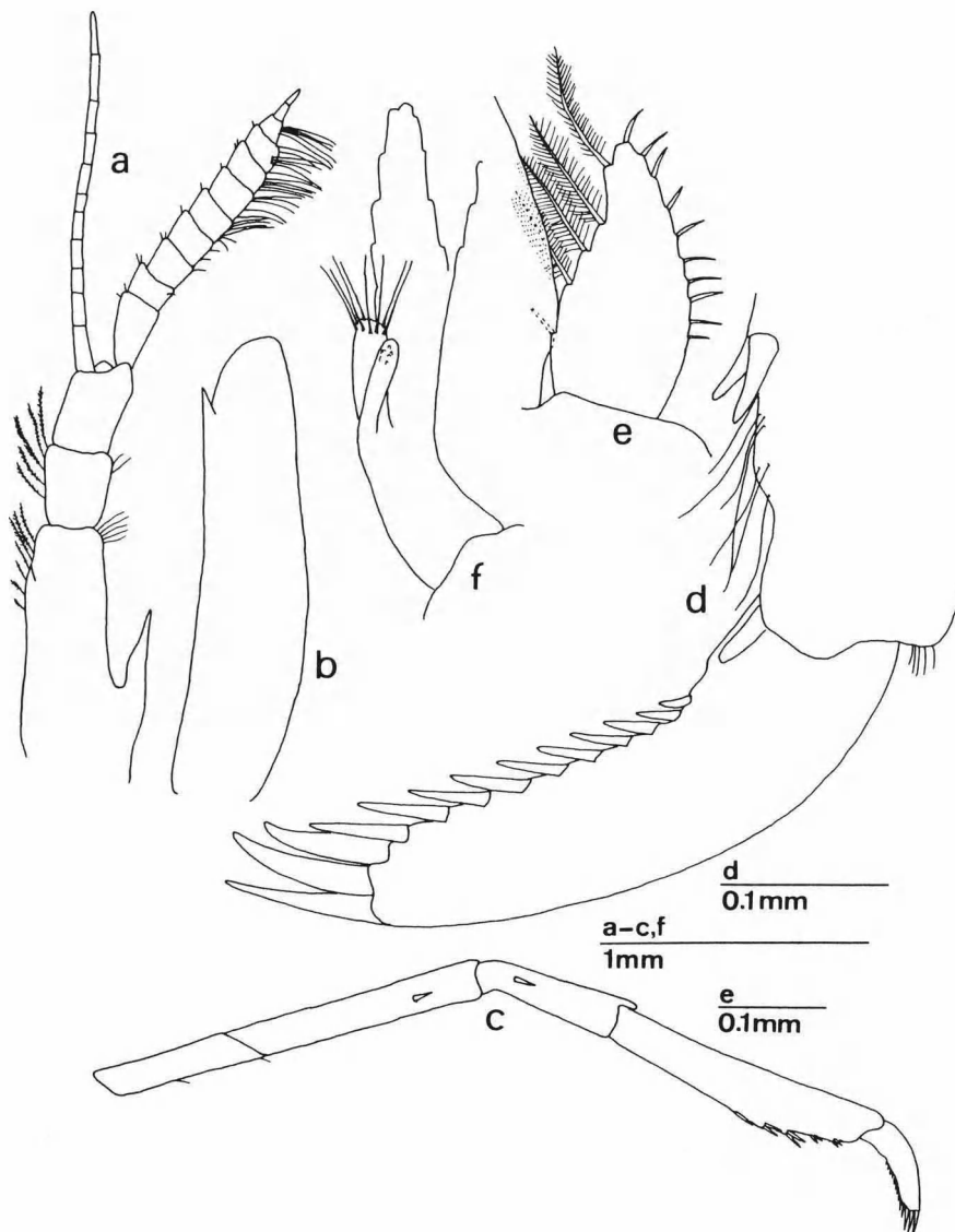
Fig. 43. Hippolyte sapphica d'Udekem d'Acoz forma B, NW Greece, Agia Triada [St. E8] (RMNH), male. a, right antennula; b, left scaphocerite; c, right third pereiopod; d, dactylus of right third pereiopod; e, endopodite of right first pleopod; f, endopodite of right second pereiopod.
