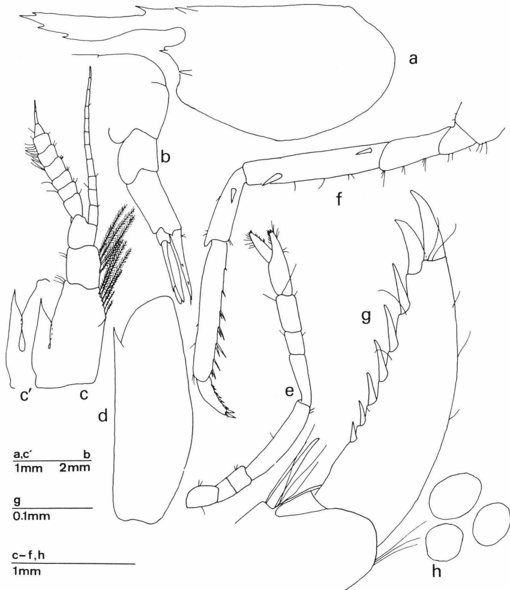
Fig. 44. Hippolyte varians Leach, mature females, Belgium, Zeebrugge, Eastern jetty (c', h, different specimen than other figures) (RMNH). a, carapace; b, posterior part of pleon; c, left antenna; c', left stylocerite; d, left scaphocerite; e, left P2; f, left P3; g, dactylus of left P3; h, eggs with embryos.
