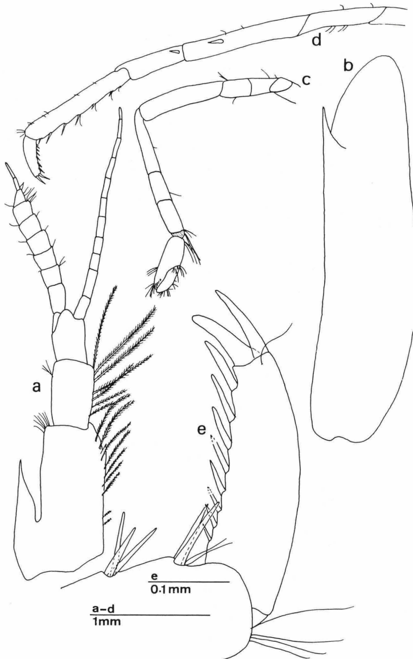
Fig. 39. Hippolyte sapphica d'Udekem d'Acoz forma A, Greece, NW of Koronissia [St. E9] (RMNH), mature female. a, left antennula; b, left scaphocerite; c, left P2; d, left P3; e, dactylus of left P3.
