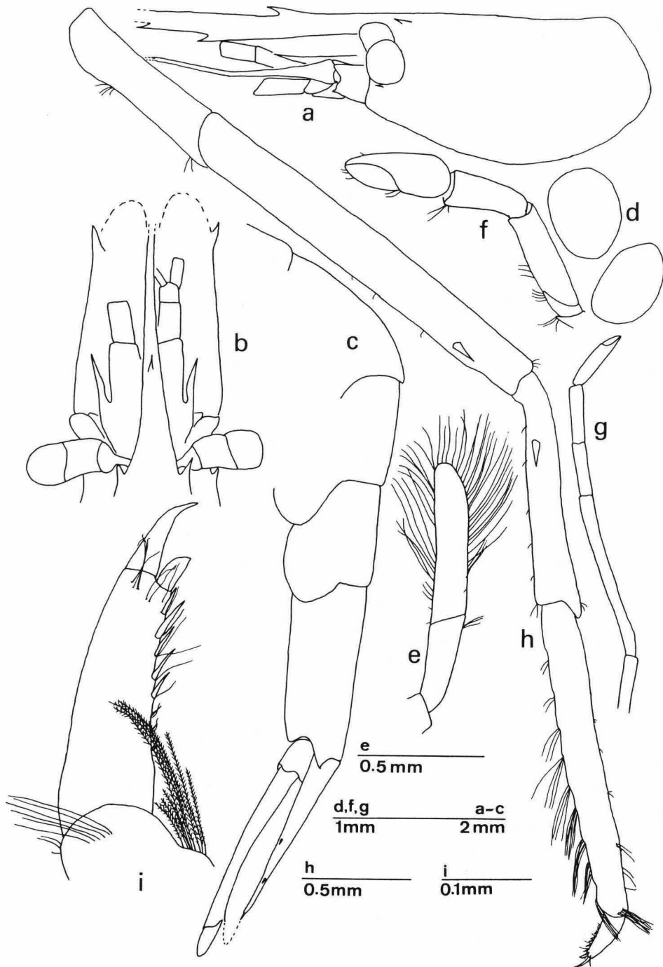
Fig. 24. Hippolyte leptometrae Ledoyer, mature female, Banyuls (MNHN Na 4960); a, cephalothorax; b, anterior part of cephalothorax in dorsal view; c, posterior part of pleon; d, eggs with embryos; e, tip of right MxP3; f, left P1; g, left P2; h, right P3; i, dactylus of left P3.
