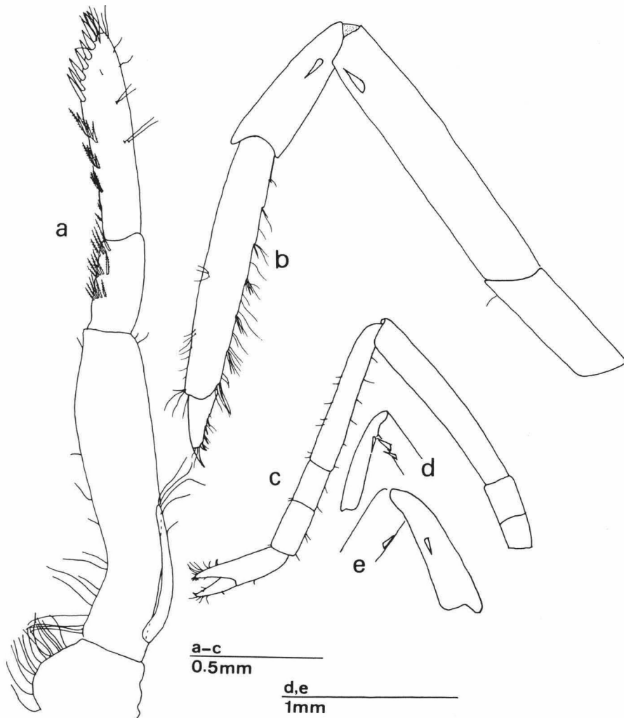
Fig. 37. Hippolyte prideauxiana Leach, females. a, Greece, fishermen of Monemvassia (RMNH); b-c, Cerbère (MNHN Na 14 653); d, Naples (RMNH D 22955); e, Málaga (sketch provided by J E García-Raso). a, left Mxp3; b, left P3; c, left P3; d, tip of merus and carpus of left P3; e, tip of merus and carpus of right P5.
