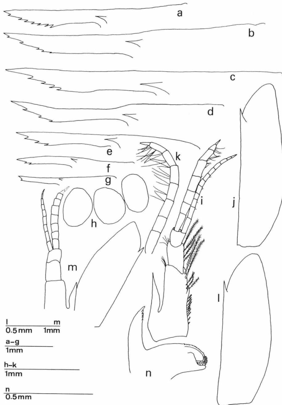
Fig. 35. Hippolyte prideauxiana Leach, females (that of fig. g is immature); a, g, Ibiza (a: SMF 22107; g: SMF 22108); b, fishermen of Lygia (RMNH); c, k, Naples (RMNH D 22955); d, h-j, n, fishermen of Monemvassia (RMNH); e, Cadaqués (RMNH D 34289); f, l, Cerbère (MNHN Na 14 653); m, Málaga (sketch provided by J E García-Raso). a-g, rostrum and dorsal part of carapace; h, eggs with embryos; i, left antennula; j-l, left scaphocerite; k, outer flagellum of left antennula; m, right antennula and scaphocerite; n, right Md.
