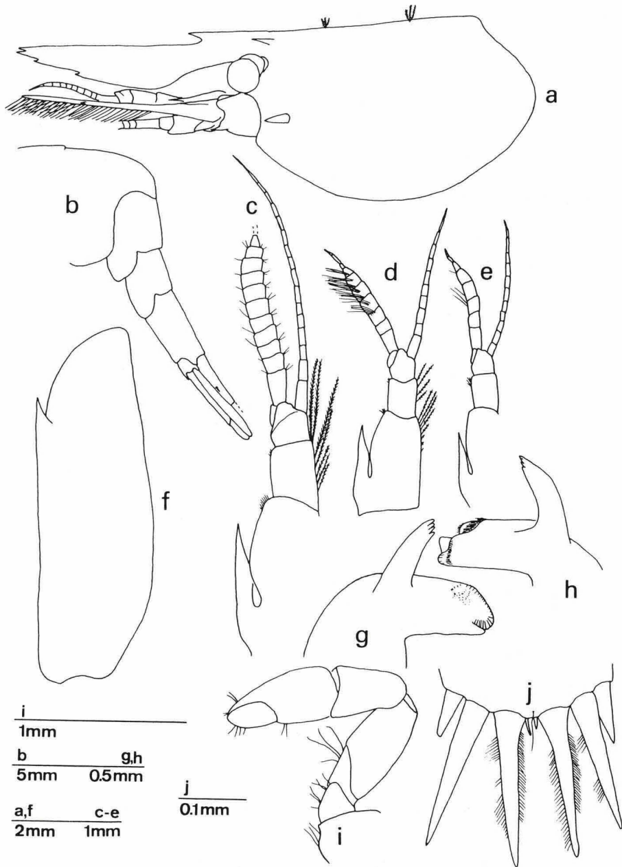
Fig. 45. Hippolyte varians Leach, Madeira, Bay of Machico (RMNH). a-c, large ovigerous female. d-j, smaller non ovigerous females. a, cephalothorax; b, posterior part of pleon; c-e, left antennula; f, left scaphocerite; g, right mandible; h, left mandible; i, left P1; j, apex of telson.
