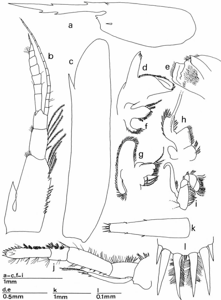
Fig. 26. Hippolyte niezabitoskii spec. nov., mature female paratype, NW Greece, Drepanos [St. E1] (RMNH). a, carapace; b, left antennula; c, left scaphocerite; d, right Md; e, left Md; f, right Mx1; g, right Mx2; h, right Mxp1; i, right Mxp2; j, right Mxp3; k, telson; l, tip of telson.
