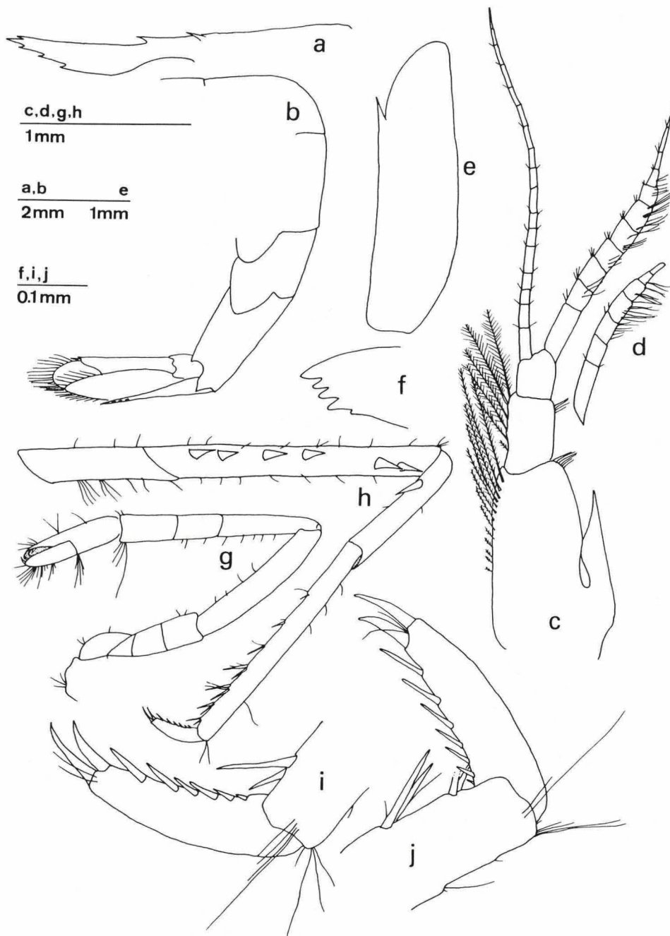
Fig. 47. Hippolyte varians Leach, females, Madeira, Caniço de Baixo, 12 ix 1994 (RMNH). a, rostrum and dorsal part of carapace; b, posterior part of pleon [abnormal telson: 3 pairs of dorsolateral spines]; c, right antenna; d, outer flagellum of right antennula of another specimen; e, left scaphocerite; f, tip of incisor process of left Md; g, left P2; h, right P3; i, dactylus of the same; j, dactylus of left P3 of another specimen.
