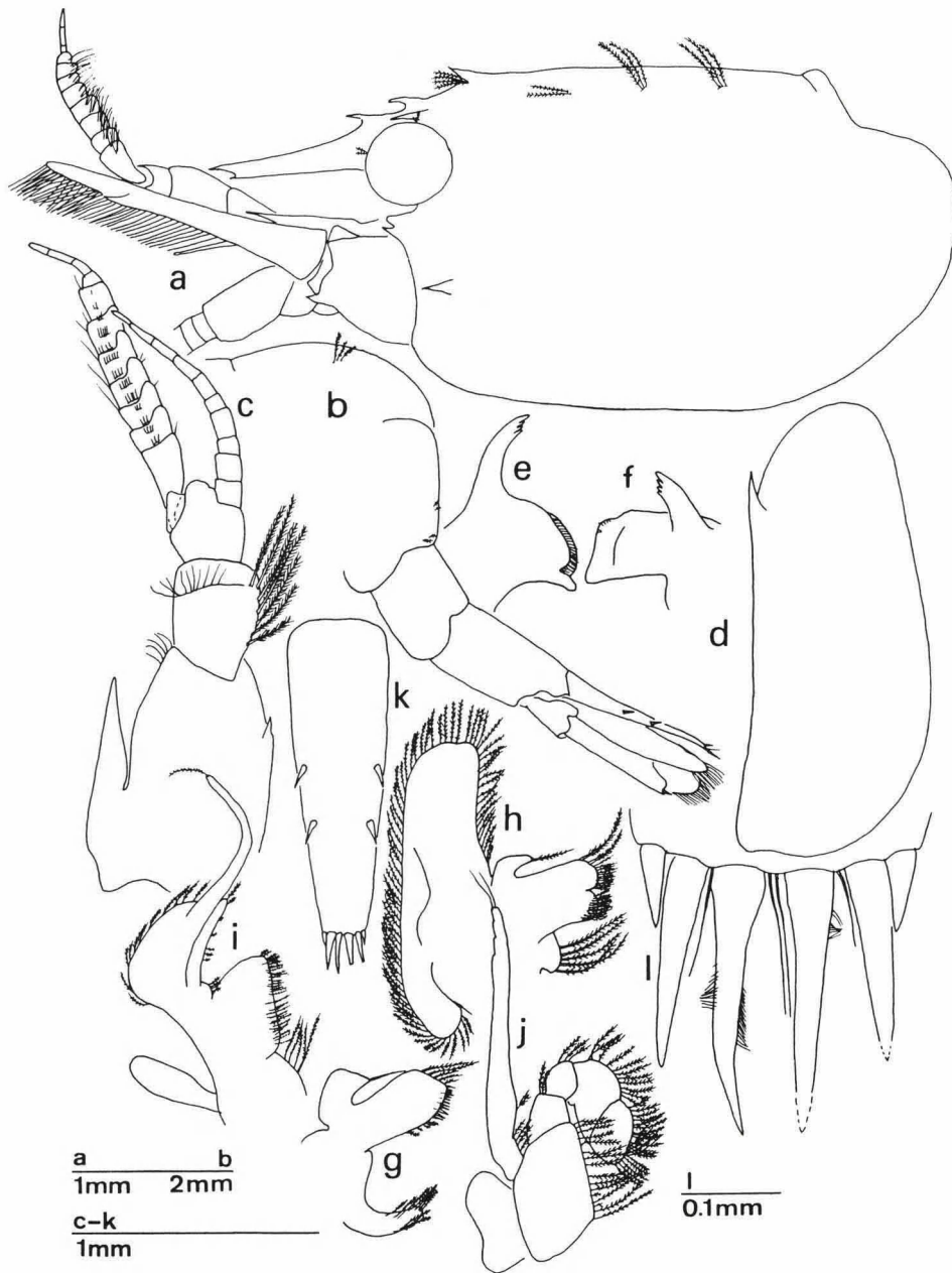
Fig. 19. Hippolyte leptocerus (Heller), mature female, Portugal, Algarve, Carveiro (RMNH). a, cephalothorax; b, posterior part of pleon; c, left antennula; d, left scaphocerite; e, right Md; f, left Md; g, right Mx1; h, right Mx2; i, right Mxp1; j, right Mxp2; k, telson; l, tip of telson.
