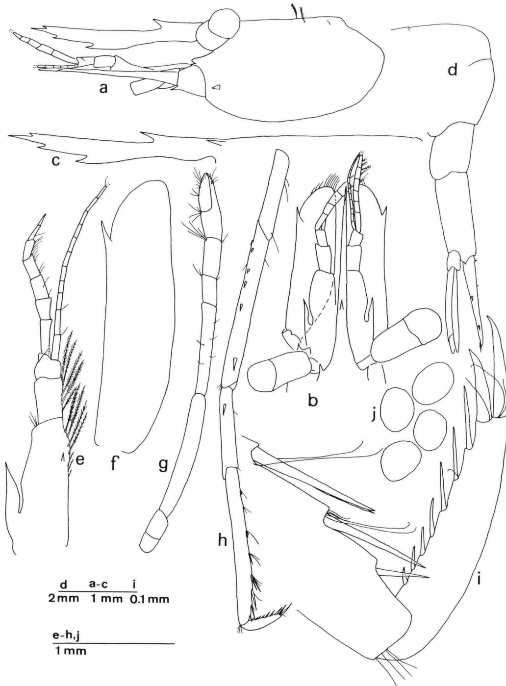
Fig. 49. Hippolyte varians Leach, a-b, female, Croatia, Rovinj [specimen with unusually long rostrum] (SMF previously 5129); c-j, female, NW Greece, Lygia (RMNH). a, cephalothorax; b, anterior part of cephalothorax in dorsal view; c, rostrum and dorsal part of carapace; d, posterior part of pleon; e, left antennula; f, left scaphocerite; g, left P2; h, left P3; i, dactylus of left P3; j, eggs recently laid.
