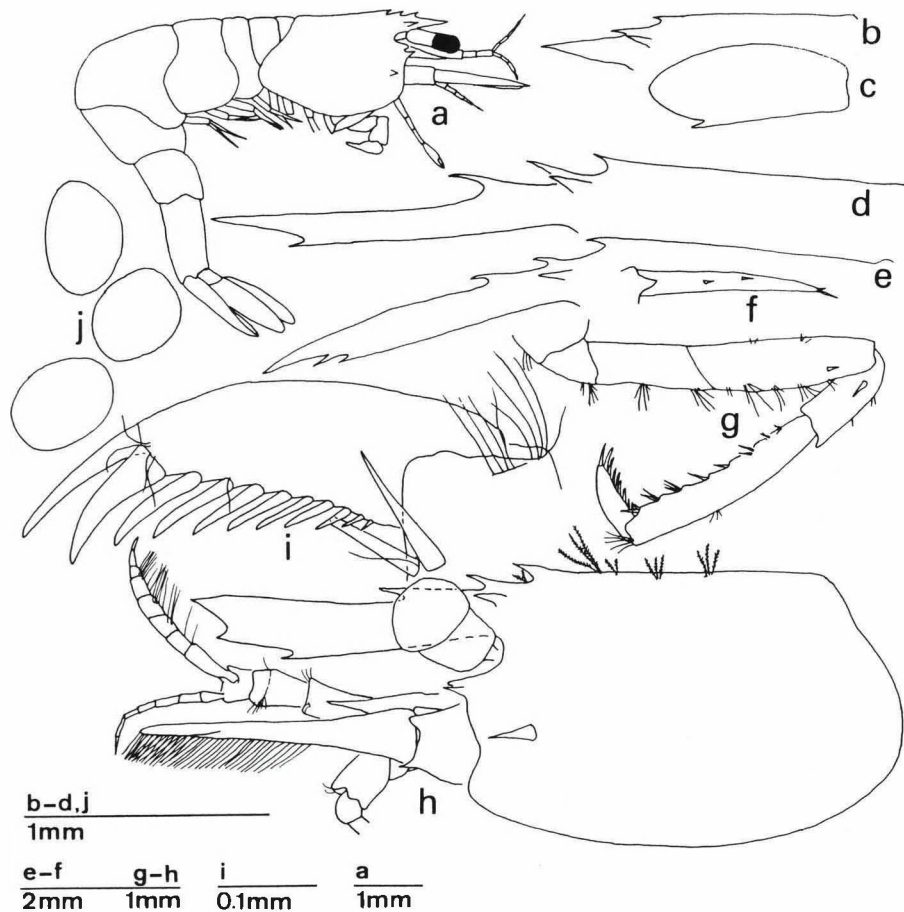
Fig. 23. Hippolyte leptocerus (Heller), a, female lectotype, Genova harbour (Museum of Natural History of Wien, Inv. Nr. 6752, after Kremer, 1990); b-c, female, Cape Verde Islands (RMNH 42897); d, ovigerous female, Madeira, Caniçal (RMNH D 42987); e-g, bopyrized female, Jersey (MNHN Na 14 675); h-j, mature female, Greece, Crete, NW of Souda Bay (RMNH). a, shrimps in toto; b, d, e, rostrum and dorsal part of carapace; c, left scaphocerite; f, telson in lateral view; g, left P5 [exceedingly rare disposition: meral spine present]; h, cephalothorax; i, dactylus of P3d; j, eggs with embryos.
