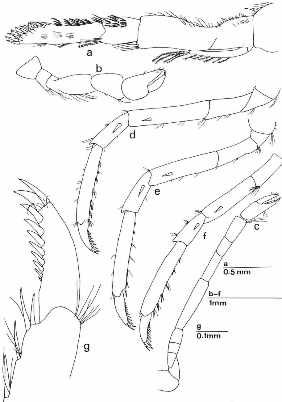
Fig. 9. Hippolyte garciarasoii spec. nov., Banyuls, female paratype (RMNH D 45590). a, right Mxp3; b, right P1; c, right P2; d, left P3; e, left P4; f, left P5; g, dactylus of left P3.
