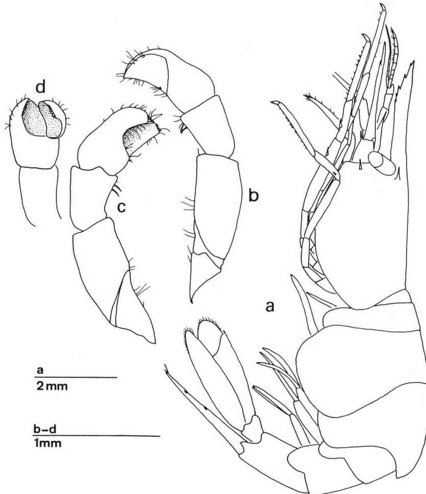
Fig. 34. Hippolyte prideauxiana Leach, female, NW Greece, fishermen of Lygia (RMNH). a, shrimp in toto; b-d, left P1 seen in different orientations.
