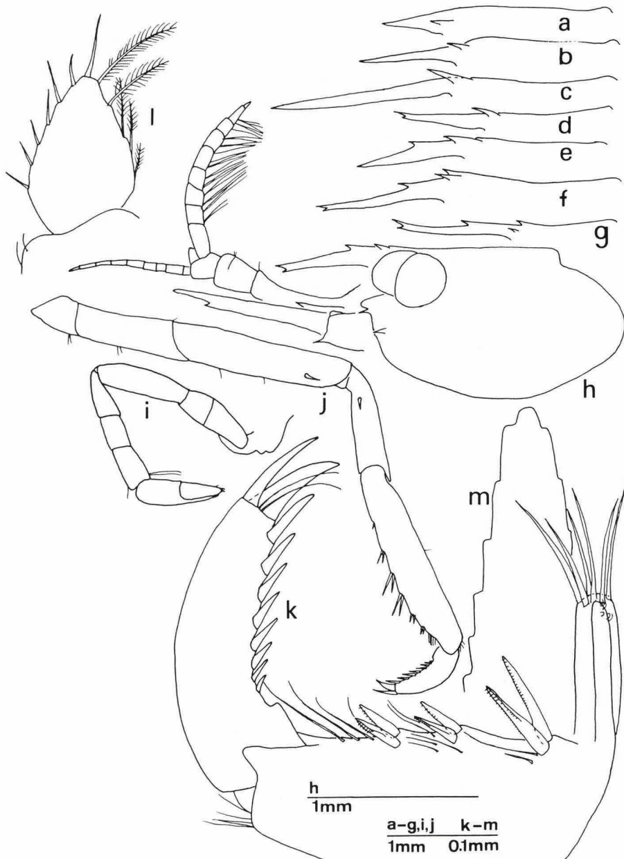
Fig. 21. Hippolyte leptocerus (Heller), males; a-f, Brittany, Roscoff (MNHN); g, Greece, Crete, NW of Souda Bay (RMNH); h-m, NW Greece, Gulf of Amvrakikos, NW of Koronissia [St. E9] (RMNH). a-g, rostrum and dorsal part of carapace; h, cephalothorax; i, left P2; j, right P3; k, dactylus of right P3; l, endopodite of first left male pleopod; m, endopodite of second left male pleopod.
