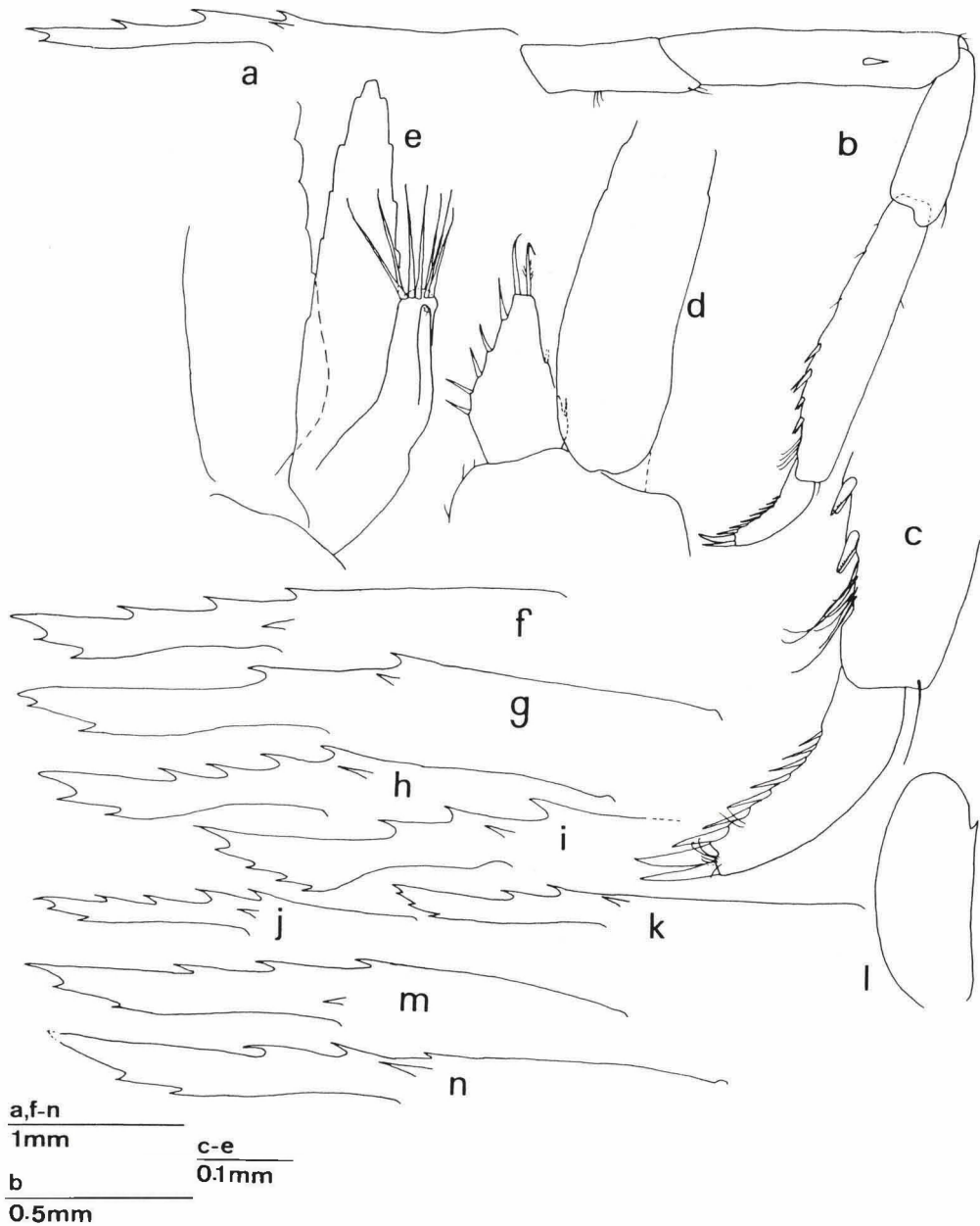
Fig. 10. a-j, m-n: Hippolyte garciaraso spec. nov., k-l: Hippolyte cf. garciaraso spec. nov. (incomplete specimen): a-e: male, S Peloponnese, Vinglafia (RMNH); f-i, females, Bay of Biscay, Bassin d'Arcachon, between Le Four and Lède-des-Oies (f = commonest rostral formula) (RMNH); j, female, S Peloponnese, Archangelos (RMNH); k-l, male, Morocco, Témara (MNHN Na 14 774); m-n, females, "Adriatic - Cadiz harbour" (BM 1911 11 8. 1683-1684). a, f-k, m-n, rostrum and dorsal part of carapace; b, right third male pereopod; c, idem, dactylus; d, first right male pleopod; e, second right male pleopod; l, right scaphocerite.
