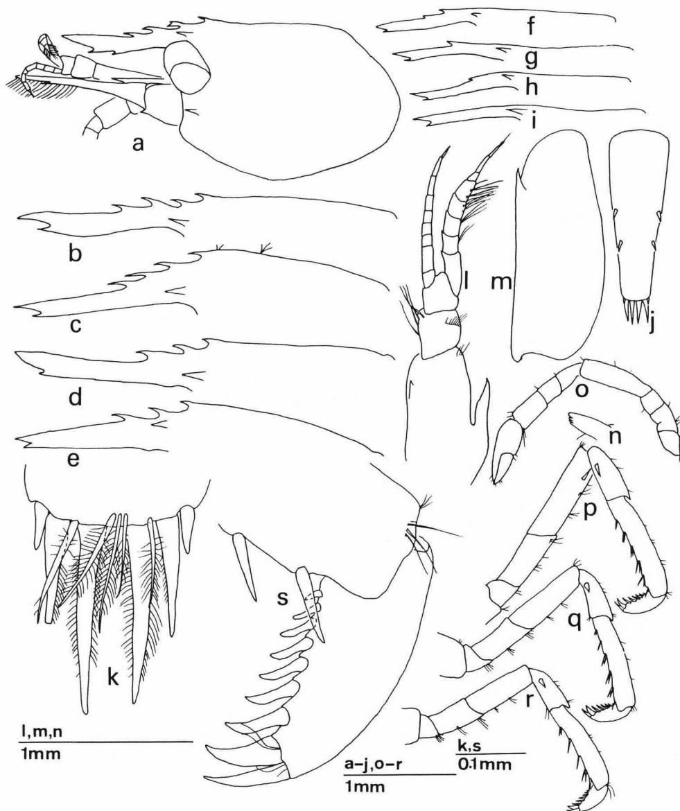
Fig. 22. Hippolyte leptocerus (Heller), Black Sea: a-e, j-s, females (a,b: MNHN Na 14 744; c-e, j-r, MNHN Na 14 743); f-i, males (MNHN Na 14 741 and 14 742). a, cephalothorax; b-i, rostrum and dorsal part of carapace; j, telson; k, tip of telson; l, right antennula; m, left scaphocerite; n, incisor of left mandible; o, left P2; p, right P3; q, right P4; r, right P5; s, dactylus of right P3.
