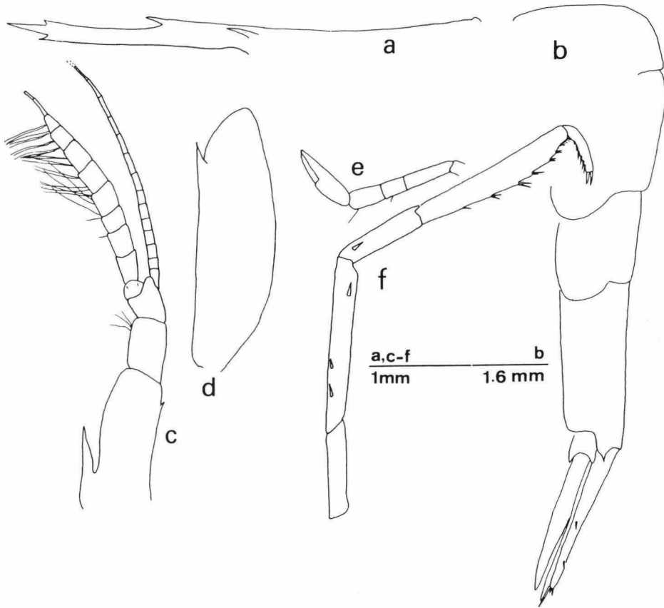
Fig. 50. Hippolyte varians Leach, male, Banyuls (MNHN Na 14 669). a, rostrum and dorsal part of carapace; b, posterior part of pleon; c, left antennula; d, left scaphocerite; e, left P2; f, right P3.
