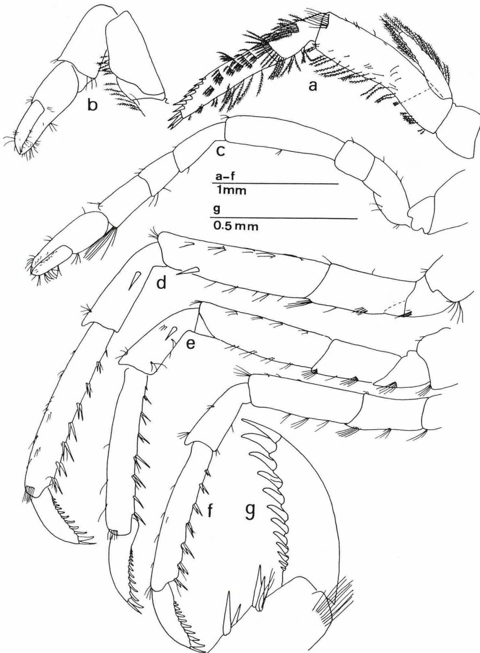
Fig. 20. Hippolyte leptocerus (Heller), mature female, Portugal, Algarve, Carveiro (RMNH). a, left Mxp3; b, left P1; c, left P2; d, left P3; e, left P4; f, left P5; g, dactylus of left P3.
