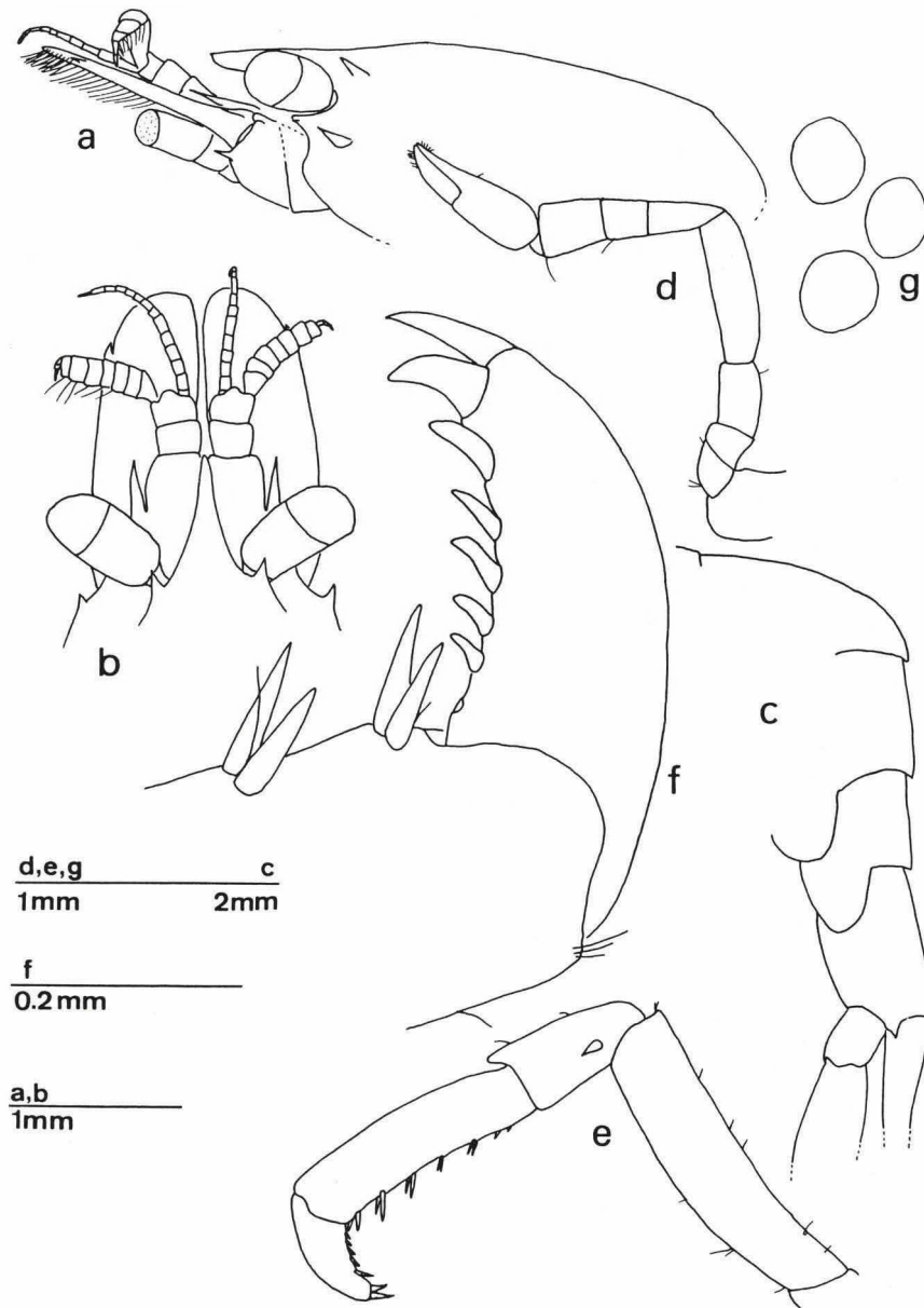
Fig. 30. Hippolyte palliola Kensley, mature female, Congo, Pointe Kounda (MNHN Na 1685). a, cephalothorax in lateral view; b, anterior part of cephalothorax in dorsal view; c, posterior part of pleon; d, left P2; e, left P3; f, dactylus of left P3; g, eggs recently laid.
