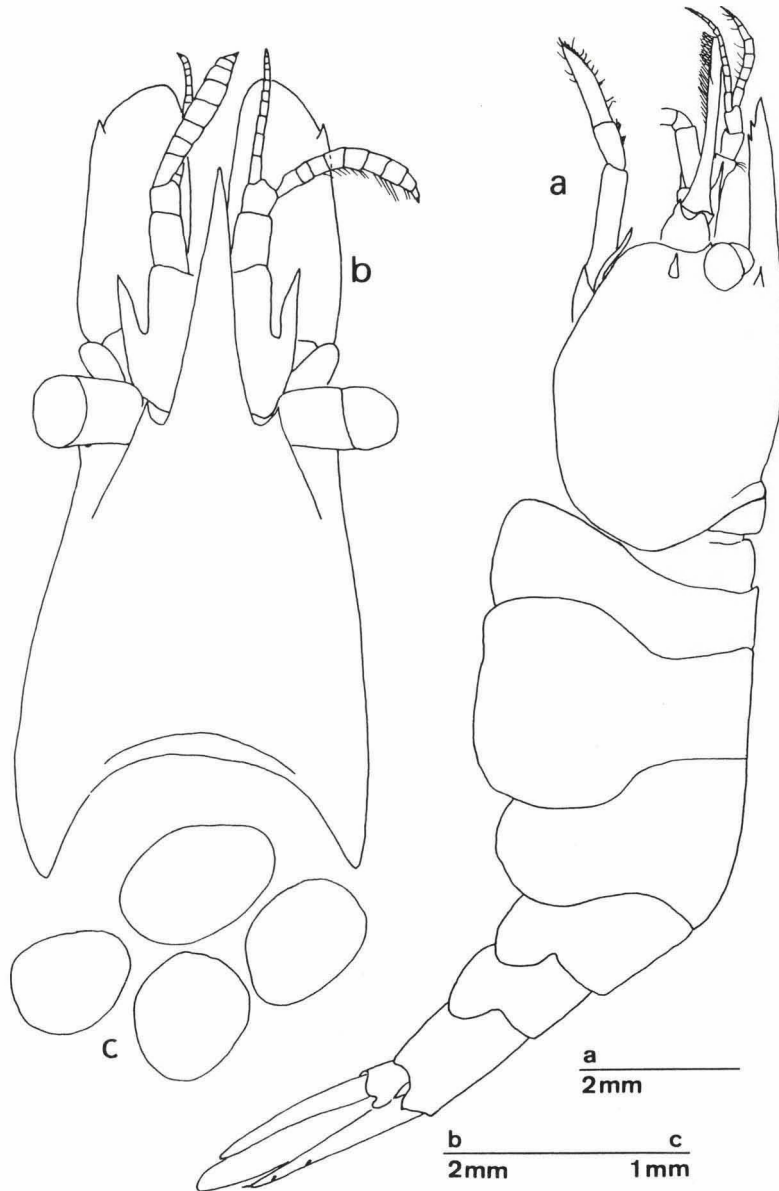
Fig. 31. Hippolyte prideauxiana Leach, mature female, Brittany, Roscoff (MNHN Na 14 651/14 654). a, body in lateral view; b, cephalothorax in dorsal view; c, eggs with embryos.
