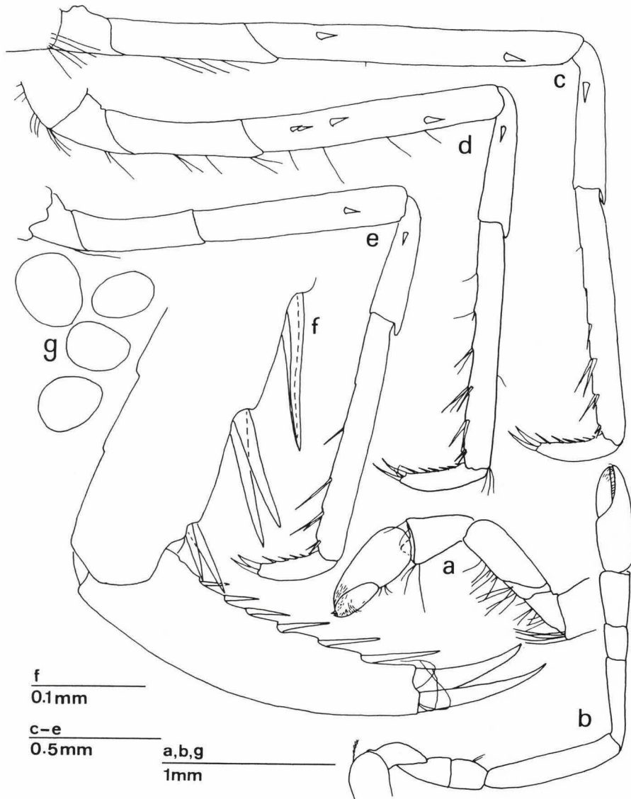
Fig. 27. Hippolyte niezabitowskii spec. nov., mature female paratype, NW Greece, Drepanos [St. E1] (RMNH). a, left P1; b, left P2; c, right P3; d, right P4; e, right P5; f, dactylus of left P3; g, eggs with embryos.
