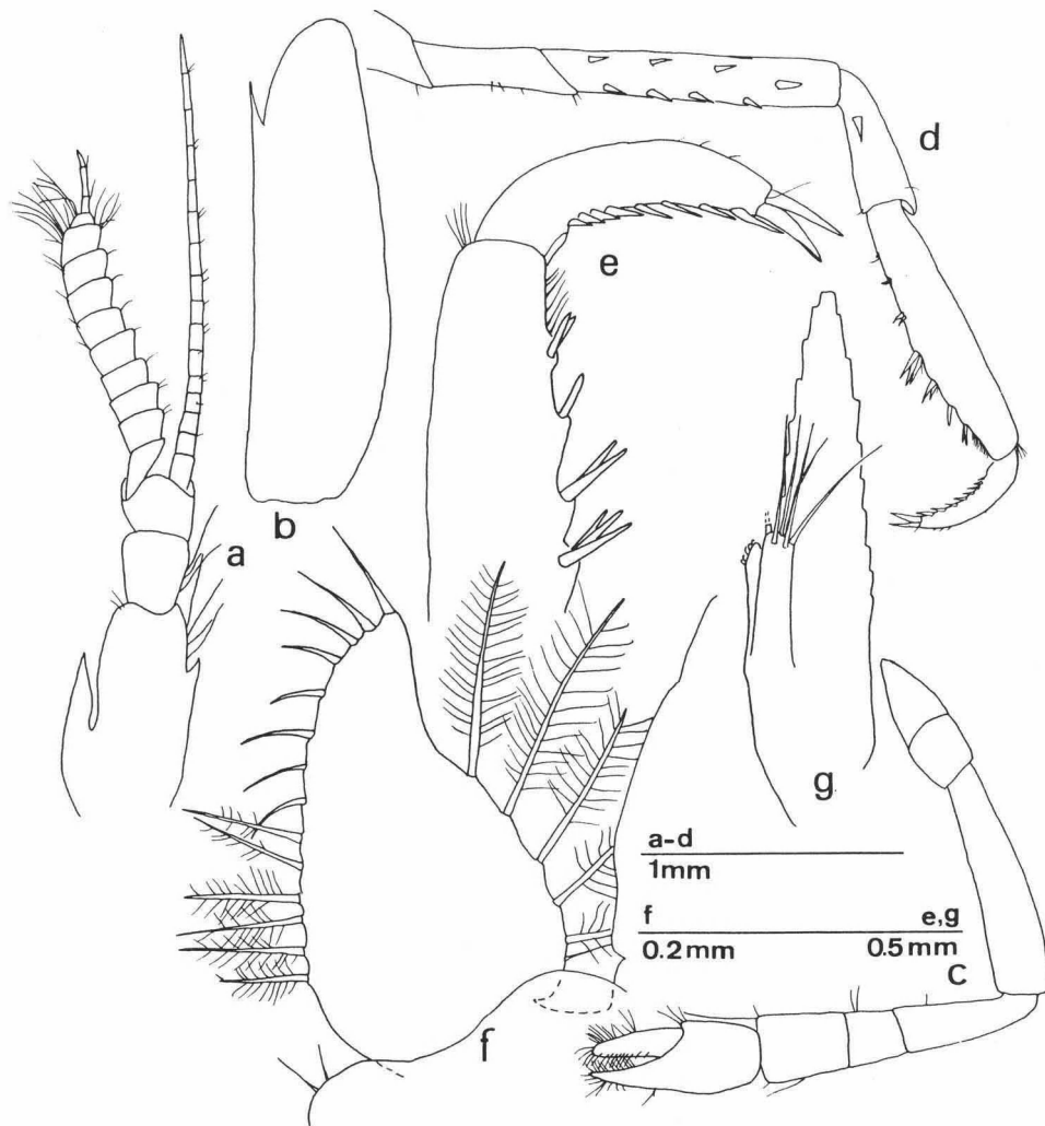
Fig. 14. Hippolyte inermis Leach, male, NW Greece, Lygia [St. E6] (RMNH). a, left antennula; b, left scaphocerite; c, right P2; d, right P3; e, dactylus of right P3; f, endopodite of first right pleopod; g, second right pleopod.
