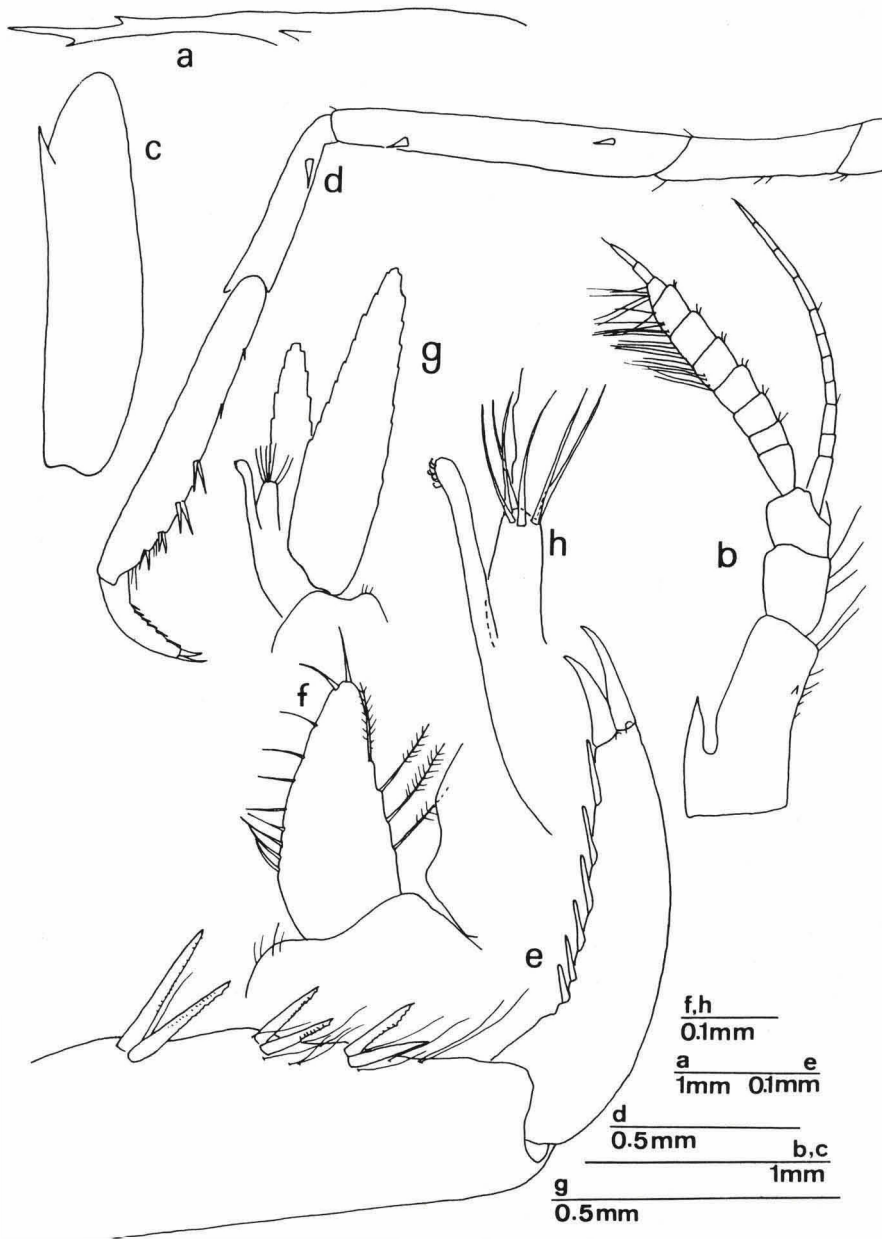
Fig. 28. Hippolyte niezabitowskii spec. nov., male, Croatia, Rovinj (RMNH). a, rostrum and dorsal part of carapace; b, left antennula; c, left scaphocerite; d, left P3; e, dactylus of left P3; f, endopodite of first left pleopod; g, second right pleopod; h, appendix masculina and interna of second right pleopod.
