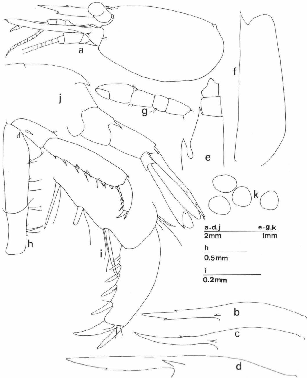
Fig. 3. Hippolyte coeruleuscs (Fabricius), a, e-g, j-f female, W Africa near to Annobon island (MNHN Na 8812); b-d, h-i, females, mid-Atlantic (MNHN Na 8261). a, cephalothorax; b-d, rostra and dorsal part of carapace; e, antennular peduncle; f, left scaphocerite; g, second left pereopod; h, right pereopod of one of the last three pairs; i, idem, dactylus; j, posterior part of pleon; k, eggs with embryos.
