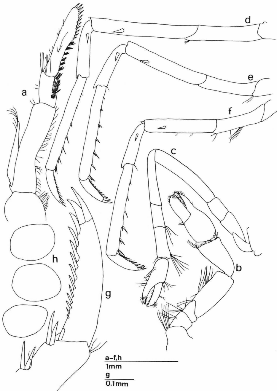
Fig. 42. Hippolyte sapphica d'Udekem d'Acoz forma B, NW Greece, Agia Triada [St. E8] (RMNH), mature females. a, left Mxp3; b, left P1; c, left P2; d, left P3; e, left P4; f, left P5; g, dactylus of left P3; h, eggs with embryos (other specimen).
