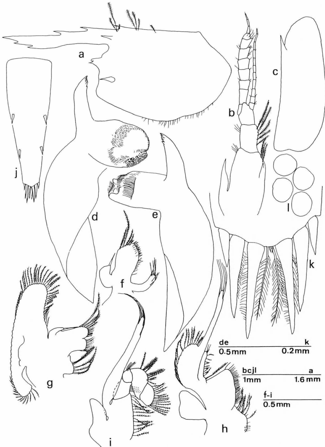
Fig. 8. Hippolyte garciaraso spec. nov., Banyuls, female paratype (RMNH D 45590). a, carapace; b, left antennula; c, left scaphocerite; d, right Md; e, left Md, f, right Mx1; g, right Mx2; h, right Mxp1; i, right Mxp2; j, telson; k, tip of telson; l, eggs with embryos.
