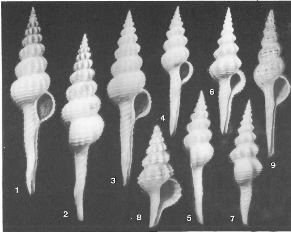
FIGS. 1-9. Western Atlantic Fusinus : 1. F. stegeri , n. sp., holotype, 102 mm, USNM 749082; 2. same, lateral view; 3. F. stegeri , paratype, 97 mm, BMNH 197810; 4. F. stegeri , paratype, 70.4 mm, ANSP 345472; 5. same, lateral view; 6. F. eucosmius , 73.8 mm, Hourglass Sta. C, 27° 37' N, 83° 28' W, depth 37 m, FSBC I 2284; 7. same, lateral view; 8. F. ampliurgus , holotype, 14 mm, USNM 508725; 9. F. halistreptus , holotype, 80 mm, USNM 93333.
