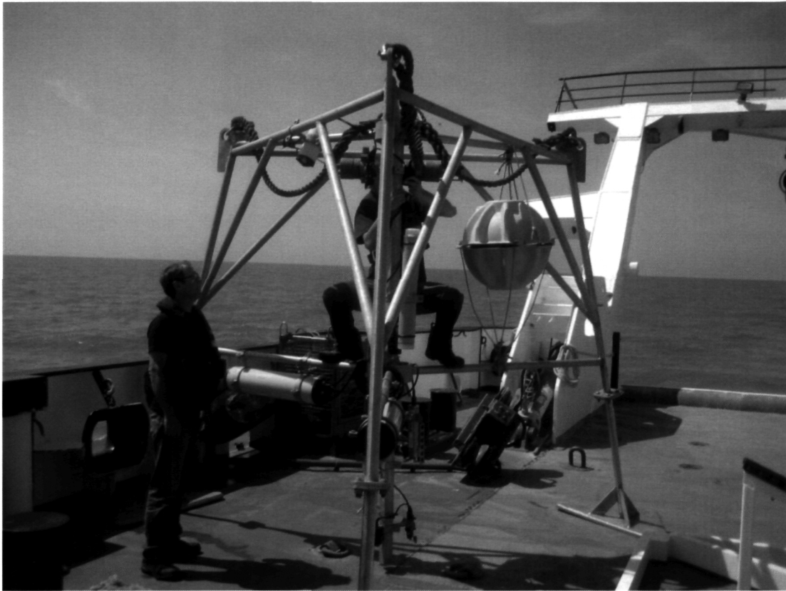
Figure 6.1. Tripod as used to deploy the underwater noise recorder to the seabed
