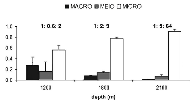
FIG. 3. – Mean ratios for the prokaryotes (MICRO), meiofauna (MEIO) and macrofauna (MACRO) biomass values on total benthic biomass (mgC m 2 ) for the three increasing depths. Data are means ± standard deviation. Ratios for macro:meio:micro are also shown.
