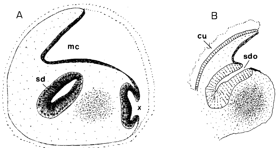
Figure 15. Notomenia clavigera : transverse sections of holotype to demonstrate openings of spawning ducts into mantle cavity. A. Section close to body end (after Thiele, 1902: fig. 16, supplemented by original body wall, stippled). B. Section further posterior to A , through opening of left spawning duct. Abbreviations: cu, mantle cuticle; mc, mantle cavity; sd, spawning duct; sdo, opening of left spawning duct into mantle cavity; x, artificial opening (by rupture) of right spawning duct.
