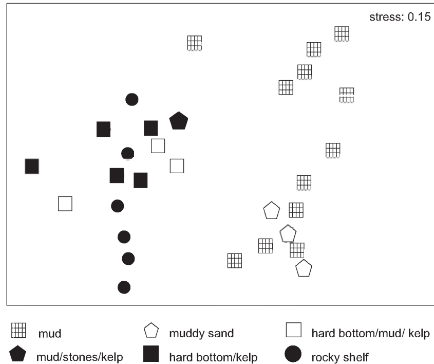
Fig. 4. The MDS plot of fourth-root-transformed data of taxa abundance in samples. The superimposed symbols indicate the bottom type at the sampling station.
