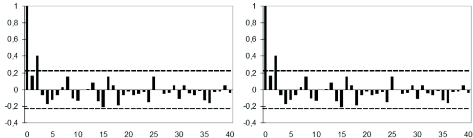
Fig. 6.3. ACF (left) and PACF (right) with half-year lags, after subtracting the linear trend and the seasonal signal from the brown shrimp abundance data.
