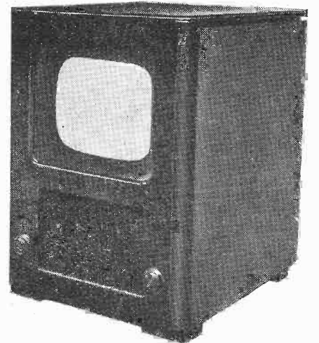
H.M.V. television receiver, Type 1800.
