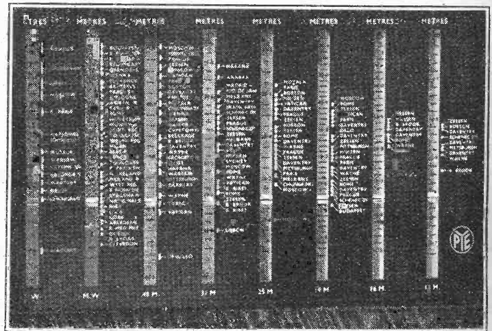
Individual calibration of short-wave stations is a feature of the Pye "International" tuning dial.
