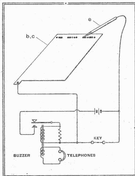
The electrical connections. The separate headphone winding may consist of a few turns of wire wound over the buzzer bobbins.
