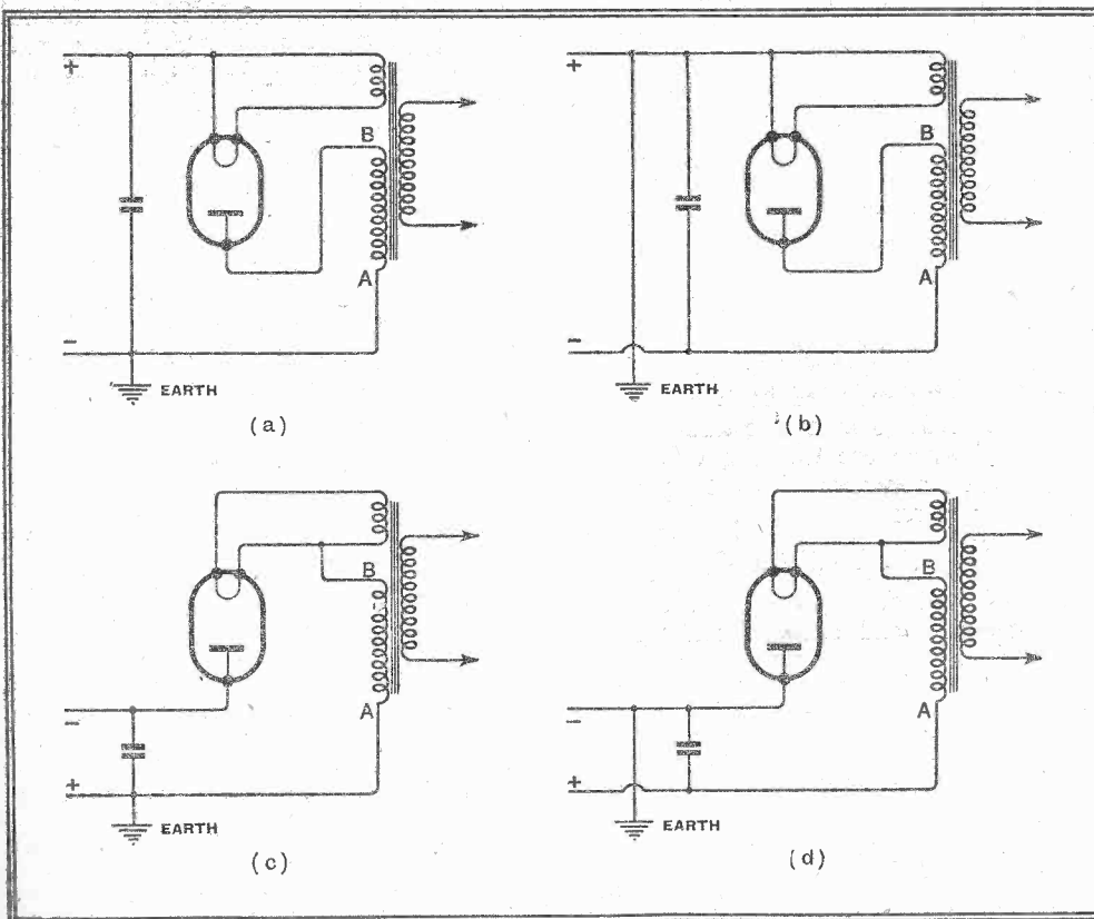
Fig. 5.—Several ways in which an HT rectifier can be arranged. The working voltages of the transformer windings are different in each case.
