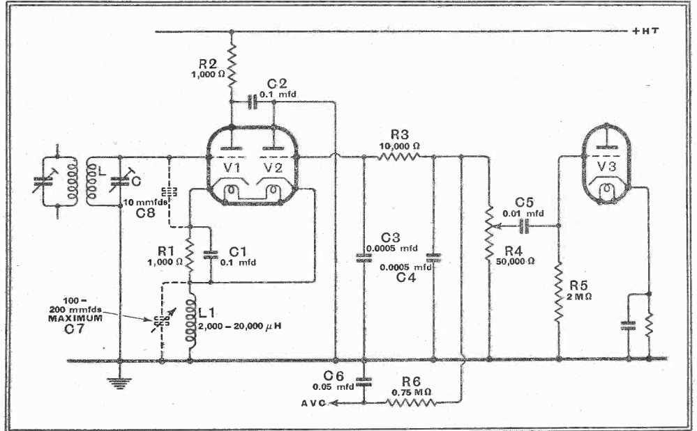
Fig. 8.—If separate valves are not used for each stage, the best arrangement is to employ a duo-triode as shown here. One triode section is used as a diode; the advantage over the diode-triode is that the cathodes are separate.
