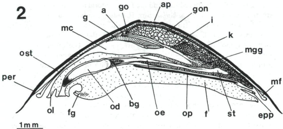
Fig. 2: Olgasolaris tollmanni gen. n. et sp. n. (longitudinal section, schematic, abbreviations see Material and Methods).
