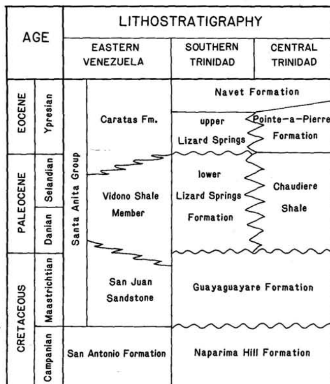
Fig. 2. Stratigraphic correlation of lithologic units in Trinidad and eastern Venezuela (from BARR & SAUNDERS, 1968, and SALVADOR & STAINFORTH, 1968). The positions of probable hiatuses are indicated by wavy lines.
