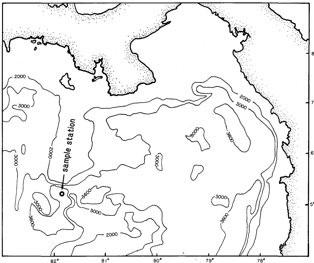
Fig. 1. Map of study area showing locations of sample station. Base map from VAN ANDEL et al. (1971), depth in meters.
