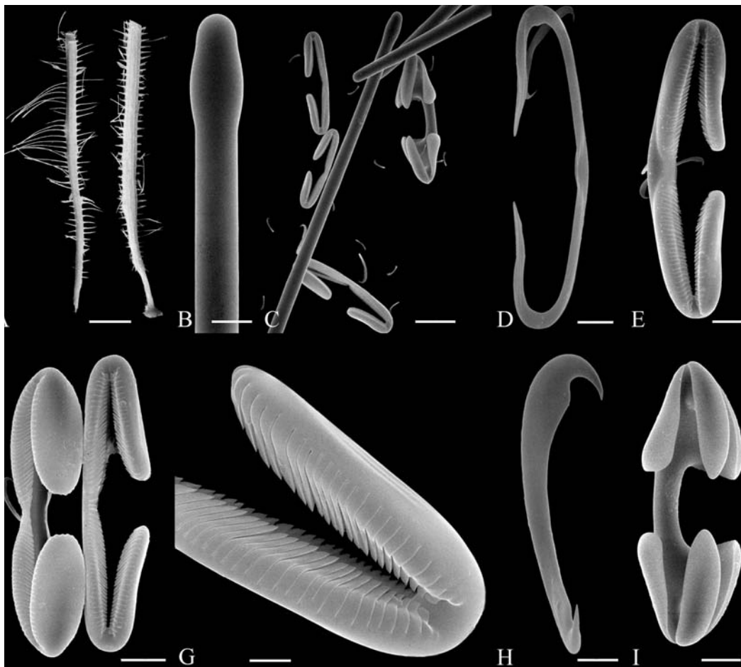
1A: Two specimens from Barbados; scale bar 4 mm; B: Head of a subtylostyle, Barbados; scale bar 10 \mu\text{m} ; C: Subtylostyles, placocheleae I and II, isochela, sigmancistras I and II, Barbados; scale bar 50 \mu\text{m} ; D: Immature placochele, holotype; scale bar 10 \mu\text{m} ; E: Placochele, holotype; scale bar 10 \mu\text{m} ; F: Placochele, Barbados; scale bar 15 \mu\text{m} ; G: Placochele, Barbados; scale bar 5 \mu\text{m} ; H: Sigmancistras I, Barbados; scale bar 2 \mu\text{m} ; I: Isochela, Barbados; scale bar 15 \mu\text{m} .
