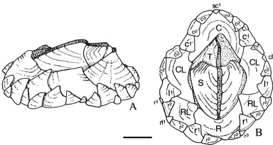
1A: Right side of the holotype; B: Above side of the same specimen; scale bar 1 mm; from YAMAGUCHI & NEWMAN (1997). Capital letters indicate the principal wall plates: R – rostrum; RL – rostrolateral; CL – carinolateral; C – carina; small letters indicate the imbricating plates
