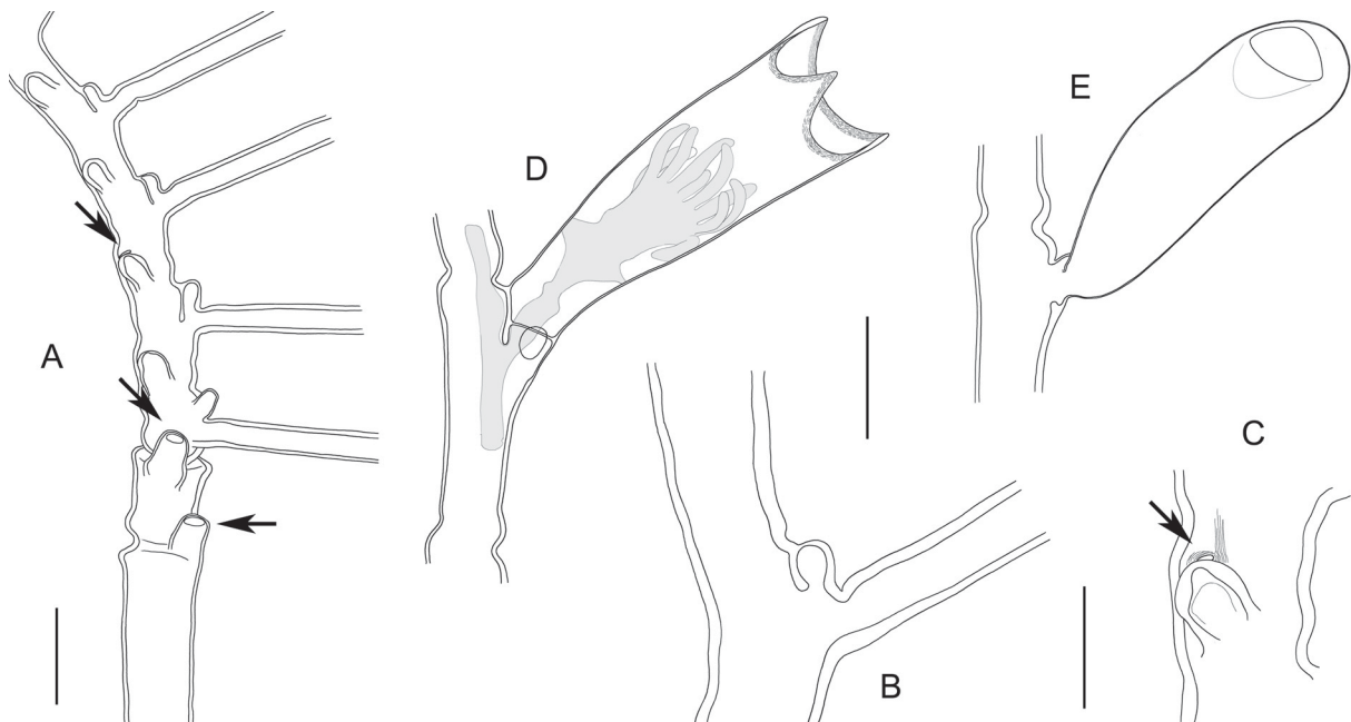
Fig. 18. Tuberoacaulus scorpioides (Vervoort, 1993) gen. et comb. nov. A–E. Junction between proximal and distal parts of stem (A), showing apically- or axillary-opened nematothecae (arrowheads), detail of insertion of cladium (B), upper stem nematotheca with aperture in axil (C, arrowhead), hydrotheca (D), gonotheca (E), all from sample MNHN-IK-2015-400. Scale bars: A = 1 mm; B–E = 500 \mu m.
