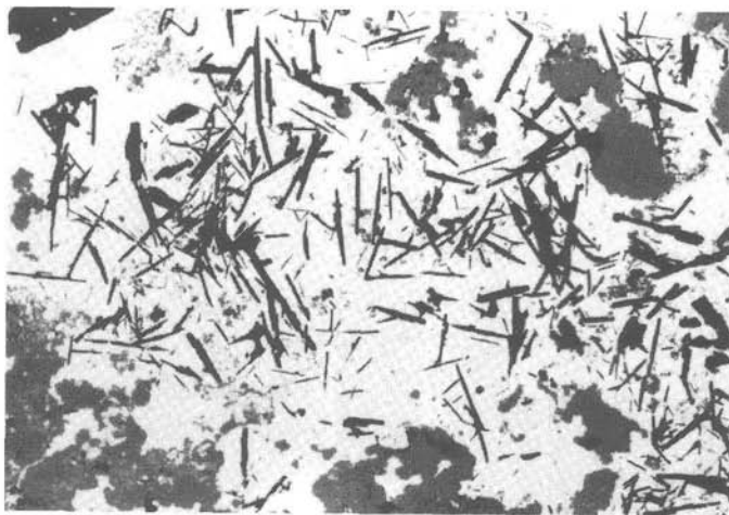
Fig. 38. Sample SO 41-181 FG 8 b. Pyrite (light gray, almost white), containing numerous inclusions of euhedral tabular barite platelets (black) of different size and schalenblende (dark gray) along with small amounts of galena (light gray). In places, the schalenblende also constitutes spheroids (upper right corner of photomicrograph). Polished section, \times 65 .
