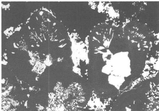
Fig. 33. Sample SO 41-181 FG 6. Rhythmic, concentrically layered schalenblende (dark gray in different shades — the slight variations in its reflectivity denote zoning) contains partly skeleton crystals of galena (light gray, almost white) in the center. In one aggregate of schalenblende (right half of photomicrograph) there is a small amount of galena adjacent to a lead sulfosalt, probably jordanite (slightly lower reflectivity than galena, in photomicrograph hardly distinguishable from galena), which locally exhibits radial inclusions in the peripheral parts of schalenblende (upper half of photomicrograph). Pyrite (almost white) overgrows schalenblende, also constituting interstitial fillings within its aggregates. Locally, the periphery of schalenblende shows delicate rhythmically layered alternations with galena. Gangue material, natural cavities and pores (all black). Polished section, oil immersion, \times 275 .
