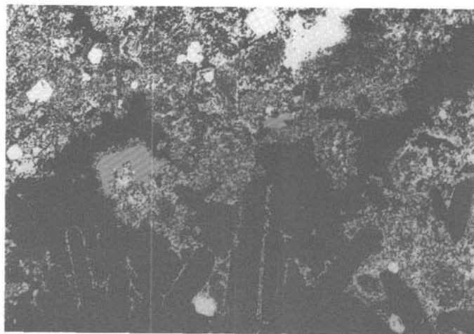
Fig. 31. Sample SO 41-181 FG 10. Euhedral plates of barite (black) rimmed by fine-grained, porous crystal aggregates of galena (light gray), which also fills interstices within the barite crystal aggregates. Within its masses of mostly fine-grained, porous crystal aggregates of the galena euhedral pyrite (light gray, almost white) and euhedral tennantite (medium gray) can be observed, both of which are rimmed by the galena crystal aggregates. Gangue material, natural cavities and pores (all likewise black). Polished section, oil immersion, \times 130 .
