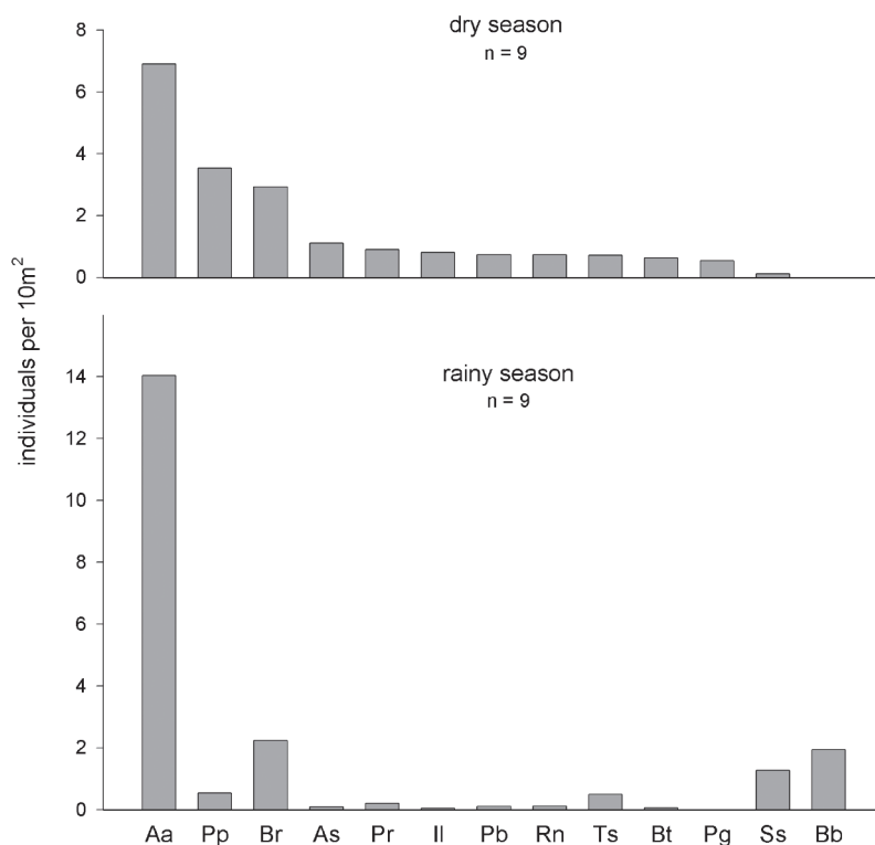
Fig. 3: Seasonal changes in density. Thirteen species in nine sites of all choritope types which were sampled in both seasons are compared. Only species with a density > 0.5 individuals per 10m 2 in any season are shown. Aa = Astyanax aeneus , Pp = Poeciliopsis paucimaculata , Br = Brachyrhaphis rhabdophora , As = Archocentrus sajica , Pr = Poeciliopsis retropinna , Il = Imparfinis lineatus , Pb = Piabucina boruca , Rg = Rhamdia guatemalensis , Ts = Tomocichla sieboldii , Bt = Bryconamericus terrabensis , Pg = Poecilia gillii , Ss = Sicydium salvini , Bb = Brycon behreae , n = sample size.
