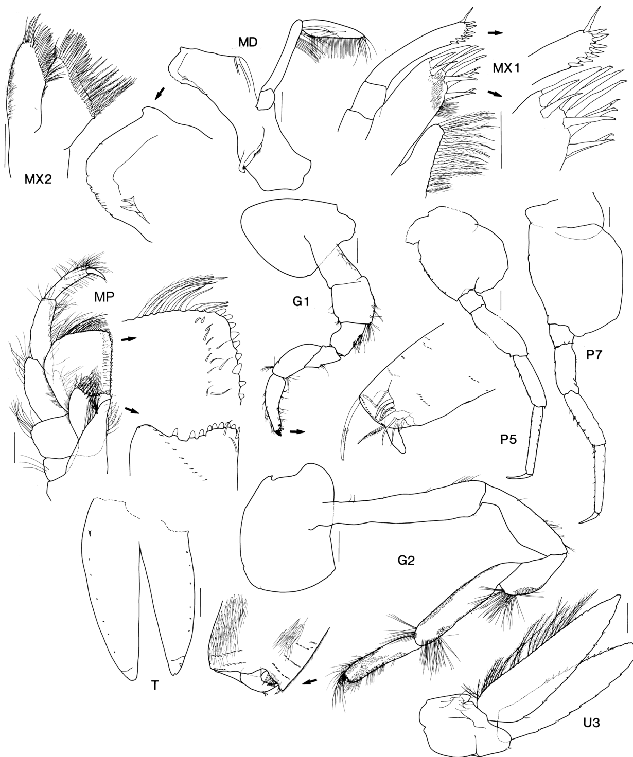
Figure 18. Bathycallisoma pacifica Dahl, 1959. Holotype female, 33 mm, ZMUC CRU-7674, Kermadec Trench. Scales for gnathopods, pereopods represent 1.0 mm; remainder represent 0.5 mm.
