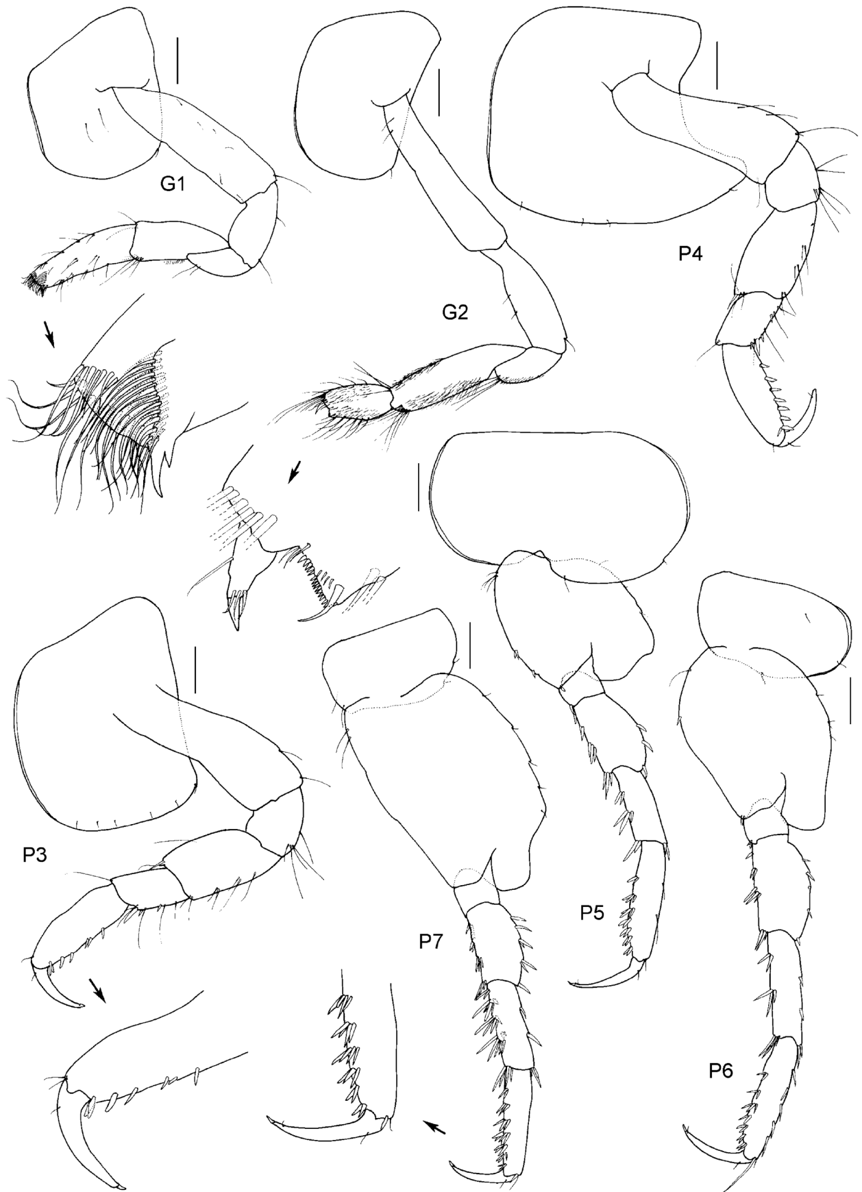
Figure 30. Paracallisoma woolgoolga sp. n. Holotype female, 10.0 mm, AM P.69088, from north-east of Coffs Harbour, New South Wales, Australia. Scales represent 0.2 mm.
