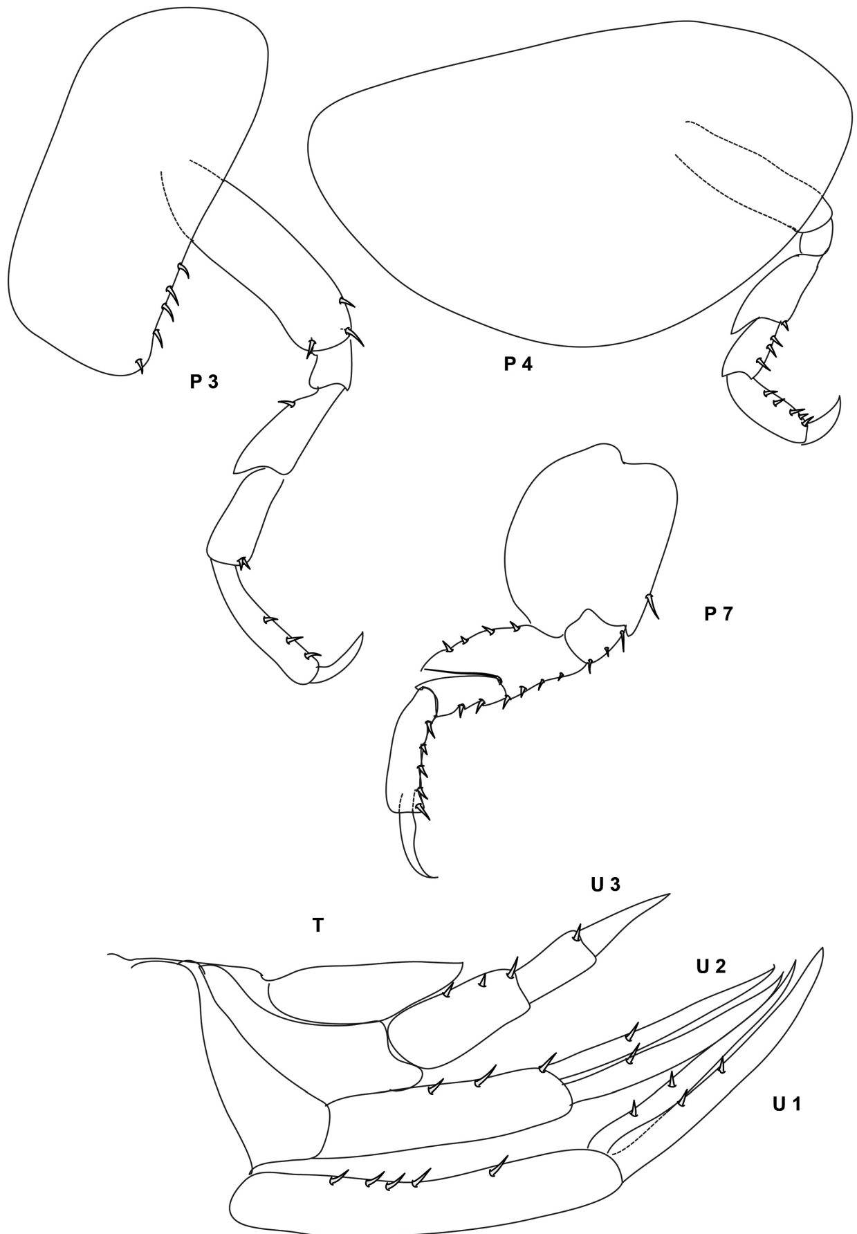
Figure 9. Metopa rubrovittata Sars, 1883 male 3 mm; P 3, 4, 7 peraeopod 3, 4, 7; U 1–3 uropod 1–3; T telson.
