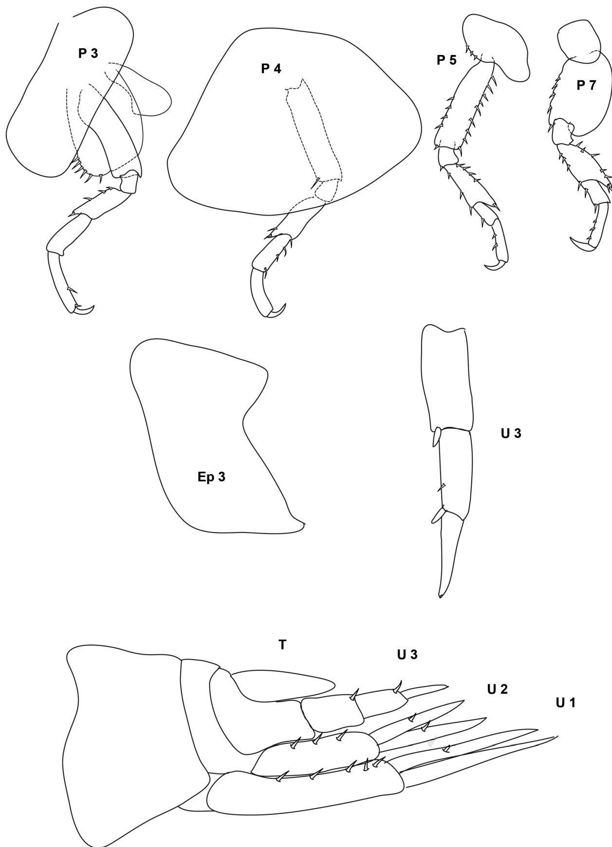
Figure 13. Stenula peltata (Smith, 1872): illustration of the single type specimen; P 3, 4 5, 7 peraeopod 3, 4, 5, 7; Ep 3 third epimeral plate; U 1, 2, 3 uropod 1, 2, 3; T telson.
