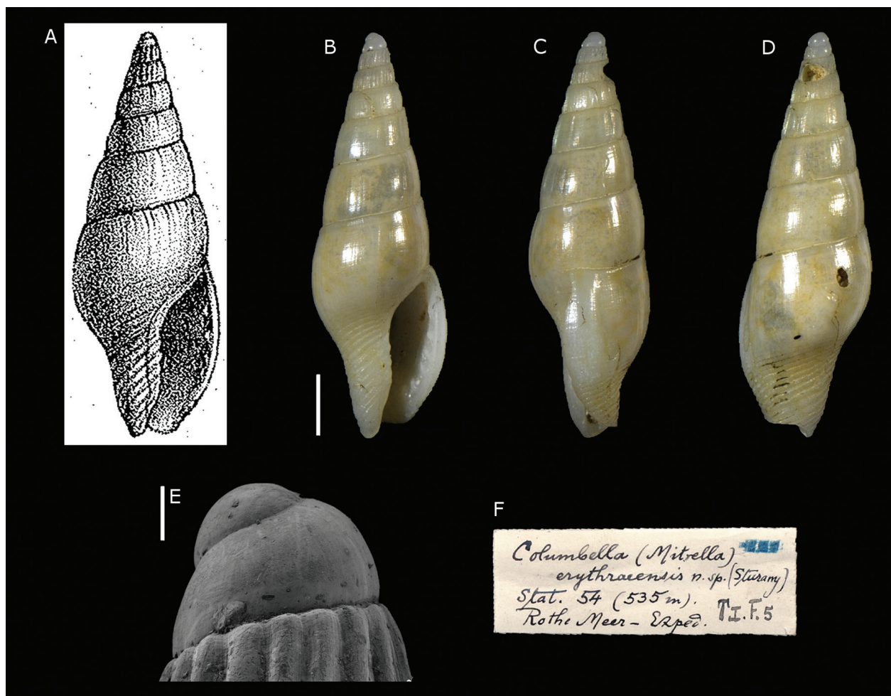
Figure 9. Columbella erythraeensis Sturany, 1900, Station 54 (Central Red Sea). A. Original figure by Sturany (1903). B–E. Holotype, NHMW 84221: front (B), right side (C), back (D), protoconch (E). F. Original holotype label. Scale bars: B–D: 2 mm, E: 0.2 mm.
