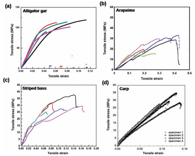
Figure 11. Comparison of the tensile response of (a) bone layer of a ganoid scale (alligator gar), [36] (b) a cosmoid scale (arapaima) (from Figure 13b in Ref. [43], reproduced with permission, 2011, Elsevier), (c) ctenoid scale (striped bass) (from Figure 3b in Ref. [25], reproduced with permission and (d) cycloid scale (carp) (from Figure 5b in Ref. [52], reproduced with permission, 2012, Elsevier). Each plot has the response of 4–5 specimens to show variation in mechanical response. The scales were all tested wet.
